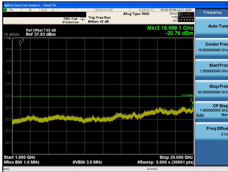
EGPRS1900-512-1000~20000
