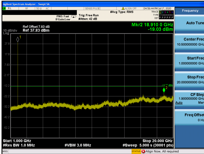
GSM1900-512-1000~20000
