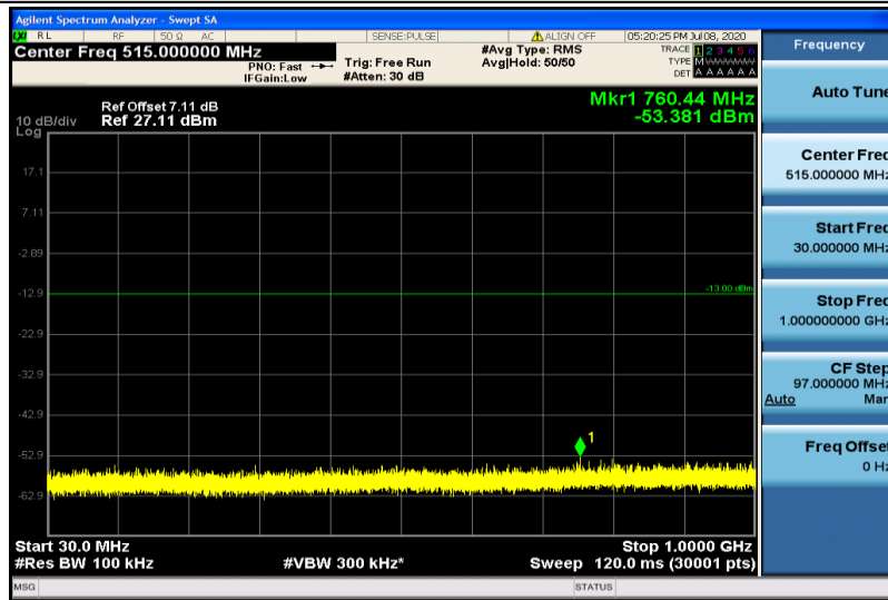
Band25-3MHz-QPSK-26055-1RB#0-30~1000MHz
