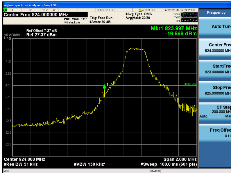
Band5-5MHz-QPSK-20425-1RB#0
