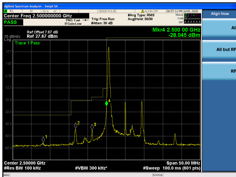
Band7-10MHz-QPSK-20800-1RB#0
