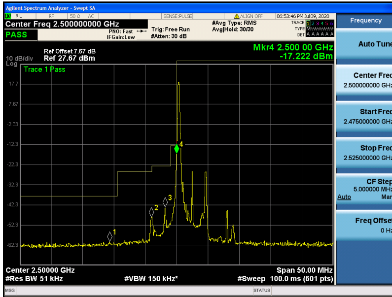
Band7-5MHz-QPSK-20775-1RB#0
