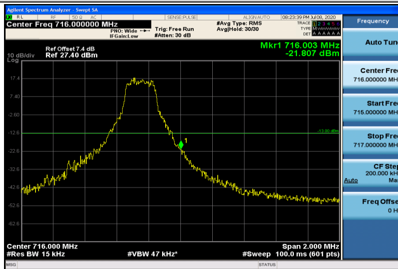
Band12-1.4MHz-QPSK-23173-1RB#5
