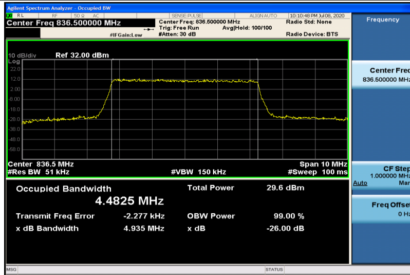
Band26-5MHz-16QAM-26915-25RB#0-4.4825
