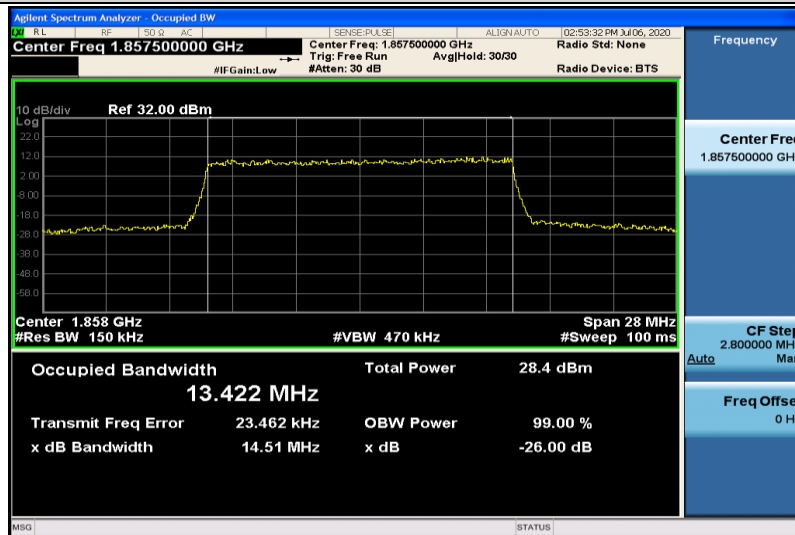
Band25-15MHz-16QAM-26115-75RB#0-13.422
