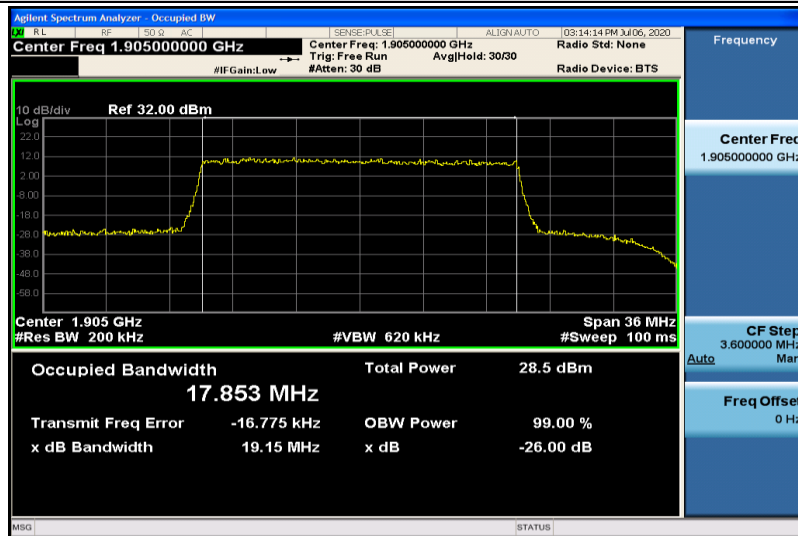
Band25-20MHz-16QAM-26590-100RB#0-17.853
