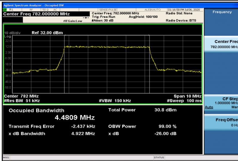
Band13-5MHz-QPSK-23230-25RB#0-4.4809
