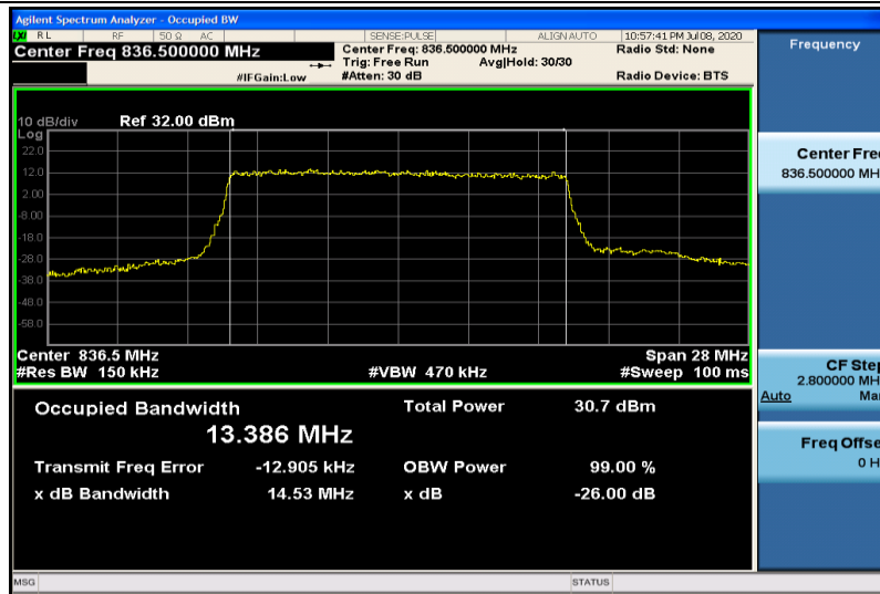
Band26-15MHz-QPSK-26915-75RB#0-13.386
