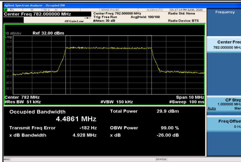
Band13-5MHz-16QAM-23230-25RB#0-4.4861
