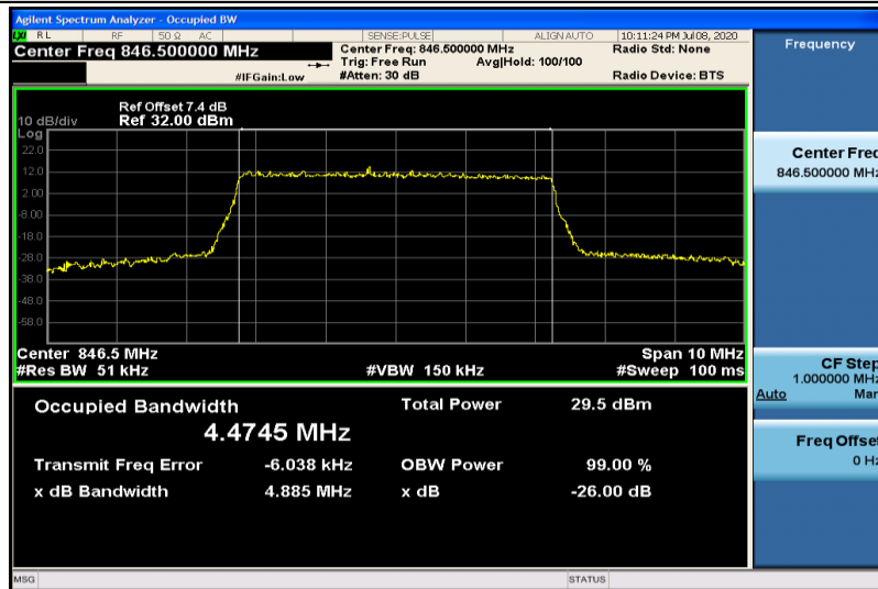
Band26-5MHz-16QAM-27015-25RB#0-4.4745
