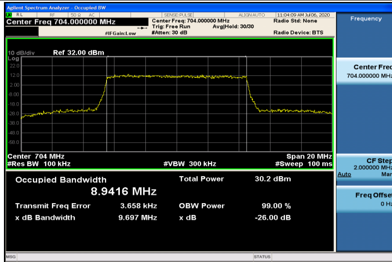
Band12-10MHz-16QAM-23060-50RB#0-8.9416
