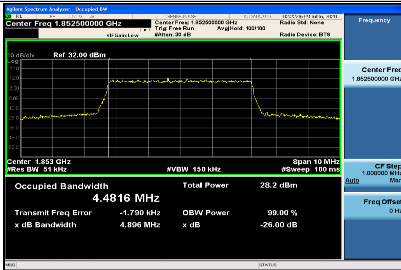
Band25-5MHz-16QAM-26065-25RB#0-4.4816
