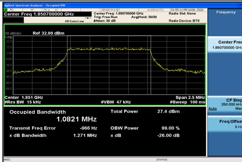
Band25-1.4MHz-16QAM-26047-6RB#0-1.0821
