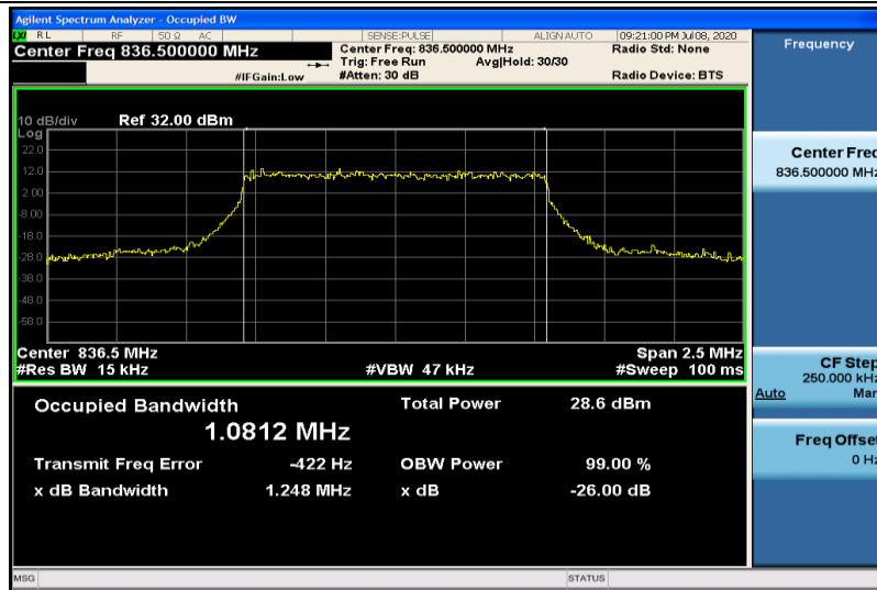
Band26-1.4MHz-16QAM-26915-6RB#0-1.0812
