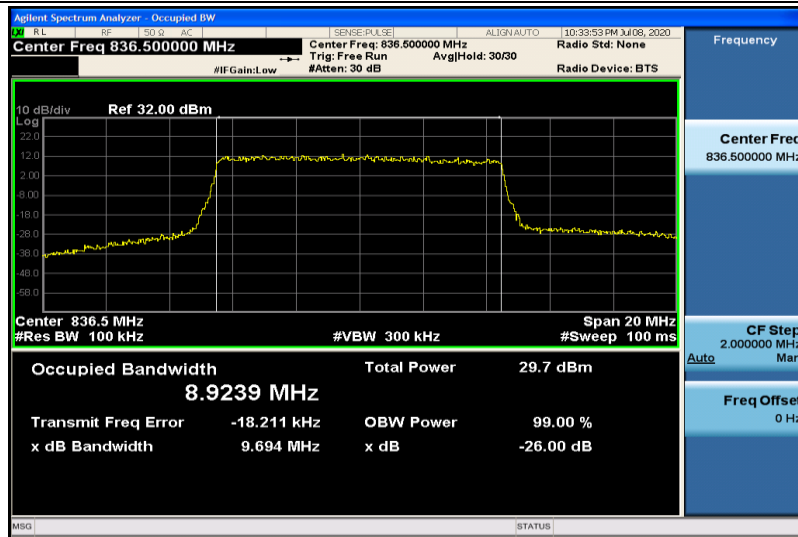
Band26-10MHz-16QAM-26915-50RB#0-8.9239
