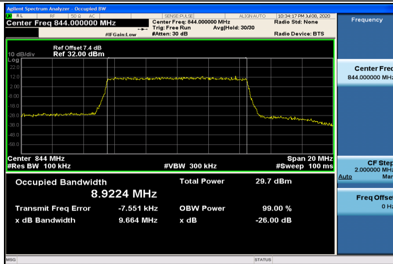
Band26-10MHz-16QAM-26990-50RB#0-8.9224
