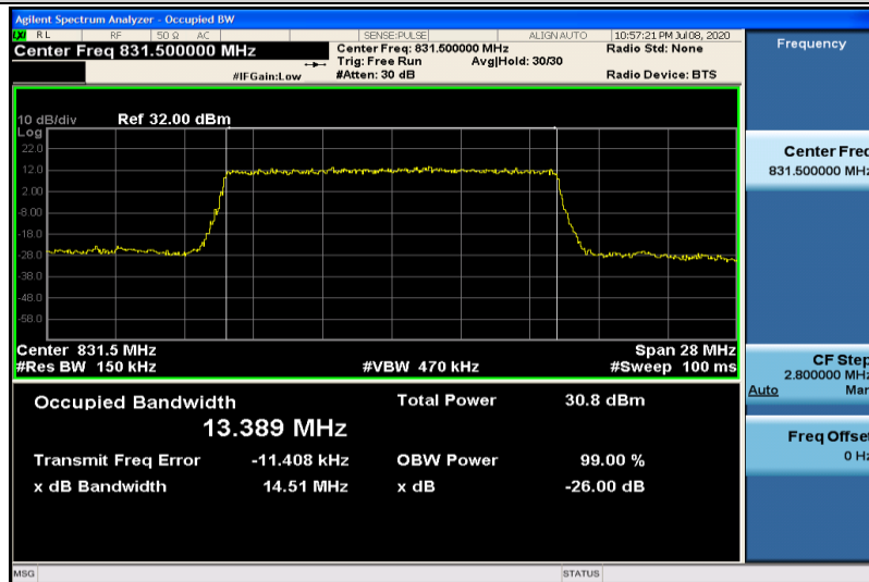
Band26-15MHz-QPSK-26865-75RB#0-13.389
