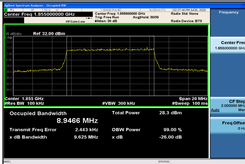
Band25-10MHz-16QAM-26090-50RB#0-8.9466
