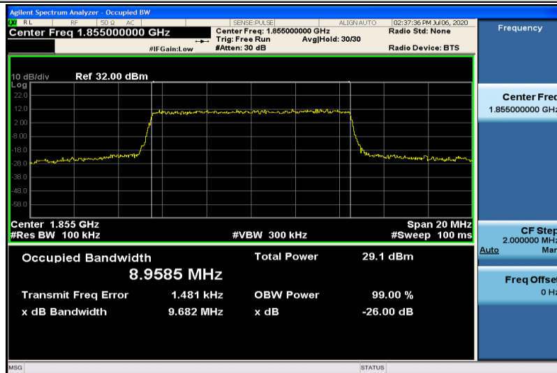
Band25-10MHz-QPSK-26090-50RB#0-8.9585
