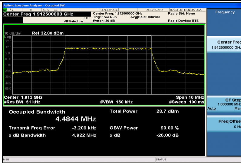
Band25-5MHz-QPSK-26665-25RB#0-4.4844
