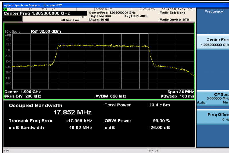
Band25-20MHz-QPSK-26590-100RB#0-17.852
