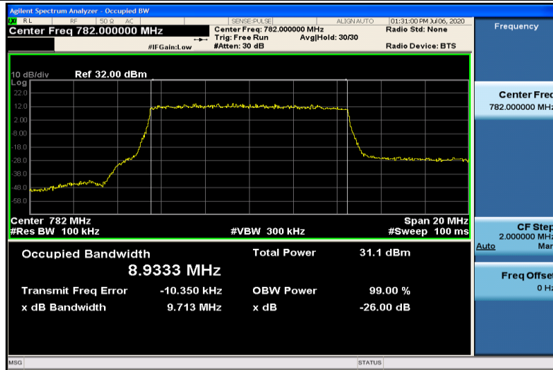
Band13-10MHz-QPSK-23230-50RB#0-8.9333
