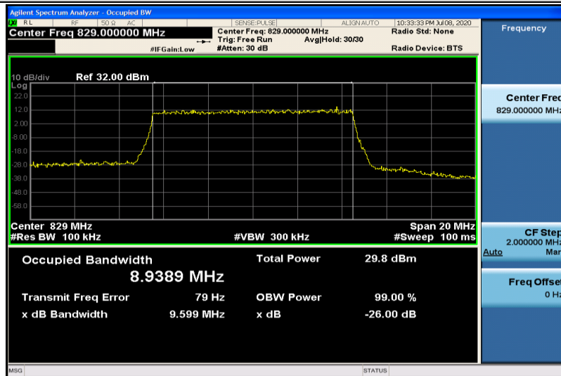
Band26-10MHz-16QAM-26840-50RB#0-8.9389
