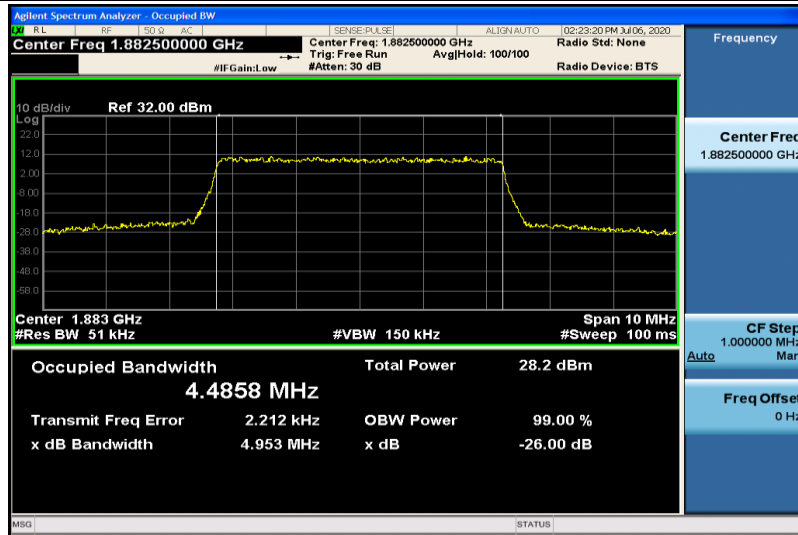
Band25-5MHz-16QAM-26365-25RB#0-4.4858
