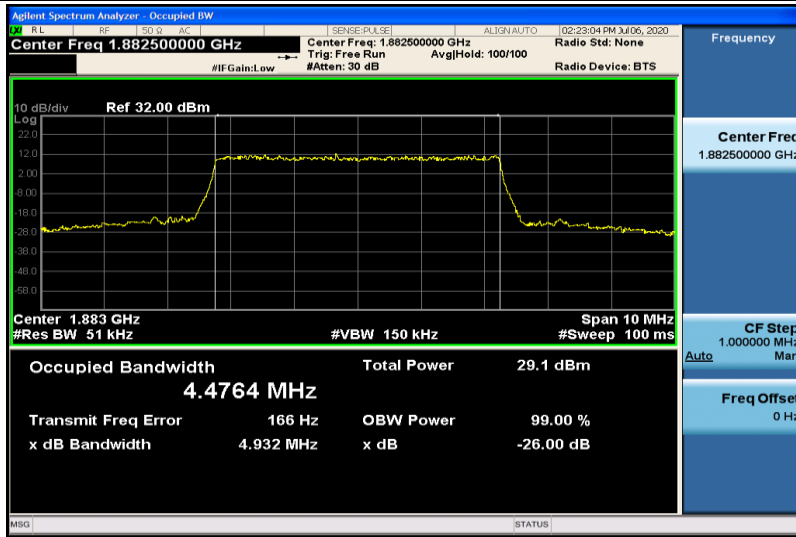
Band25-5MHz-QPSK-26365-25RB#0-4.4764
