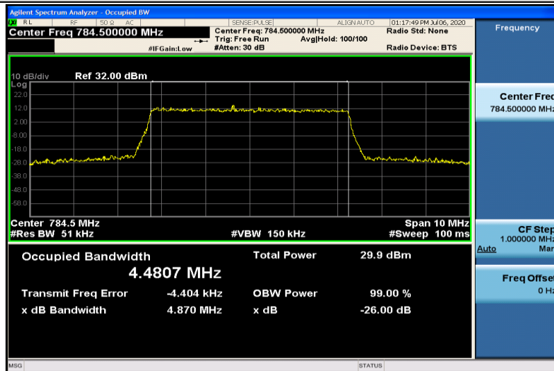
Band13-5MHz-16QAM-23255-25RB#0-4.4807
