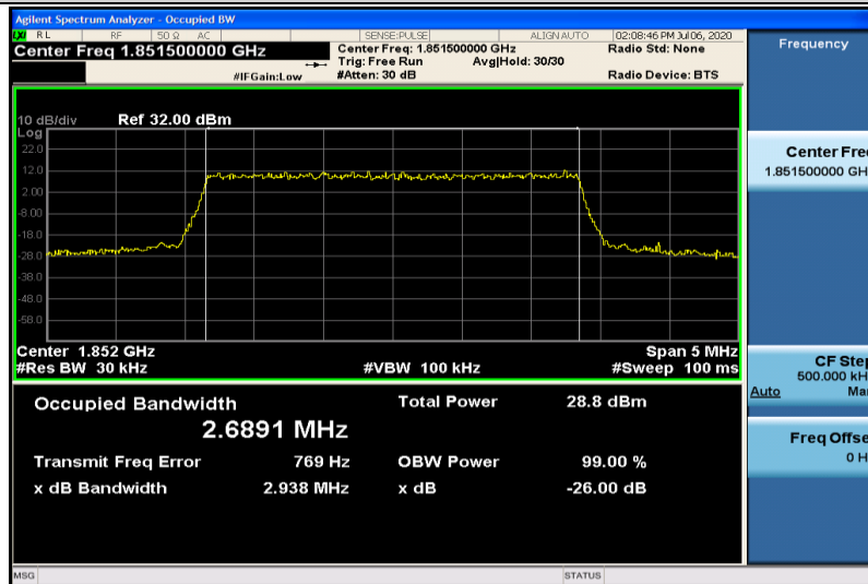
Band25-3MHz-QPSK-26055-15RB#0-2.6891
