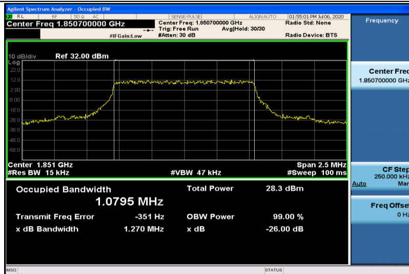
Band25-1.4MHz-QPSK-26047-6RB#0-1.0795
