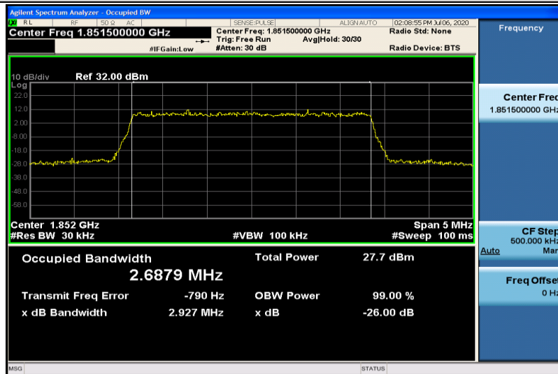
Band25-3MHz-16QAM-26055-15RB#0-2.6879
