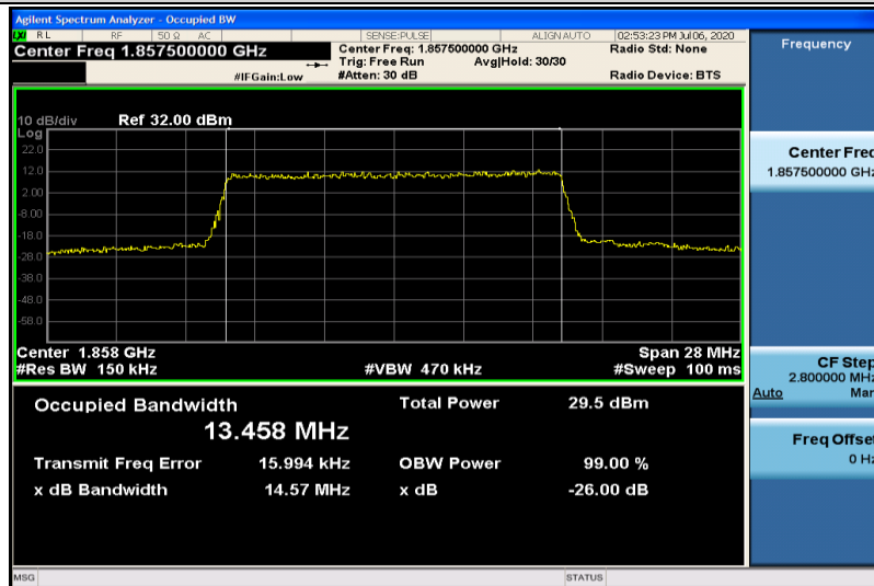
Band25-15MHz-QPSK-26115-75RB#0-13.458
