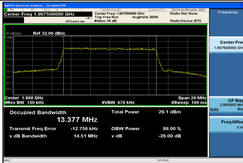
Band25-15MHz-QPSK-26615-75RB#0-13.377
