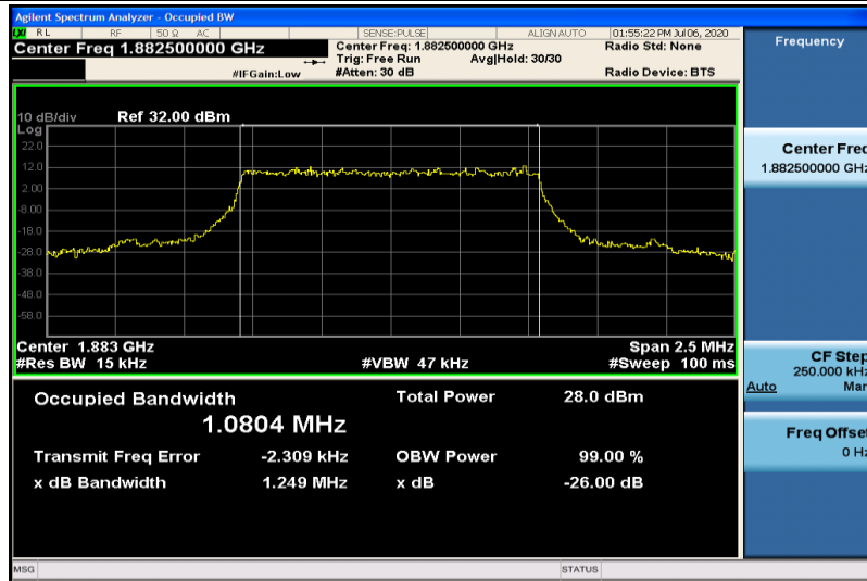
Band25-1.4MHz-QPSK-26365-6RB#0-1.0804
