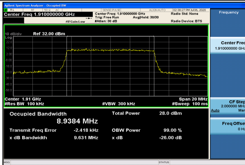
Band25-10MHz-16QAM-26640-50RB#0-8.9384
