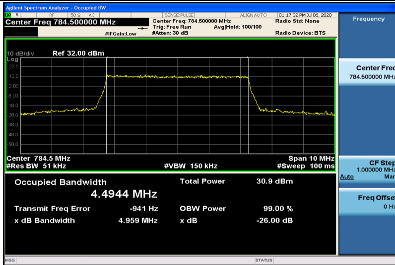
Band13-5MHz-QPSK-23255-25RB#0-4.4944
