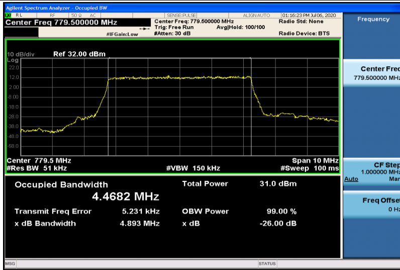
Band13-5MHz-QPSK-23205-25RB#0-4.4682
