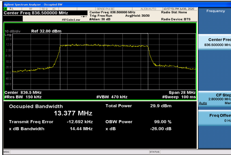
Band26-15MHz-16QAM-26915-75RB#0-13.377
