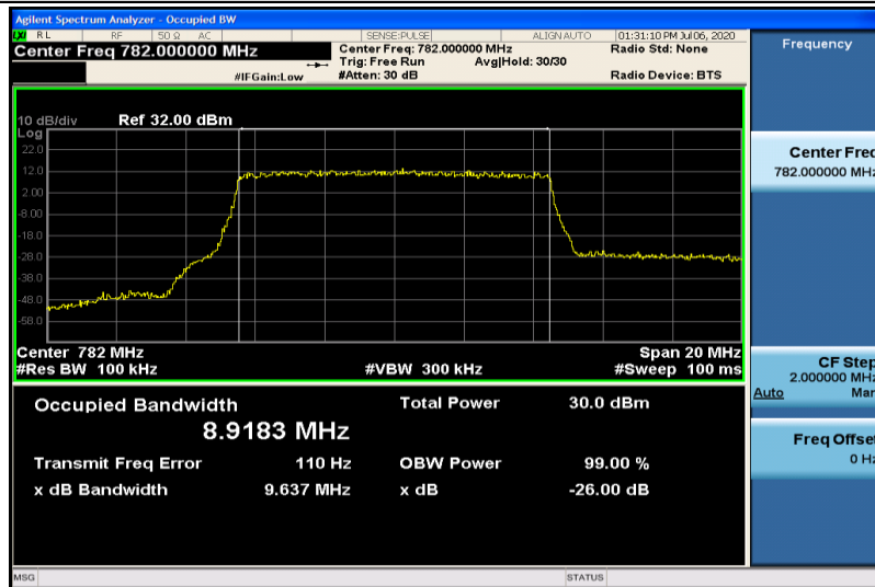
Band13-10MHz-16QAM-23230-50RB#0-8.9183
