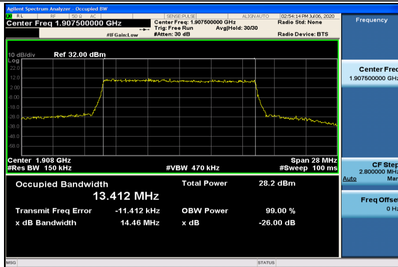
Band25-15MHz-16QAM-26615-75RB#0-13.412
