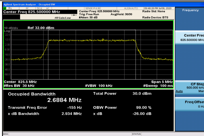
Band26-3MHz-QPSK-26805-15RB#0-2.6884
