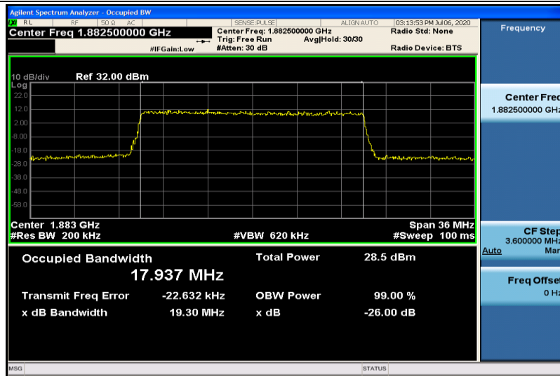
Band25-20MHz-16QAM-26365-100RB#0-17.937
