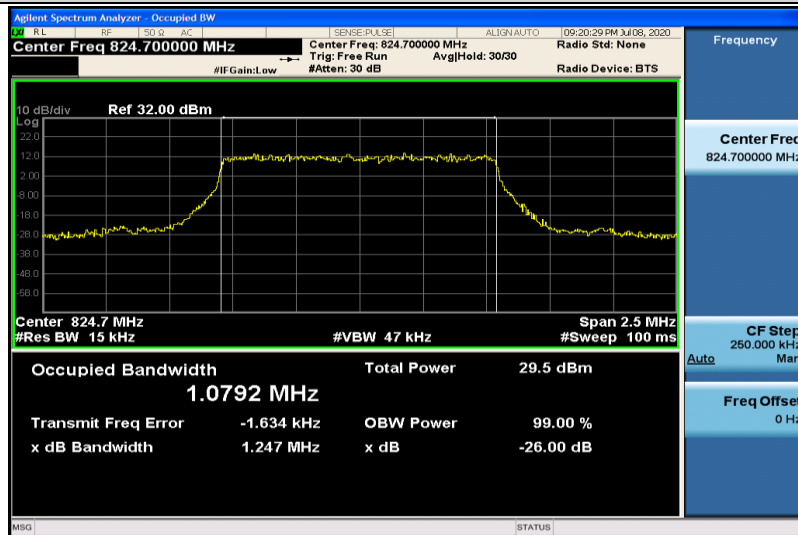
Band26-1.4MHz-QPSK-26797-6RB#0-1.0792
