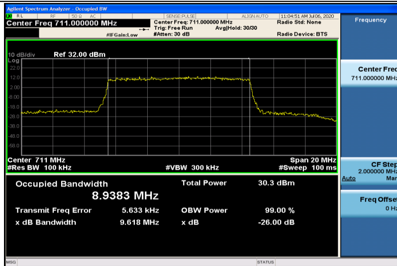
Band12-10MHz-16QAM-23130-50RB#0-8.9383
