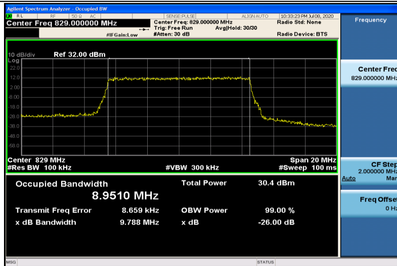
Band26-10MHz-QPSK-26840-50RB#0-8.9510
