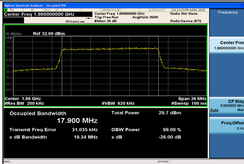
Band25-20MHz-QPSK-26140-100RB#0-17.900
