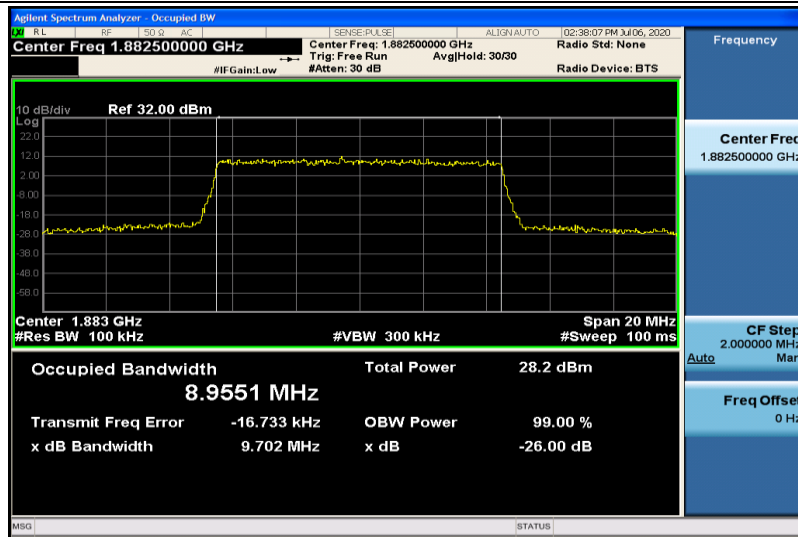
Band25-10MHz-16QAM-26365-50RB#0-8.9551
