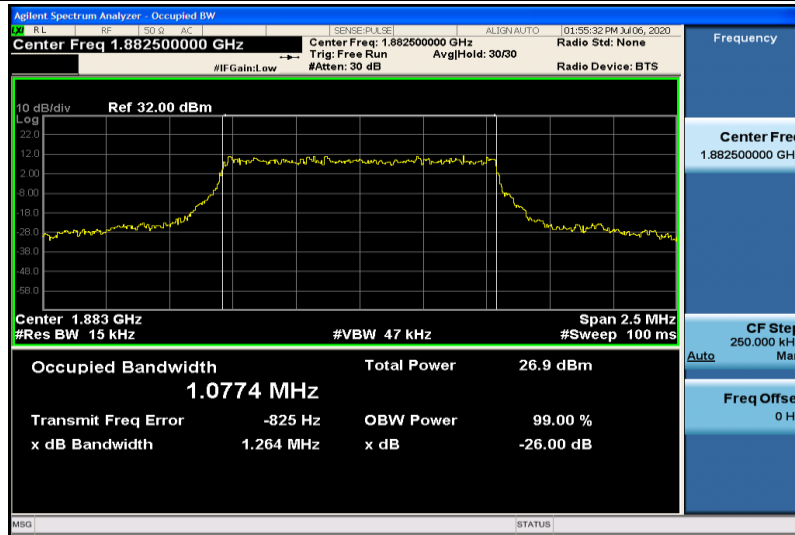
Band25-1.4MHz-16QAM-26365-6RB#0-1.0774
