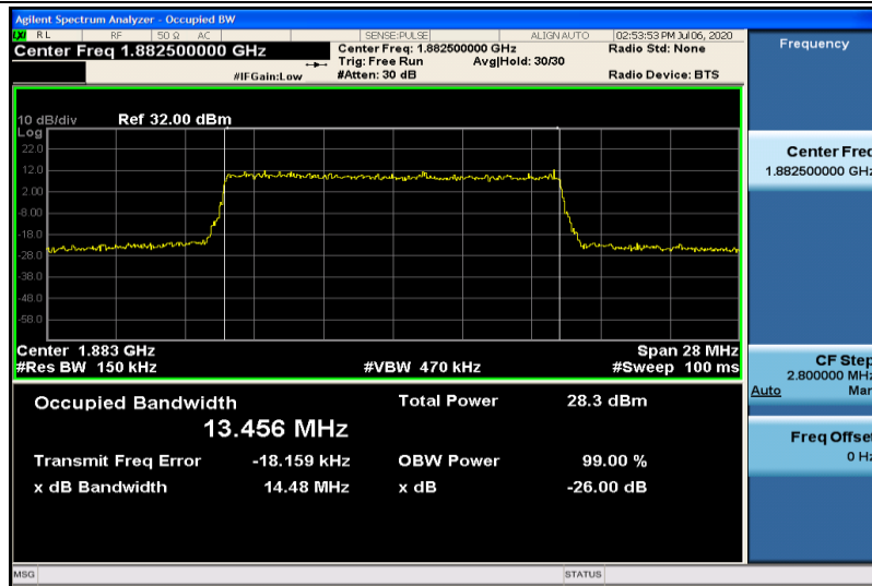
Band25-15MHz-16QAM-26365-75RB#0-13.456
