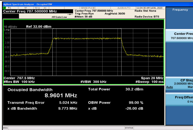
Band12-10MHz-16QAM-23095-50RB#0-8.9601
