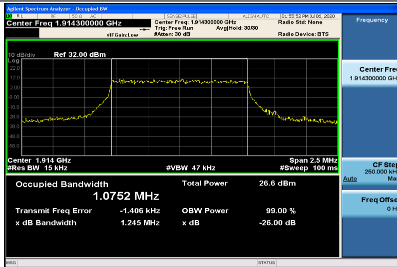
Band25-1.4MHz-16QAM-26683-6RB#0-1.0752
