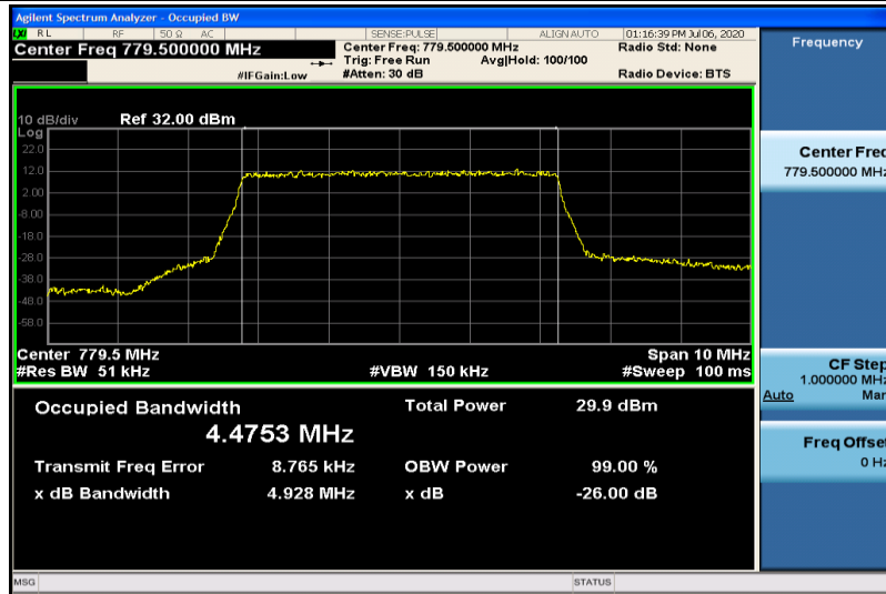
Band13-5MHz-16QAM-23205-25RB#0-4.4753
