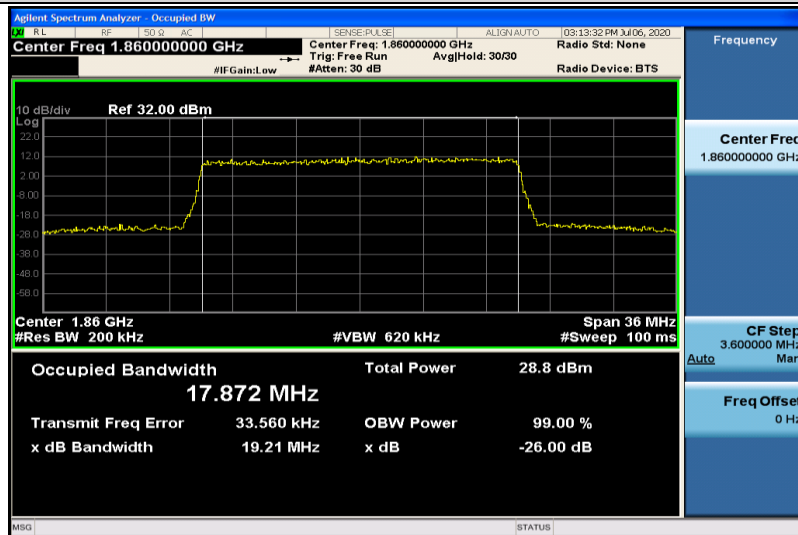
Band25-20MHz-16QAM-26140-100RB#0-17.872
