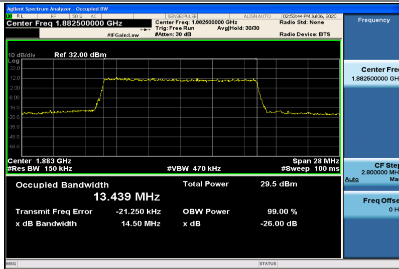
Band25-15MHz-QPSK-26365-75RB#0-13.439
