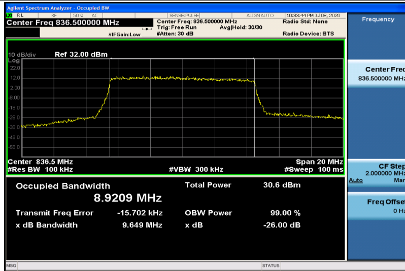
Band26-10MHz-QPSK-26915-50RB#0-8.9209
