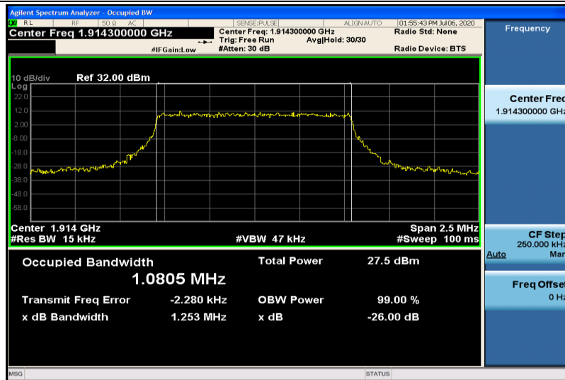
Band25-1.4MHz-QPSK-26683-6RB#0-1.0805
