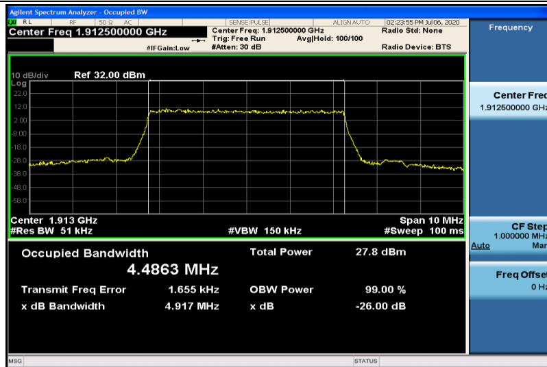
Band25-5MHz-16QAM-26665-25RB#0-4.4863
