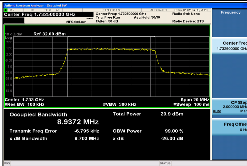
Band4-10MHz-QPSK-20175-50RB#0-8.9372
