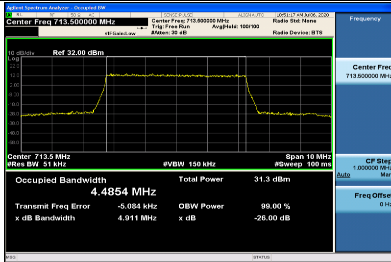
Band12-5MHz-QPSK-23155-25RB#0-4.4854
