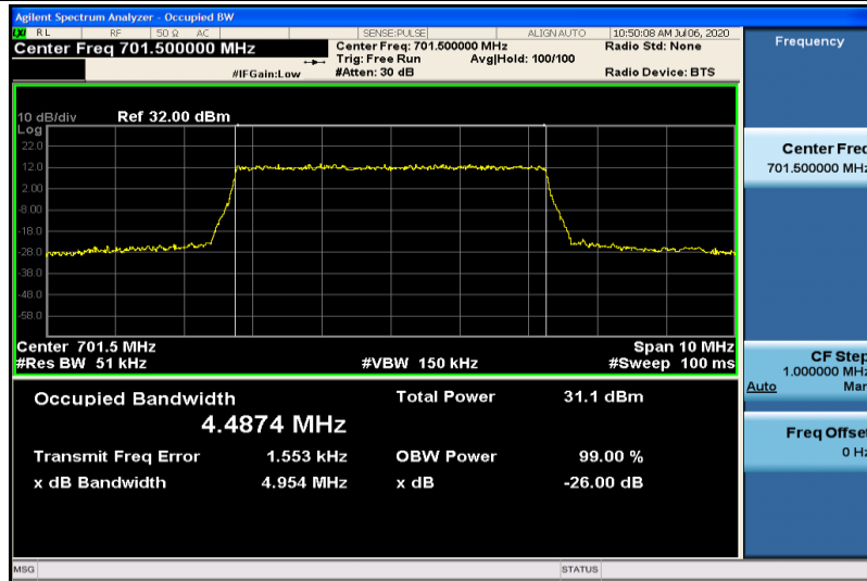
Band12-5MHz-QPSK-23035-25RB#0-4.4874
