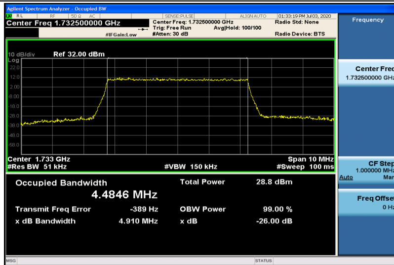
Band4-5MHz-16QAM-20175-25RB#0-4.4846
