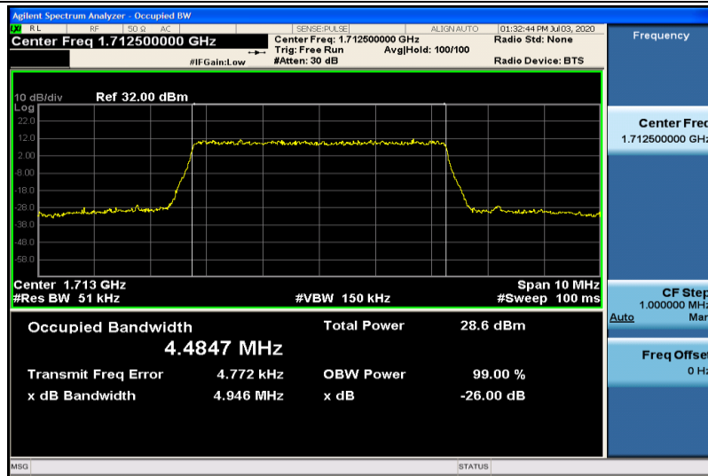
Band4-5MHz-16QAM-19975-25RB#0-4.4847
