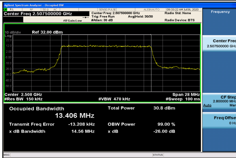
Band7-15MHz-QPSK-20825-75RB#0-13.406
