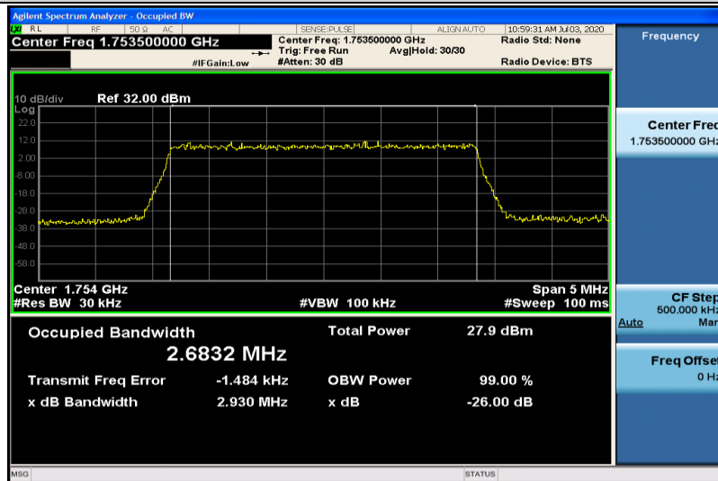
Band4-3MHz-16QAM-20385-15RB#0-2.6832
