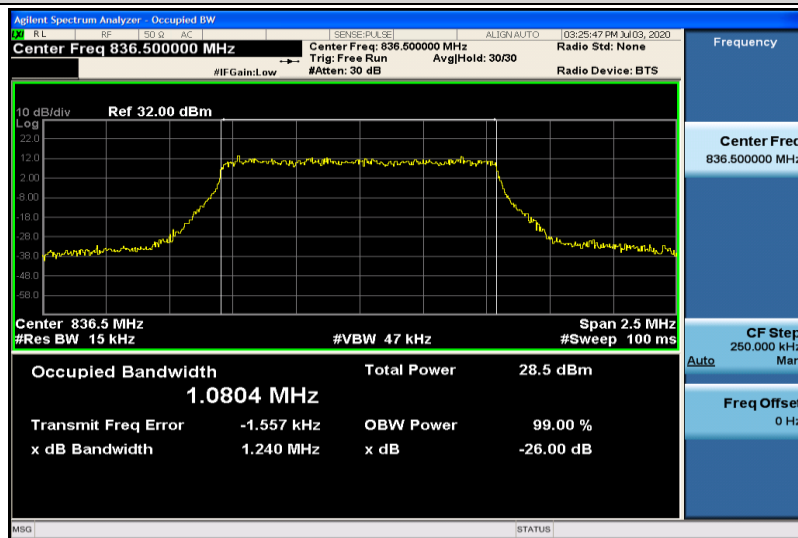
Band5-1.4MHz-16QAM-20525-6RB#0-1.0804
