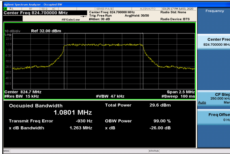
Band5-1.4MHz-QPSK-20407-6RB#0-1.0801
