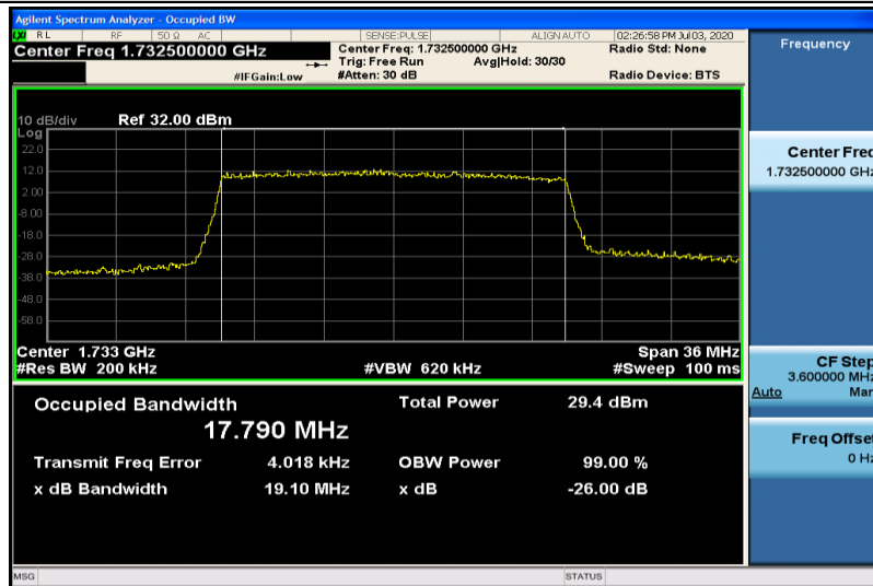
Band4-20MHz-QPSK-20175-100RB#0-17.790
