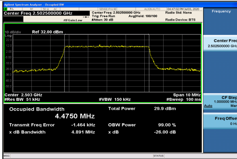
Band7-5MHz-16QAM-20775-25RB#0-4.4750
