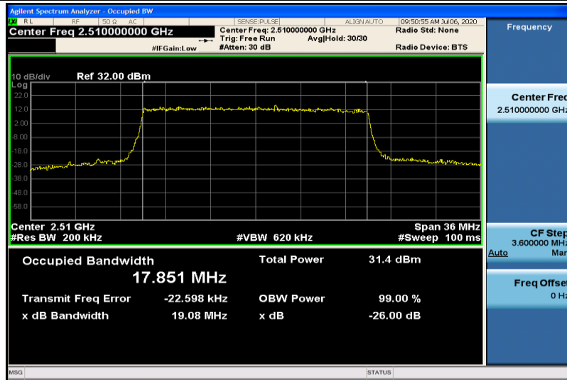
Band7-20MHz-QPSK-20850-100RB#0-17.851
