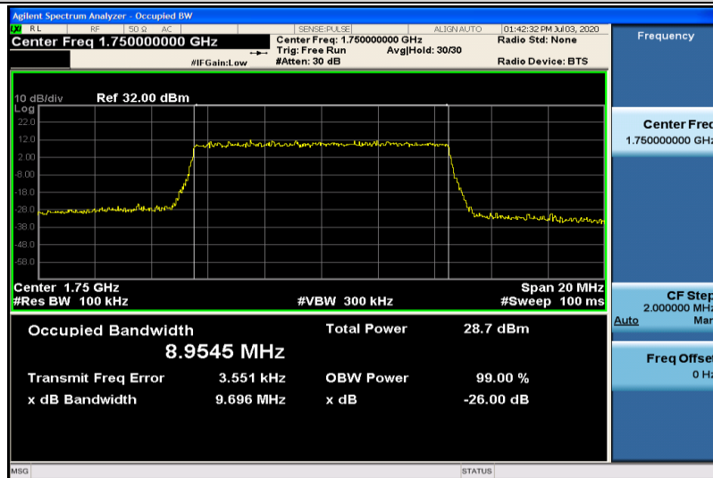
Band4-10MHz-16QAM-20350-50RB#0-8.9545
