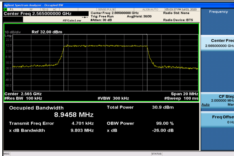
Band7-10MHz-QPSK-21400-50RB#0-8.9458
