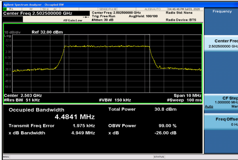
Band7-5MHz-QPSK-20775-25RB#0-4.4841
