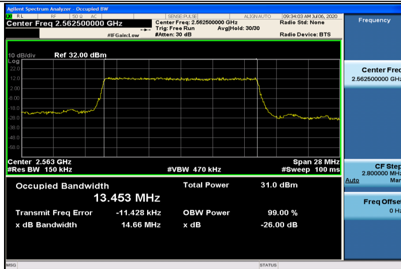
Band7-15MHz-QPSK-21375-75RB#0-13.453
