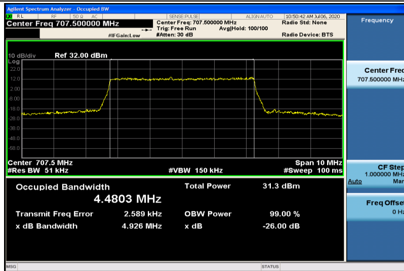
Band12-5MHz-QPSK-23095-25RB#0-4.4803
