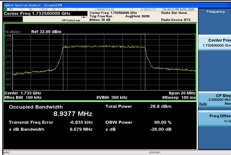
Band4-10MHz-16QAM-20175-50RB#0-8.9377
