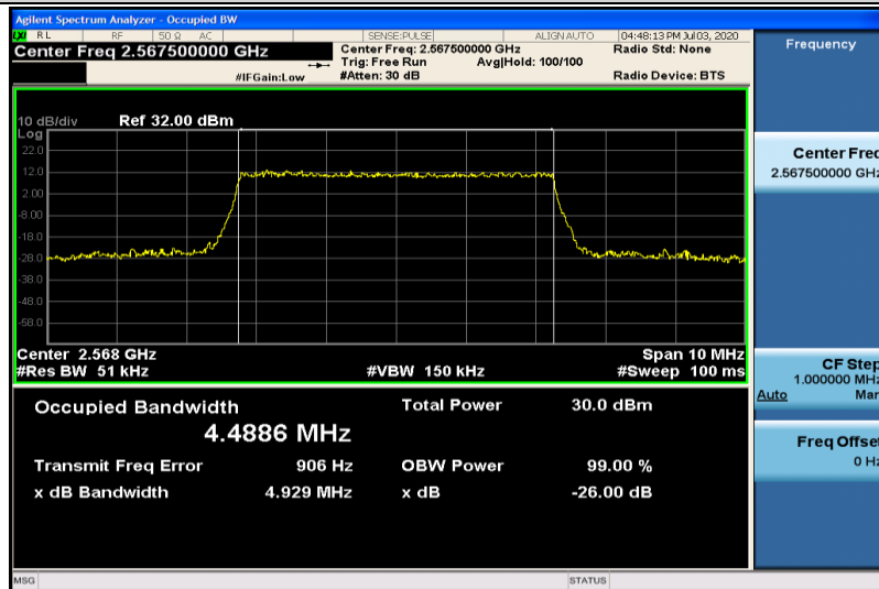
Band7-5MHz-16QAM-21425-25RB#0-4.4886
