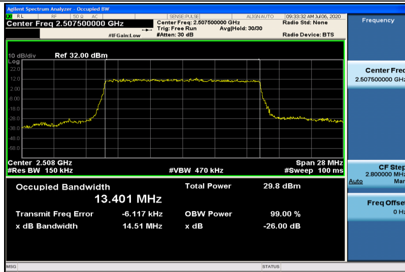
Band7-15MHz-16QAM-20825-75RB#0-13.401
