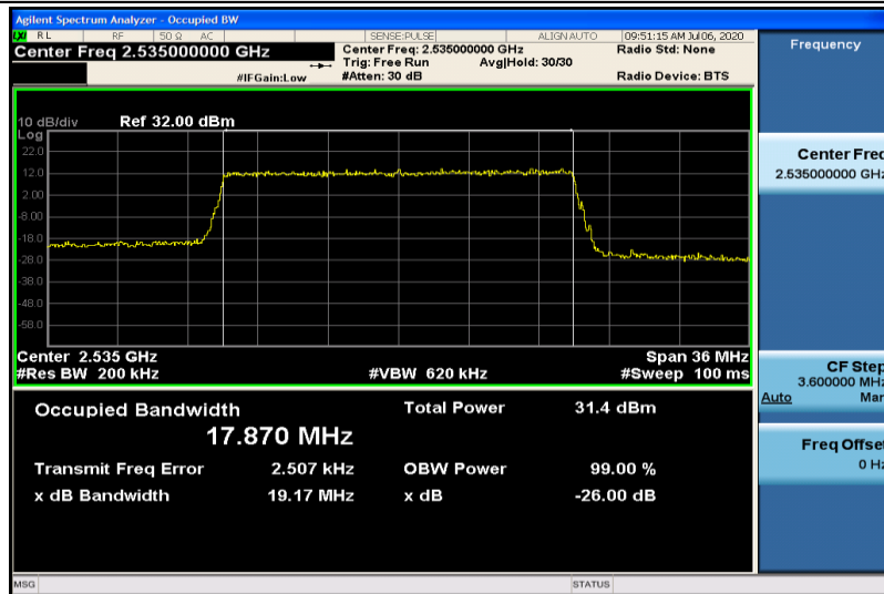
Band7-20MHz-QPSK-21100-100RB#0-17.870
