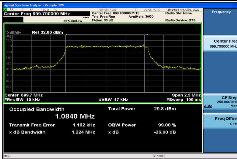
Band12-1.4MHz-QPSK-23017-6RB#0-1.0840
