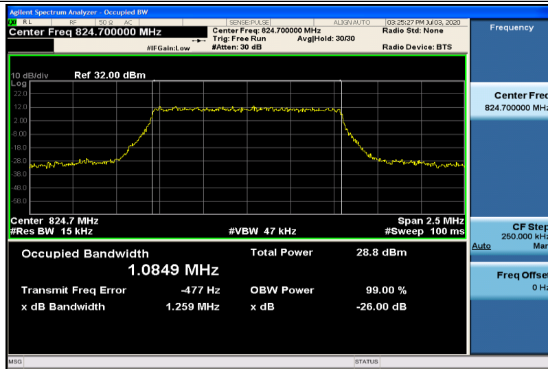
Band5-1.4MHz-16QAM-20407-6RB#0-1.0849
