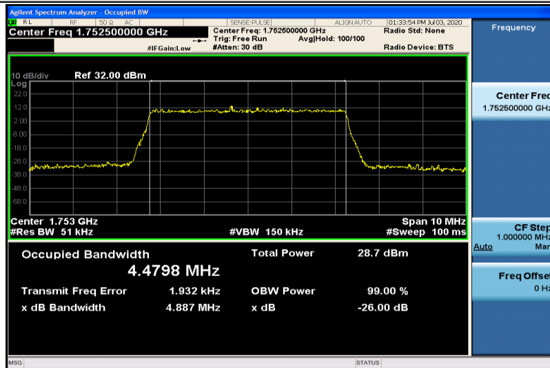
Band4-5MHz-16QAM-20375-25RB#0-4.4798
