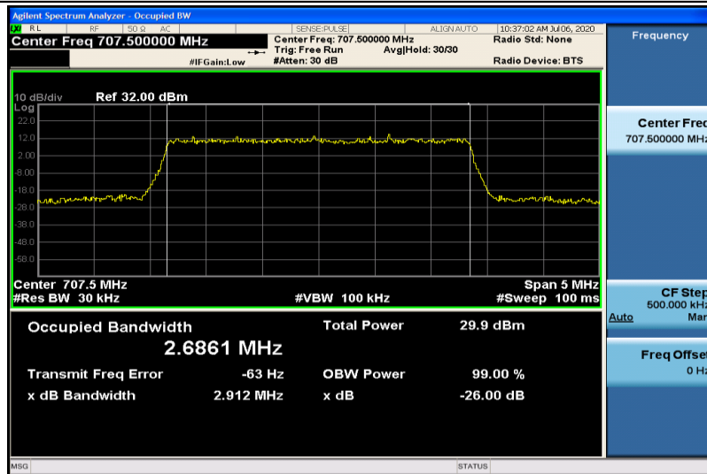
Band12-3MHz-16QAM-23095-15RB#0-2.6861
