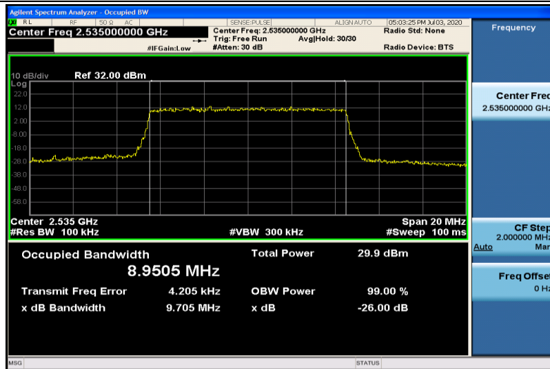
Band7-10MHz-16QAM-21100-50RB#0-8.9505
