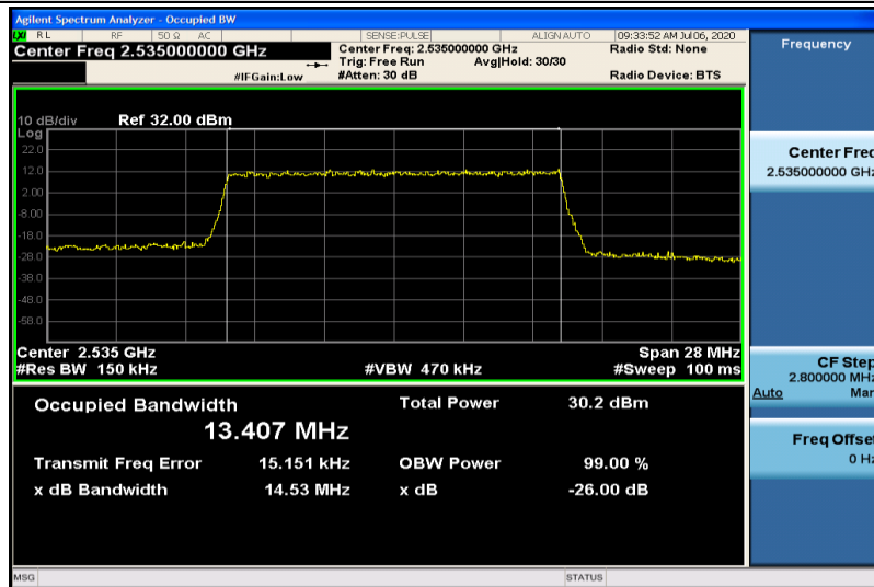
Band7-15MHz-16QAM-21100-75RB#0-13.407
