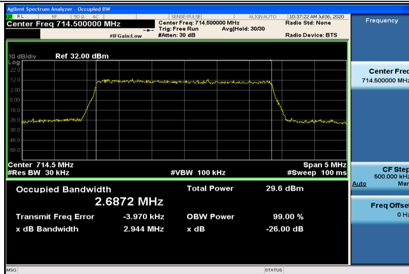
Band12-3MHz-16QAM-23165-15RB#0-2.6872
