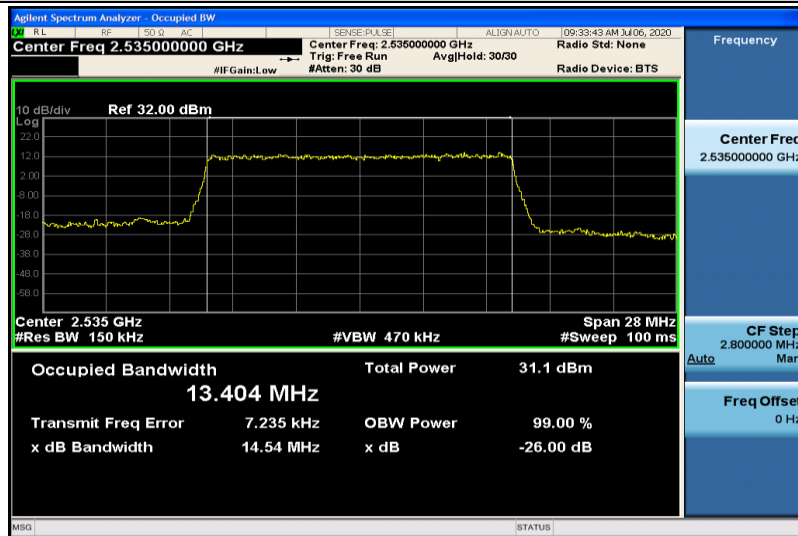
Band7-15MHz-QPSK-21100-75RB#0-13.404
