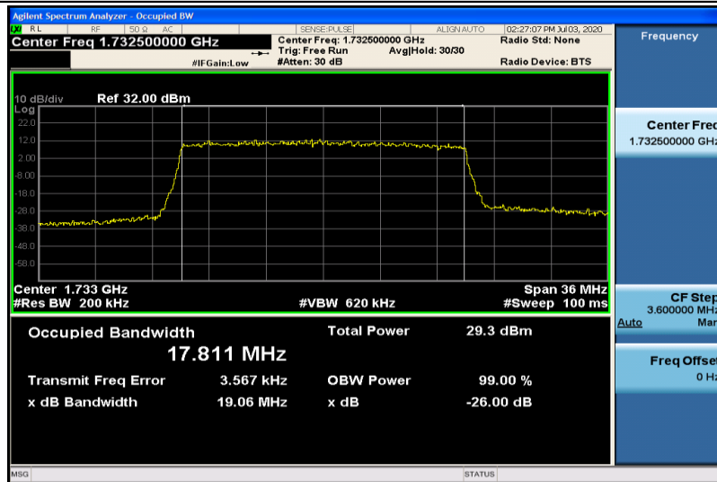
Band4-20MHz-16QAM-20175-100RB#0-17.811
