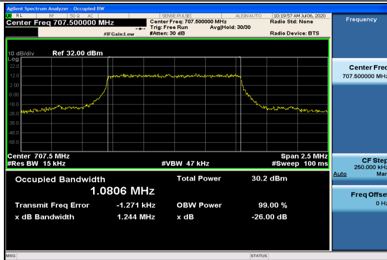
Band12-1.4MHz-QPSK-23095-6RB#0-1.0806
