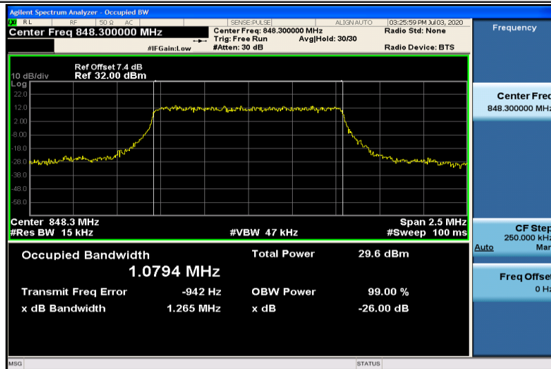
Band5-1.4MHz-QPSK-20643-6RB#0-1.0794
