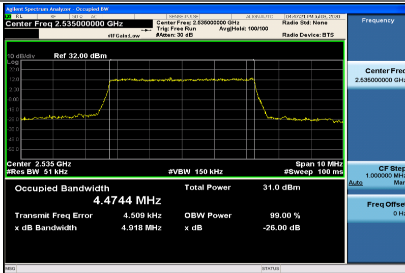
Band7-5MHz-QPSK-21100-25RB#0-4.4744
