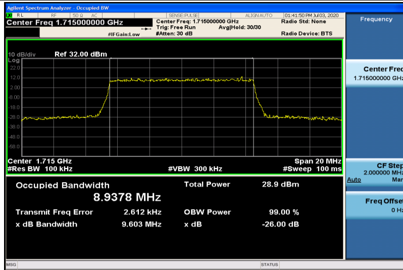
Band4-10MHz-16QAM-20000-50RB#0-8.9378
