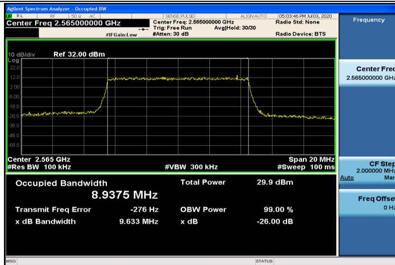
Band7-10MHz-16QAM-21400-50RB#0-8.9375
