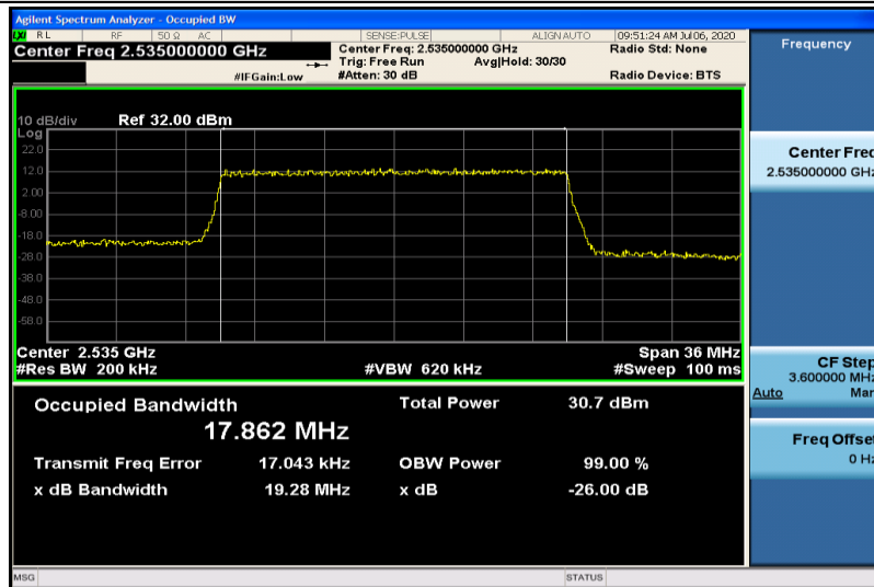
Band7-20MHz-16QAM-21100-100RB#0-17.862
