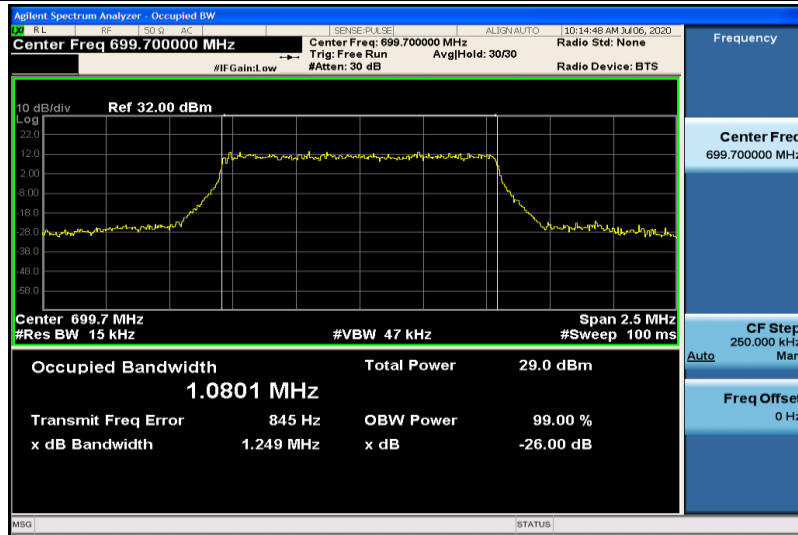
Band12-1.4MHz-16QAM-23017-6RB#0-1.0801
