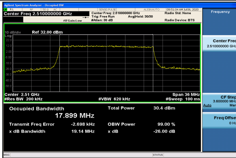
Band7-20MHz-16QAM-20850-100RB#0-17.899
