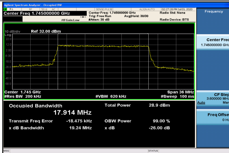
Band4-20MHz-16QAM-20300-100RB#0-17.914
