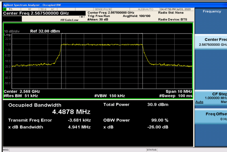
Band7-5MHz-QPSK-21425-25RB#0-4.4878
