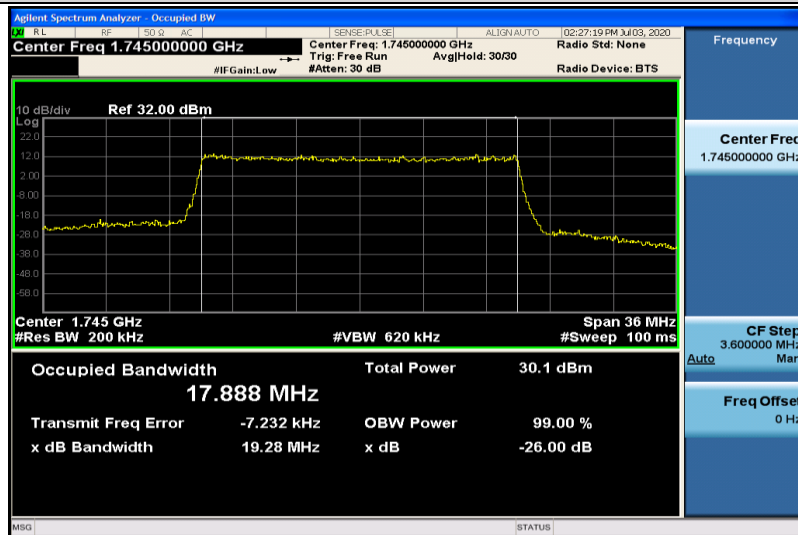
Band4-20MHz-QPSK-20300-100RB#0-17.888
