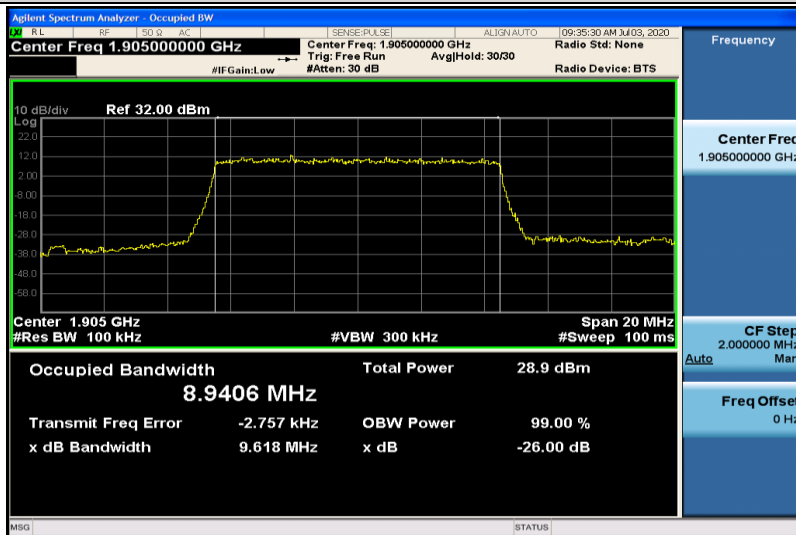
Band2-10MHz-QPSK-19150-50RB#0-8.9406
