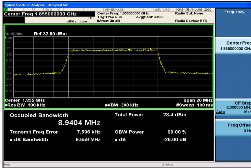
Band2-10MHz-16QAM-18650-50RB#0-8.9404
