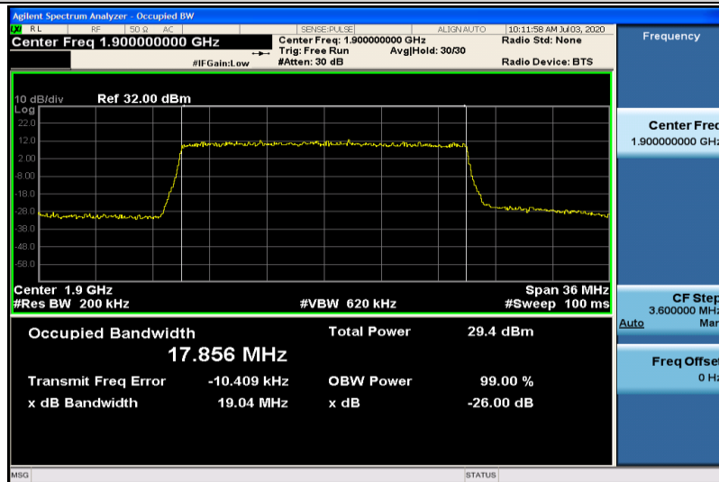
Band2-20MHz-QPSK-19100-100RB#0-17.856
