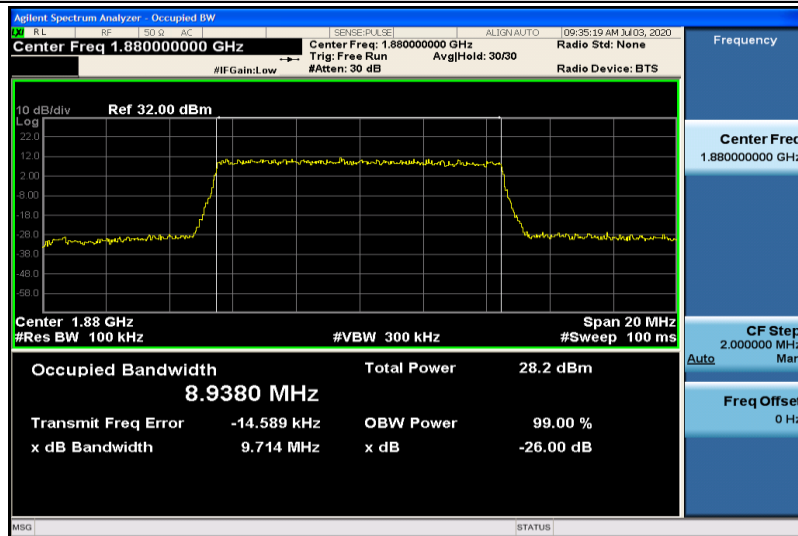
Band2-10MHz-16QAM-18900-50RB#0-8.9380
