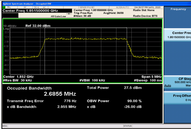
Band2-3MHz-16QAM-18615-15RB#0-2.6855
