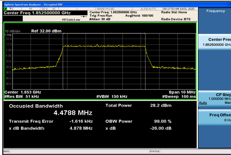
Band2-5MHz-16QAM-18525-25RB#0-4.4788
