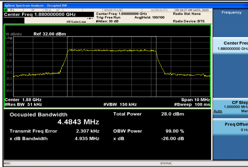
Band2-5MHz-16QAM-18900-25RB#0-4.4843
