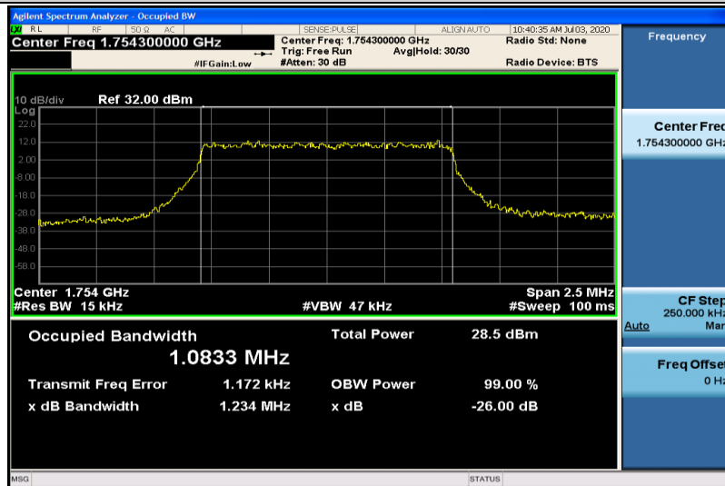
Band4-1.4MHz-QPSK-20393-6RB#0-1.0833
