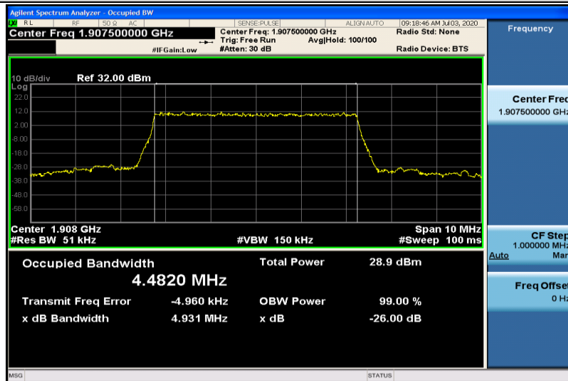
Band2-5MHz-QPSK-19175-25RB#0-4.4820
