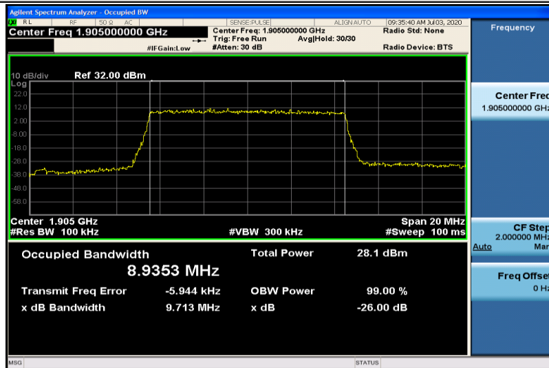
Band2-10MHz-16QAM-19150-50RB#0-8.9353
