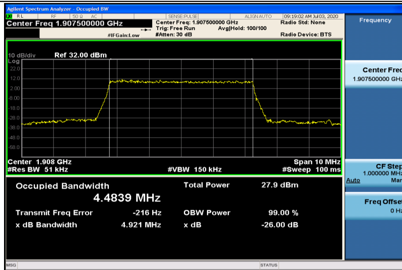
Band2-5MHz-16QAM-19175-25RB#0-4.4839
