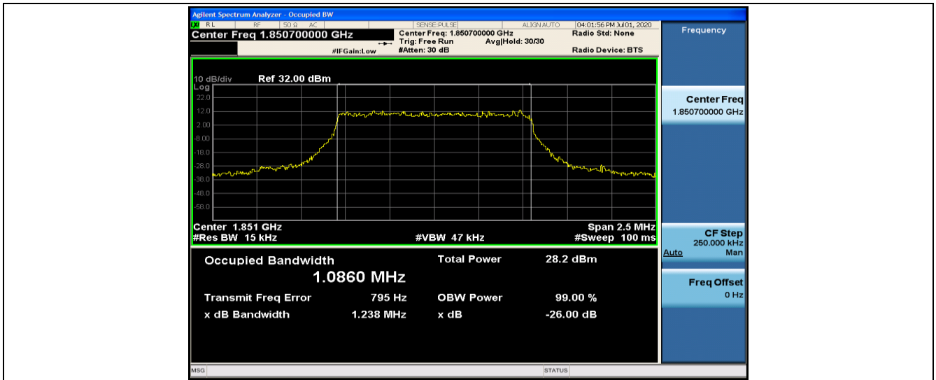
Band2-1.4MHz-QPSK-18607-6RB#0-1.0860
