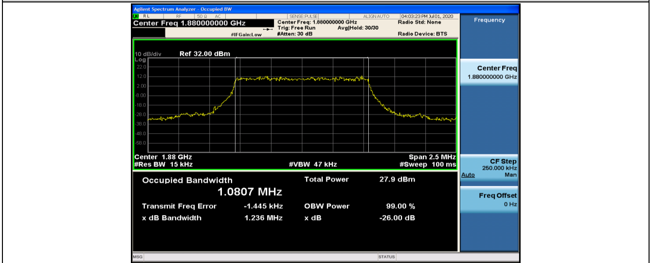
Band2-1.4MHz-QPSK-18900-6RB#0-1.0807
