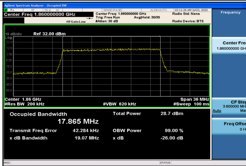
Band2-20MHz-16QAM-18700-100RB#0-17.865
