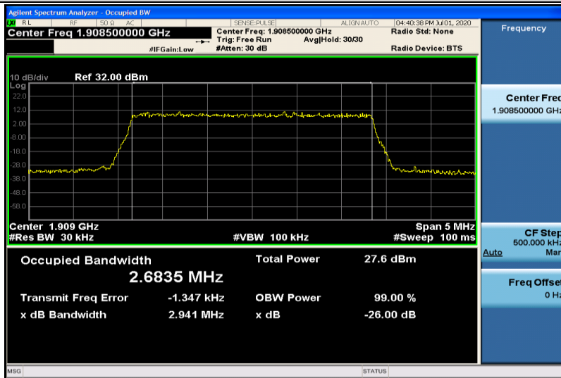
Band2-3MHz-16QAM-19185-15RB#0-2.6835
