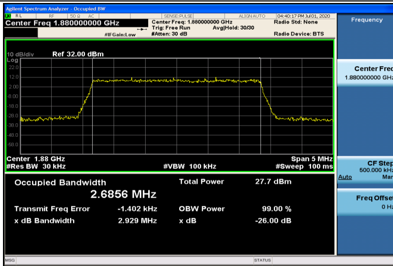
Band2-3MHz-16QAM-18900-15RB#0-2.6856
