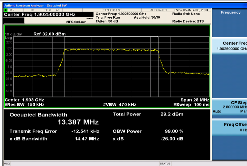
Band2-15MHz-QPSK-19125-75RB#0-13.387
