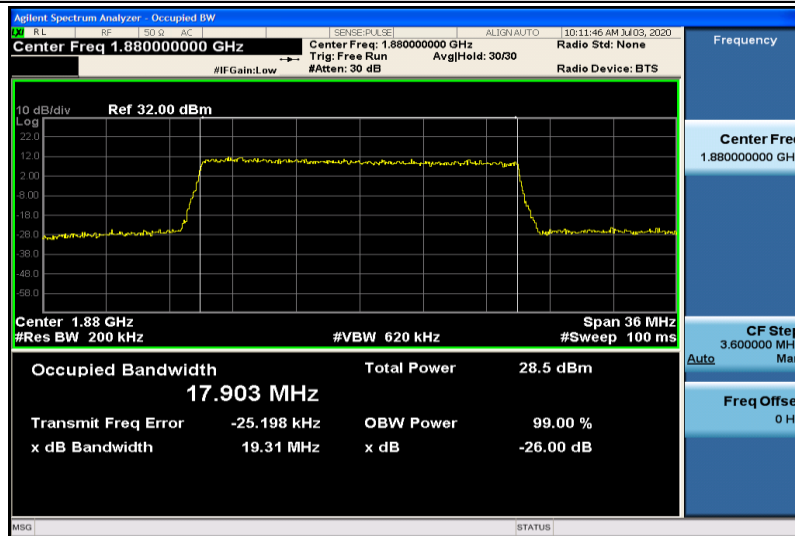
Band2-20MHz-16QAM-18900-100RB#0-17.903
