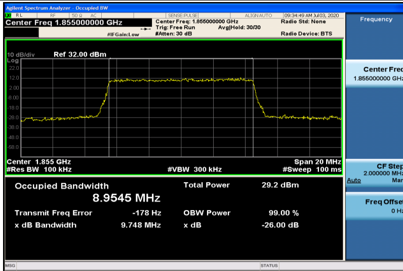
Band2-10MHz-QPSK-18650-50RB#0-8.9545
