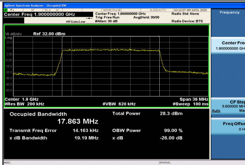
Band2-20MHz-16QAM-19100-100RB#0-17.863
