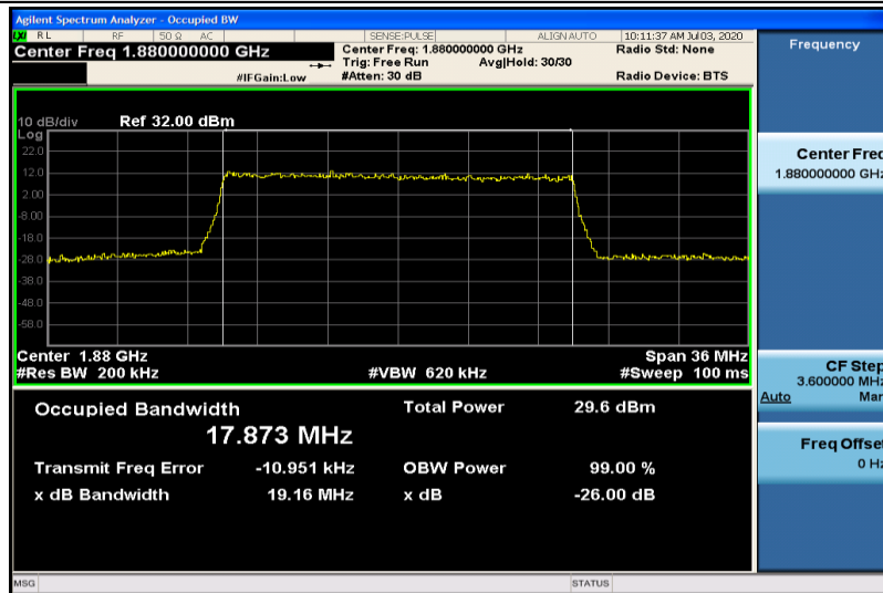
Band2-20MHz-QPSK-18900-100RB#0-17.873
