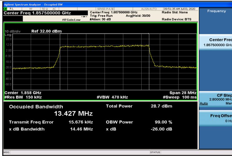
Band2-15MHz-16QAM-18675-75RB#0-13.427
