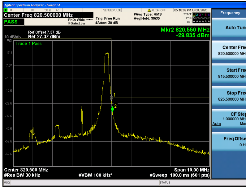
Band26-3MHz-16QAM-26740-1RB#14
