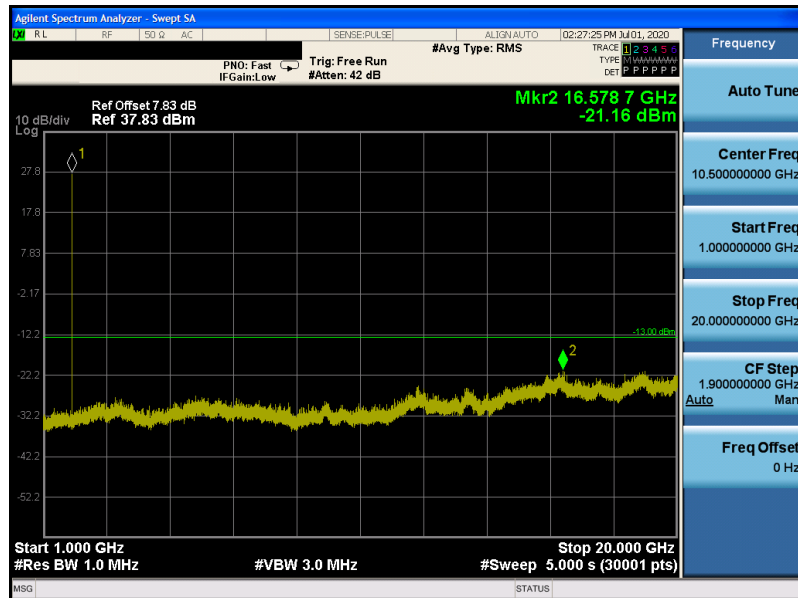
EGPRS1900-512-1000~20000
