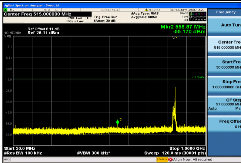
Band5-10MHz-16QAM-20600-1RB#0-30~1000MHz
