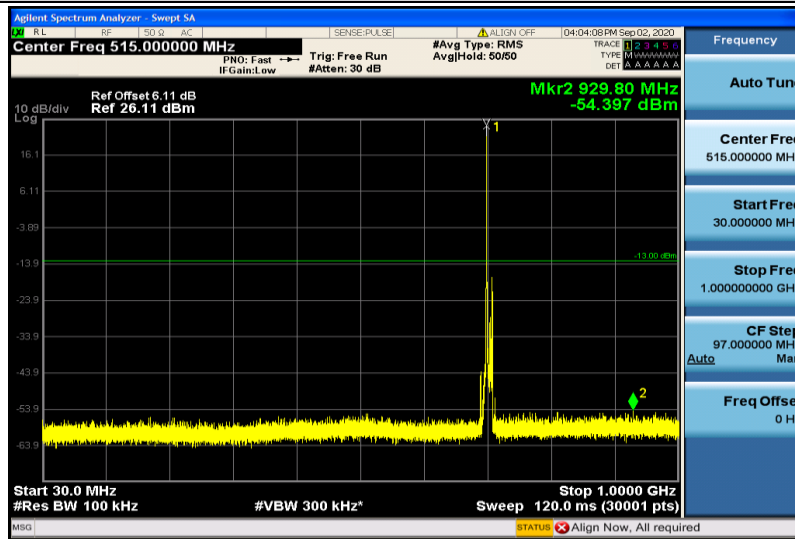
Band12-10MHz-QPSK-23130-1RB#0-30~1000MHz
