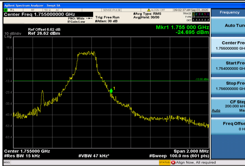
Band4-1.4MHz-16QAM-20393-1RB#5
