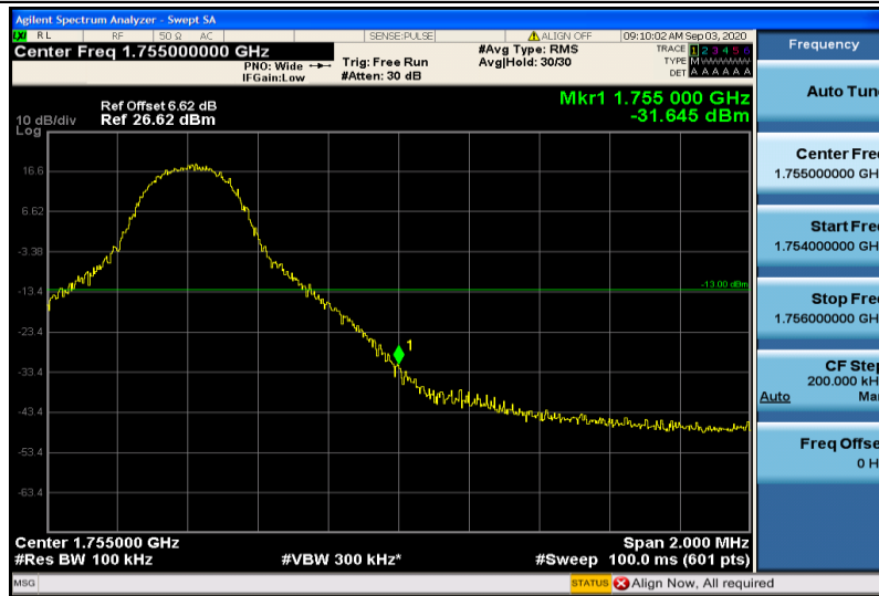
Band4-10MHz-16QAM-20350-1RB#49
