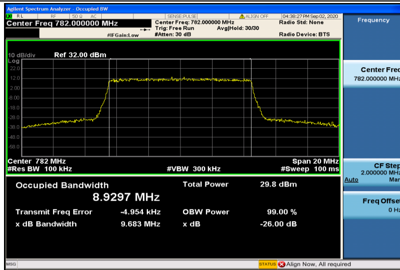
Band13-10MHz-16QAM-23230-50RB#0-8.9297
