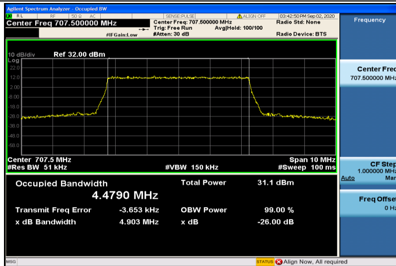
Band12-5MHz-QPSK-23095-25RB#0-4.4790
