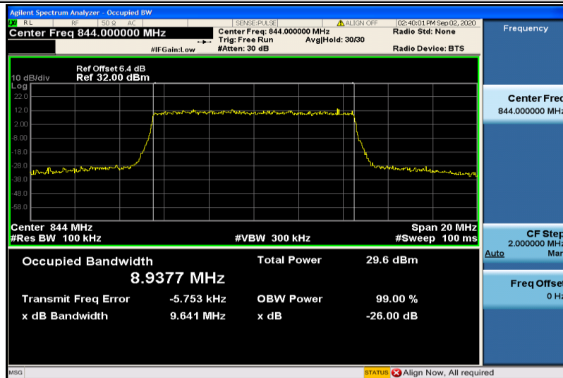
Band5-10MHz-16QAM-20600-50RB#0-8.9377
