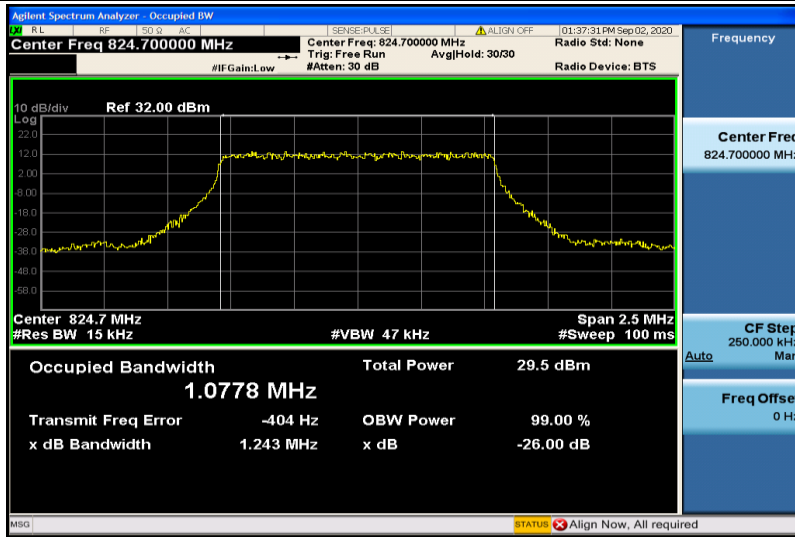
Band5-1.4MHz-QPSK-20407-6RB#0-1.0778
