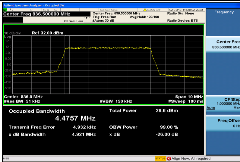
Band5-5MHz-16QAM-20525-25RB#0-4.4757
