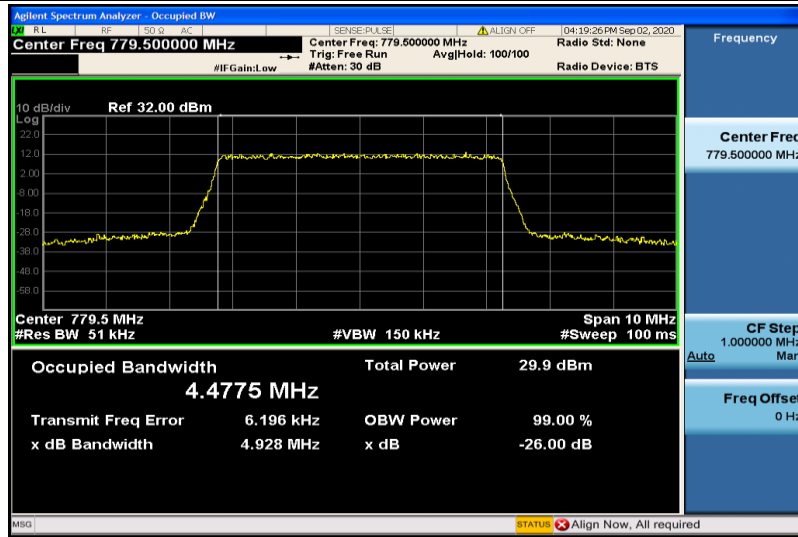
Band13-5MHz-16QAM-23205-25RB#0-4.4775
