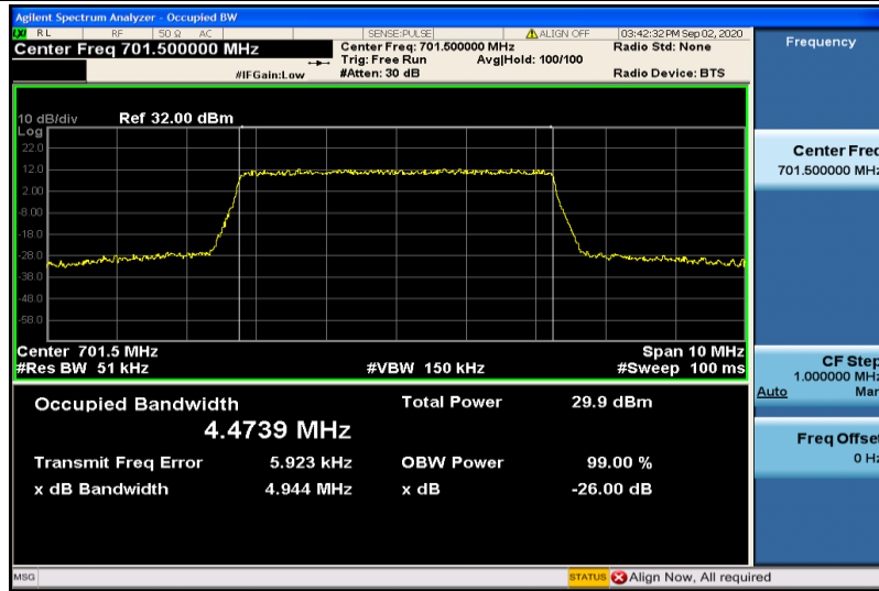
Band12-5MHz-16QAM-23035-25RB#0-4.4739
