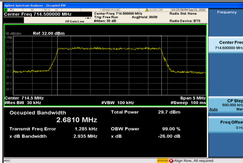
Band12-3MHz-16QAM-23165-15RB#0-2.6810
