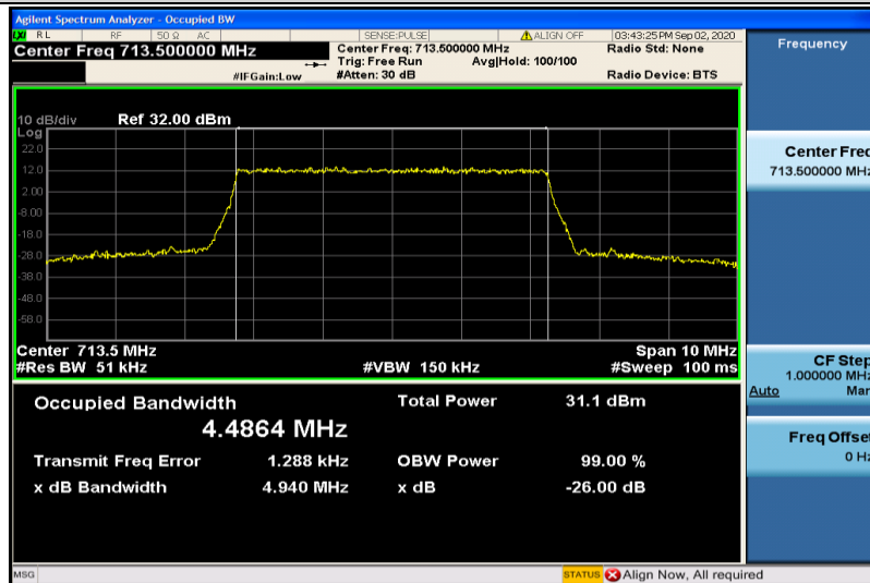
Band12-5MHz-QPSK-23155-25RB#0-4.4864
