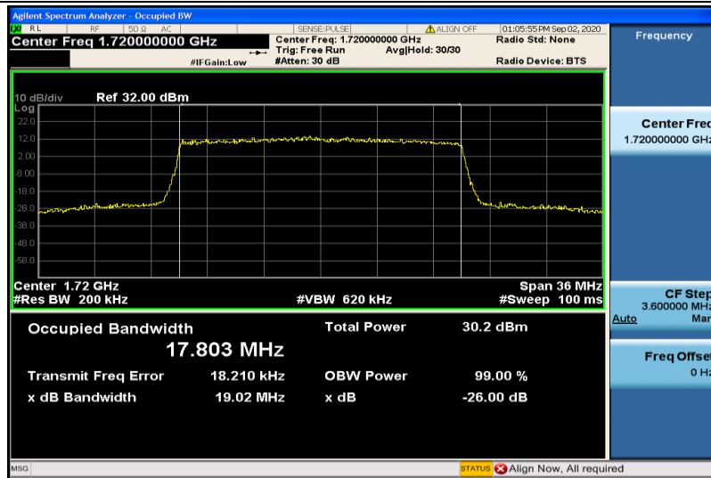
Band4-20MHz-16QAM-20050-100RB#0-17.803
