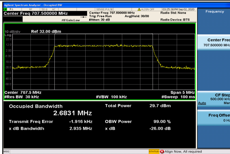
Band12-3MHz-16QAM-23095-15RB#0-2.6831
