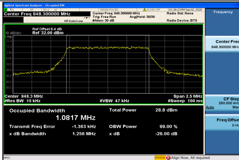
Band5-1.4MHz-16QAM-20643-6RB#0-1.0817
