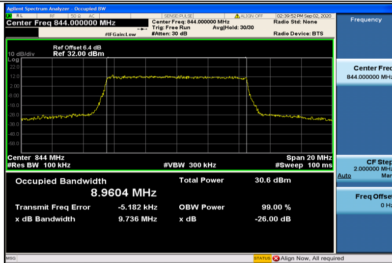
Band5-10MHz-QPSK-20600-50RB#0-8.9604
