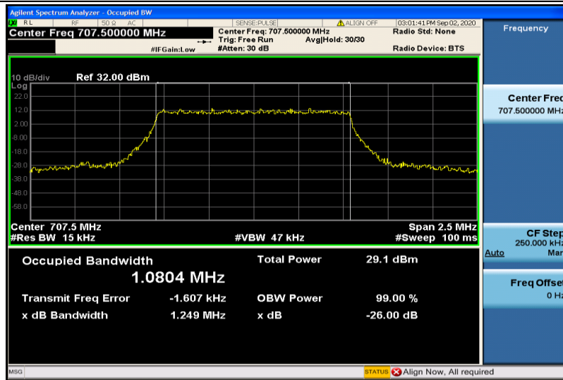
Band12-1.4MHz-16QAM-23095-6RB#0-1.0804
