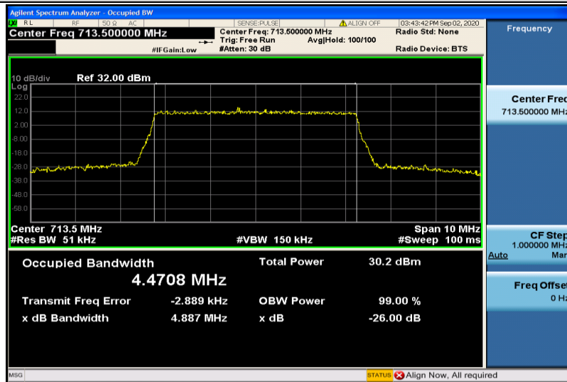
Band12-5MHz-16QAM-23155-25RB#0-4.4708
