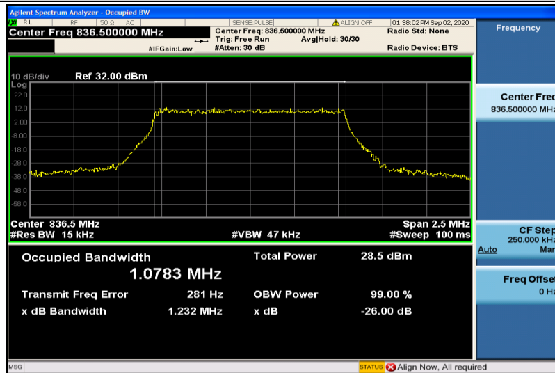
Band5-1.4MHz-16QAM-20525-6RB#0-1.0783
