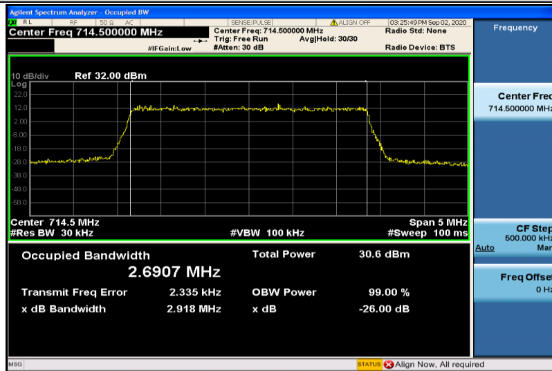
Band12-3MHz-QPSK-23165-15RB#0-2.6907
