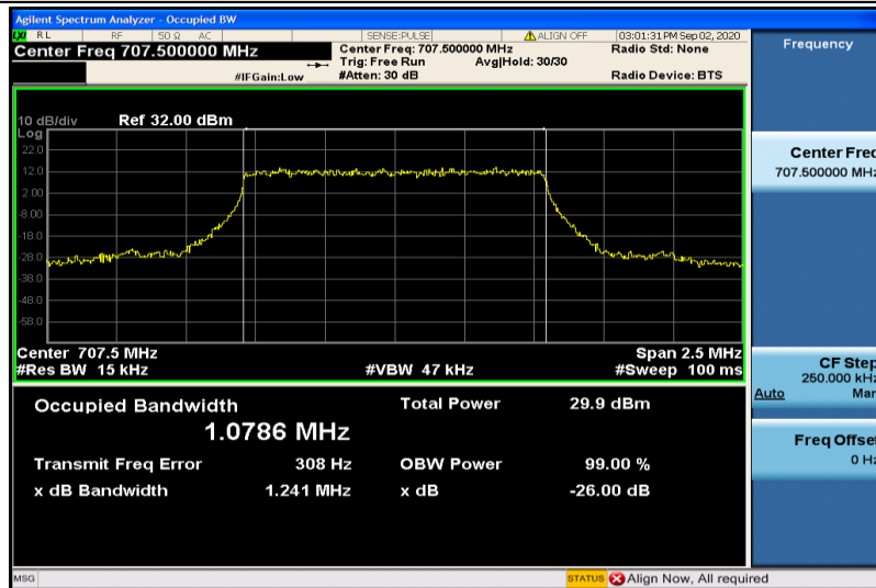
Band12-1.4MHz-QPSK-23095-6RB#0-1.0786
