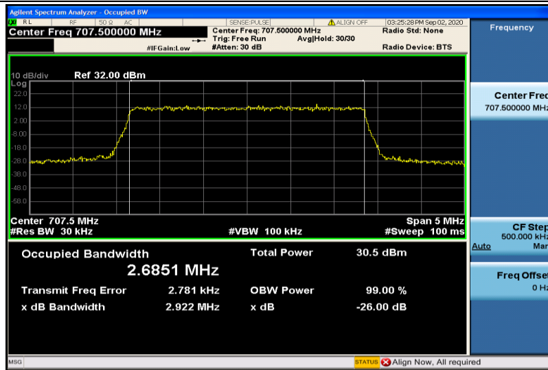
Band12-3MHz-QPSK-23095-15RB#0-2.6851
