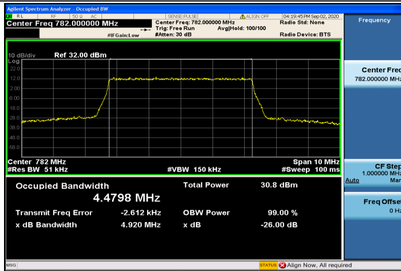
Band13-5MHz-QPSK-23230-25RB#0-4.4798
