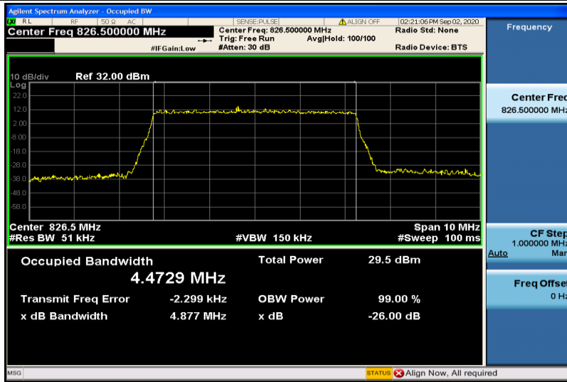
Band5-5MHz-16QAM-20425-25RB#0-4.4729
