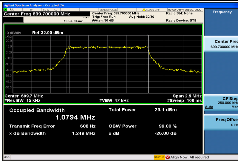
Band12-1.4MHz-16QAM-23017-6RB#0-1.0794
