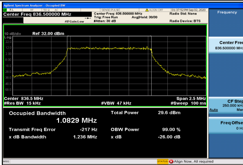
Band5-1.4MHz-QPSK-20525-6RB#0-1.0829
