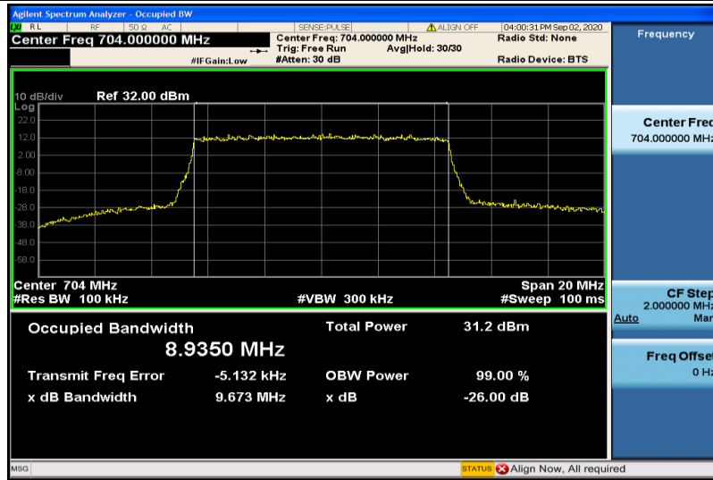
Band12-10MHz-QPSK-23060-50RB#0-8.9350
