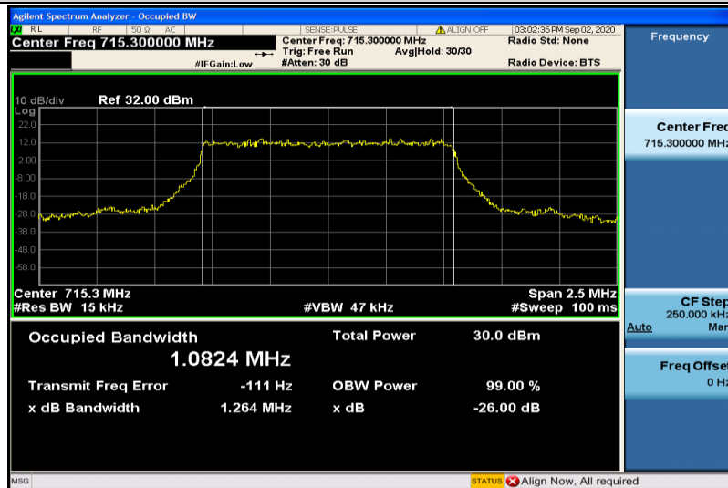
Band12-1.4MHz-QPSK-23173-6RB#0-1.0824
