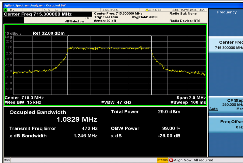
Band12-1.4MHz-16QAM-23173-6RB#0-1.0829
