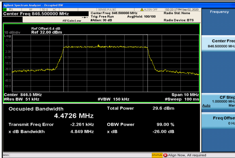
Band5-5MHz-16QAM-20625-25RB#0-4.4726
