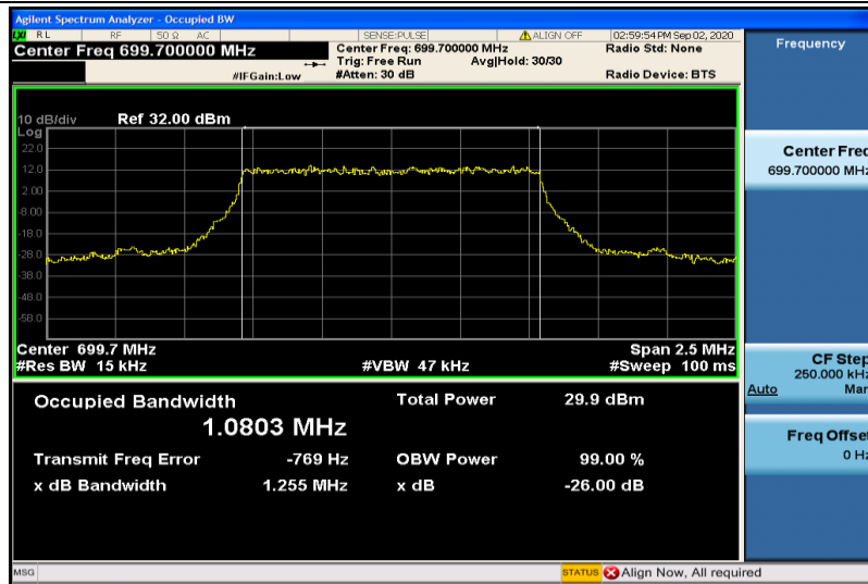
Band12-1.4MHz-QPSK-23017-6RB#0-1.0803
