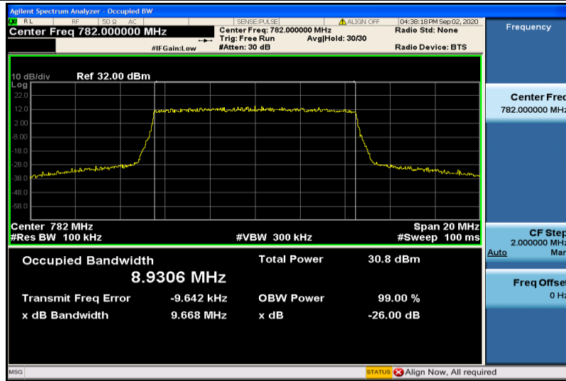
Band13-10MHz-QPSK-23230-50RB#0-8.9306
