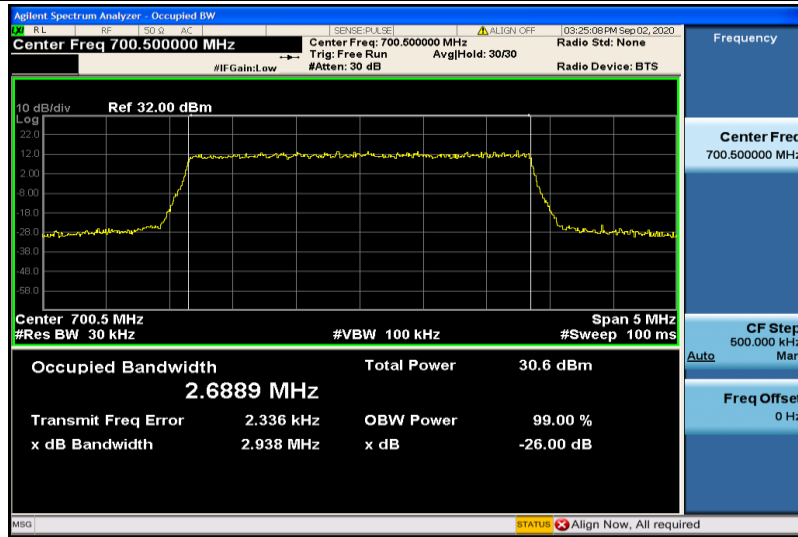
Band12-3MHz-QPSK-23025-15RB#0-2.6889
