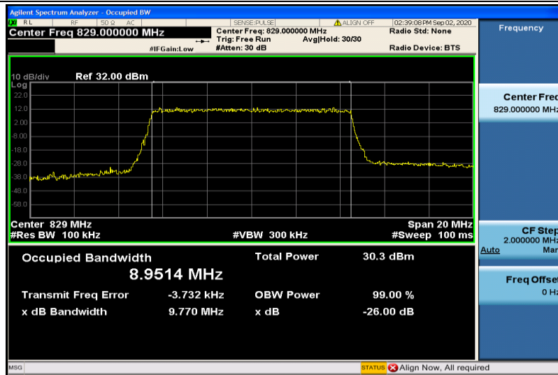
Band5-10MHz-QPSK-20450-50RB#0-8.9514
