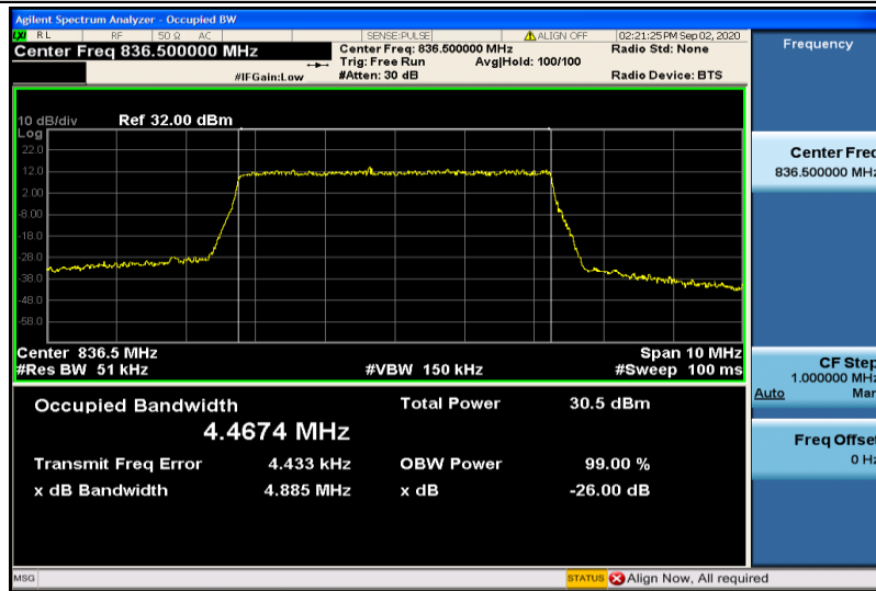
Band5-5MHz-QPSK-20525-25RB#0-4.4674
