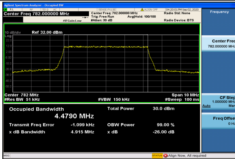
Band13-5MHz-16QAM-23230-25RB#0-4.4790
