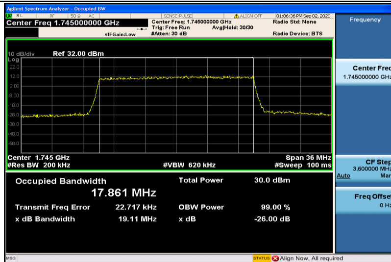
Band4-20MHz-16QAM-20300-100RB#0-17.861
