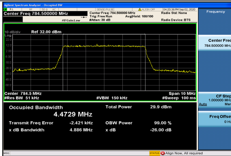
Band13-5MHz-16QAM-23255-25RB#0-4.4729
