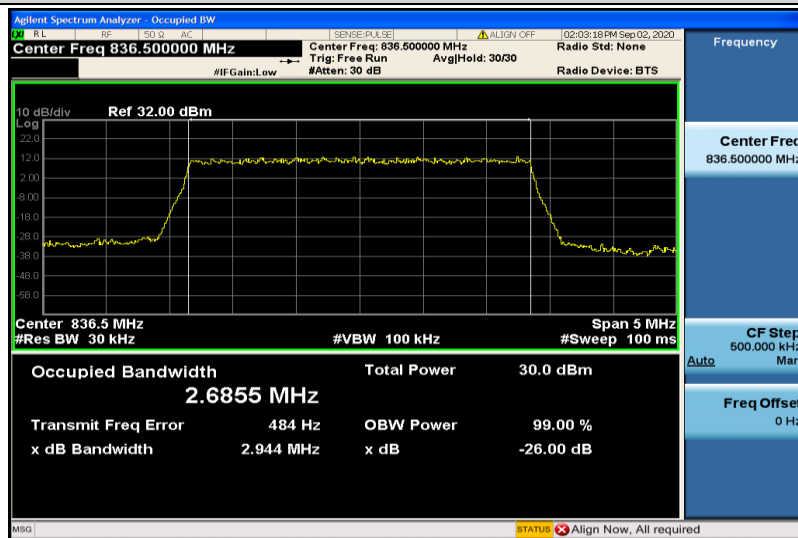
Band5-3MHz-QPSK-20525-15RB#0-2.6855
