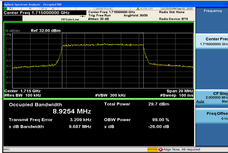
Band4-10MHz-16QAM-20000-50RB#0-8.9254
