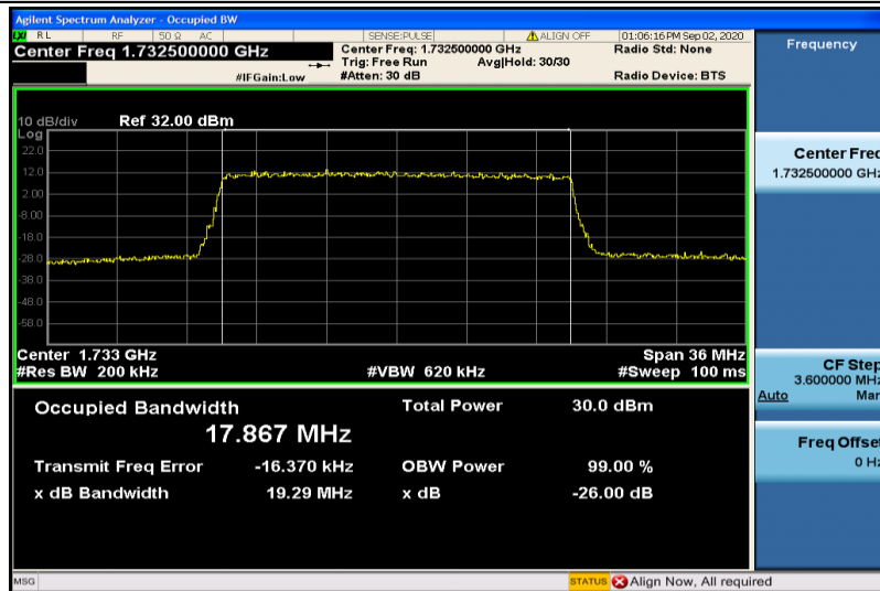
Band4-20MHz-16QAM-20175-100RB#0-17.867
