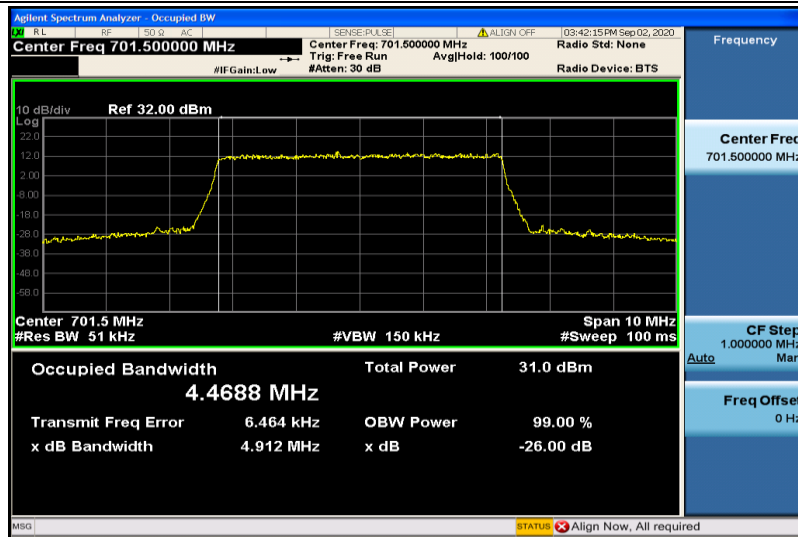
Band12-5MHz-QPSK-23035-25RB#0-4.4688
