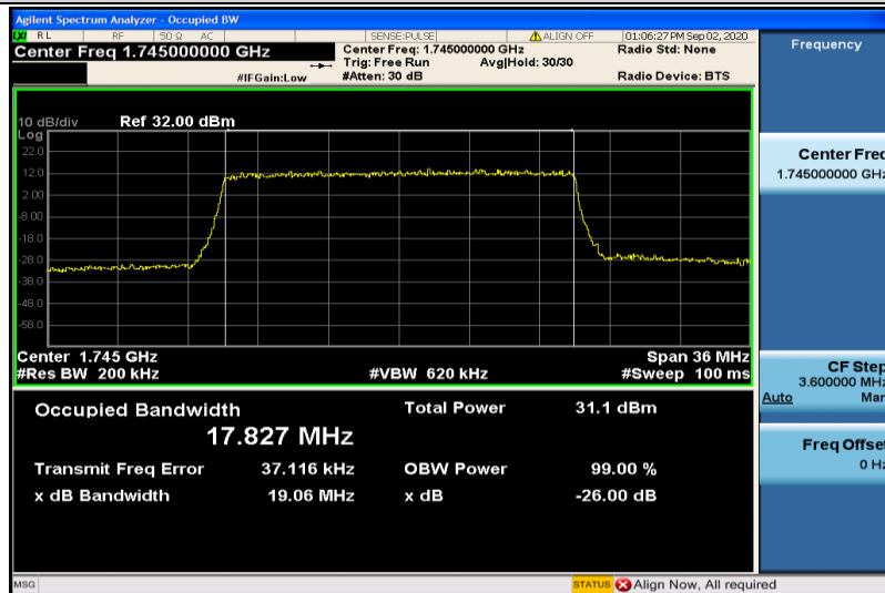
Band4-20MHz-QPSK-20300-100RB#0-17.827
