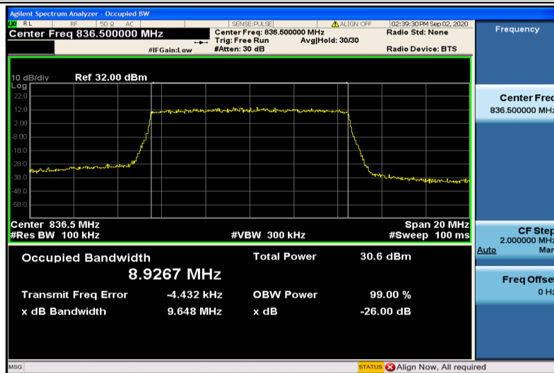
Band5-10MHz-QPSK-20525-50RB#0-8.9267
