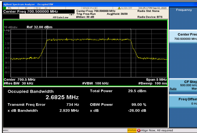
Band12-3MHz-16QAM-23025-15RB#0-2.6825
