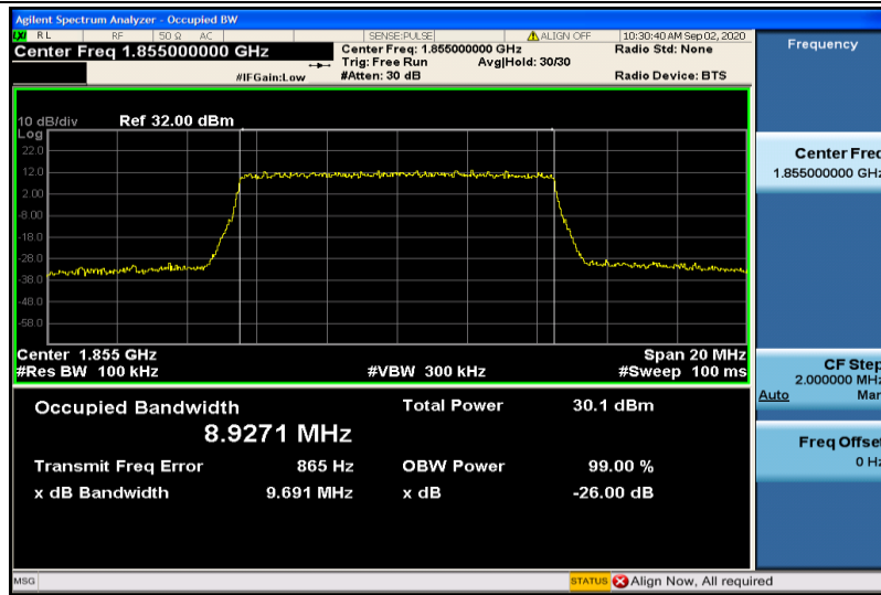
Band2-10MHz-16QAM-18650-50RB#0-8.9271
