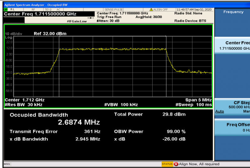
Band4-3MHz-QPSK-19965-15RB#0-2.6874
