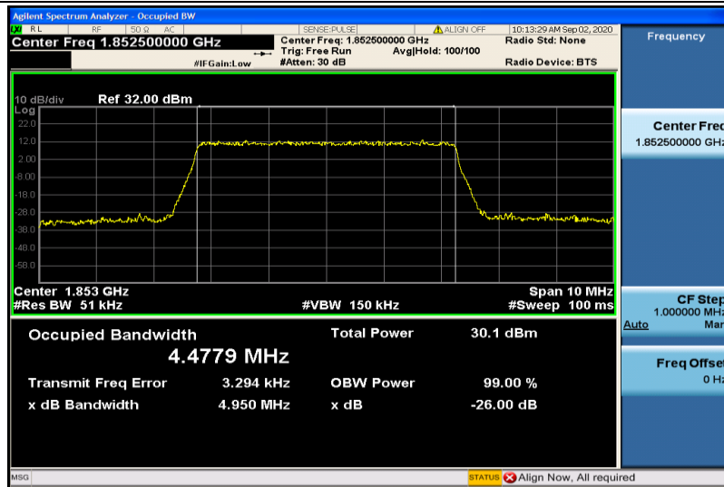
Band2-5MHz-16QAM-18625-25RB#0-4.4779
