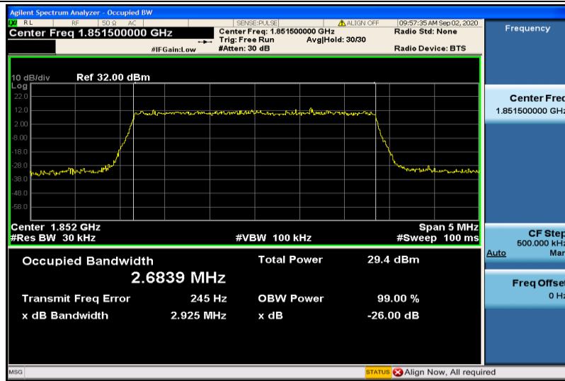
Band2-3MHz-16QAM-18615-15RB#0-2.6839
