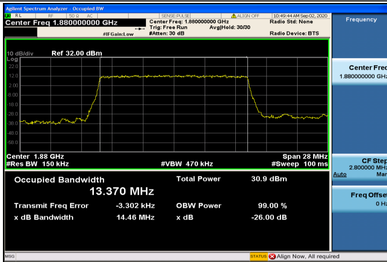
Band2-15MHz-QPSK-18900-75RB#0-13.370
