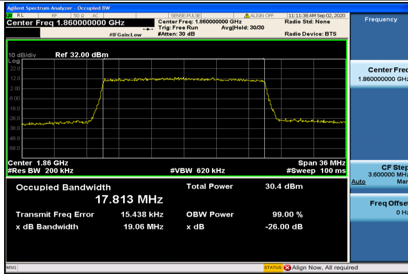
Band2-20MHz-16QAM-18700-100RB#0-17.813
