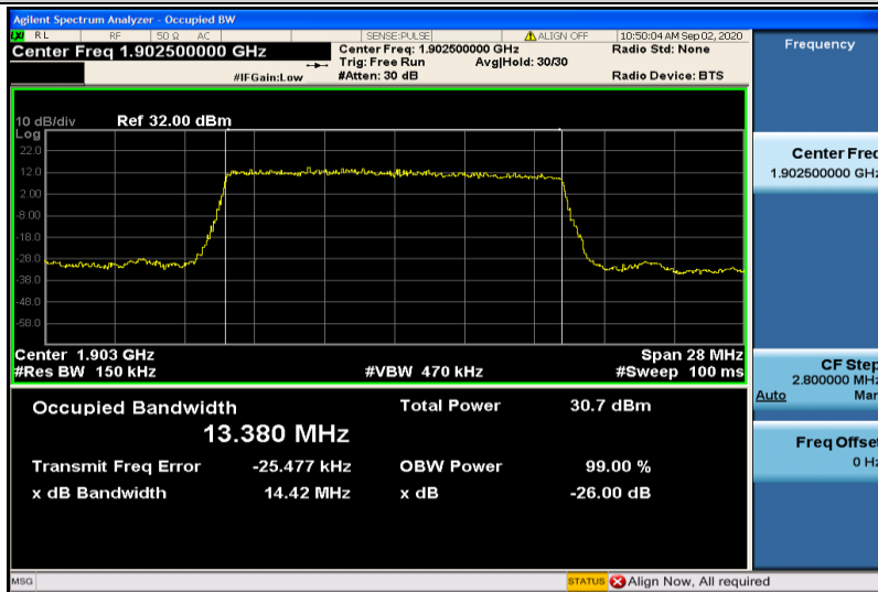
Band2-15MHz-QPSK-19125-75RB#0-13.380
