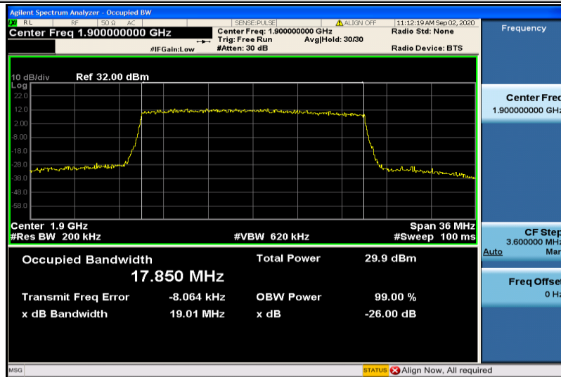
Band2-20MHz-16QAM-19100-100RB#0-17.850
