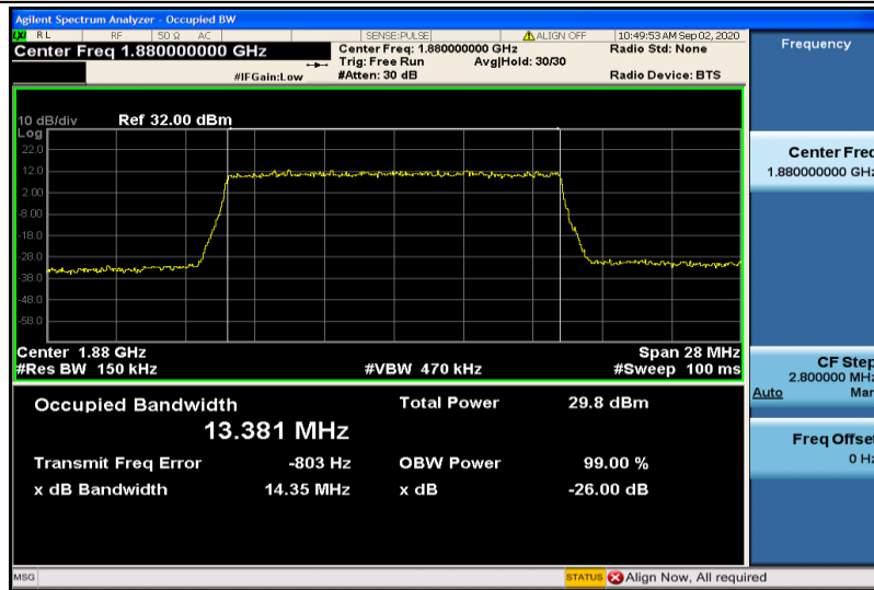
Band2-15MHz-16QAM-18900-75RB#0-13.381
