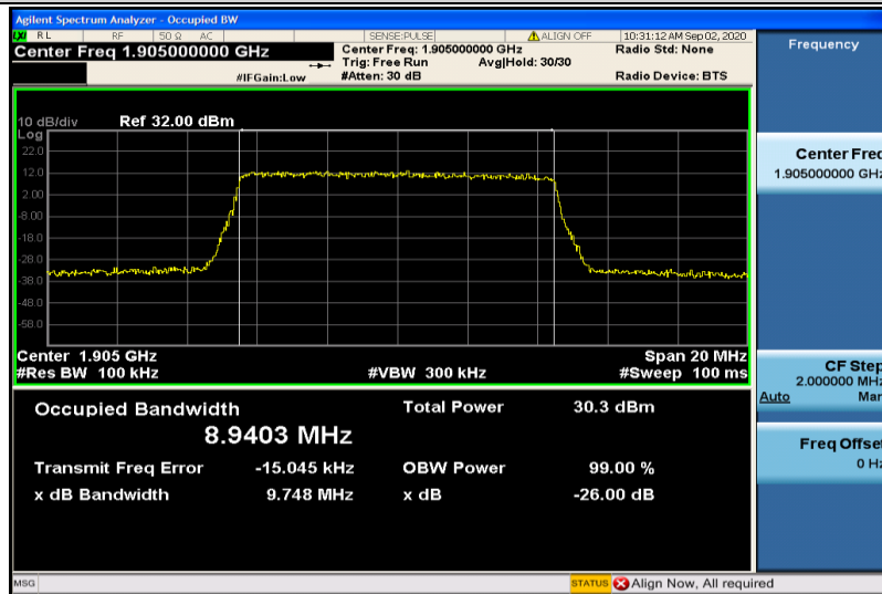
Band2-10MHz-QPSK-19150-50RB#0-8.9403
