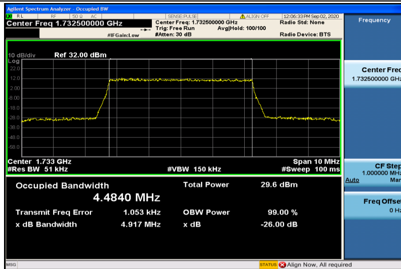
Band4-5MHz-16QAM-20175-25RB#0-4.4840
