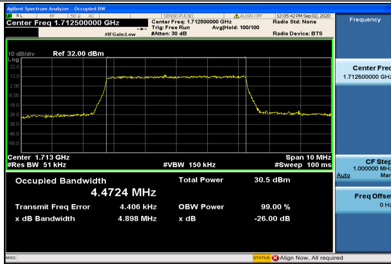
Band4-5MHz-QPSK-19975-25RB#0-4.4724
