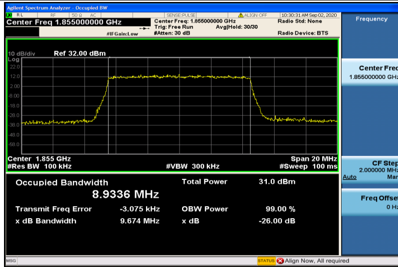
Band2-10MHz-QPSK-18650-50RB#0-8.9336
