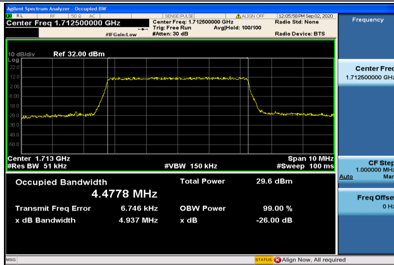
Band4-5MHz-16QAM-19975-25RB#0-4.4778
