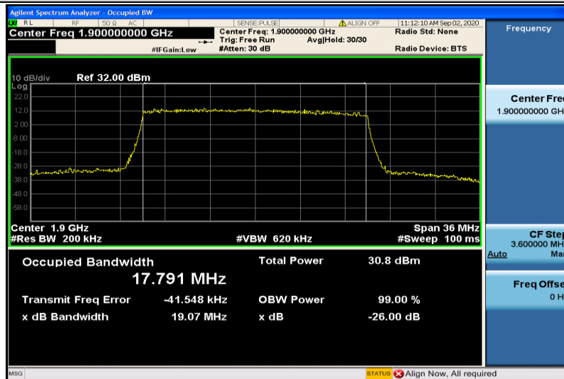
Band2-20MHz-QPSK-19100-100RB#0-17.791
