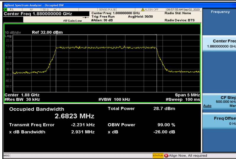
Band2-3MHz-16QAM-18900-15RB#0-2.6823
