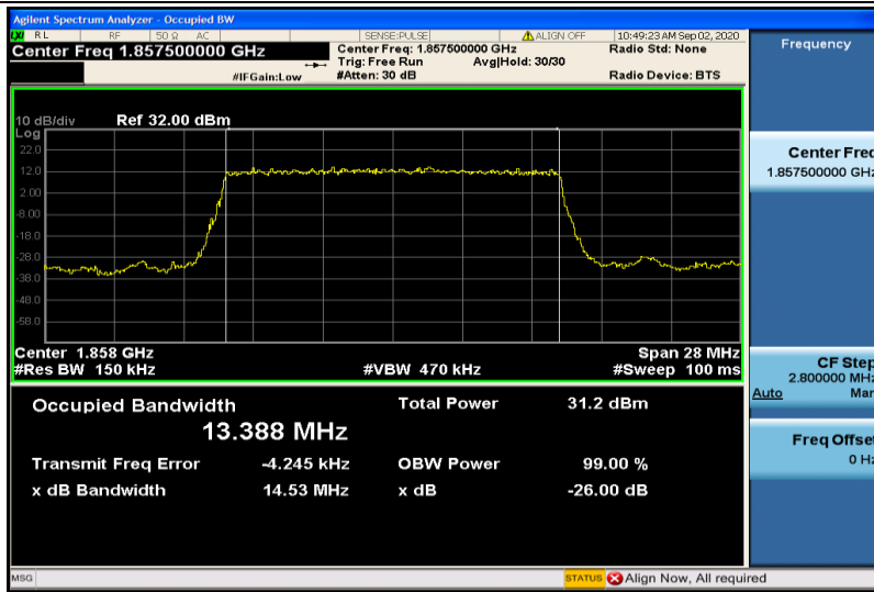
Band2-15MHz-QPSK-18675-75RB#0-13.388
