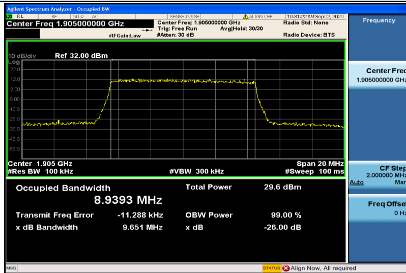
Band2-10MHz-16QAM-19150-50RB#0-8.9393
