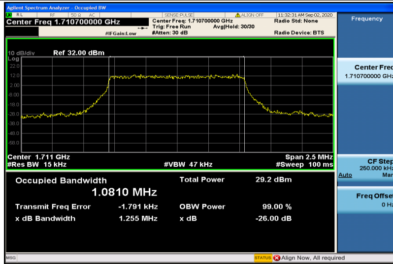
Band4-1.4MHz-QPSK-19957-6RB#0-1.0810
