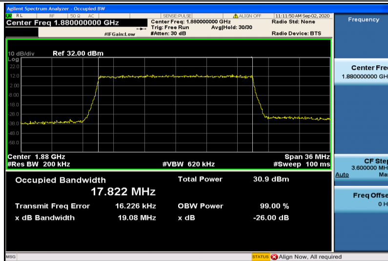
Band2-20MHz-QPSK-18900-100RB#0-17.822
