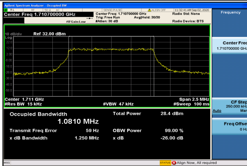
Band4-1.4MHz-16QAM-19957-6RB#0-1.0810
