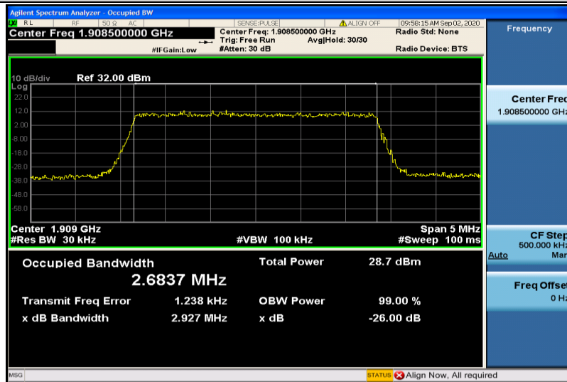
Band2-3MHz-16QAM-19185-15RB#0-2.6837
