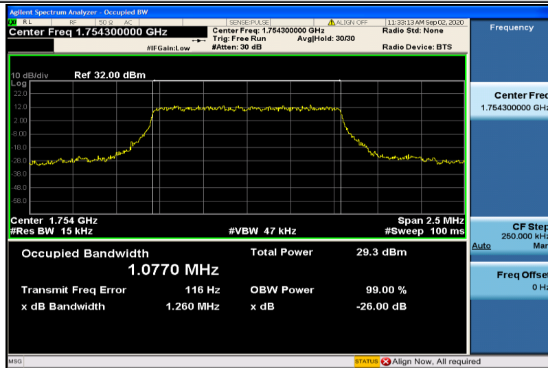
Band4-1.4MHz-QPSK-20393-6RB#0-1.0770
