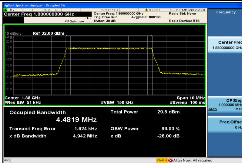
Band2-5MHz-16QAM-18900-25RB#0-4.4819
