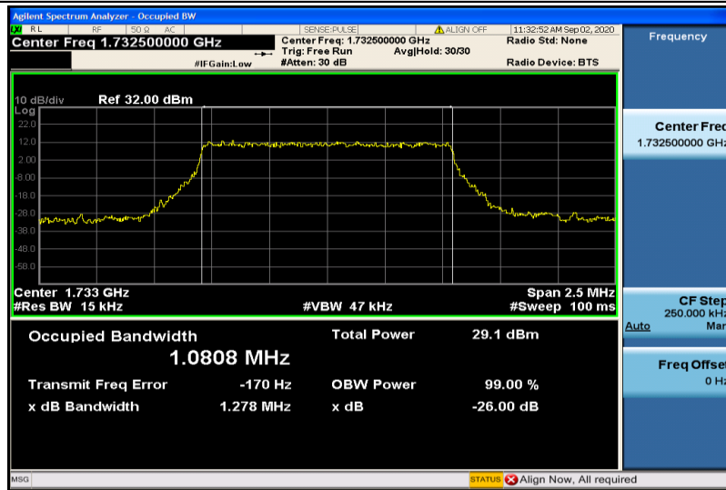
Band4-1.4MHz-QPSK-20175-6RB#0-1.0808
