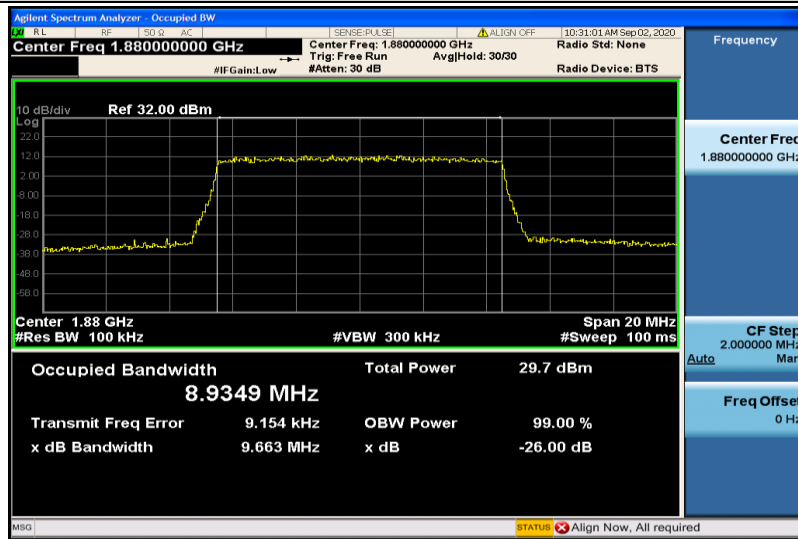
Band2-10MHz-16QAM-18900-50RB#0-8.9349
