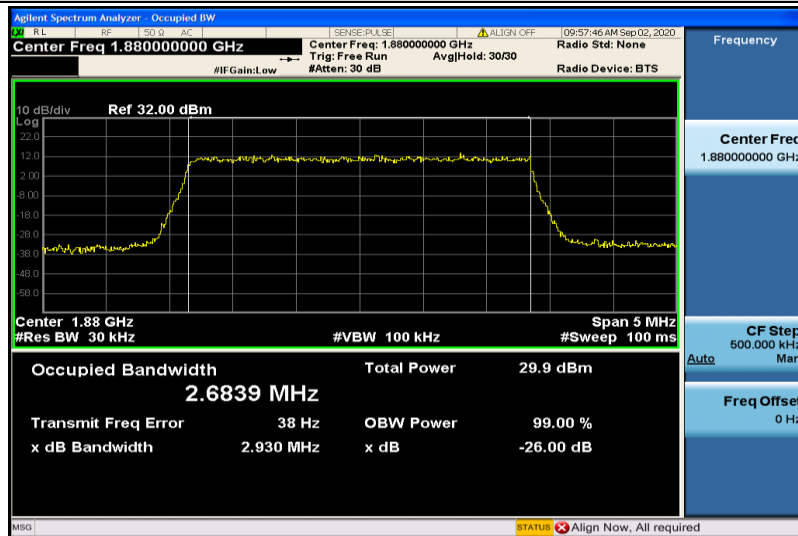
Band2-3MHz-QPSK-18900-15RB#0-2.6839
