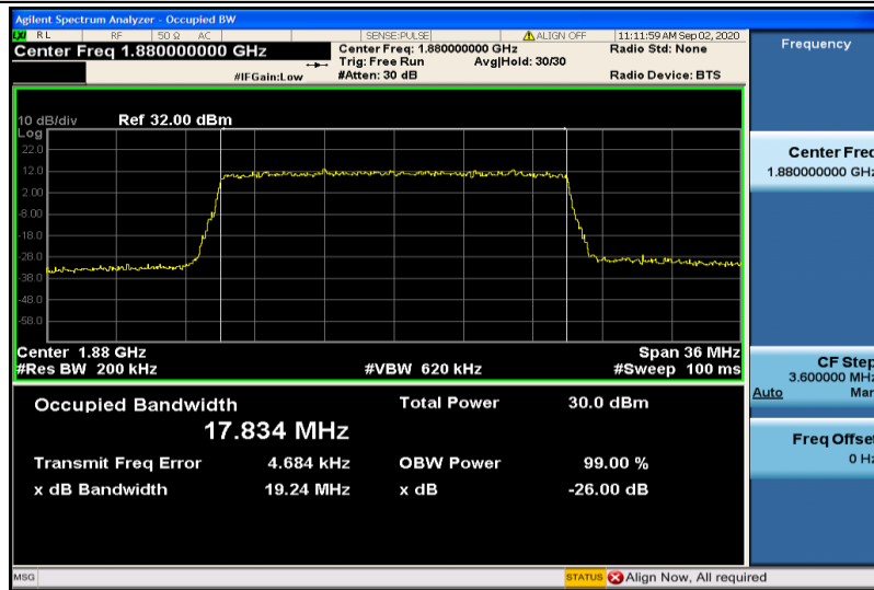
Band2-20MHz-16QAM-18900-100RB#0-17.834
