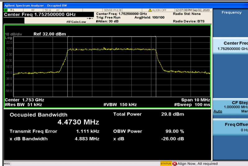
Band4-5MHz-16QAM-20375-25RB#0-4.4730
