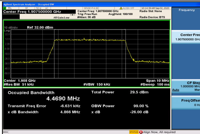
Band2-5MHz-16QAM-19175-25RB#0-4.4690
