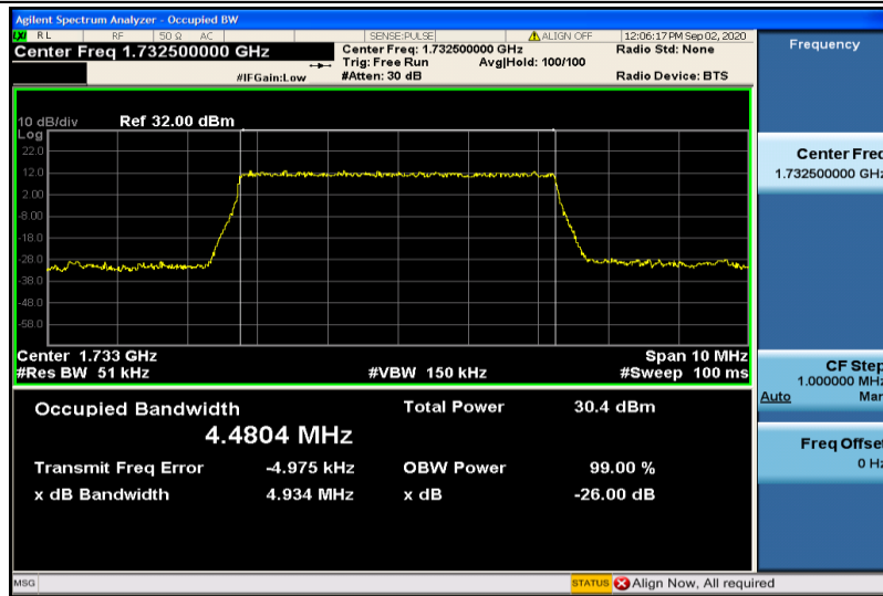
Band4-5MHz-QPSK-17325-25RB#0-4.4804
