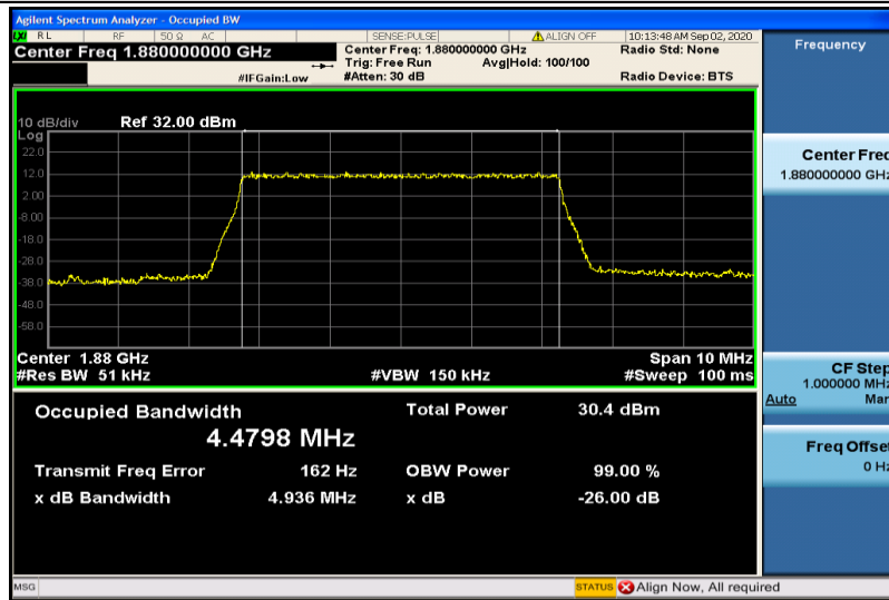
Band2-5MHz-QPSK-18900-25RB#0-4.4798
