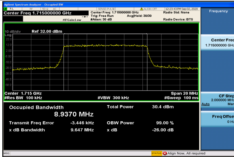
Band4-10MHz-QPSK-20000-50RB#0-8.9370
