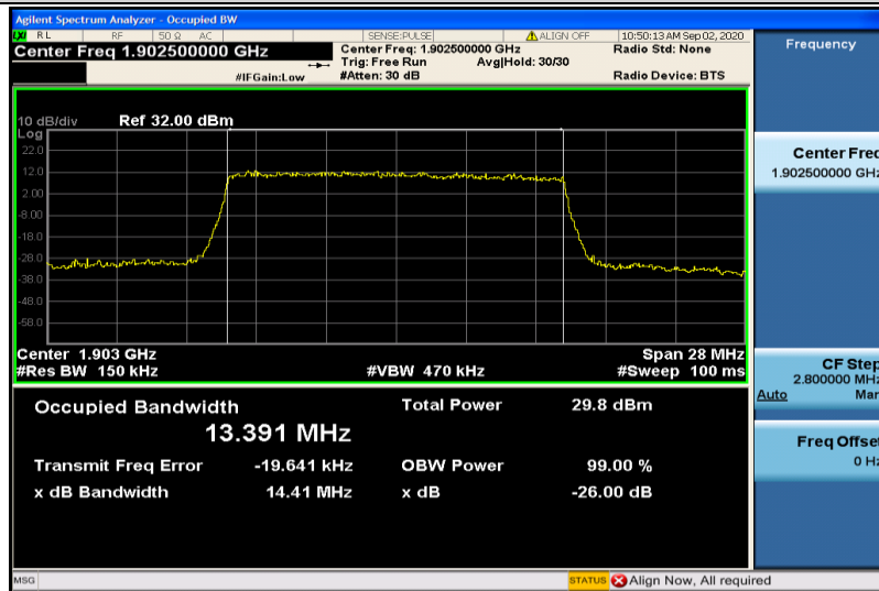
Band2-15MHz-16QAM-19125-75RB#0-13.391
