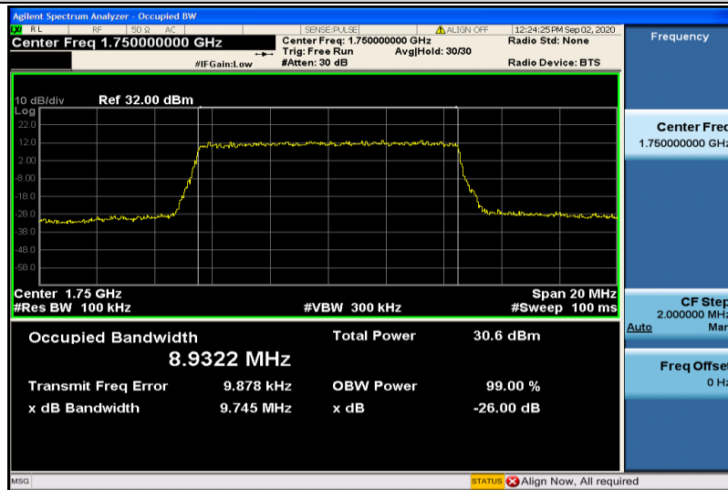
Band4-10MHz-QPSK-20350-50RB#0-8.9322
