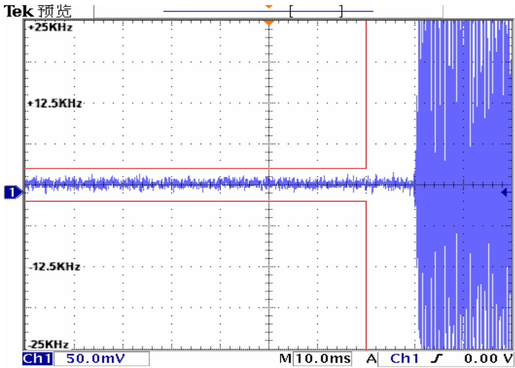
Transmitter Frequency Behaviour @ 25 KHz Channel Separations-----On – Off
