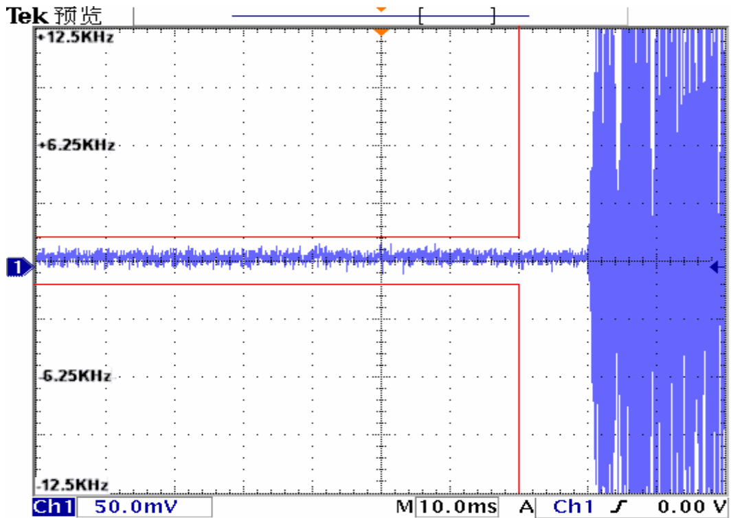
Transmitter Frequency Behaviour @ 12.5 KHz Channel Separation-----On - Off
