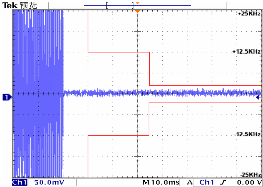
Transmitter Frequency Behaviour @ 25 KHz Channel Separation-----Off – On
