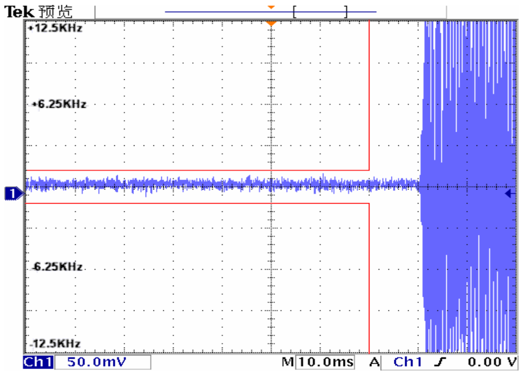
Transmitter Frequency Behaviour @ 12.5 KHz Channel Separation-----On - Off
