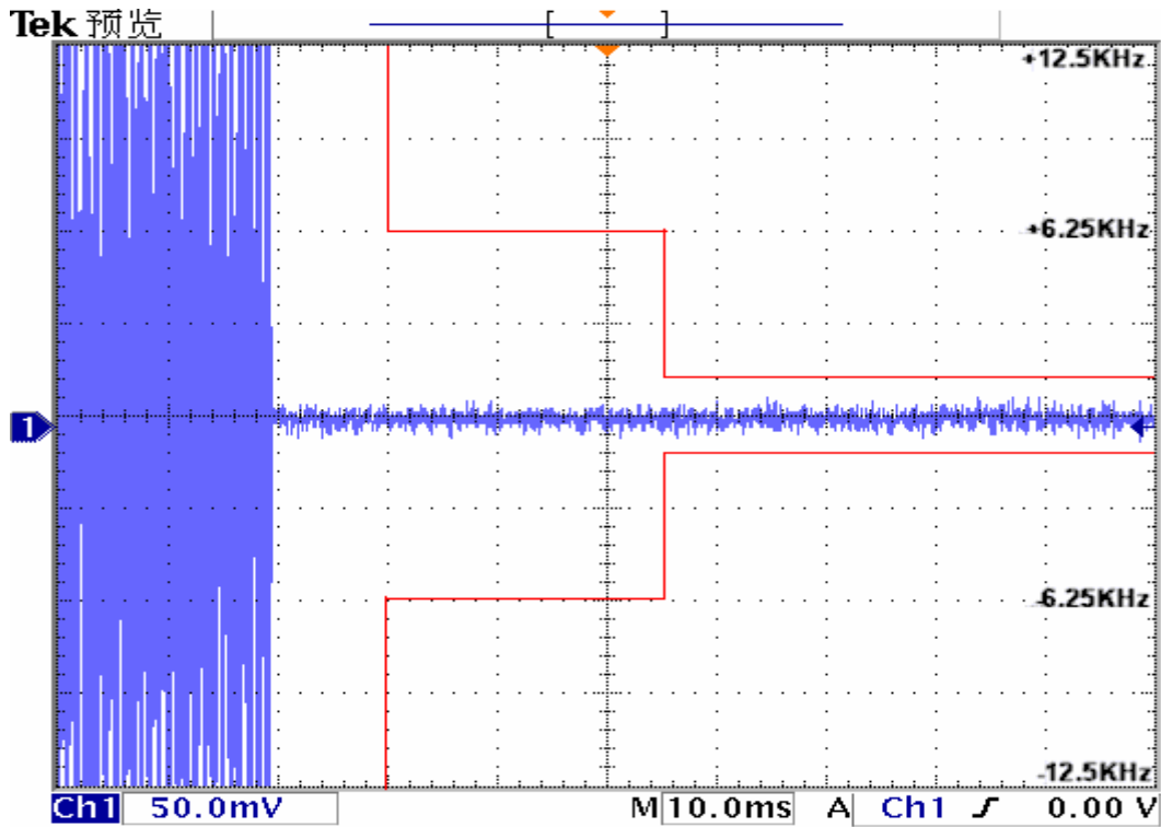
Transmitter Frequency Behaviour @ 12.5 KHz Channel Separation-----Off – On
