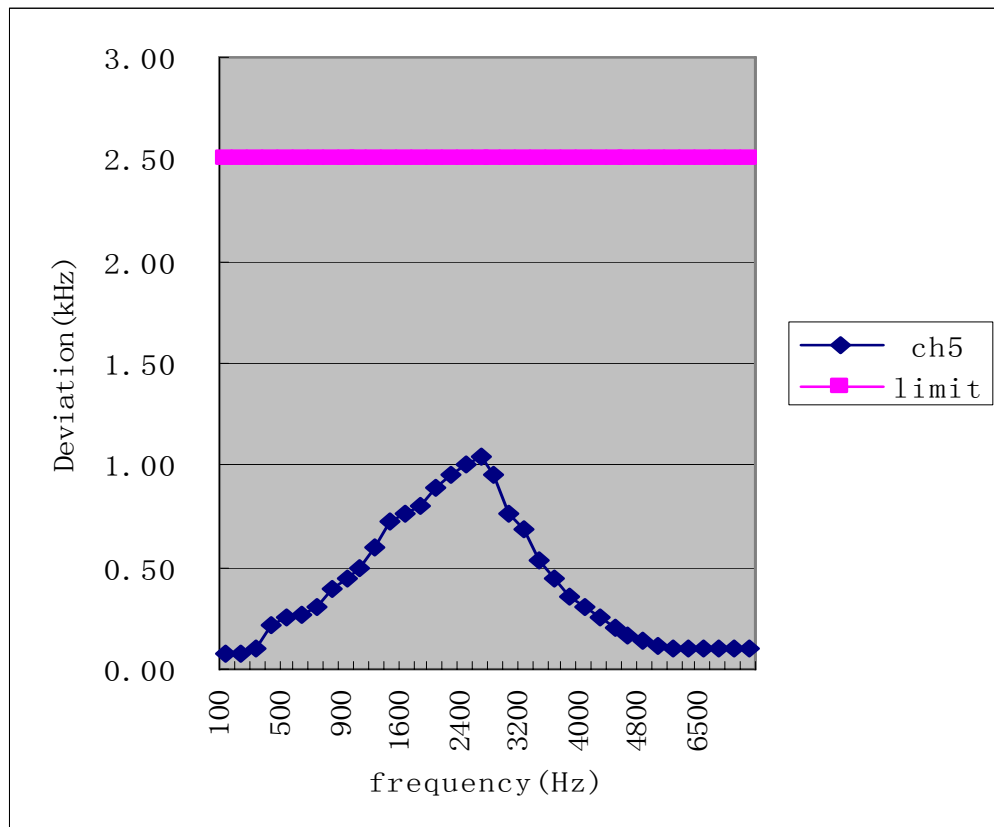
Figure 7 modulation test result
