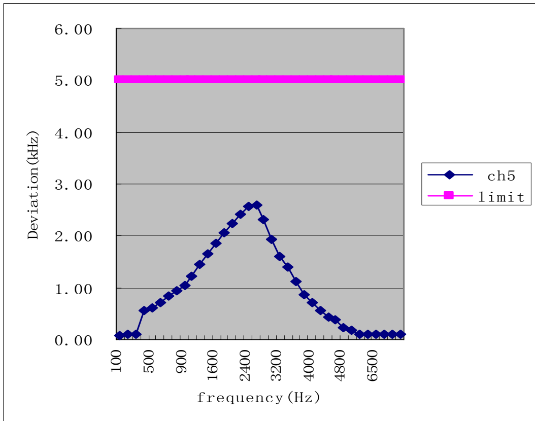
Figure 6 modulation test result
