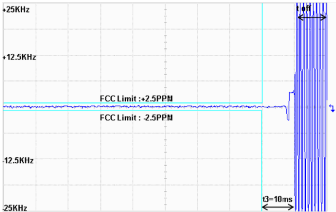
Transmitter Frequency Behaviour @ 12.5 KHz Channel Separation-----On - Off
