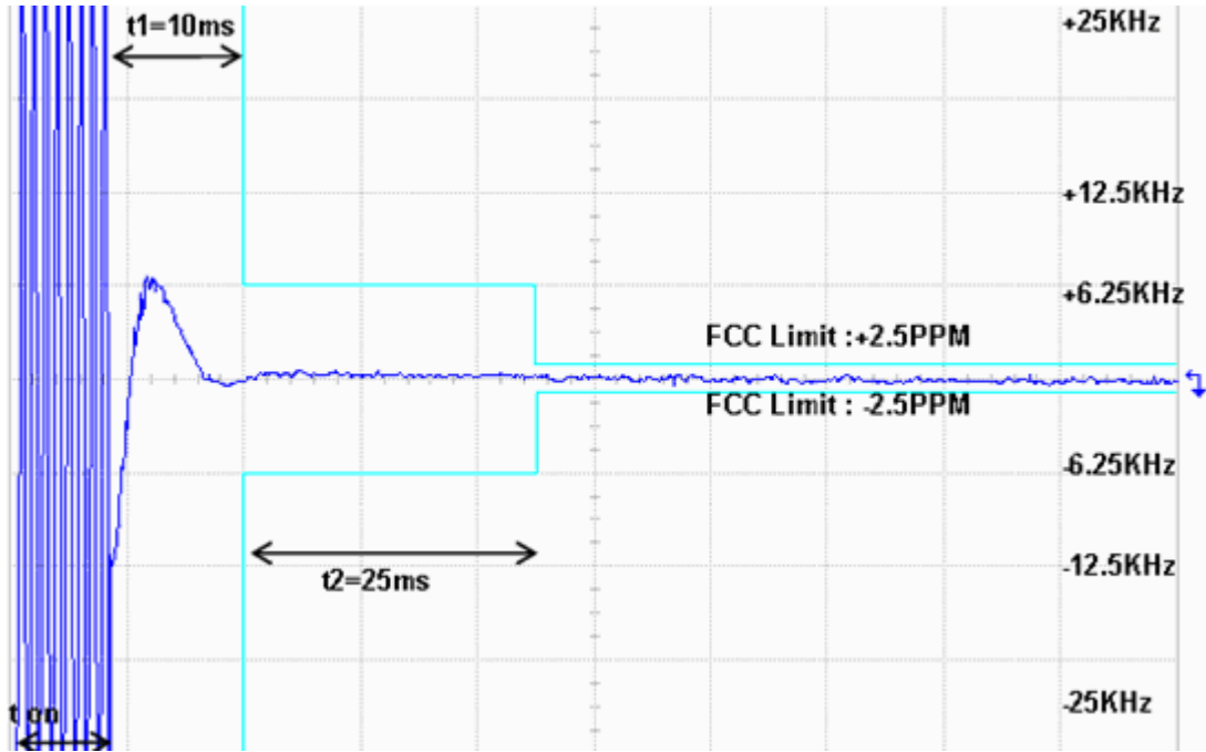
Transmitter Frequency Behaviour @ 12.5 KHz Channel Separation-----Off – On
