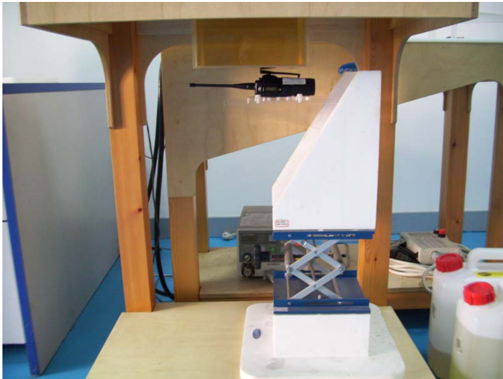
Fig.1 SARA2 System Test Layout
