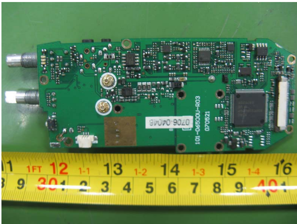
EUT – Main Board Bottom Components View
