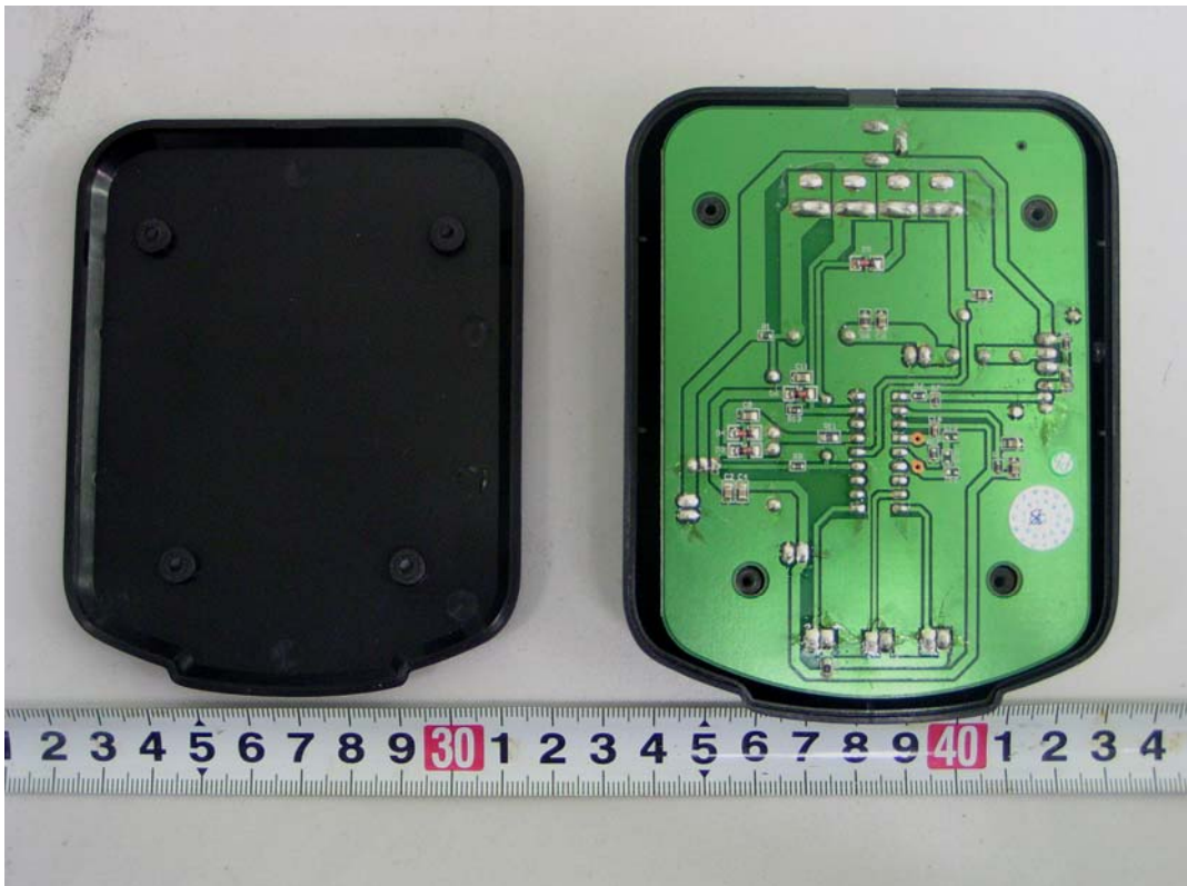
EUT – Charger Cover off View
