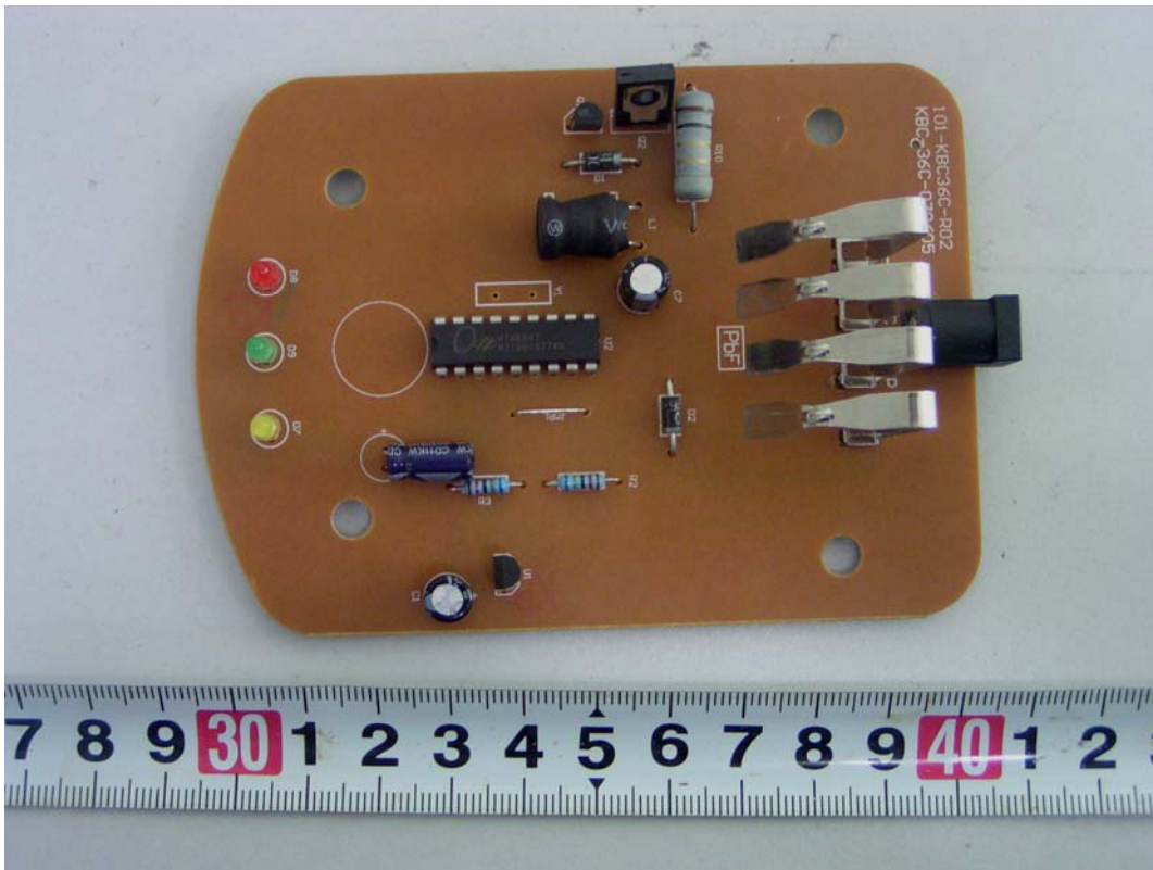
EUT – Charger Board Bottom Components View
