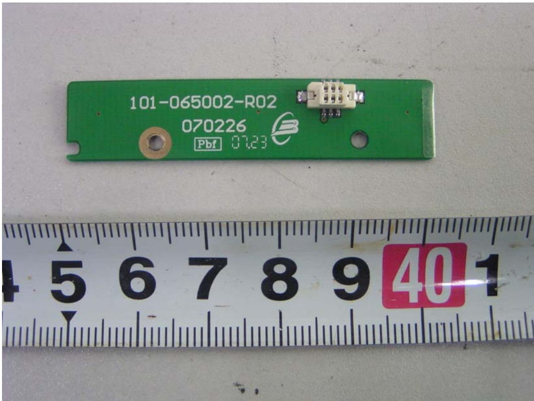
EUT – PTT Keyboard Board Bottom Components View
