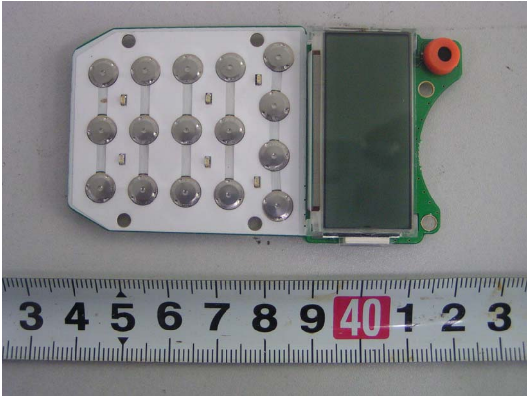
EUT – Main Keyboard Board Bottom Components View
