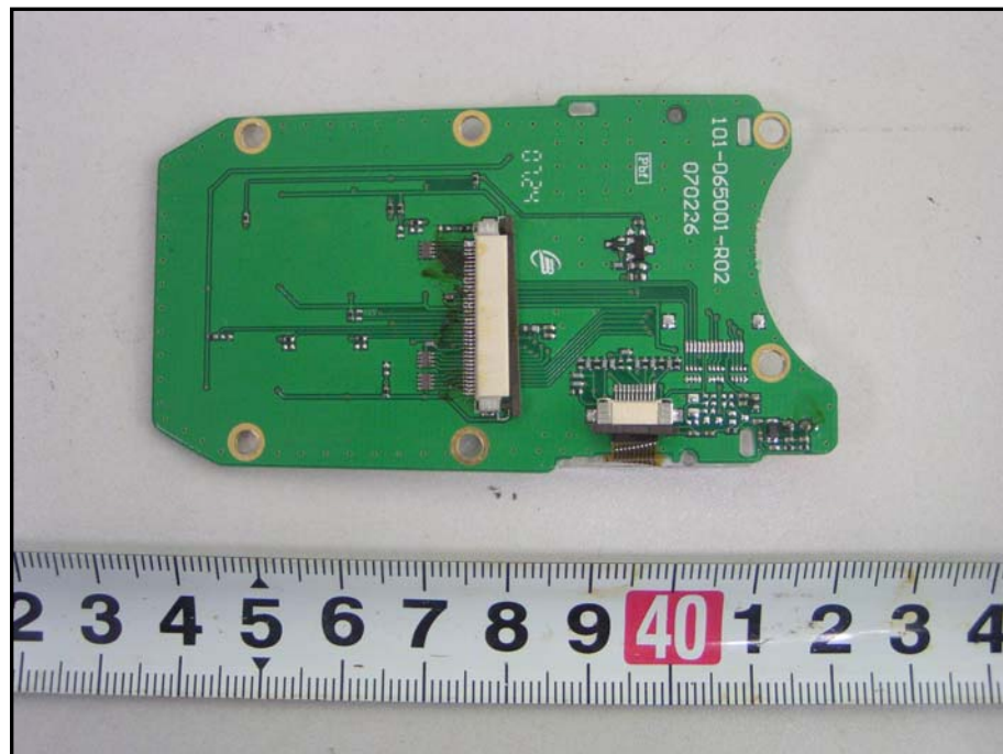
EUT – Main Keyboard Bottom View
