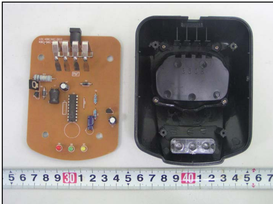
EUT – Charger Socket Uncovered off View
