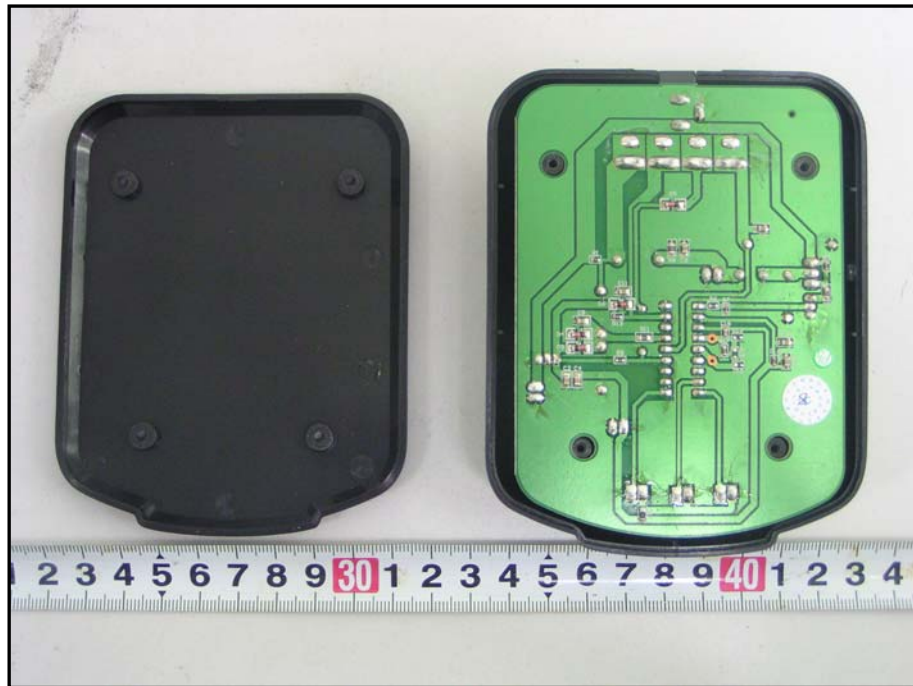
EUT – Charger Uncovered off View
