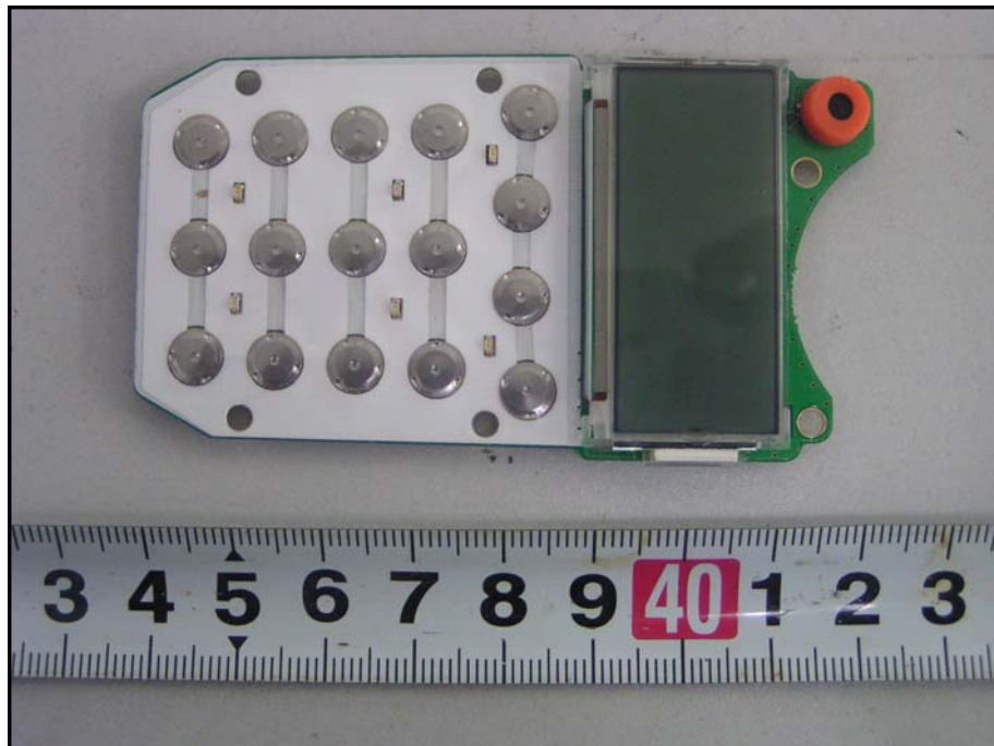
EUT – Main Keyboard Top View
