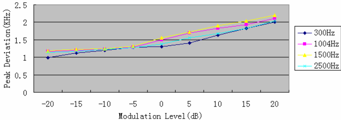
Modulation Limit-CH3
