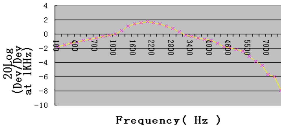
Audio Frequency Response - CH 03
