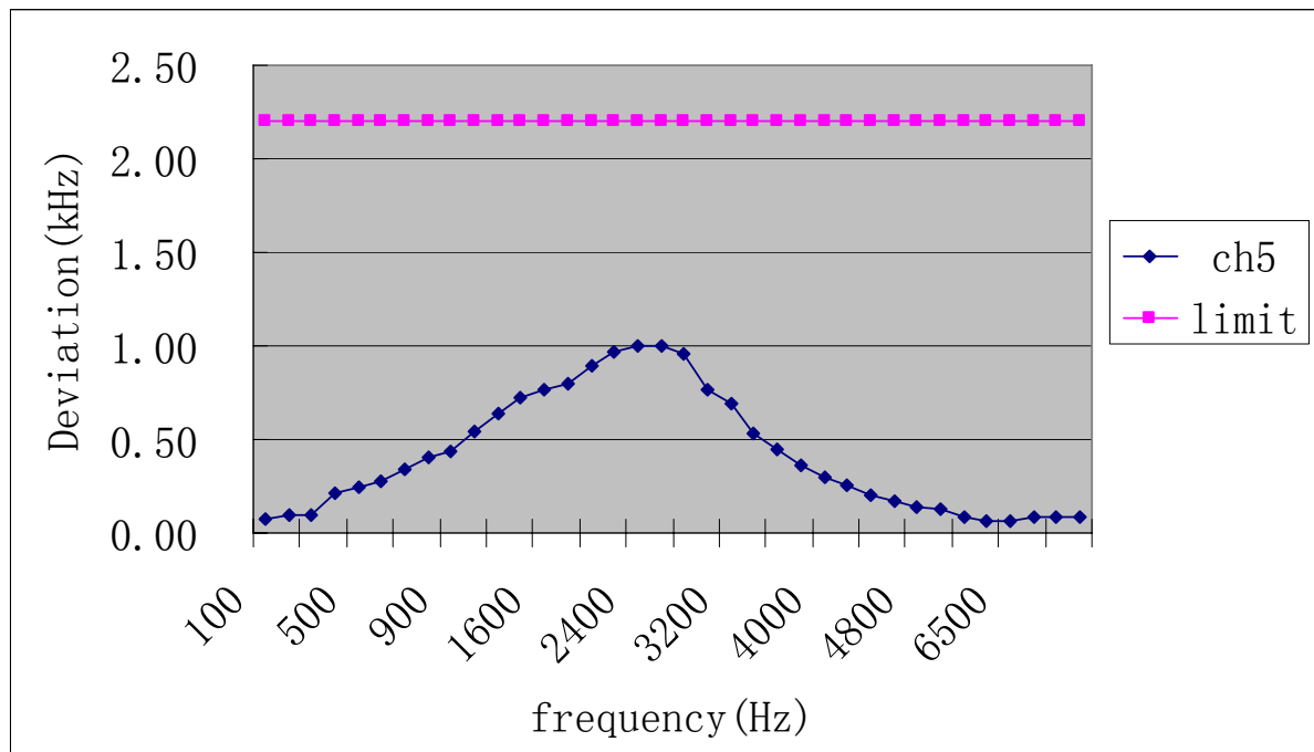
Figure 7 modulation test result
