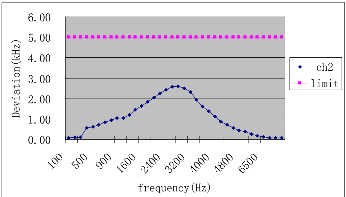
Figure 6 modulation test result
