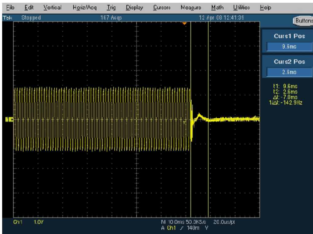
Transmitter Frequency Behaviour @ 12.5 KHz Channel Separation-----On - Off
