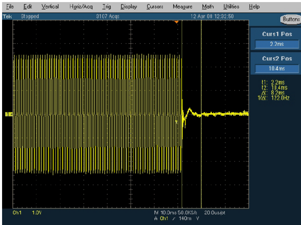
Transmitter Frequency Behaviour @ 25 KHz Channel Separation-----Off – On
