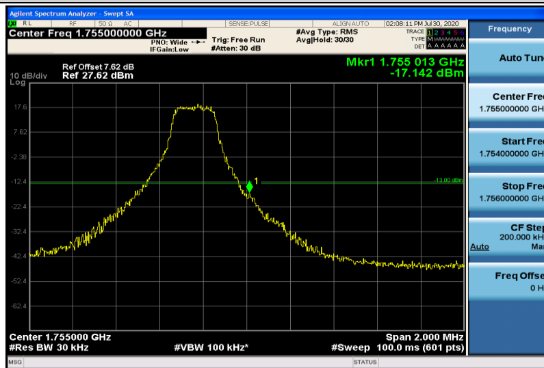
Band4-3MHz-QPSK-20385-1RB#14
