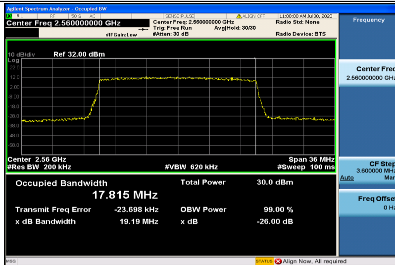
Band7-20MHz-16QAM-21350-100RB#0-17.815
