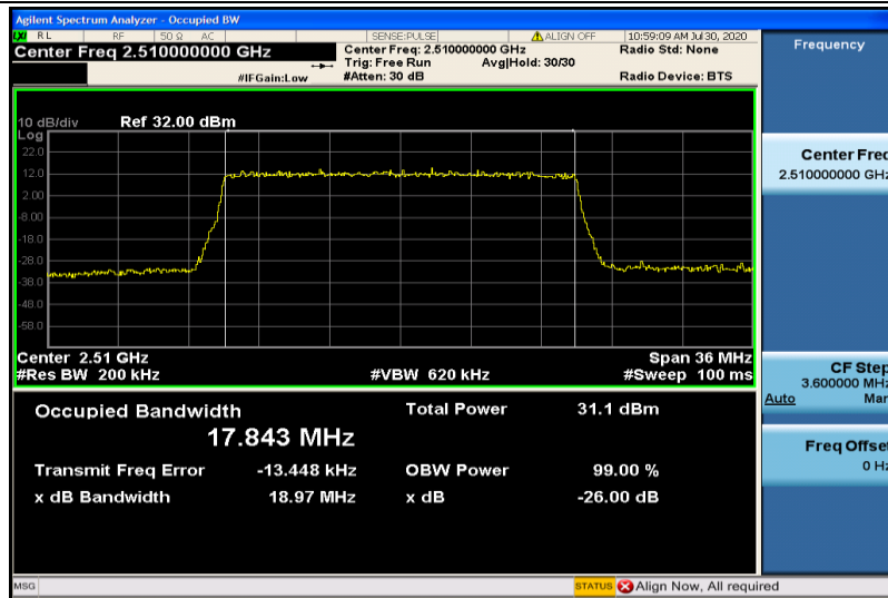
Band7-20MHz-QPSK-20850-100RB#0-17.843
