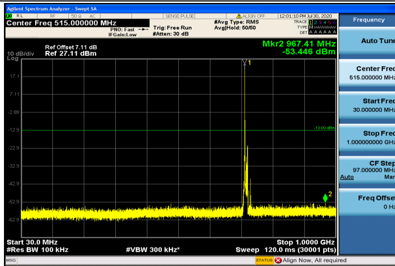
Band28-10MHz-16QAM-27410-1RB#0-30~1000MHz
