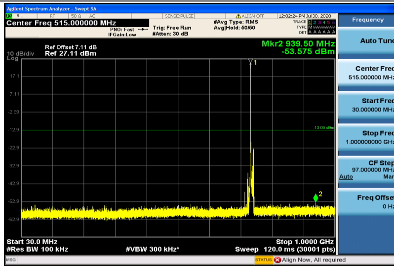
Band28-10MHz-16QAM-27610-1RB#0-30~1000MHz
