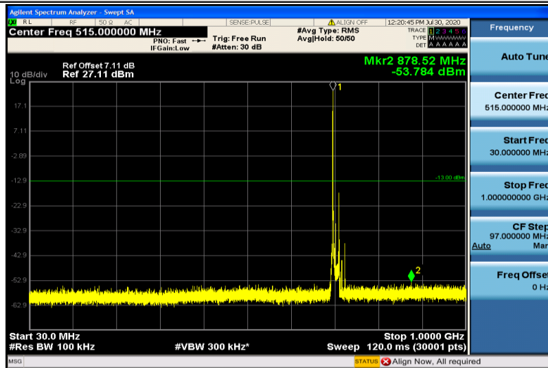
Band28-15MHz-QPSK-27285-1RB#0-30~1000MHz
