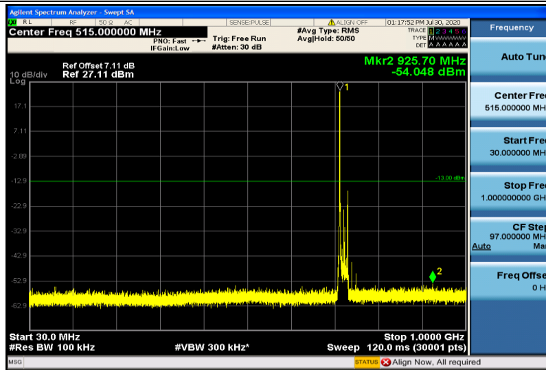
Band28-20MHz-16QAM-27460-1RB#0-30~1000MHz
