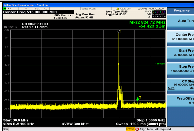
Band28-20MHz-16QAM-27310-1RB#0-30~1000MHz
