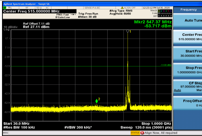
Band28-15MHz-QPSK-27585-1RB#0-30~1000MHz
