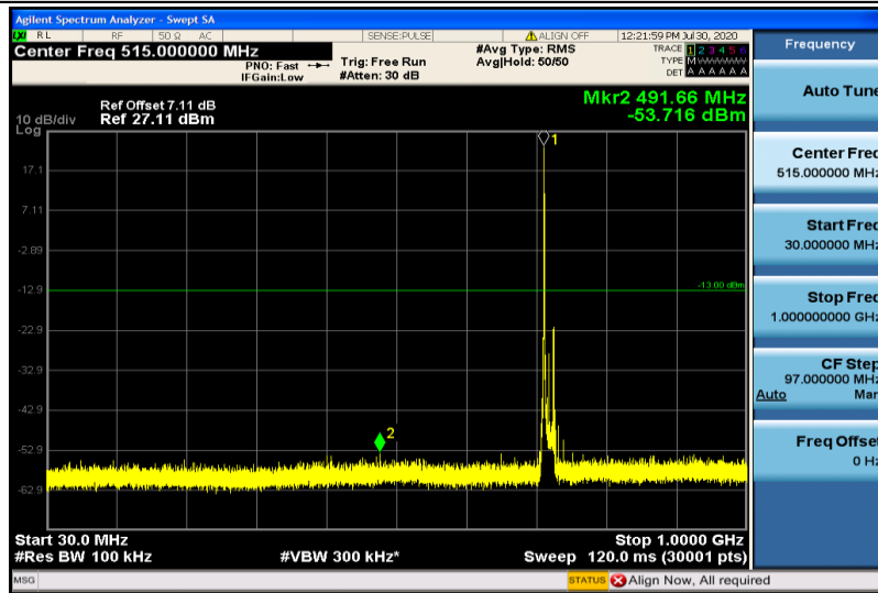
Band28-15MHz-QPSK-27435-1RB#0-30~1000MHz
