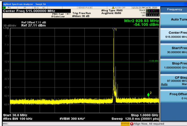
Band28-15MHz-16QAM-27285-1RB#0-30~1000MHz
