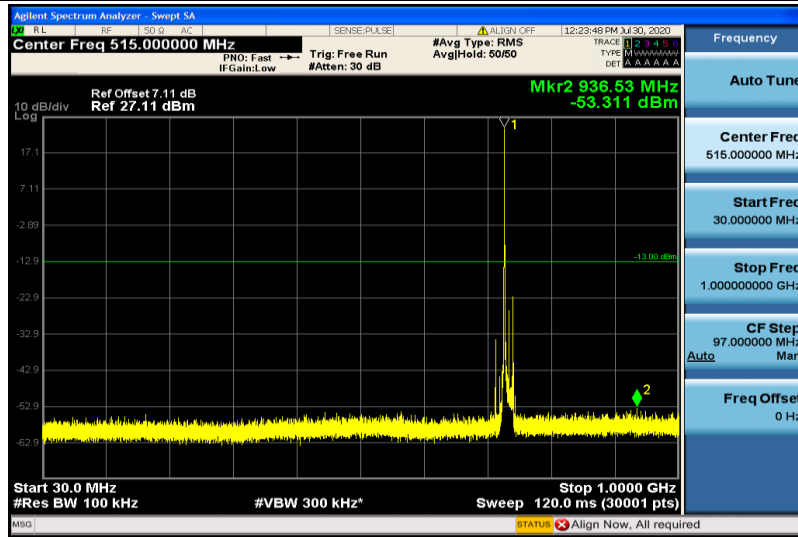
Band28-15MHz-16QAM-27585-1RB#0-30~1000MHz
