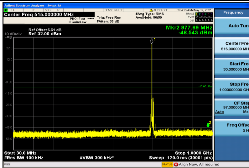
Band12-10MHz-16QAM-23095-1RB#0-30~1000MHz
