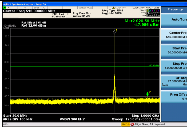
Band12-5MHz-16QAM-23095-1RB#0-30~1000MHz
