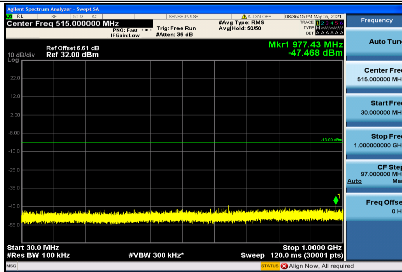
Band4-15MHz-QPSK-20175-1RB#0-30~1000MHz
