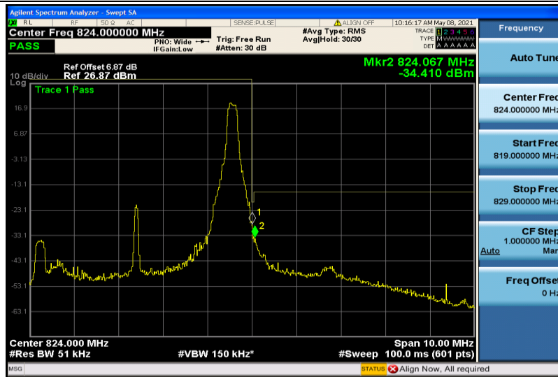
Band26-5MHz-QPSK-26765-1RB#24
