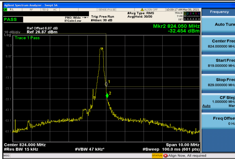
Band26-1.4MHz-16QAM-26783-1RB#5
