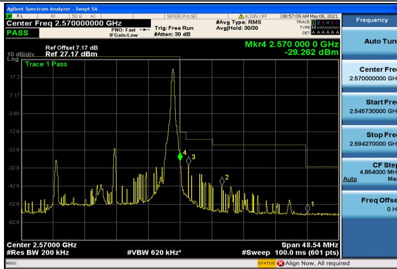
Band7-20MHz-QPSK-21350-1RB#99
