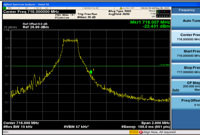
Band12-1.4MHz-16QAM-23173-1RB#5
