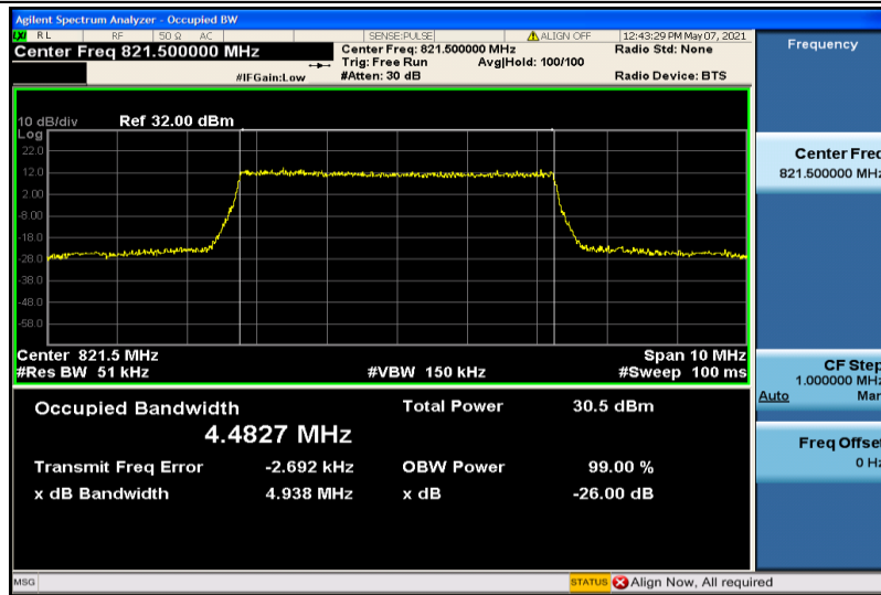
Band26-5MHz-QPSK-26765-25RB#0-4.4827
