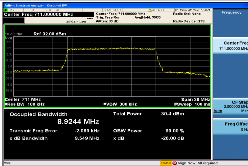
Band12-10MHz-16QAM-23130-50RB#0-8.9244
