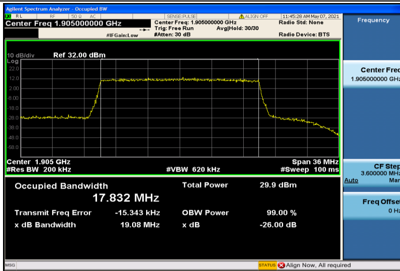
Band25-20MHz-16QAM-26590-100RB#0-17.832
