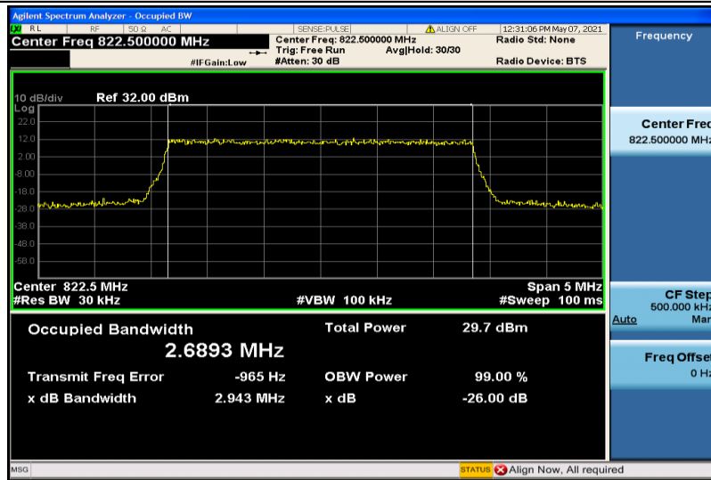
Band26-3MHz-QPSK-26775-15RB#0-2.6893
