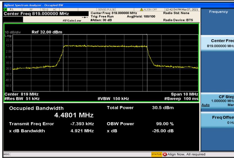
Band26-5MHz-QPSK-26740-25RB#0-4.4801
