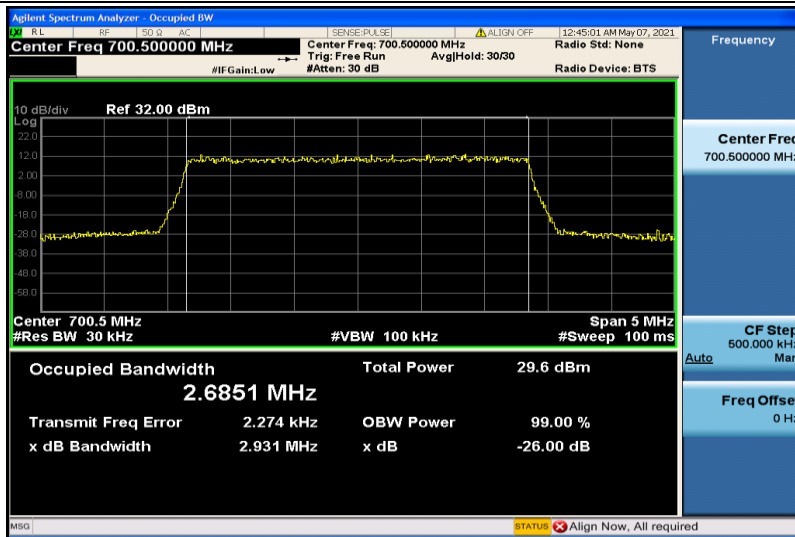
Band12-3MHz-16QAM-23025-15RB#0-2.6851
