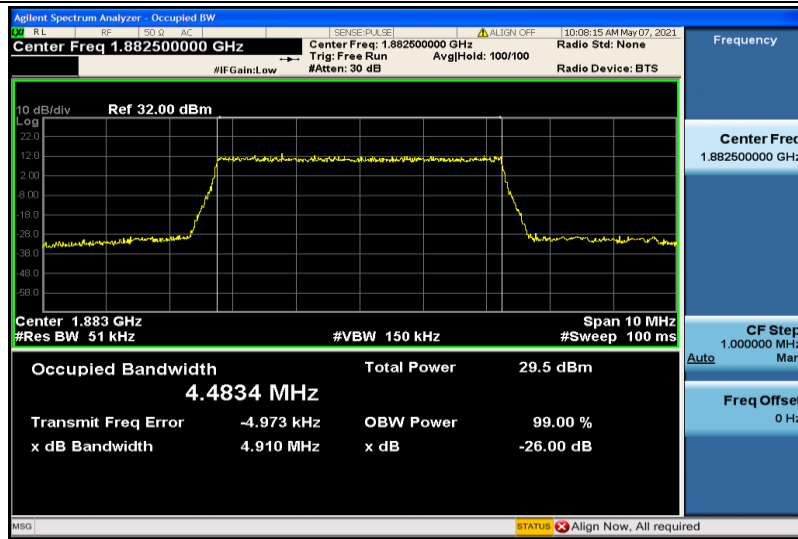
Band25-5MHz-16QAM-26365-25RB#0-4.4834
