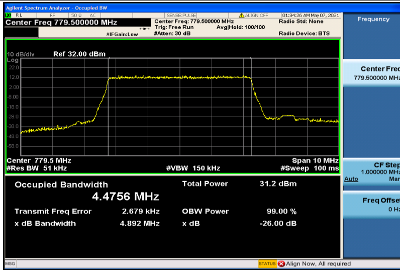
Band13-5MHz-QPSK-23205-25RB#0-4.4756
