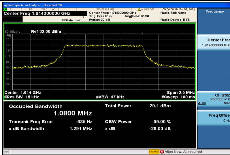
Band25-1.4MHz-QPSK-26683-6RB#0-1.0800
