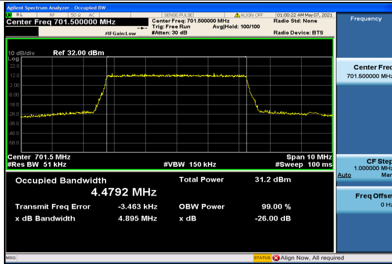
Band12-5MHz-QPSK-23035-25RB#0-4.4792
