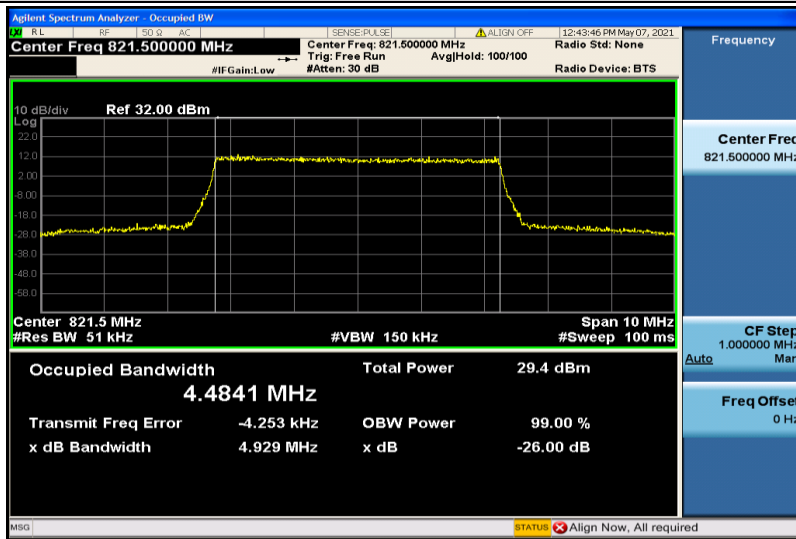
Band26-5MHz-16QAM-26765-25RB#0-4.4841
