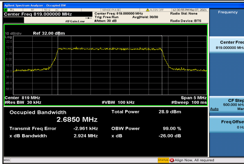
Band26-3MHz-16QAM-26740-15RB#0-2.6850
