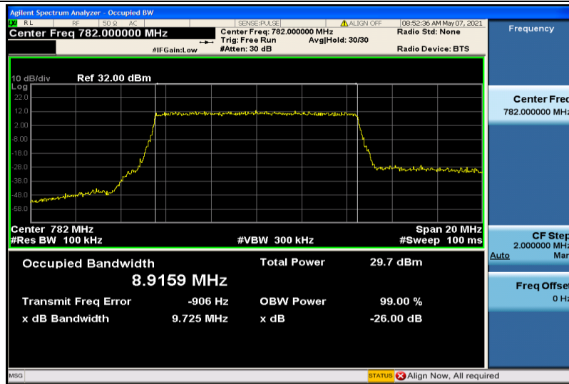
Band13-10MHz-16QAM-23230-50RB#0-8.9159
