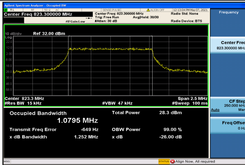
Band26-1.4MHz-16QAM-26783-6RB#0-1.0795
