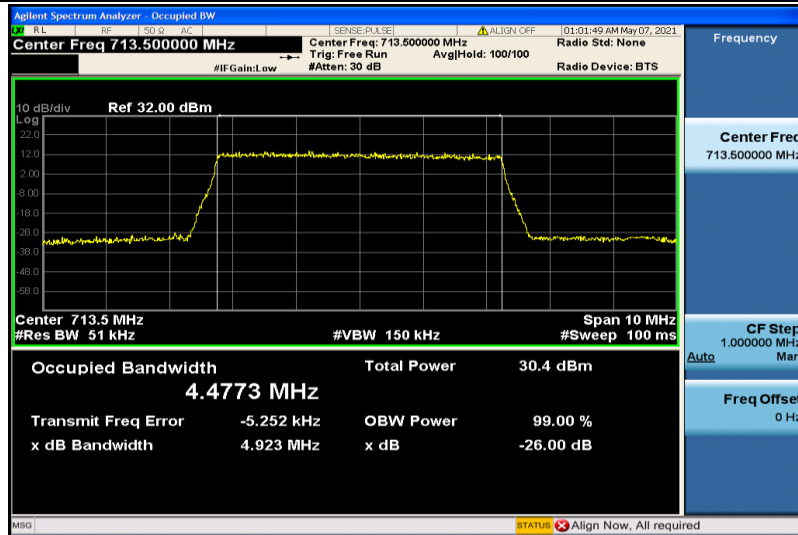
Band12-5MHz-16QAM-23155-25RB#0-4.4773
