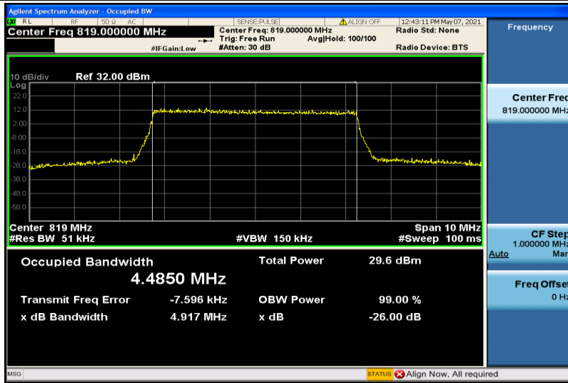
Band26-5MHz-16QAM-26740-25RB#0-4.4850
