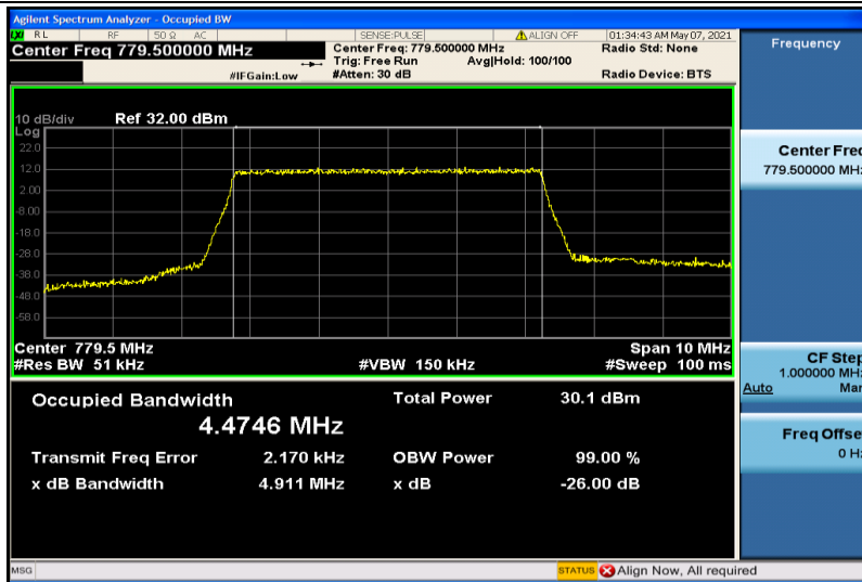
Band13-5MHz-16QAM-23205-25RB#0-4.4746
