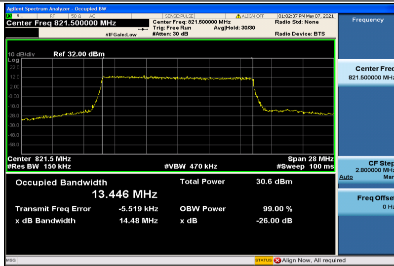
Band26-15MHz-QPSK-26765-75RB#0-13.446
