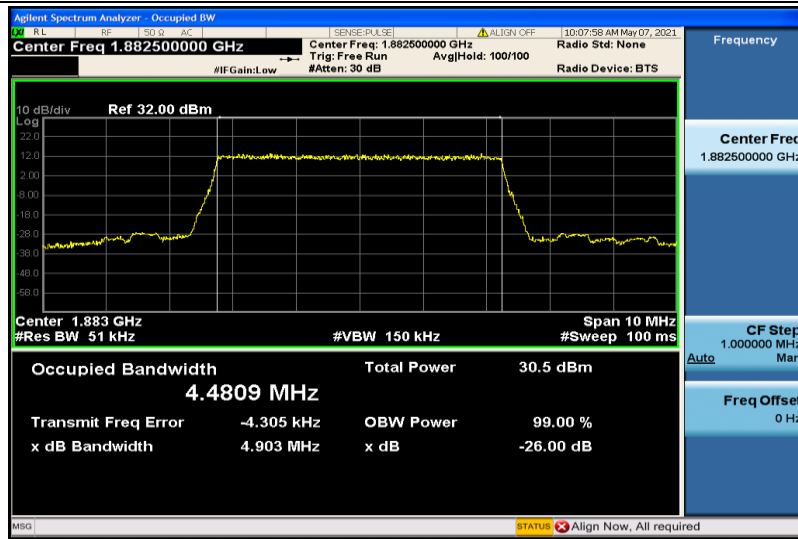
Band25-5MHz-QPSK-26365-25RB#0-4.4809
