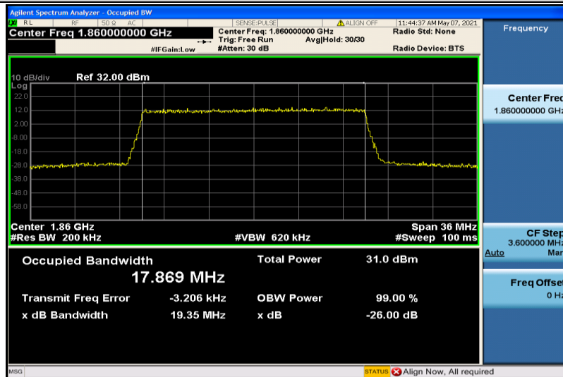
Band25-20MHz-QPSK-26140-100RB#0-17.869
