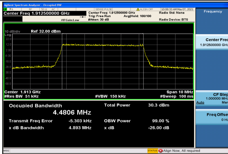
Band25-5MHz-QPSK-26665-25RB#0-4.4806
