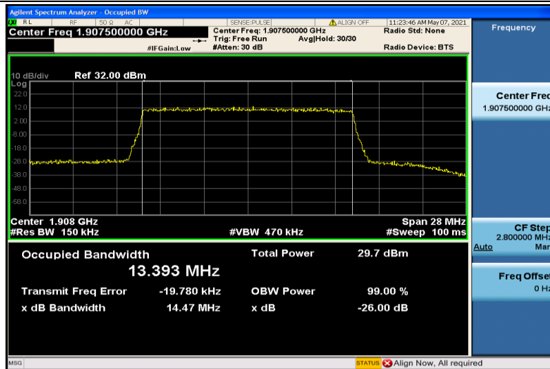
Band25-15MHz-16QAM-26615-75RB#0-13.393
