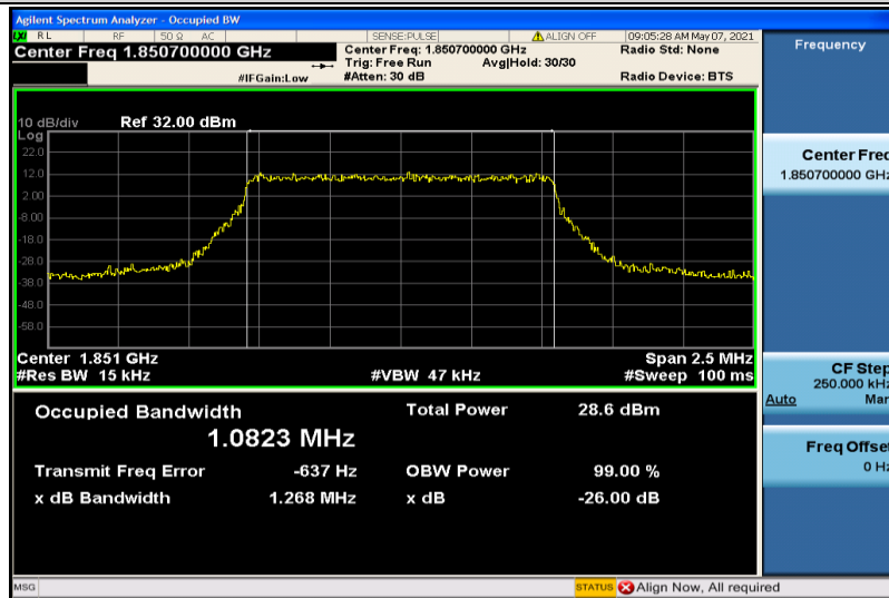
Band25-1.4MHz-16QAM-26047-6RB#0-1.0823
