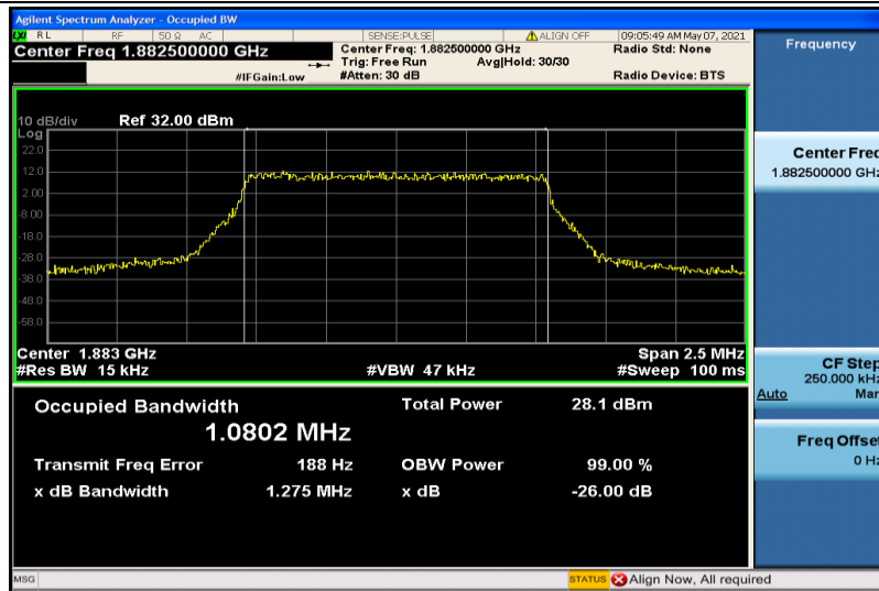
Band25-1.4MHz-16QAM-26365-6RB#0-1.0802
