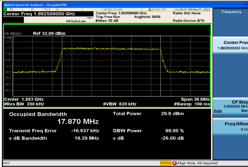
Band25-20MHz-16QAM-26365-100RB#0-17.870
