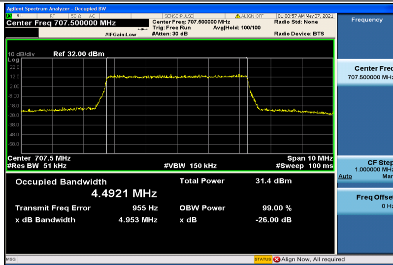
Band12-5MHz-QPSK-23095-25RB#0-4.4921
