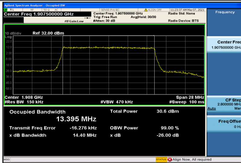
Band25-15MHz-QPSK-26615-75RB#0-13.395
