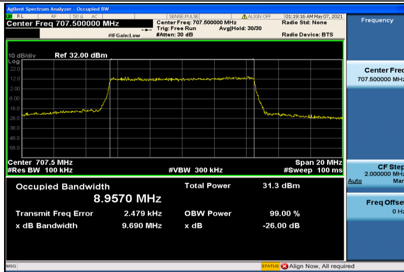
Band12-10MHz-QPSK-23095-50RB#0-8.9570
