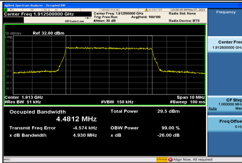
Band25-5MHz-16QAM-26665-25RB#0-4.4812
