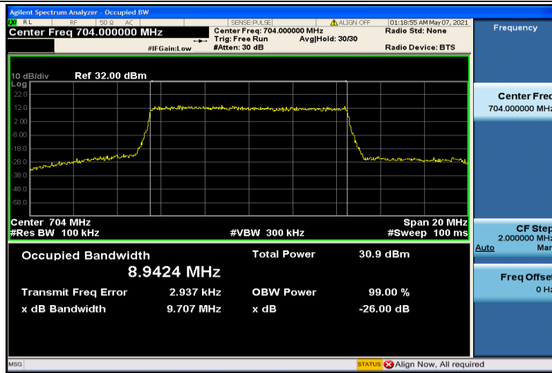
Band12-10MHz-QPSK-23060-50RB#0-8.9424
