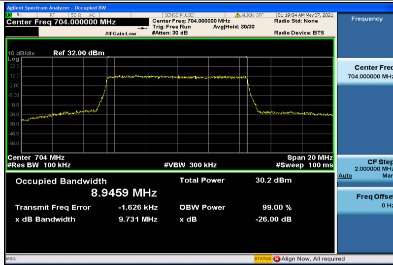
Band12-10MHz-16QAM-23060-50RB#0-8.9459
