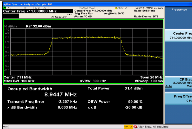
Band12-10MHz-QPSK-23130-50RB#0-8.9447
