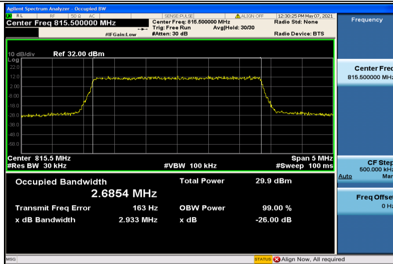
Band26-3MHz-QPSK-26705-15RB#0-2.6854
