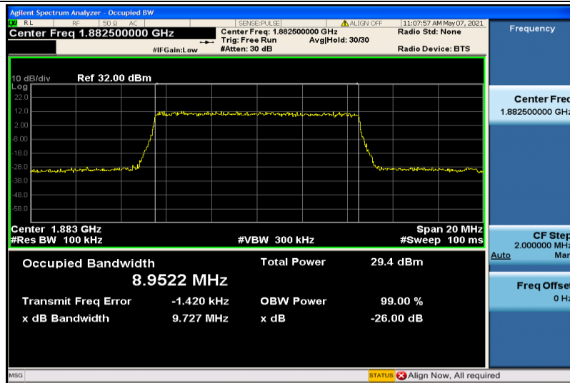
Band25-10MHz-16QAM-26365-50RB#0-8.9522
