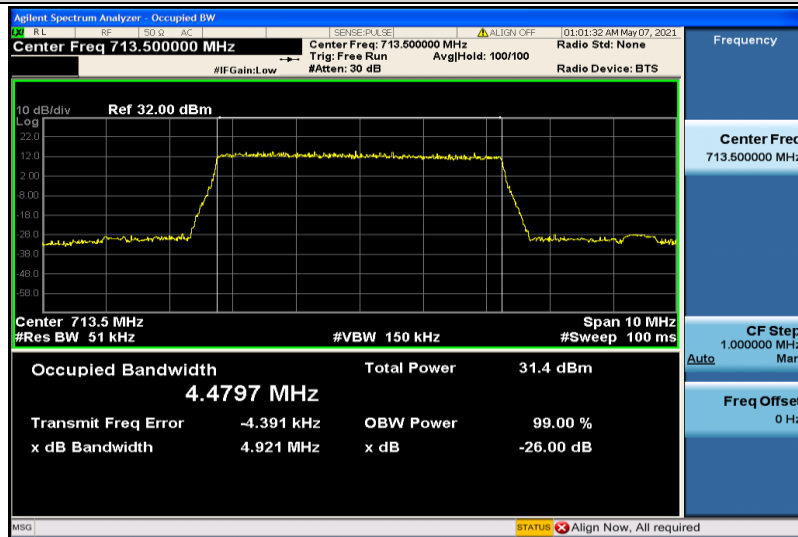
Band12-5MHz-QPSK-23155-25RB#0-4.4797
