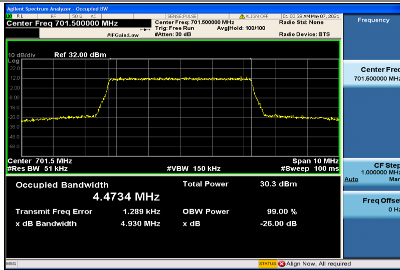
Band12-5MHz-16QAM-23035-25RB#0-4.4734
