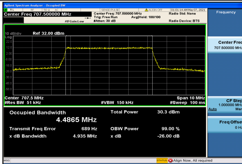
Band12-5MHz-16QAM-23095-25RB#0-4.4865
