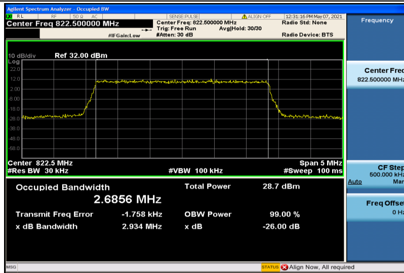
Band26-3MHz-16QAM-26775-15RB#0-2.6856
