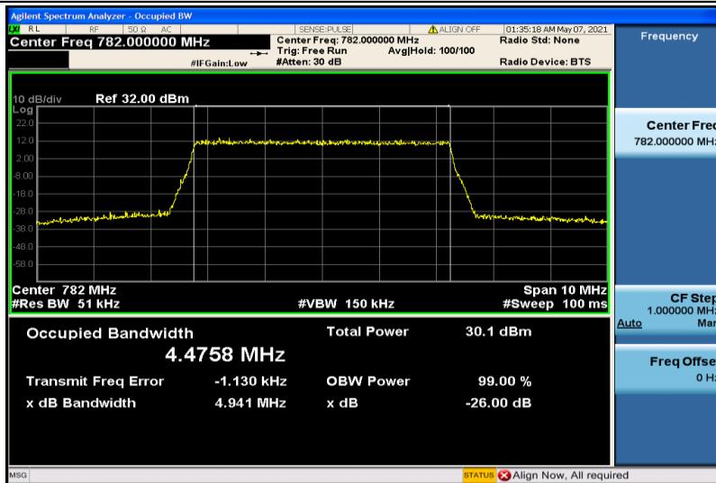
Band13-5MHz-16QAM-23230-25RB#0-4.4758
