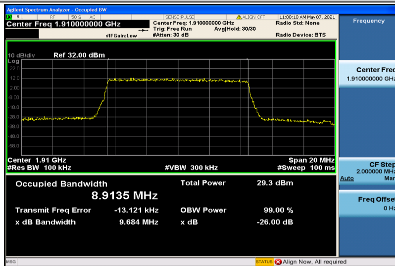
Band25-10MHz-16QAM-26640-50RB#0-8.9135
