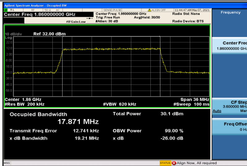
Band25-20MHz-16QAM-26140-100RB#0-17.871
