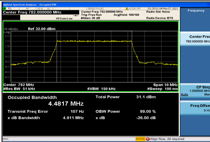
Band13-5MHz-QPSK-23230-25RB#0-4.4817
