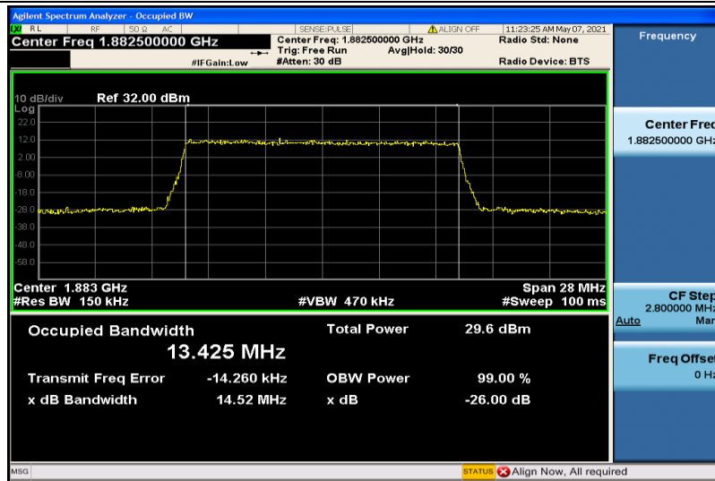
Band25-15MHz-16QAM-26365-75RB#0-13.425
