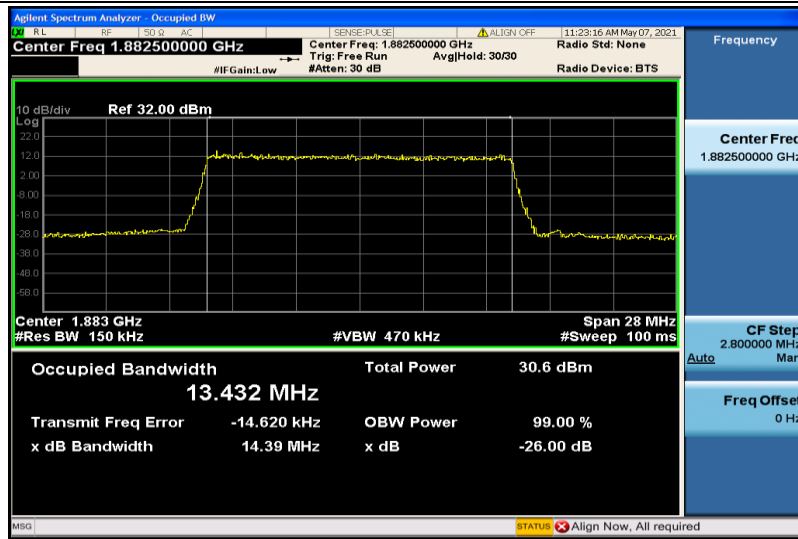
Band25-15MHz-QPSK-26365-75RB#0-13.432
