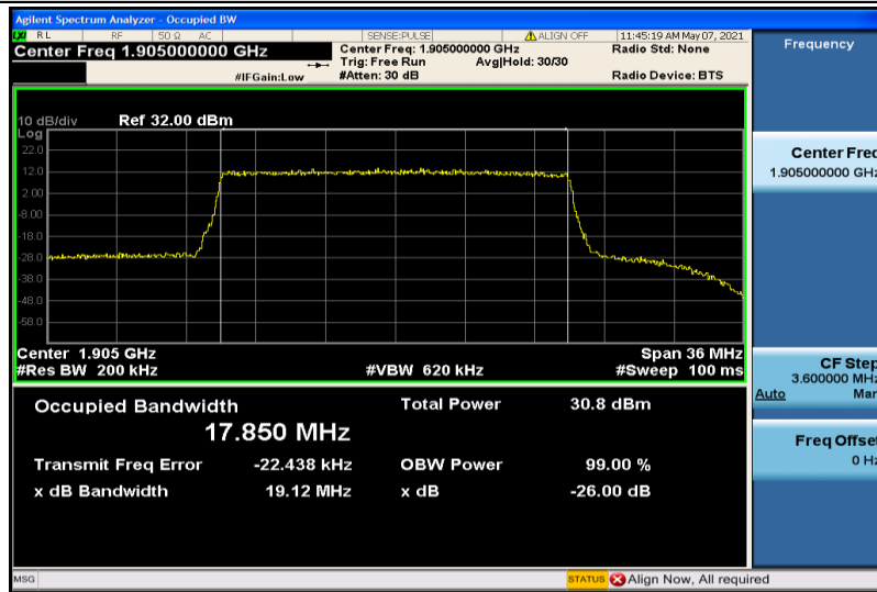
Band25-20MHz-QPSK-26590-100RB#0-17.850
