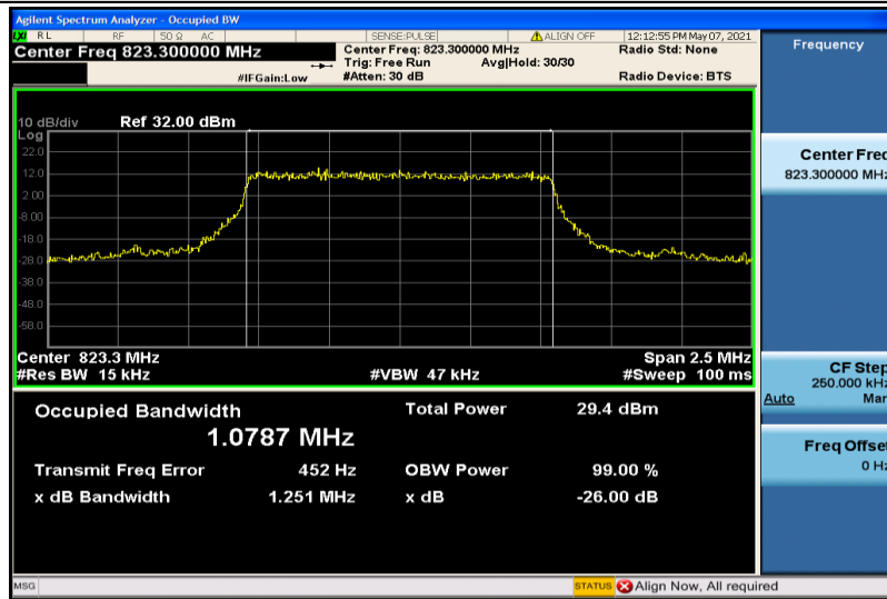
Band26-1.4MHz-QPSK-26783-6RB#0-1.0787
