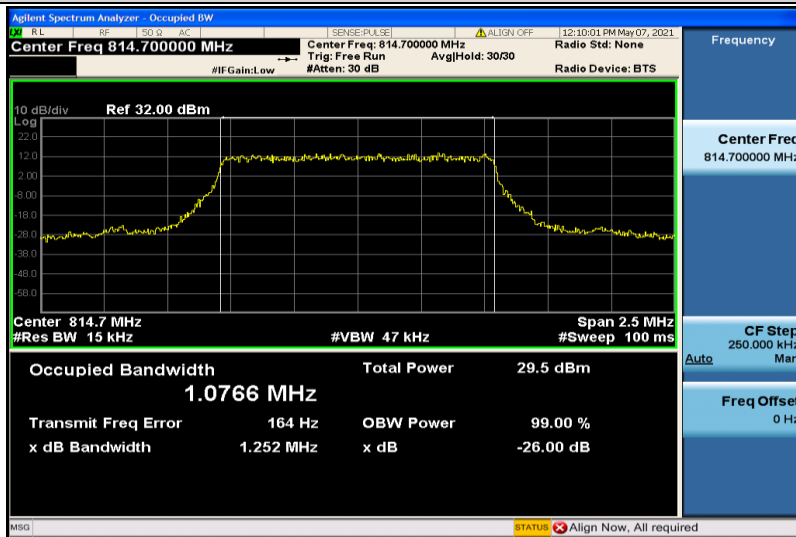
Band26-1.4MHz-QPSK-26697-6RB#0-1.0766
