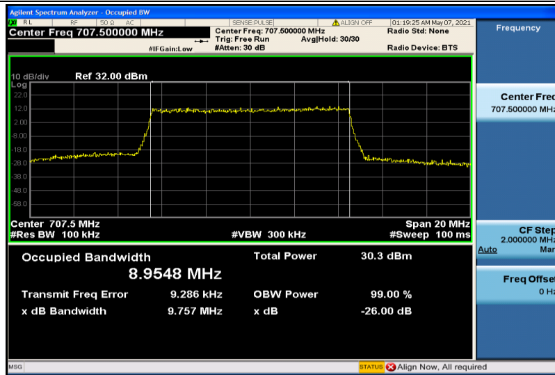
Band12-10MHz-16QAM-23095-50RB#0-8.9548
