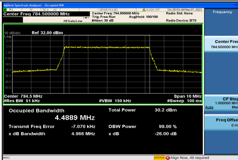
Band13-5MHz-16QAM-23255-25RB#0-4.4889
