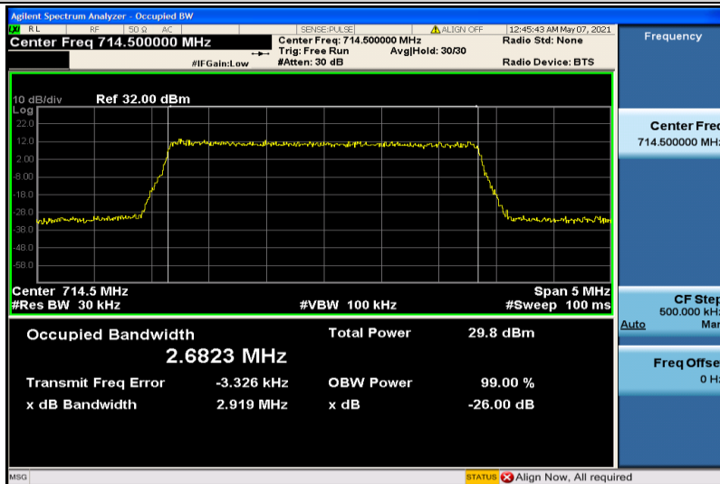
Band12-3MHz-16QAM-23165-15RB#0-2.6823
