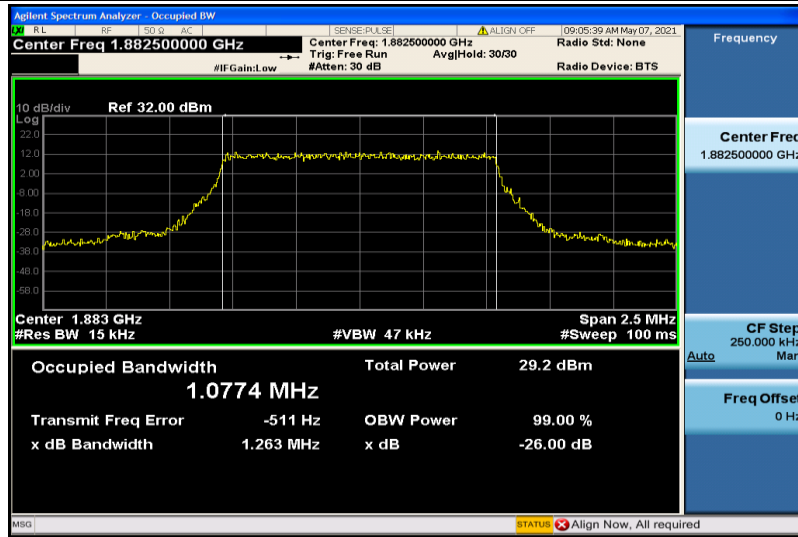
Band25-1.4MHz-QPSK-26365-6RB#0-1.0774
