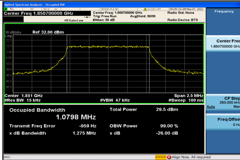
Band25-1.4MHz-QPSK-26047-6RB#0-1.0798
