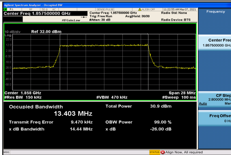
Band25-15MHz-QPSK-26115-75RB#0-13.403
