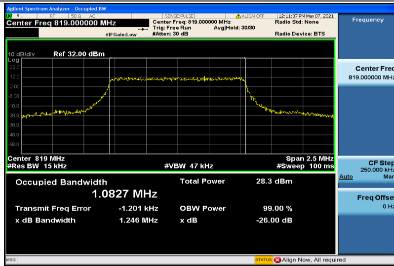
Band26-1.4MHz-16QAM-26740-6RB#0-1.0827
