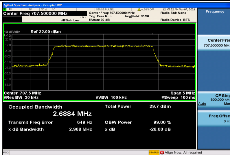
Band12-3MHz-16QAM-23095-15RB#0-2.6884
