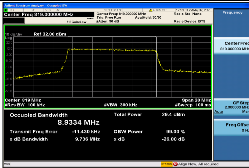
Band26-10MHz-16QAM-26740-50RB#0-8.9334
