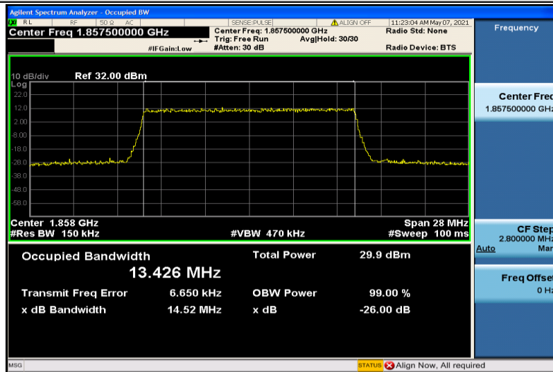
Band25-15MHz-16QAM-26115-75RB#0-13.426
