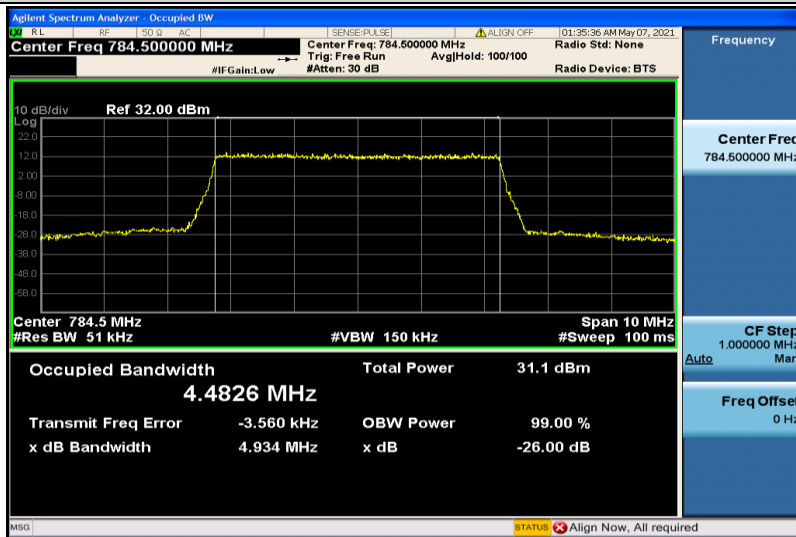
Band13-5MHz-QPSK-23255-25RB#0-4.4826
