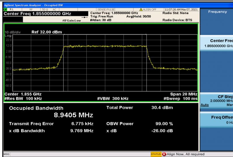
Band25-10MHz-QPSK-26090-50RB#0-8.9405
