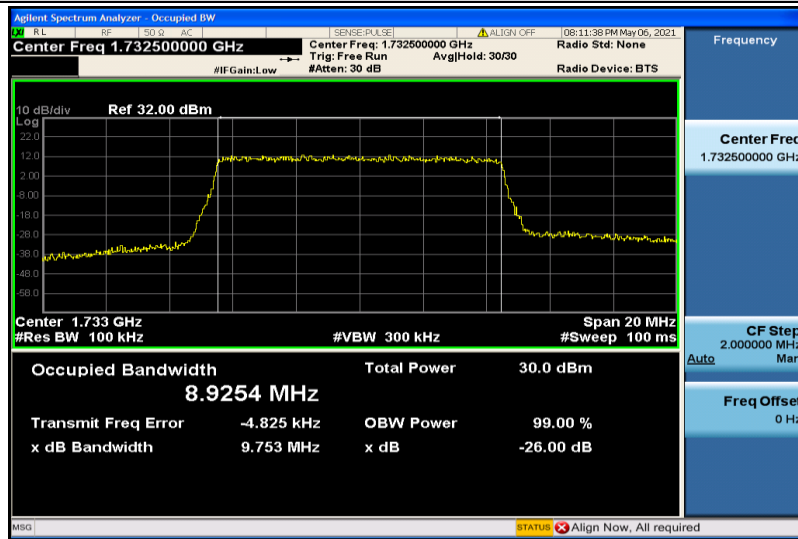
Band4-10MHz-16QAM-20175-50RB#0-8.9254
