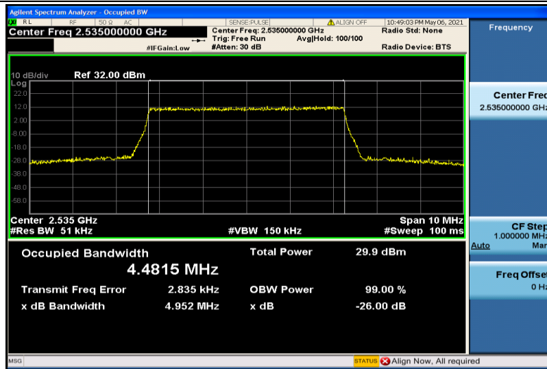
Band7-5MHz-16QAM-21100-25RB#0-4.4815
