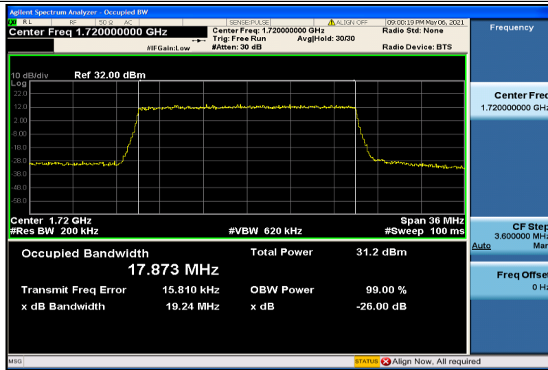
Band4-20MHz-QPSK-20050-100RB#0-17.873
