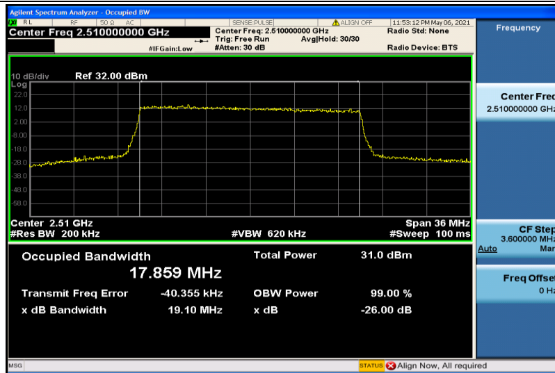
Band7-20MHz-QPSK-20850-100RB#0-17.859
