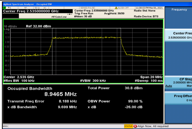
Band7-10MHz-QPSK-21100-50RB#0-8.9465
