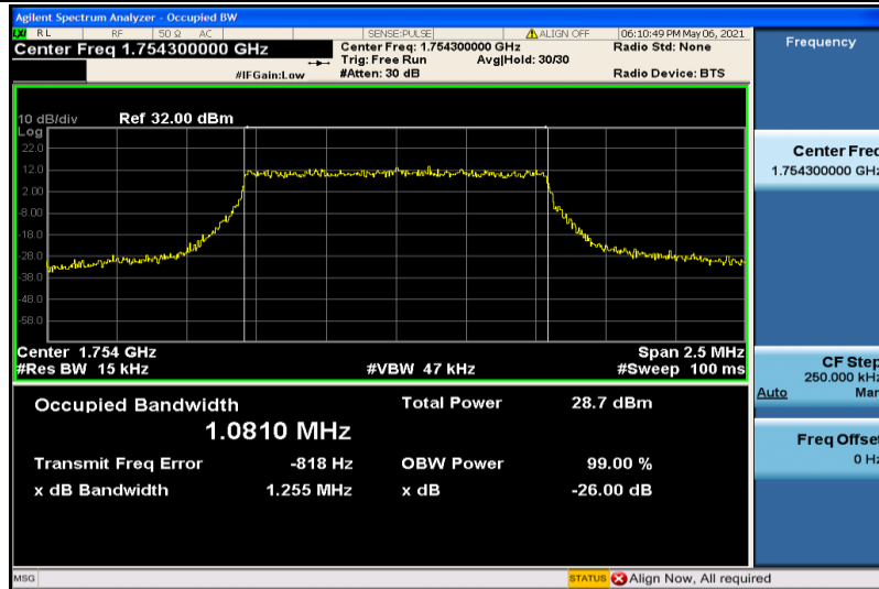
Band4-1.4MHz-16QAM-20393-6RB#0-1.0810
