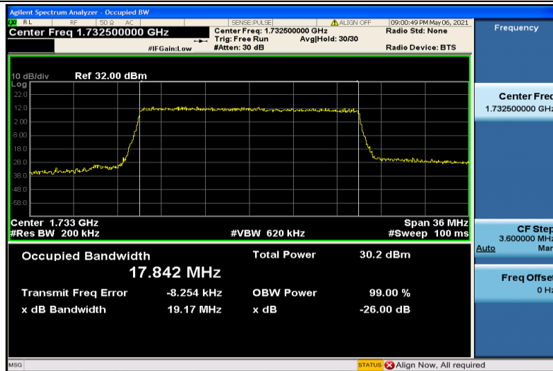
Band4-20MHz-16QAM-20175-100RB#0-17.842
