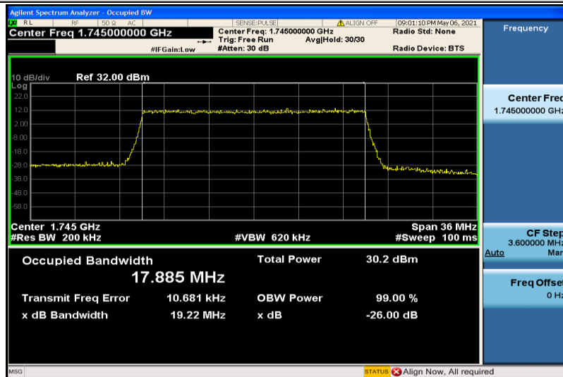
Band4-20MHz-16QAM-20300-100RB#0-17.885
