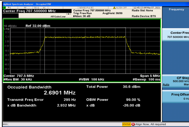
Band12-3MHz-QPSK-23095-15RB#0-2.6901
