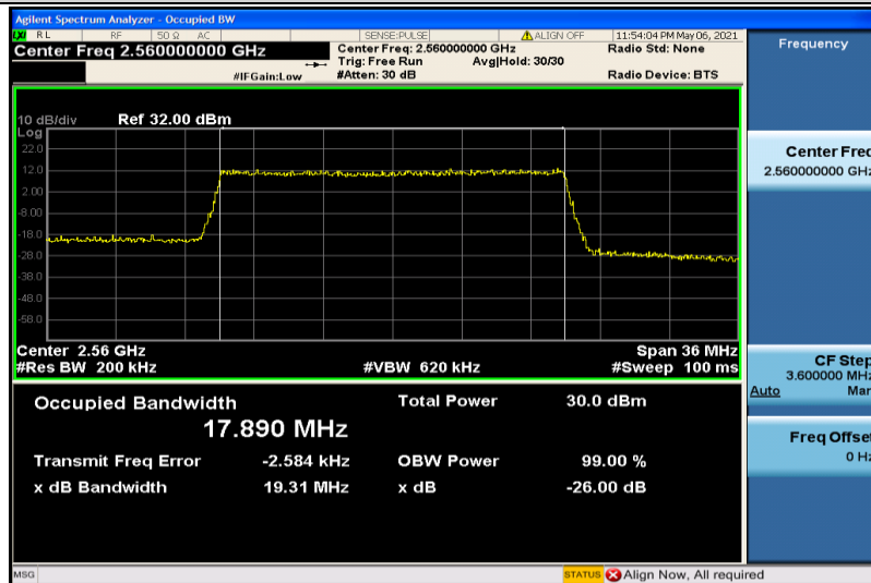
Band7-20MHz-16QAM-21350-100RB#0-17.890
