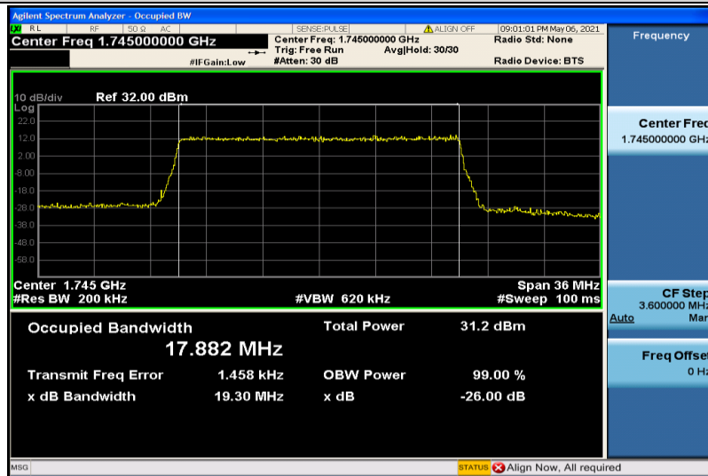
Band4-20MHz-QPSK-20300-100RB#0-17.882
