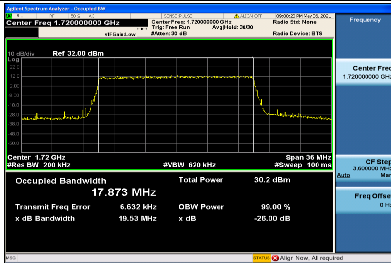
Band4-20MHz-16QAM-20050-100RB#0-17.873
