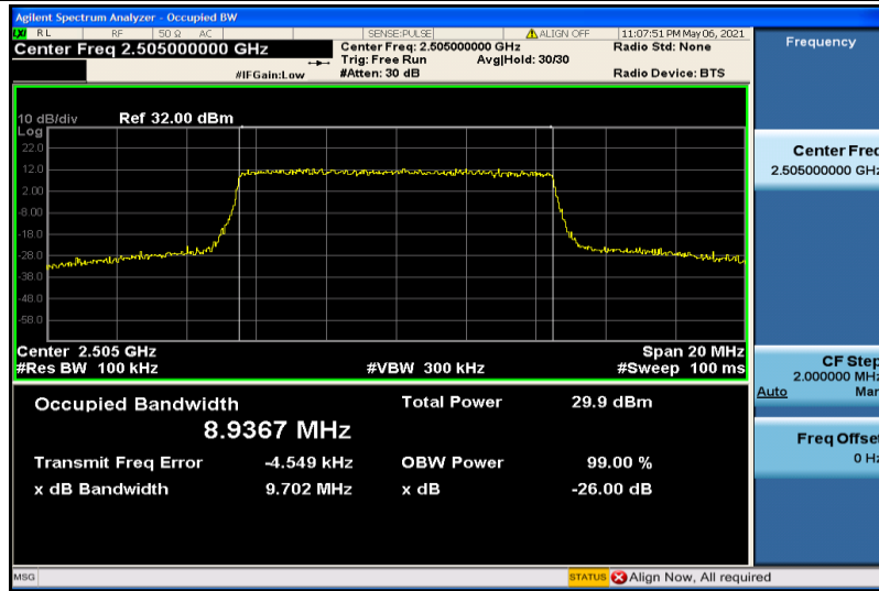
Band7-10MHz-16QAM-20800-50RB#0-8.9367
