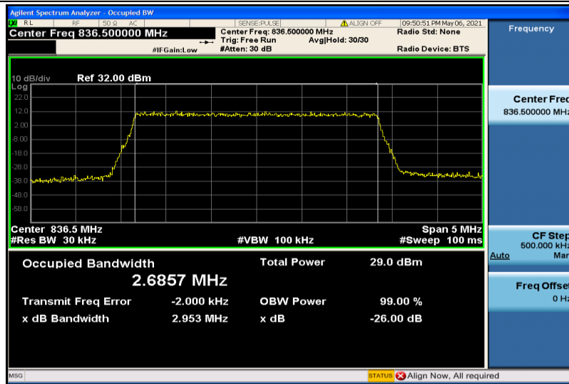
Band5-3MHz-16QAM-20525-15RB#0-2.6857
