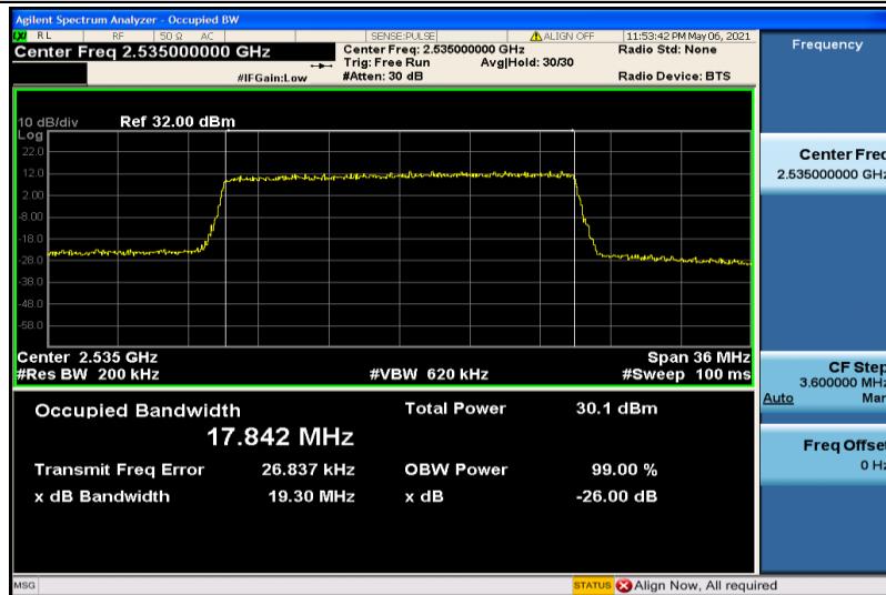
Band7-20MHz-16QAM-21100-100RB#0-17.842
