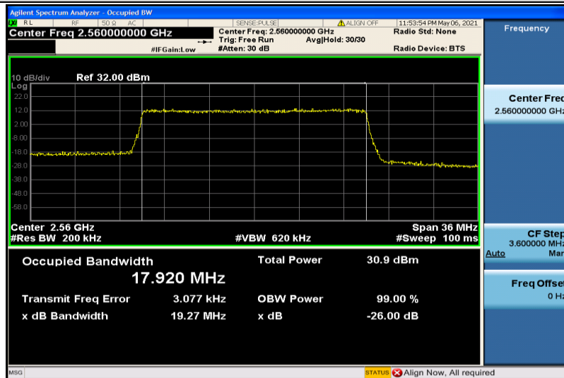
Band7-20MHz-QPSK-21350-100RB#0-17.920
