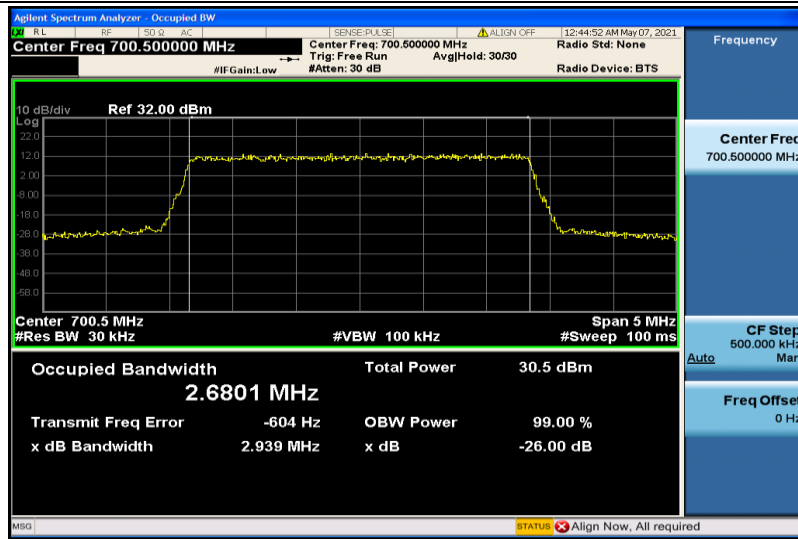
Band12-3MHz-QPSK-23025-15RB#0-2.6801
