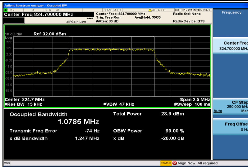
Band5-1.4MHz-16QAM-20407-6RB#0-1.0785
