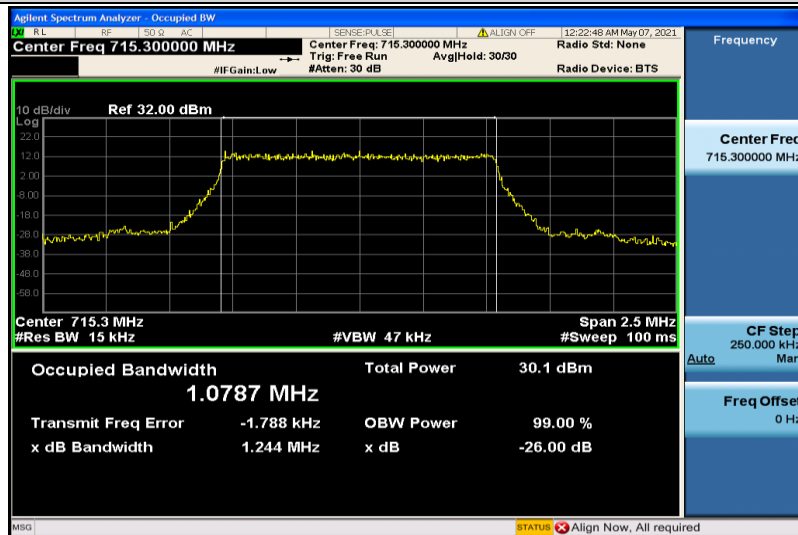
Band12-1.4MHz-QPSK-23173-6RB#0-1.0787
