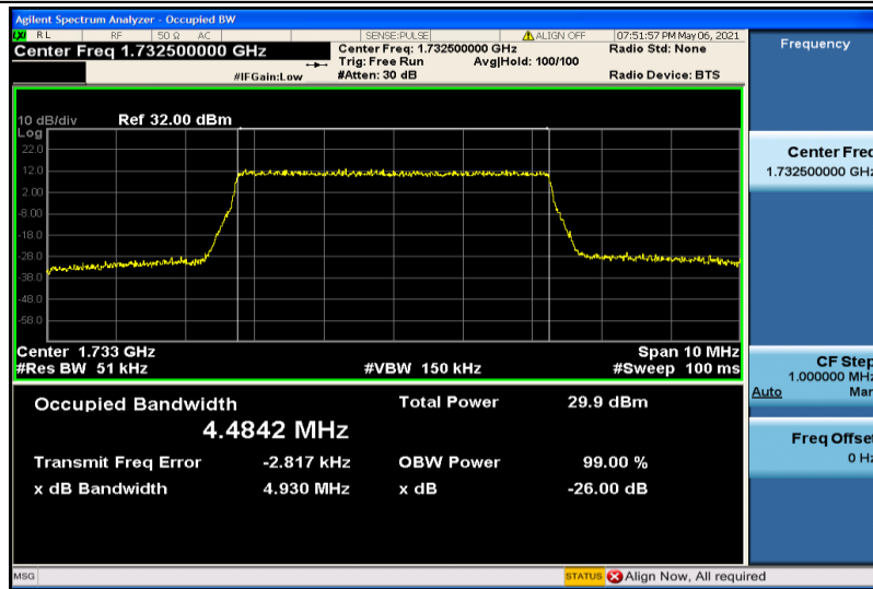
Band4-5MHz-16QAM-20175-25RB#0-4.4842
