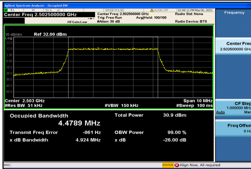
Band7-5MHz-QPSK-20775-25RB#0-4.4789
