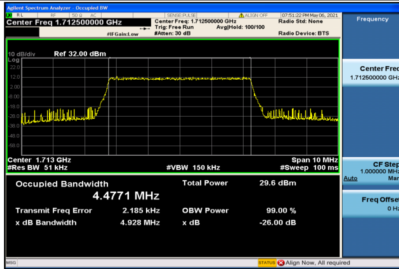
Band4-5MHz-16QAM-19975-25RB#0-4.4771
