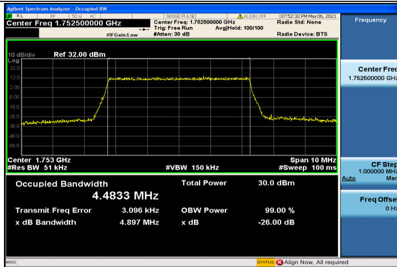
Band4-5MHz-16QAM-20375-25RB#0-4.4833
