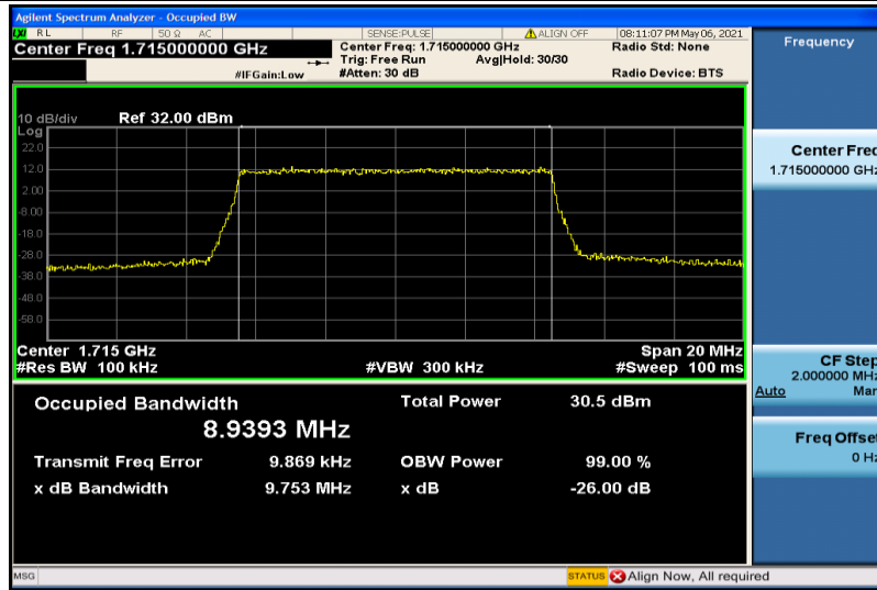
Band4-10MHz-QPSK-20000-50RB#0-8.9393
