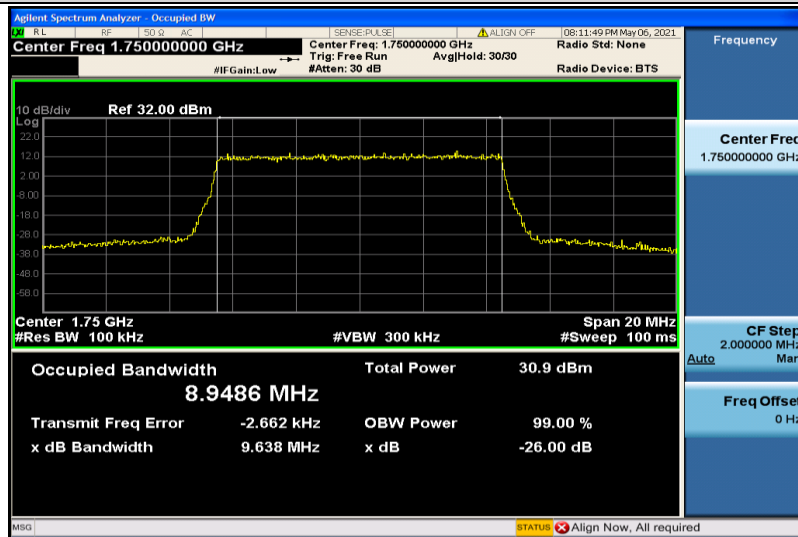
Band4-10MHz-QPSK-20350-50RB#0-8.9486
