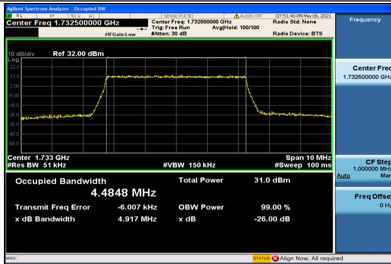
Band4-5MHz-QPSK-17325-25RB#0-4.4848
