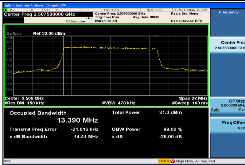
Band7-15MHz-QPSK-20825-75RB#0-13.390
