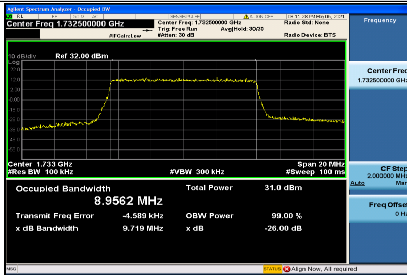
Band4-10MHz-QPSK-20175-50RB#0-8.9562
