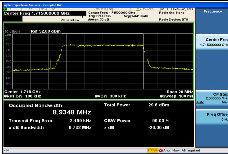
Band4-10MHz-16QAM-20000-50RB#0-8.9348
