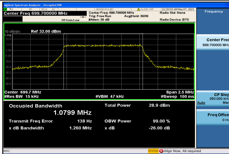
Band12-1.4MHz-16QAM-23017-6RB#0-1.0799
