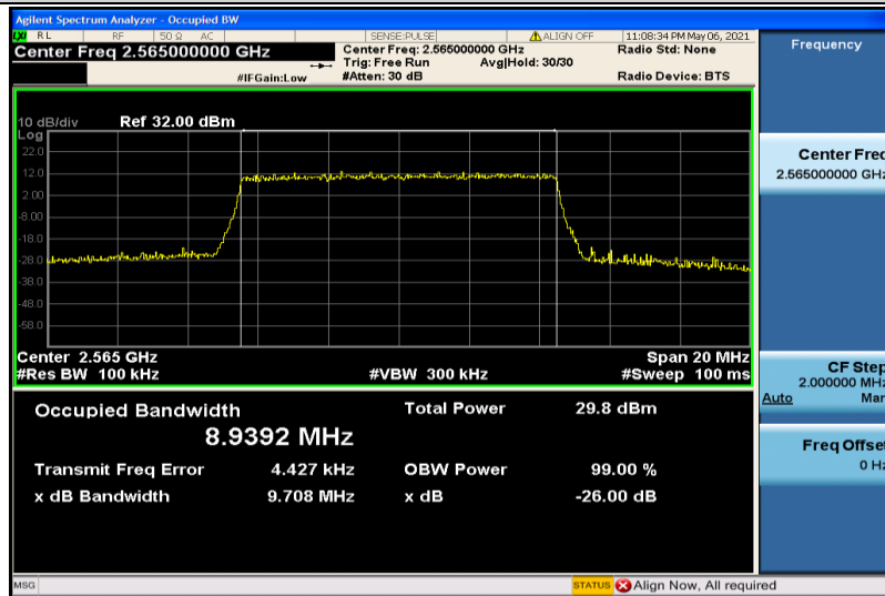
Band7-10MHz-16QAM-21400-50RB#0-8.9392
