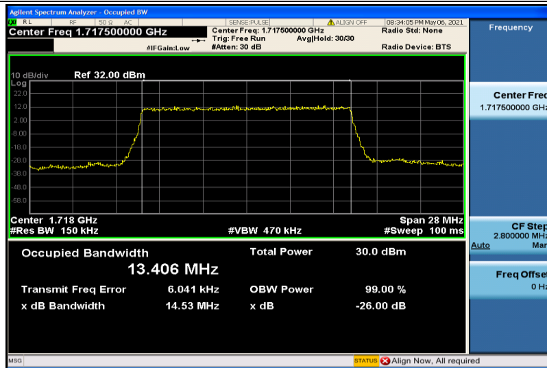
Band4-15MHz-16QAM-20025-75RB#0-13.406
