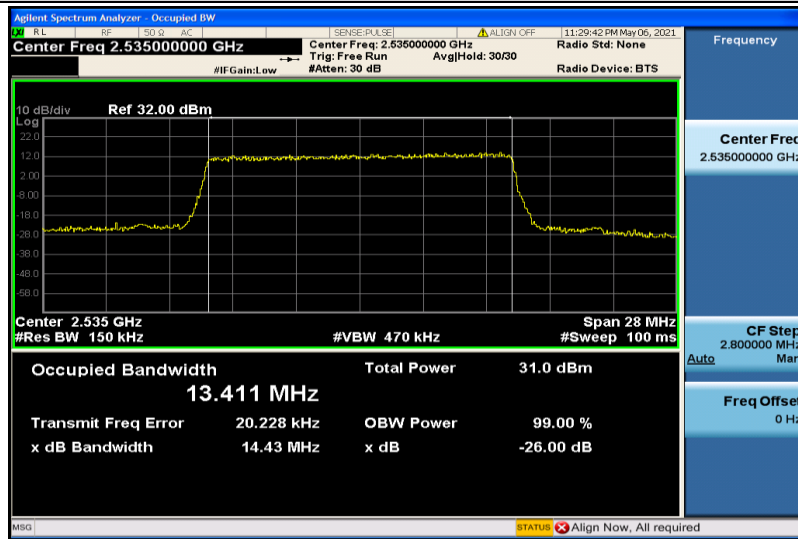
Band7-15MHz-QPSK-21100-75RB#0-13.411
