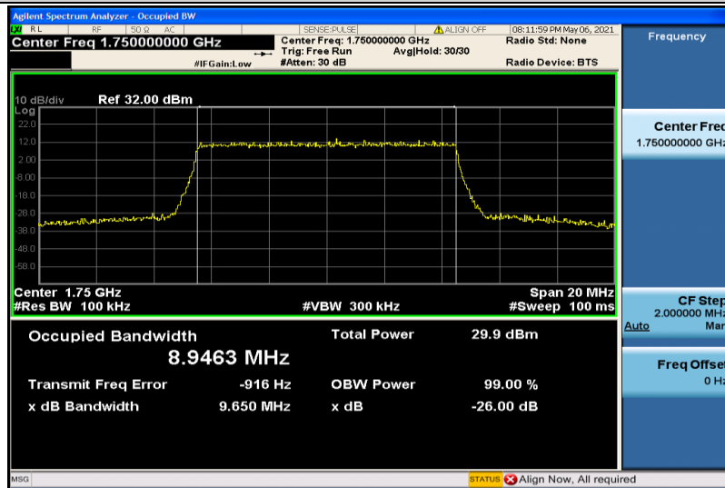
Band4-10MHz-16QAM-20350-50RB#0-8.9463
