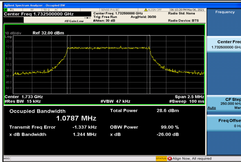
Band4-1.4MHz-16QAM-20175-6RB#0-1.0787
