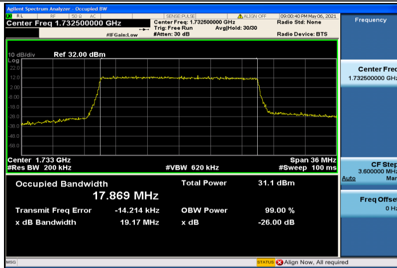
Band4-20MHz-QPSK-20175-100RB#0-17.869
