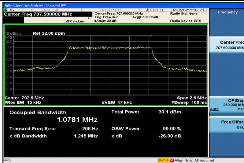
Band12-1.4MHz-QPSK-23095-6RB#0-1.0781
