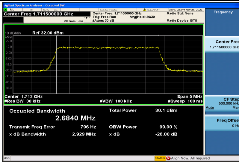
Band4-3MHz-QPSK-19965-15RB#0-2.6840
