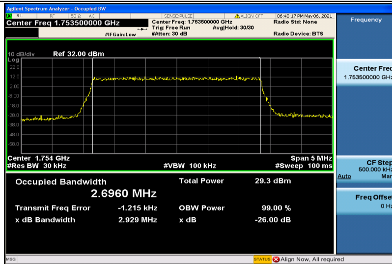
Band4-3MHz-16QAM-20385-15RB#0-2.6960
