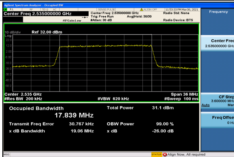
Band7-20MHz-QPSK-21100-100RB#0-17.839
