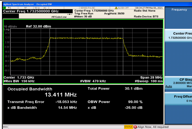
Band4-15MHz-16QAM-20175-75RB#0-13.411
