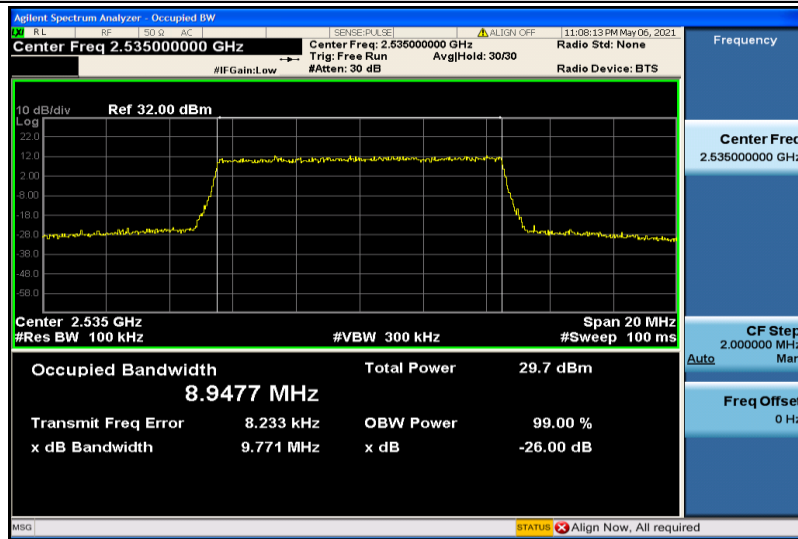
Band7-10MHz-16QAM-21100-50RB#0-8.9477
