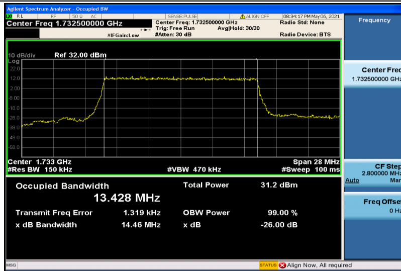
Band4-15MHz-QPSK-20175-75RB#0-13.428
