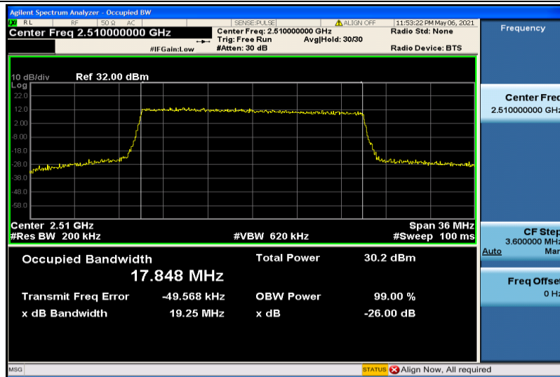
Band7-20MHz-16QAM-20850-100RB#0-17.848
