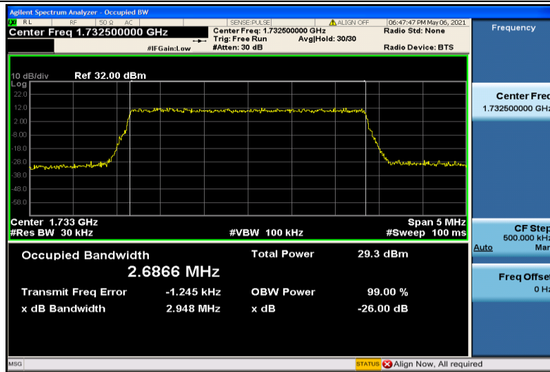
Band4-3MHz-QPSK-20175-15RB#0-2.6866
