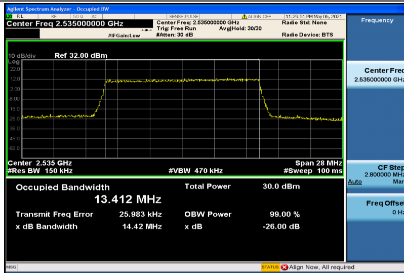
Band7-15MHz-16QAM-21100-75RB#0-13.412
