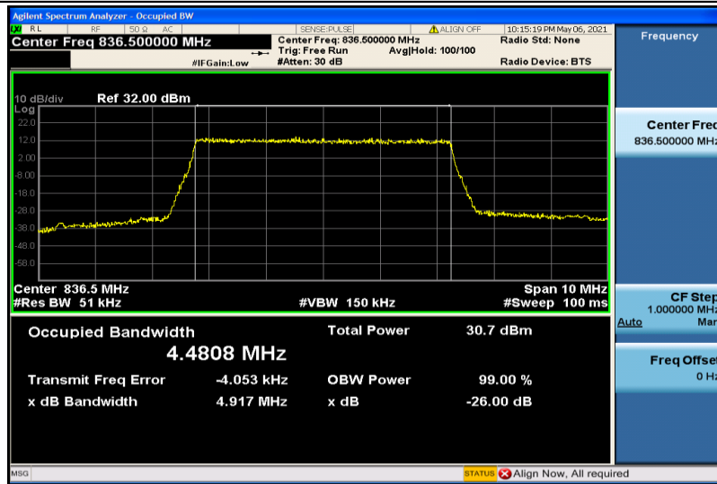
Band5-5MHz-QPSK-20525-25RB#0-4.4808
