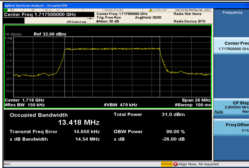
Band4-15MHz-QPSK-20025-75RB#0-13.418
