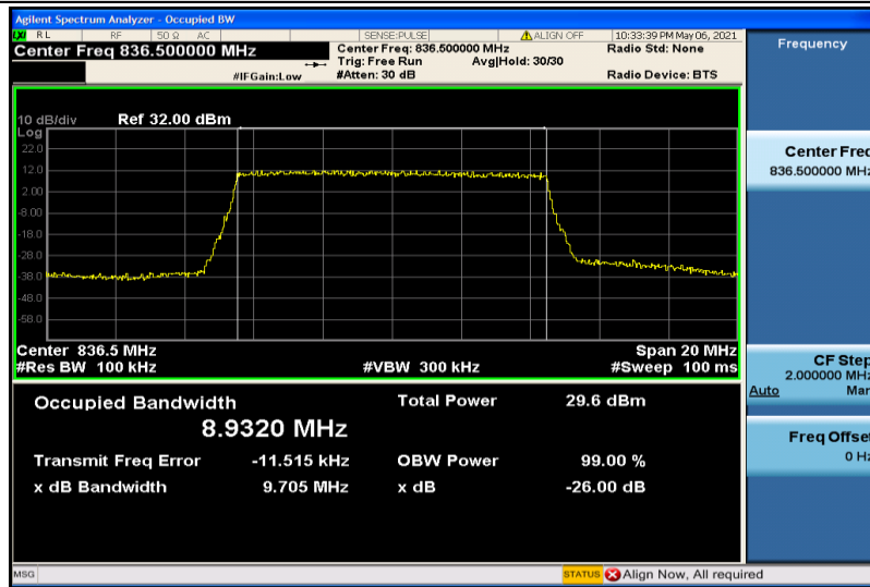
Band5-10MHz-16QAM-20525-50RB#0-8.9320
