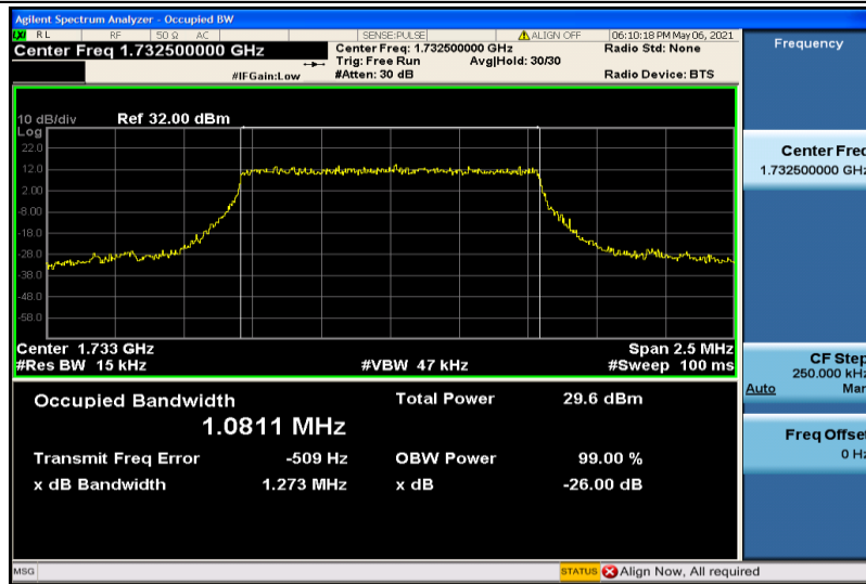
Band4-1.4MHz-QPSK-20175-6RB#0-1.0811
