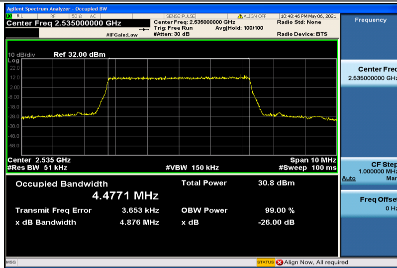
Band7-5MHz-QPSK-21100-25RB#0-4.4771
