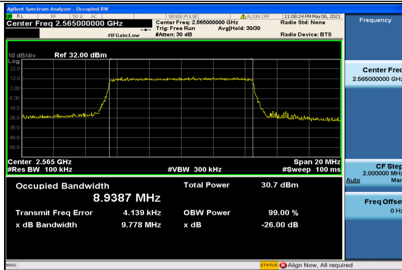
Band7-10MHz-QPSK-21400-50RB#0-8.9387
