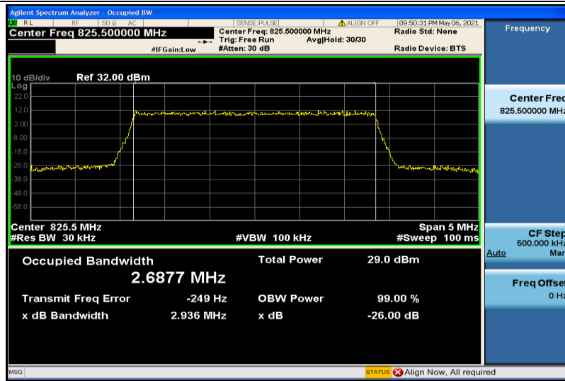
Band5-3MHz-16QAM-20415-15RB#0-2.6877
