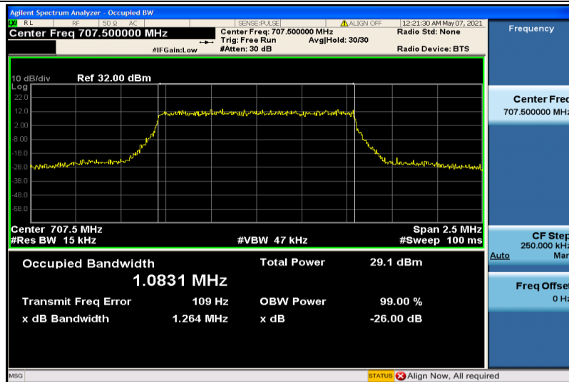
Band12-1.4MHz-16QAM-23095-6RB#0-1.0831
