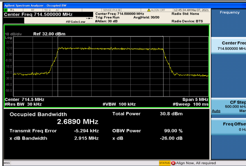
Band12-3MHz-QPSK-23165-15RB#0-2.6890
