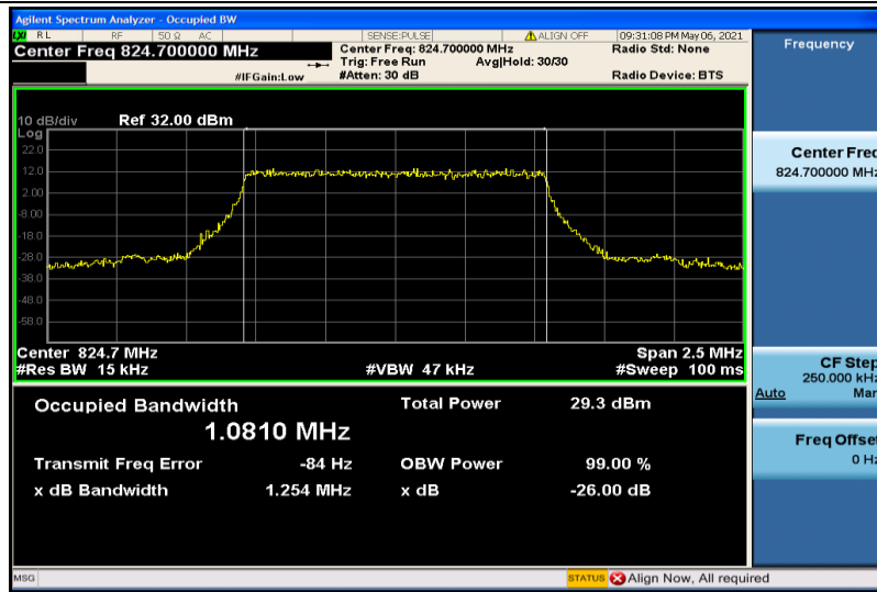
Band5-1.4MHz-QPSK-20407-6RB#0-1.0810
