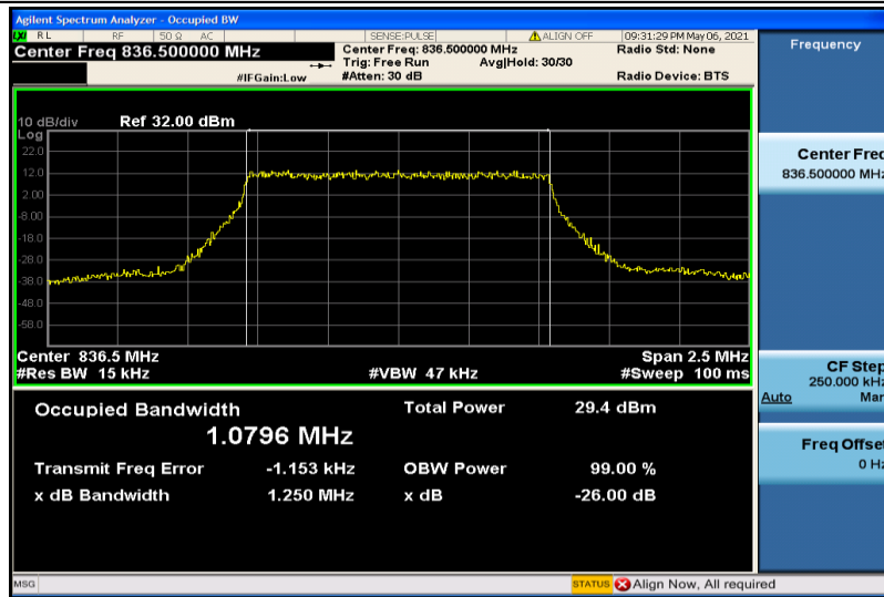
Band5-1.4MHz-QPSK-20525-6RB#0-1.0796
