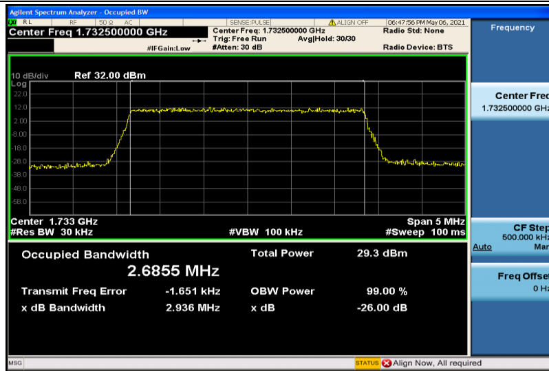
Band4-3MHz-16QAM-20175-15RB#0-2.6855
