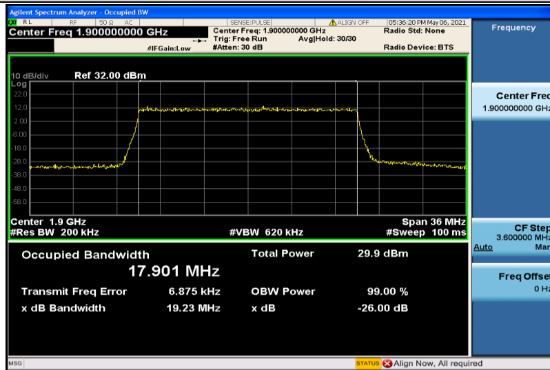
Band2-20MHz-16QAM-19000-100RB#0-17.901
