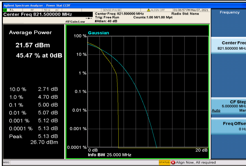
Band26-15MHz-16QAM-26765-1RB#0
