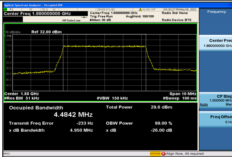
Band2-5MHz-16QAM-18900-25RB#0-4.4842
