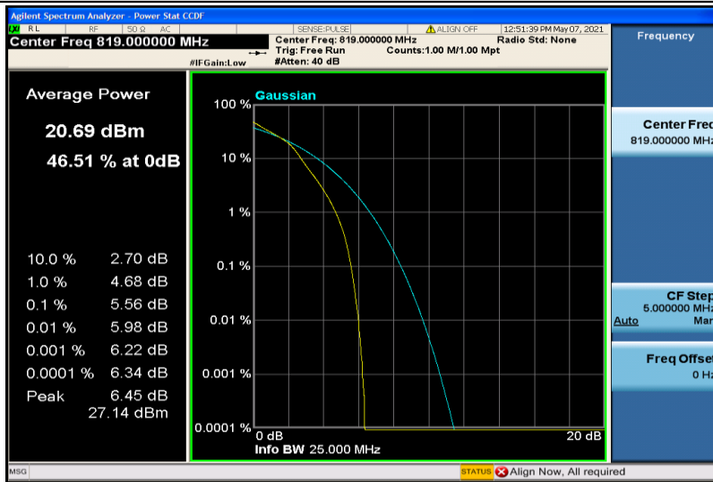
Band26-5MHz-16QAM-26740-25RB#0
