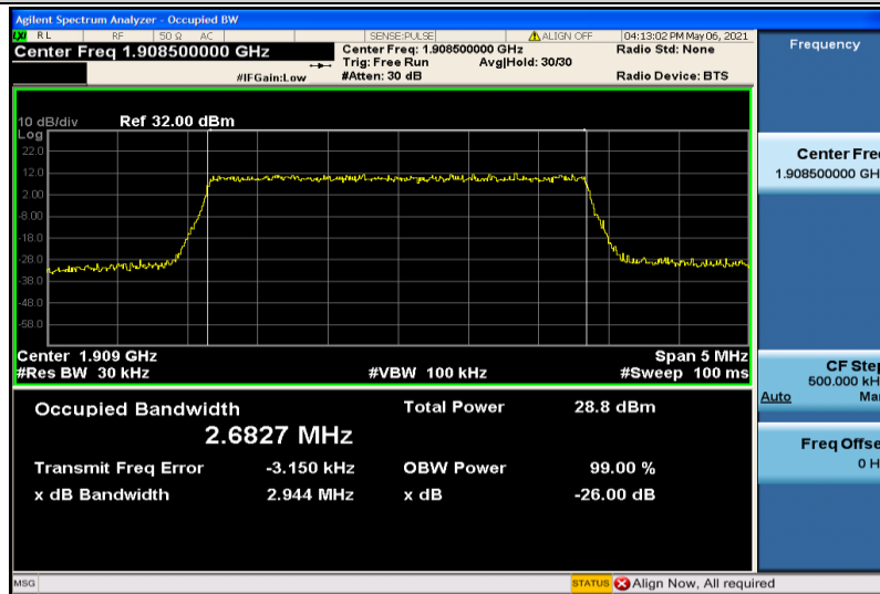
Band2-3MHz-16QAM-19185-15RB#0-2.6827
