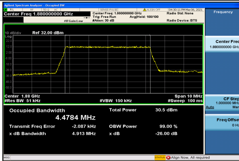
Band2-5MHz-QPSK-18900-25RB#0-4.4784
