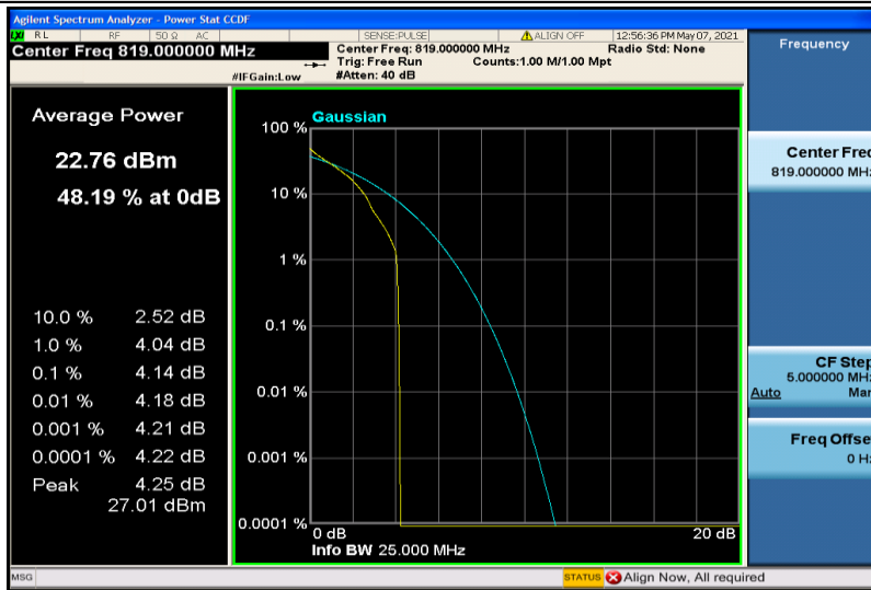
Band26-10MHz-QPSK-26740-1RB#0
