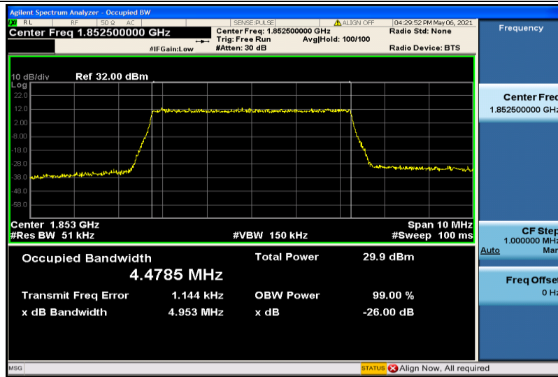
Band2-5MHz-16QAM-18625-25RB#0-4.4785
