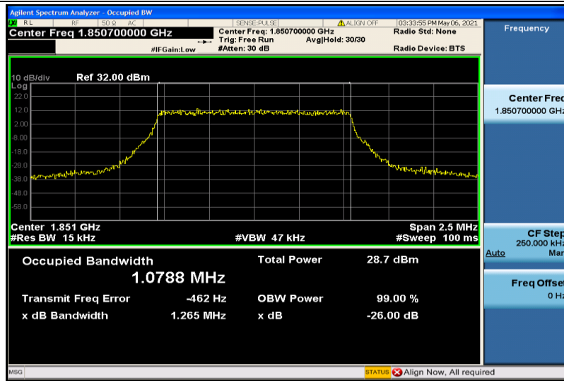
Band2-1.4MHz-16QAM-18607-6RB#0-1.0788
