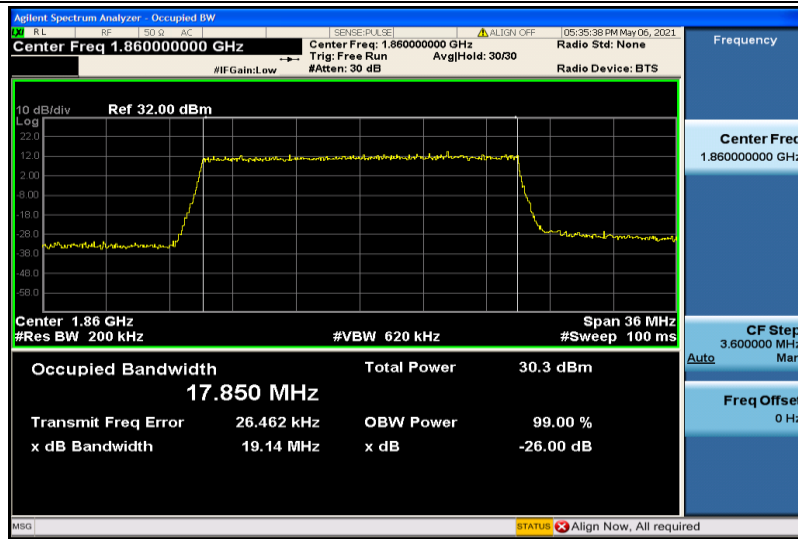
Band2-20MHz-16QAM-18600-100RB#0-17.850
