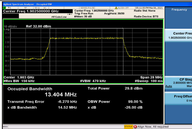
Band2-15MHz-16QAM-19125-75RB#0-13.404
