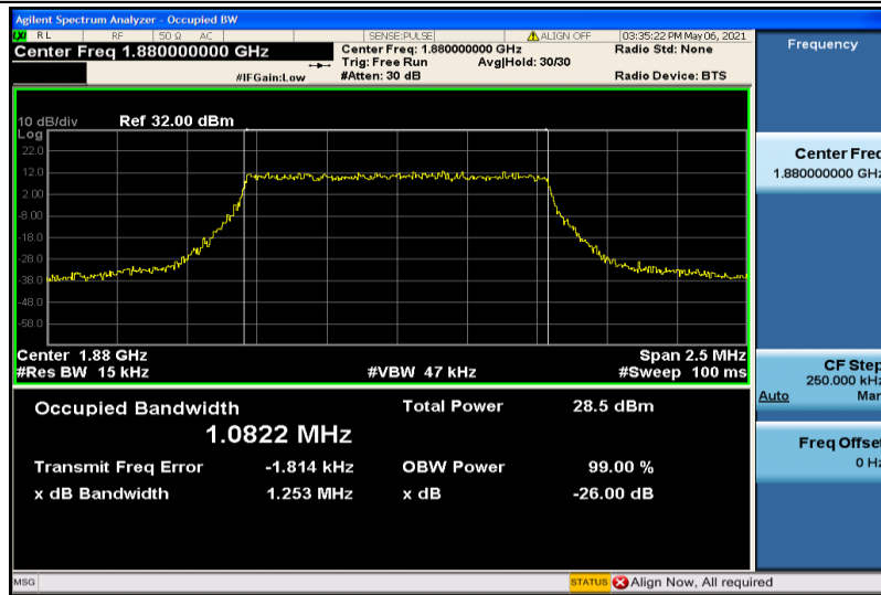
Band2-1.4MHz-16QAM-18900-6RB#0-1.0822
