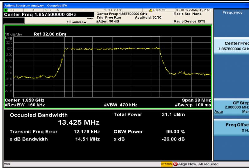
Band2-15MHz-QPSK-18675-75RB#0-13.425
