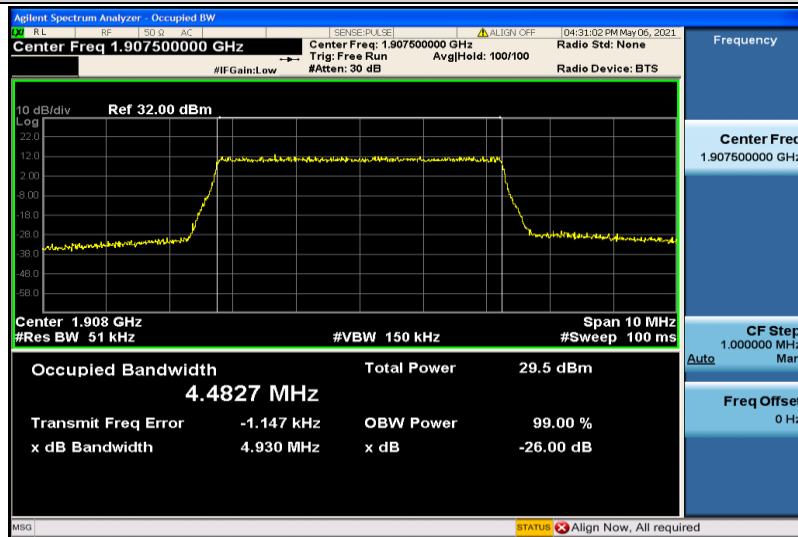
Band2-5MHz-16QAM-19175-25RB#0-4.4827
