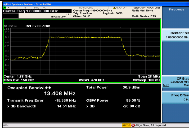
Band2-15MHz-QPSK-18900-75RB#0-13.406
