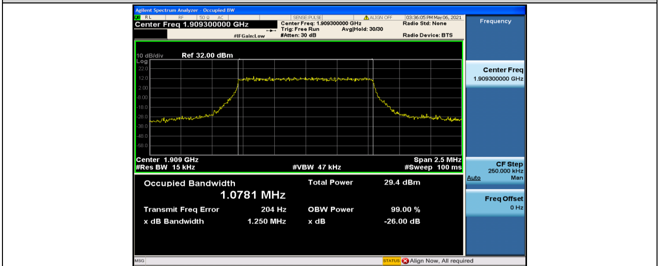
Band2-1.4MHz-QPSK-19193-6RB#0-1.0781
