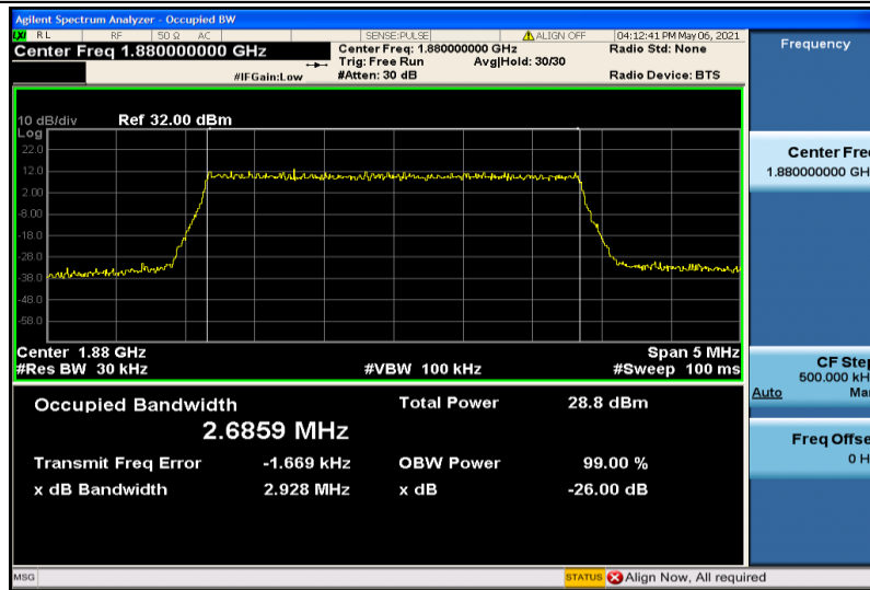
Band2-3MHz-16QAM-18900-15RB#0-2.6859
