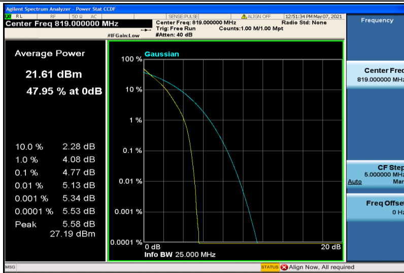
Band26-5MHz-QPSK-26740-25RB#0
