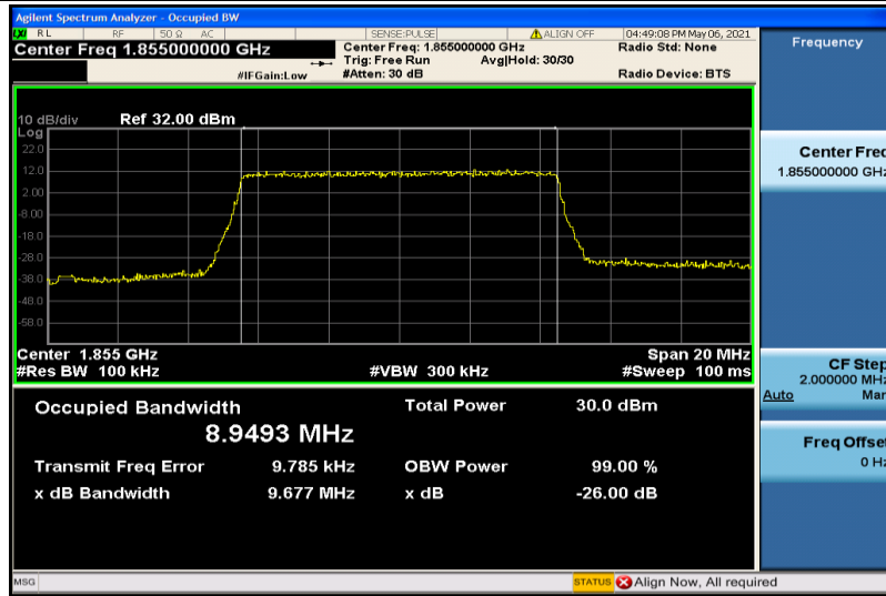
Band2-10MHz-16QAM-18650-50RB#0-8.9493
