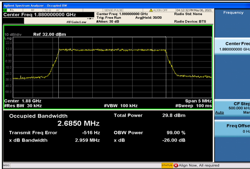
Band2-3MHz-QPSK-18900-15RB#0-2.6850
