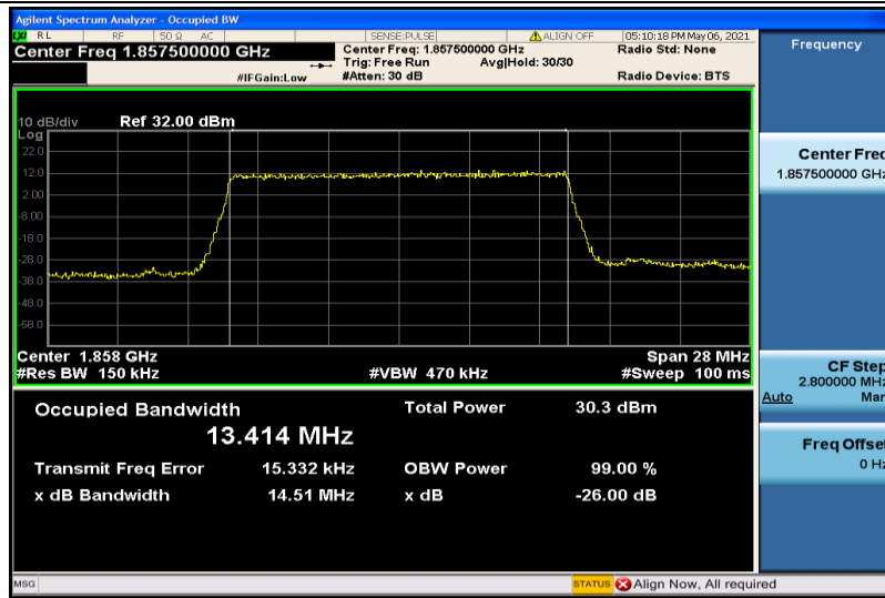
Band2-15MHz-16QAM-18675-75RB#0-13.414
