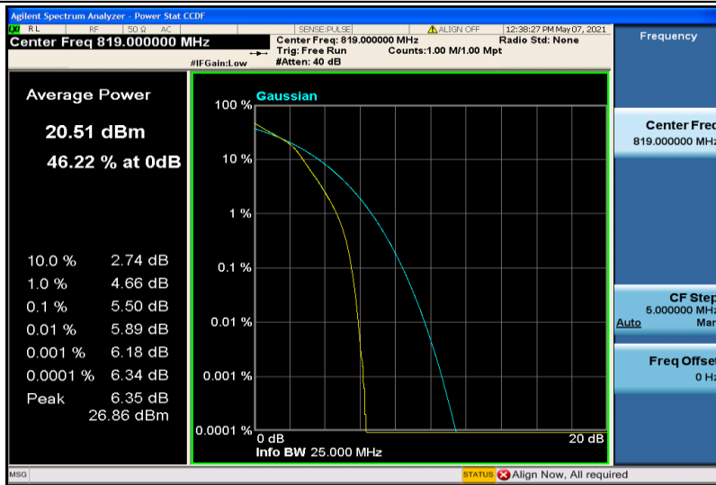
Band26-3MHz-16QAM-26740-15RB#0
