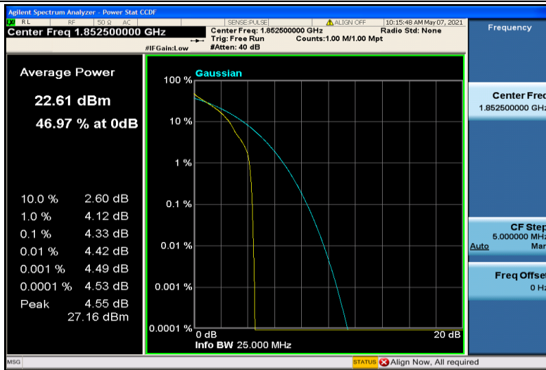
Band25-5MHz-QPSK-26065-1RB#0
