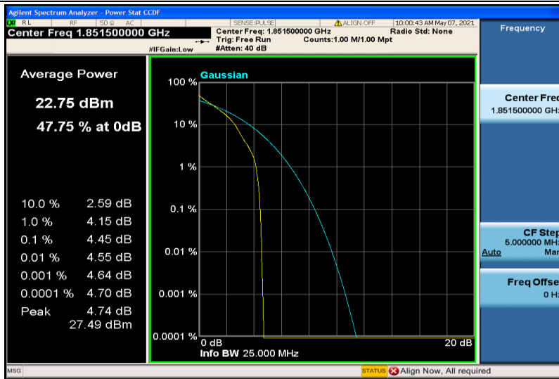
Band25-3MHz-QPSK-26055-1RB#0
