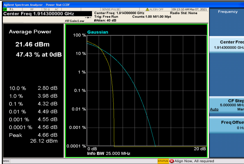
Band25-1.4MHz-16QAM-26683-1RB#0
