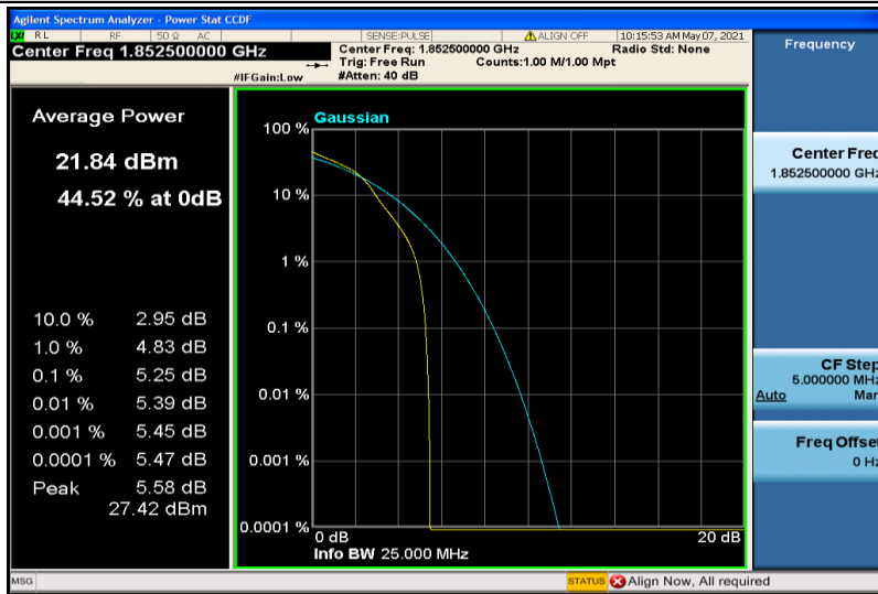
Band25-5MHz-16QAM-26065-1RB#0
