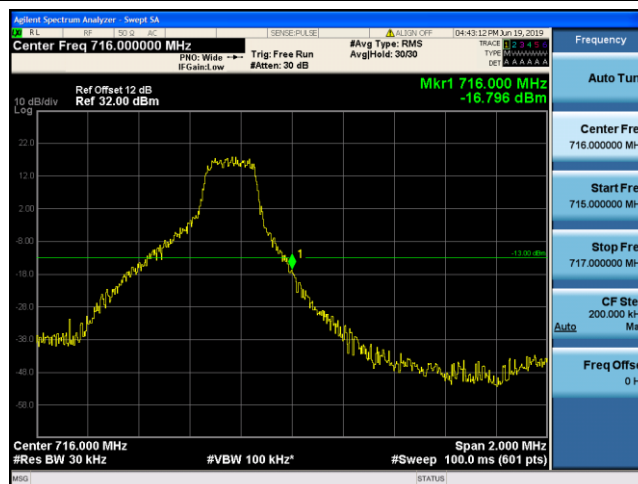
Band12_3MHz_16QAM_23165_1RB#14
