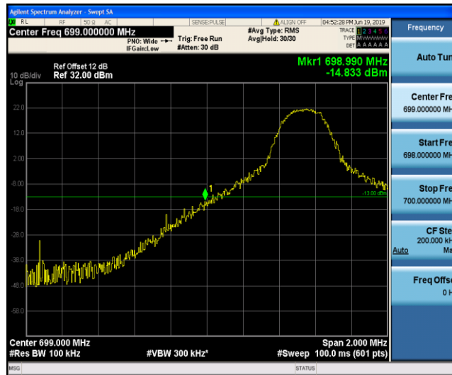
Band12_5MHz_23035_1RB#0
