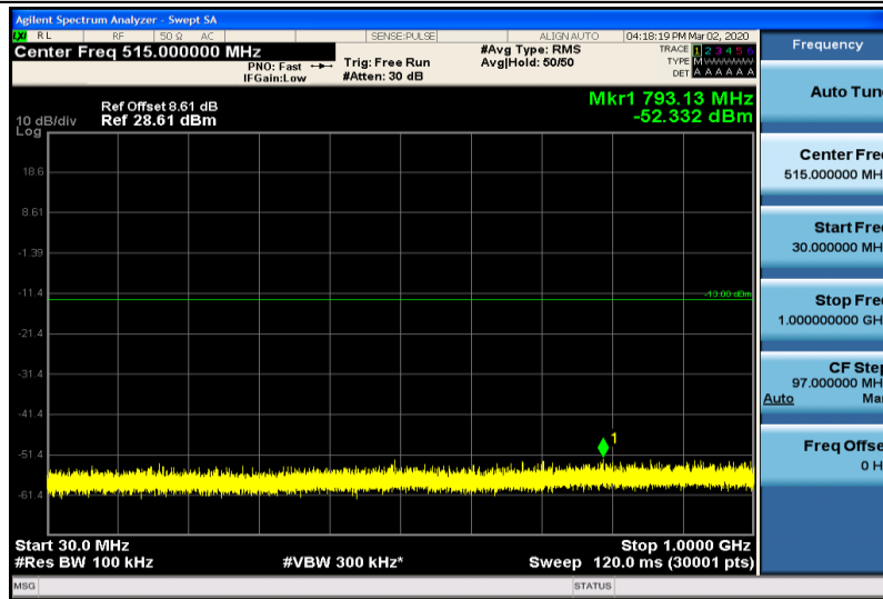
Band4-3MHz-16QAM-19965-1RB#0-30~1000MHz
