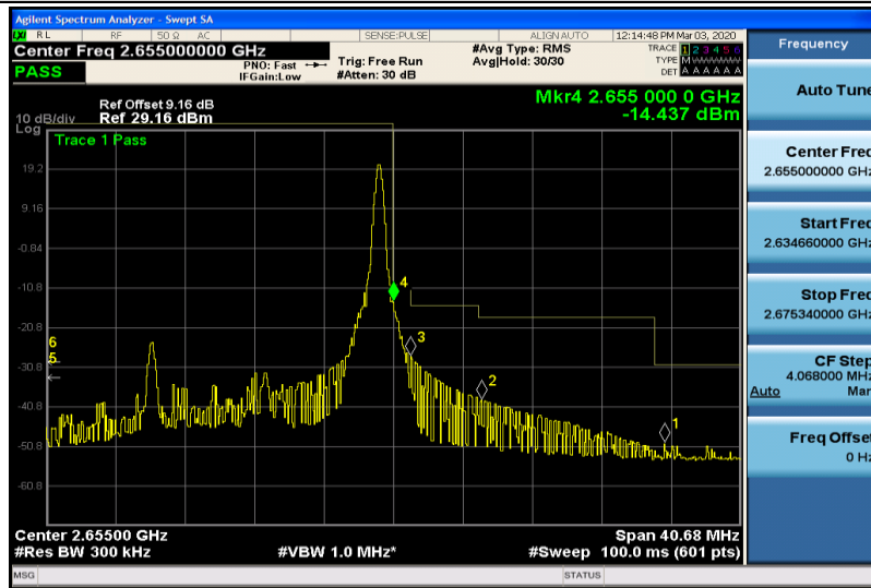
Band41-15MHz-16QAM-41165-1RB#74
