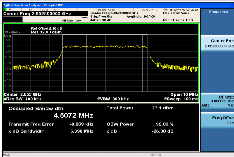
Band41-5MHz-16QAM-41215-25RB#0-4.5072
