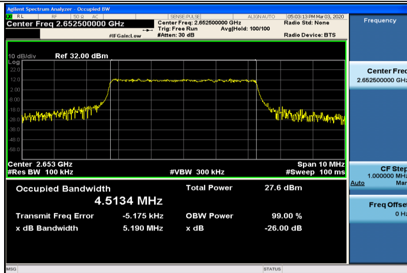
Band41-5MHz-QPSK-41215-25RB#0-4.5134
