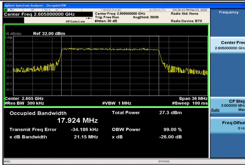
Band41-20MHz-16QAM-40740-100RB#0-17.924
