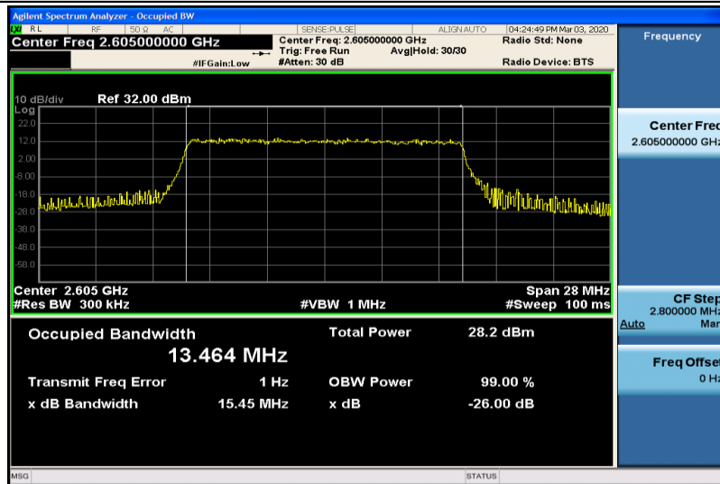
Band41-15MHz-QPSK-40740-75RB#0-13.464
