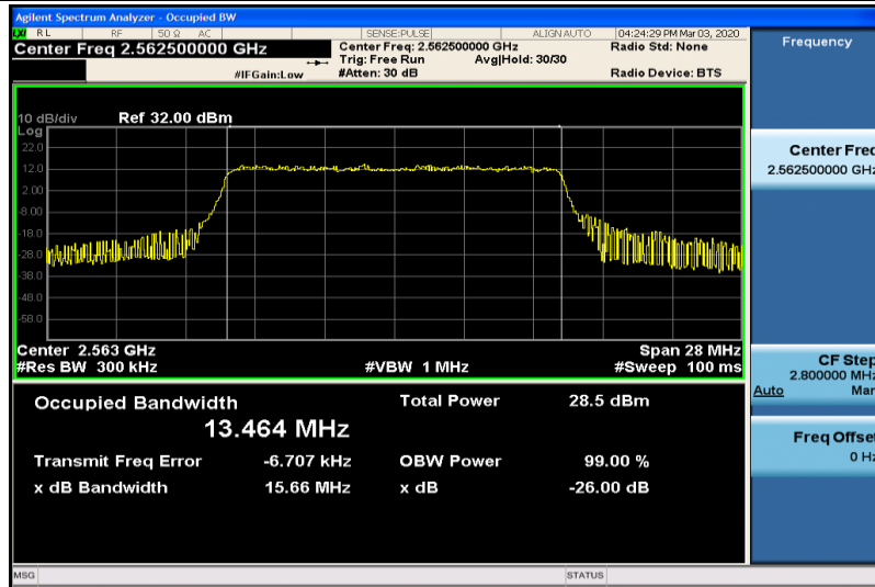
Band41-15MHz-QPSK-40315-75RB#0-13.464
