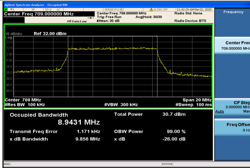
Band17-10MHz-QPSK-23780-50RB#0-8.9431
