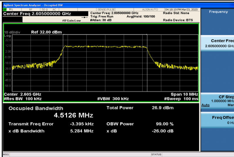
Band41-5MHz-16QAM-40740-25RB#0-4.5126
