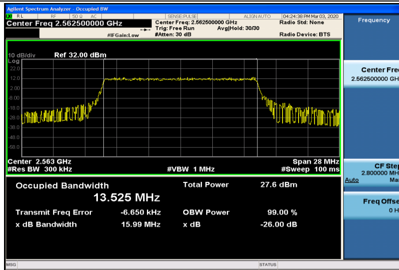
Band41-15MHz-16QAM-40315-75RB#0-13.525
