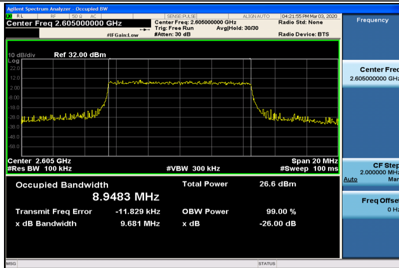
Band41-10MHz-16QAM-40740-50RB#0-8.9483
