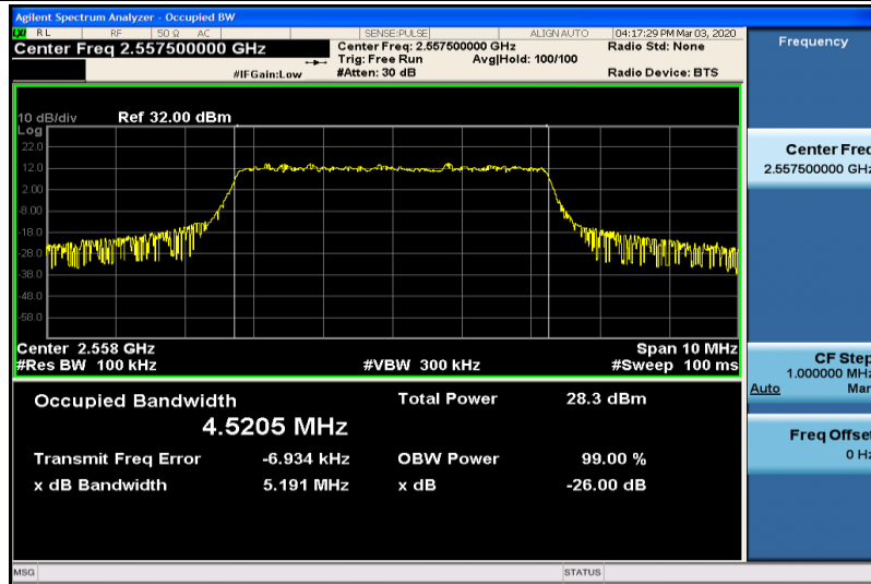
Band41-5MHz-QPSK-40265-25RB#0-4.5205
