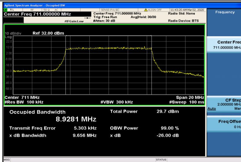
Band17-10MHz-16QAM-23800-50RB#0-8.9281
