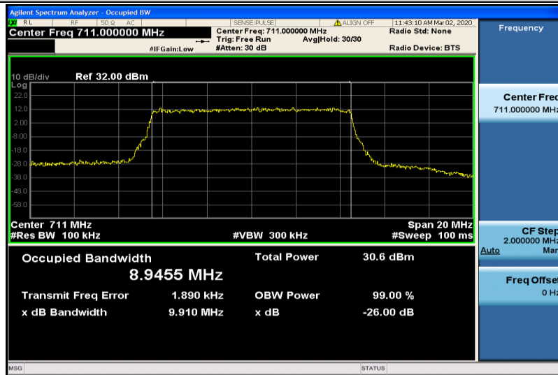
Band17-10MHz-QPSK-23800-50RB#0-8.9455
