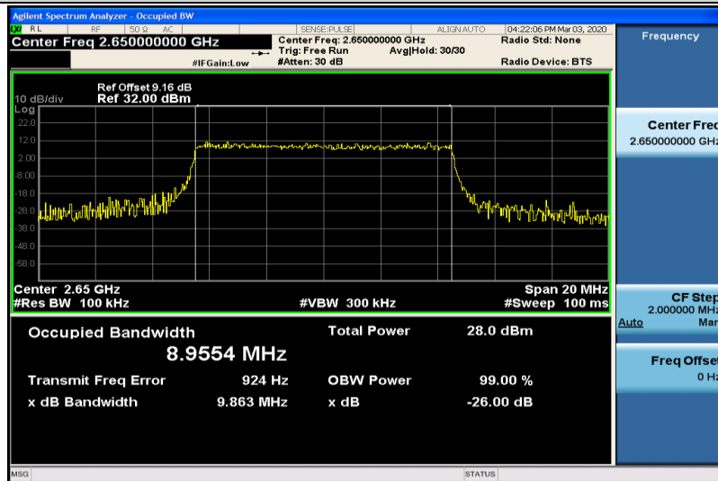
Band41-10MHz-QPSK-41190-50RB#0-8.9554
