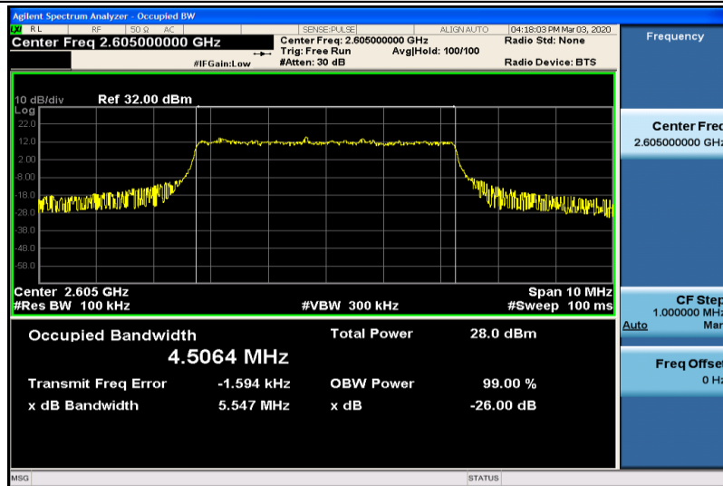
Band41-5MHz-QPSK-40740-25RB#0-4.5064
