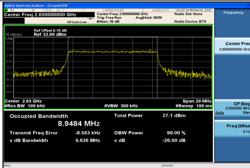
Band41-10MHz-16QAM-41190-50RB#0-8.9484
