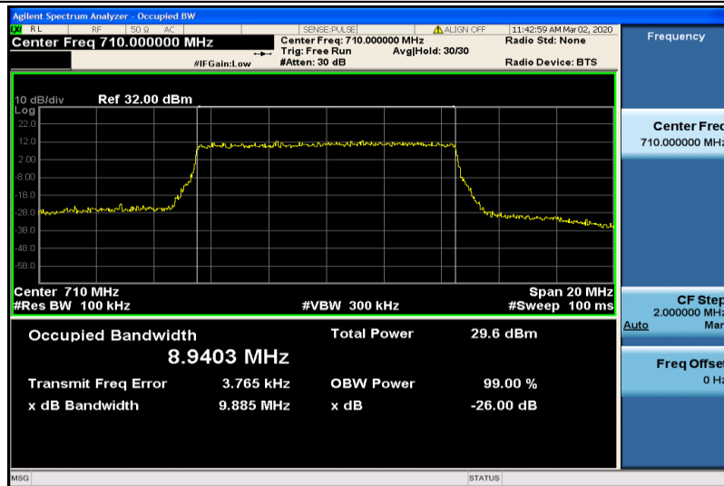
Band17-10MHz-16QAM-23790-50RB#0-8.9403
