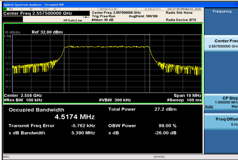
Band41-5MHz-16QAM-40265-25RB#0-4.5174
