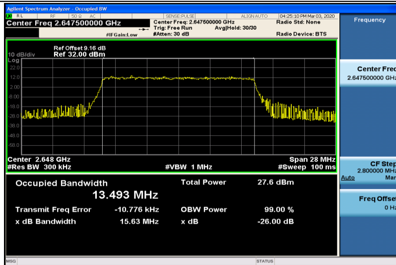
Band41-15MHz-QPSK-41165-75RB#0-13.493
