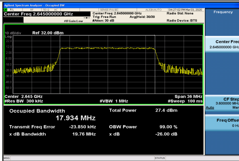
Band41-20MHz-16QAM-41140-100RB#0-17.934
