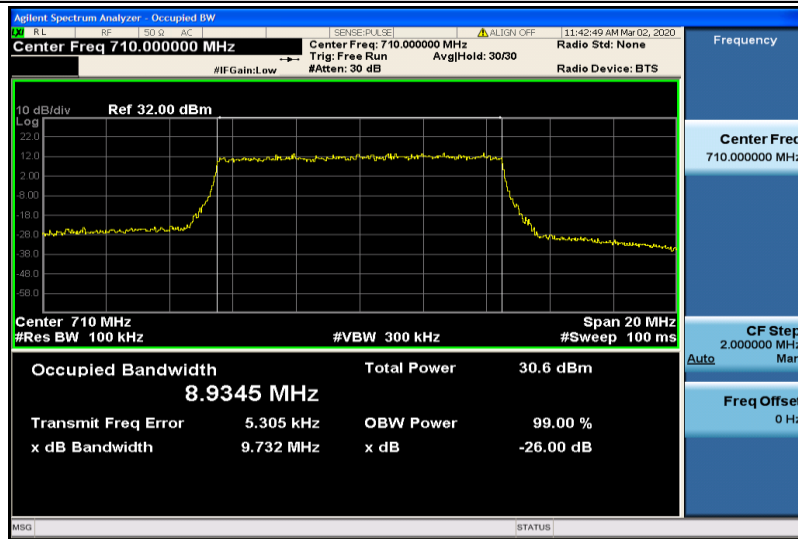
Band17-10MHz-QPSK-23790-50RB#0-8.9345
