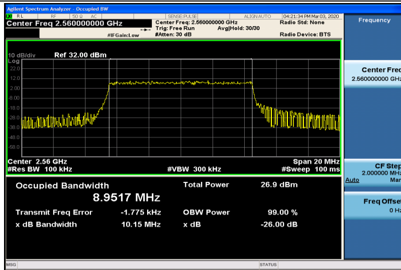
Band41-10MHz-16QAM-40290-50RB#0-8.9517
