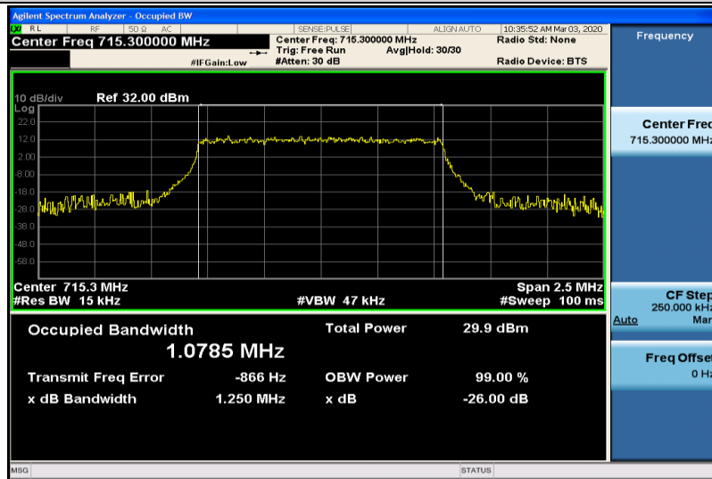
Band12-1.4MHz-QPSK-23173-6RB#0-1.0785
