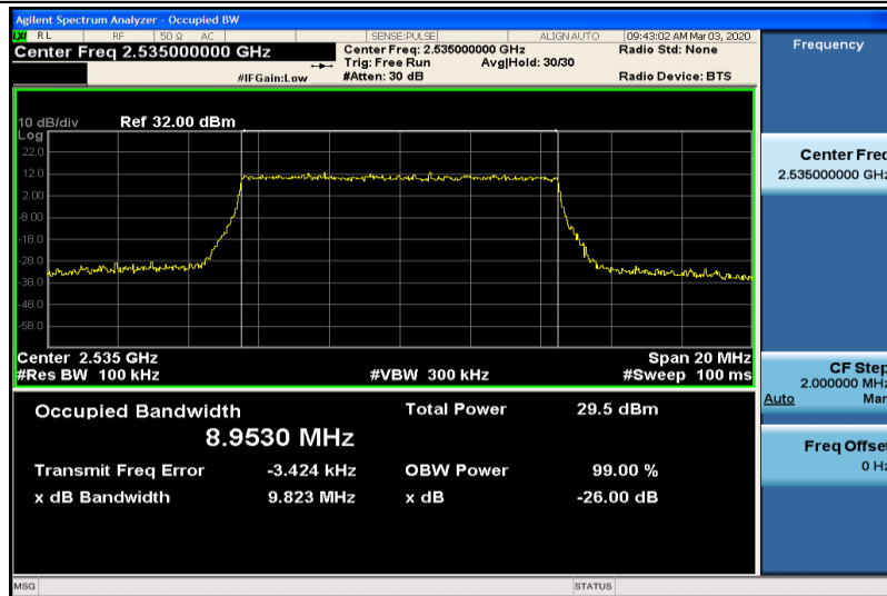
Band7-10MHz-QPSK-21100-50RB#0-8.9530
