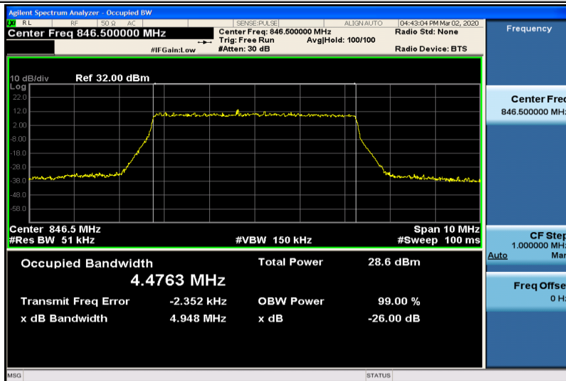
Band5-5MHz-16QAM-20625-25RB#0-4.4763
