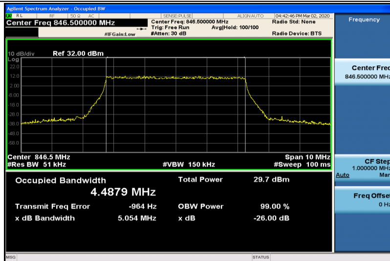
Band5-5MHz-QPSK-20625-25RB#0-4.4879
