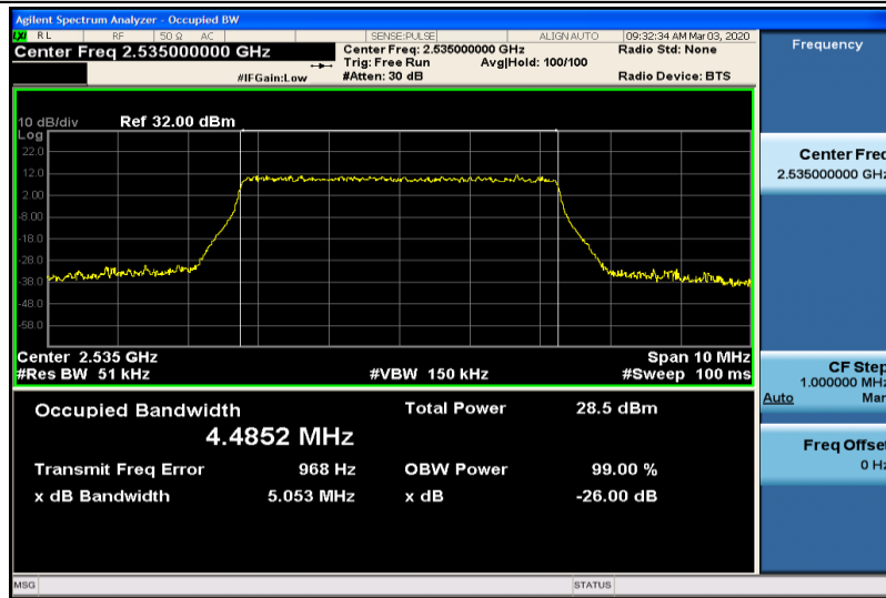
Band7-5MHz-16QAM-21100-25RB#0-4.4852
