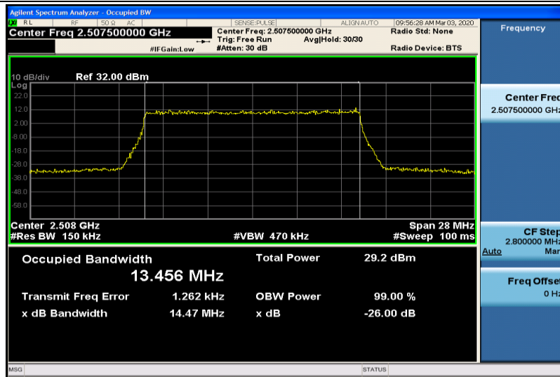
Band7-15MHz-16QAM-20825-75RB#0-13.456
