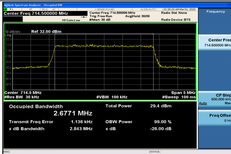
Band12-3MHz-16QAM-23165-15RB#0-2.6771
