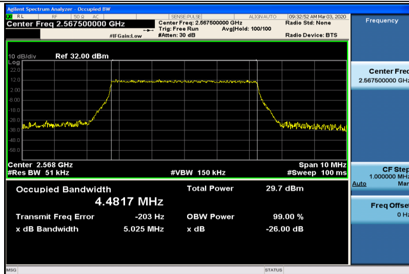
Band7-5MHz-QPSK-21425-25RB#0-4.4817
