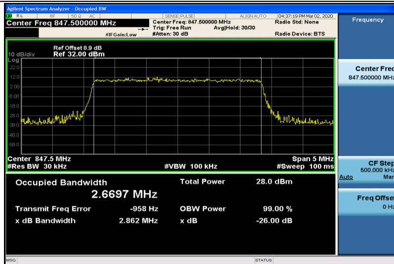
Band5-3MHz-16QAM-20635-15RB#0-2.6697
