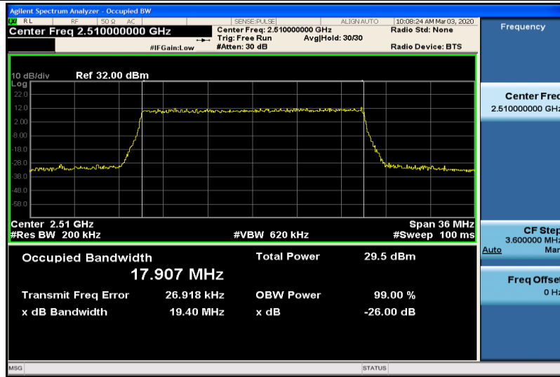
Band7-20MHz-16QAM-20850-100RB#0-17.907
