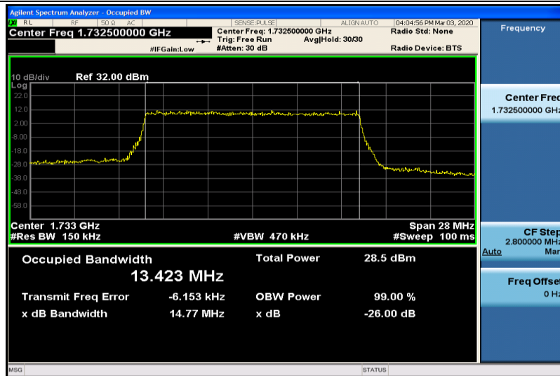
Band4-15MHz-16QAM-20175-75RB#0-13.423
