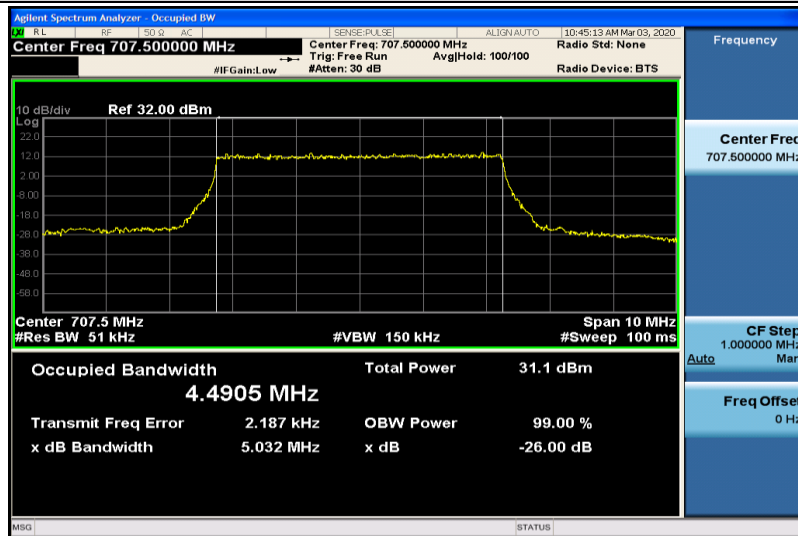
Band12-5MHz-QPSK-23095-25RB#0-4.4905
