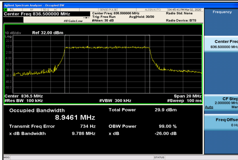
Band5-10MHz-QPSK-20525-50RB#0-8.9461
