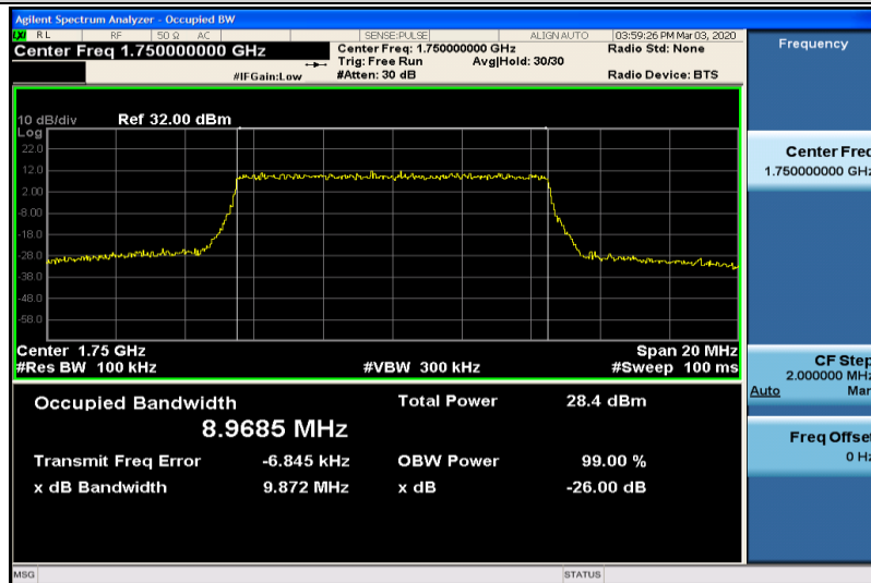
Band4-10MHz-16QAM-20350-50RB#0-8.9685
