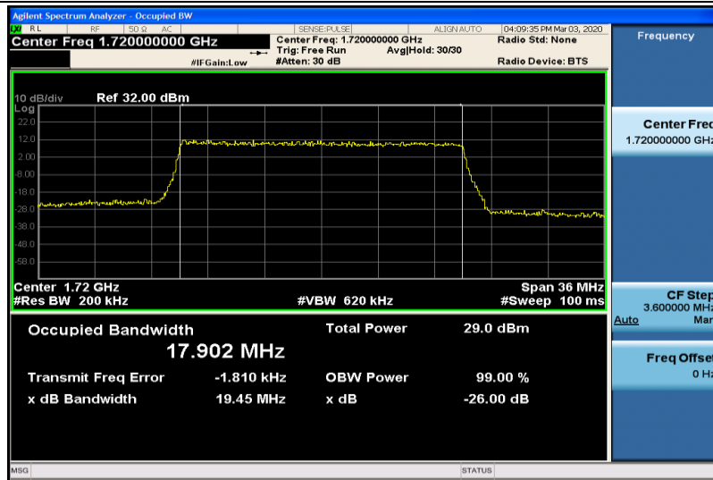
Band4-20MHz-16QAM-20050-100RB#0-17.902
