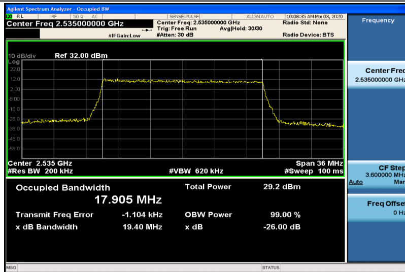
Band7-20MHz-QPSK-21100-100RB#0-17.905
