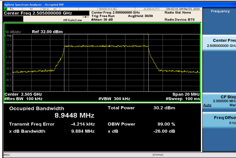
Band7-10MHz-QPSK-20800-50RB#0-8.9448
