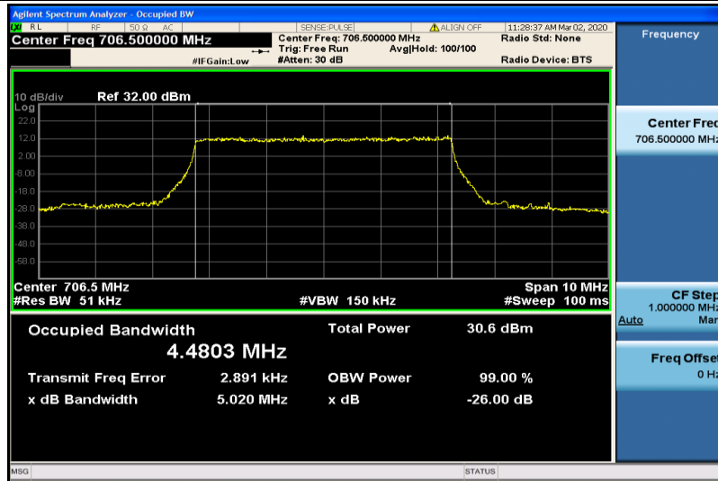
Band17-5MHz-QPSK-23755-25RB#0-4.4803
