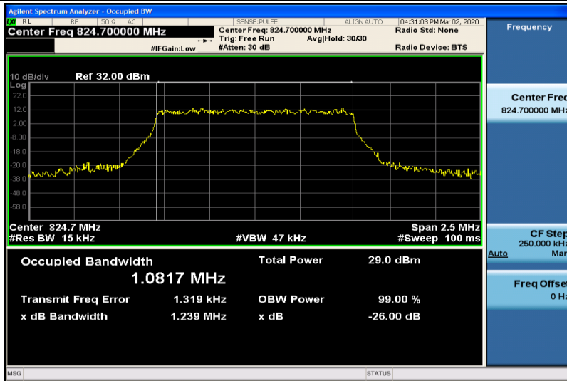
Band5-1.4MHz-QPSK-20407-6RB#0-1.0817
