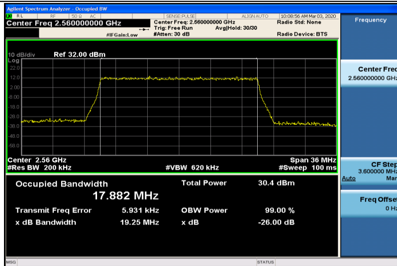
Band7-20MHz-QPSK-21350-100RB#0-17.882
