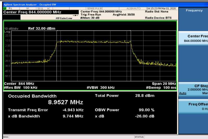
Band5-10MHz-16QAM-20600-50RB#0-8.9527
