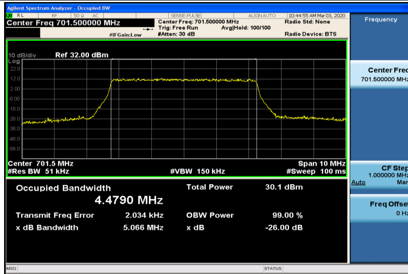
Band12-5MHz-16QAM-23035-25RB#0-4.4790
