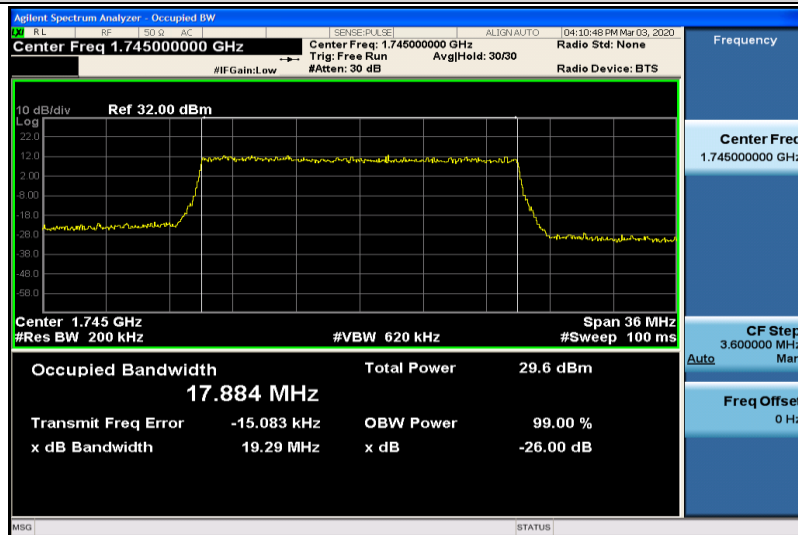
Band4-20MHz-QPSK-20300-100RB#0-17.884
