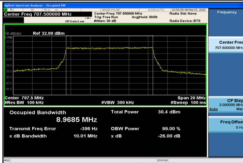
Band12-10MHz-16QAM-23095-50RB#0-8.9685
