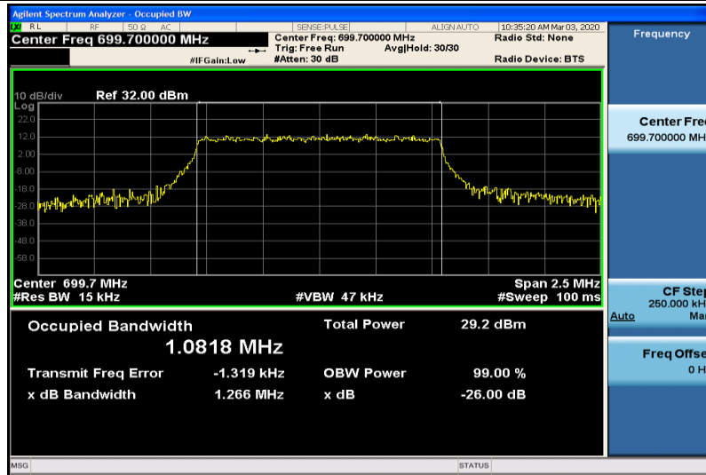
Band12-1.4MHz-16QAM-23017-6RB#0-1.0818
