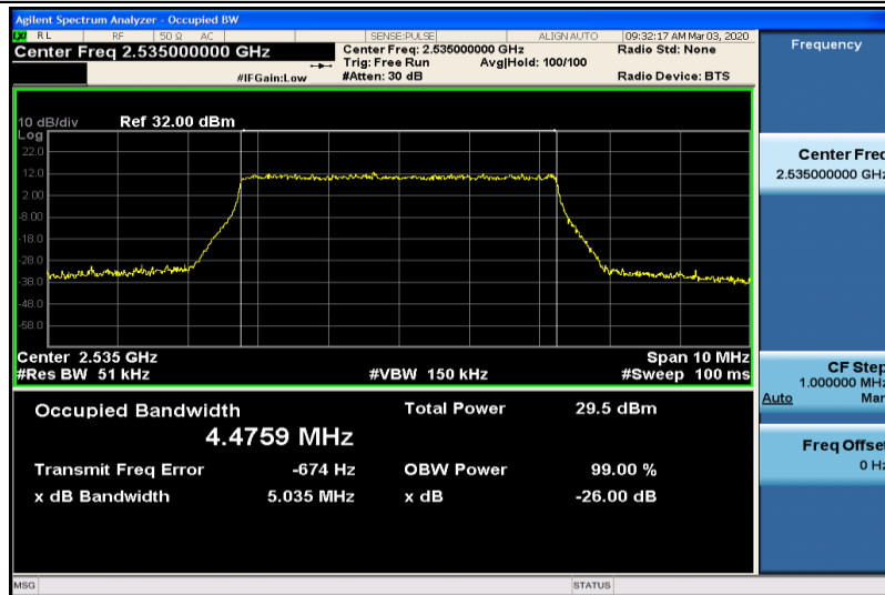
Band7-5MHz-QPSK-21100-25RB#0-4.4759
