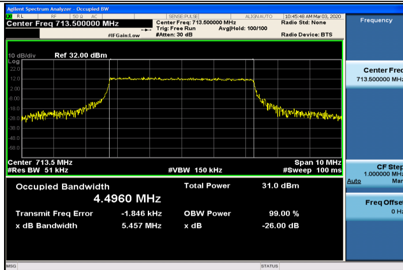
Band12-5MHz-QPSK-23155-25RB#0-4.4960
