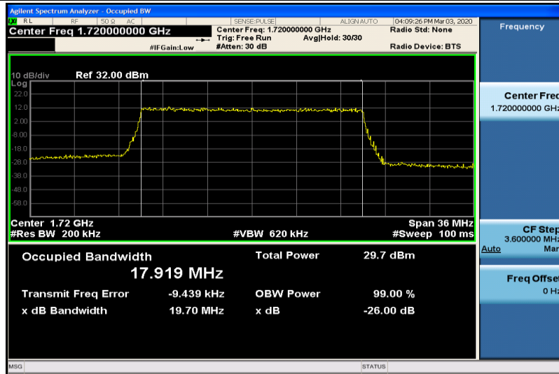
Band4-20MHz-QPSK-20050-100RB#0-17.919
