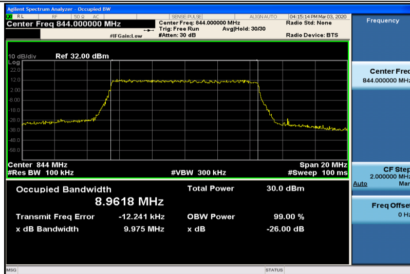
Band5-10MHz-QPSK-20600-50RB#0-8.9618
