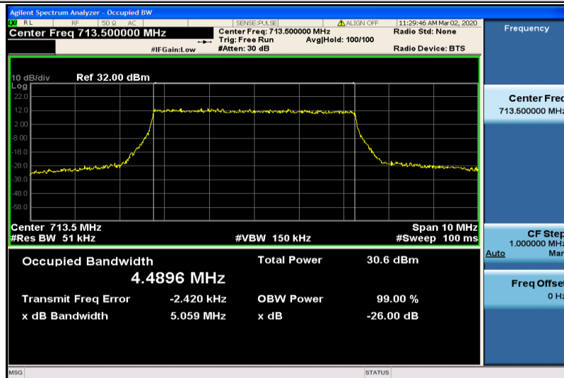
Band17-5MHz-QPSK-23825-25RB#0-4.4896
