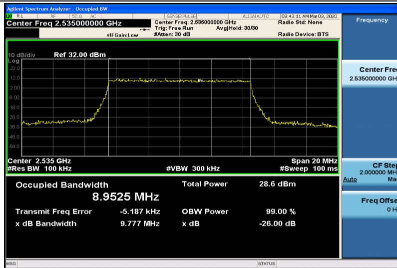
Band7-10MHz-16QAM-21100-50RB#0-8.9525
