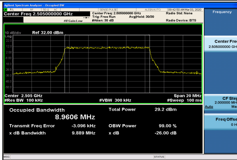
Band7-10MHz-16QAM-20800-50RB#0-8.9606
