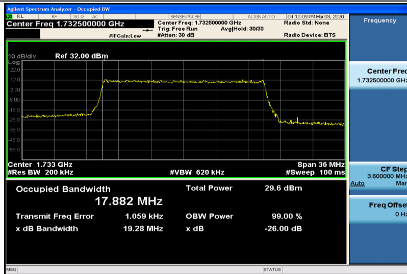
Band4-20MHz-QPSK-20175-100RB#0-17.882
