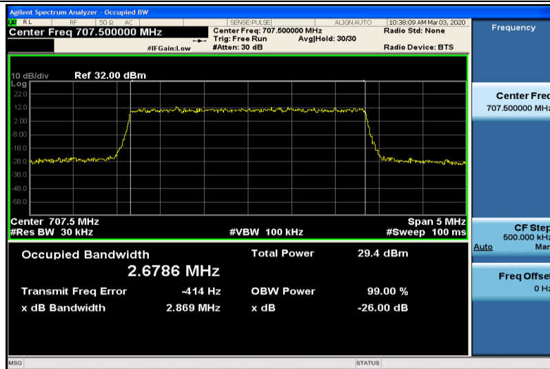
Band12-3MHz-16QAM-23095-15RB#0-2.6786
