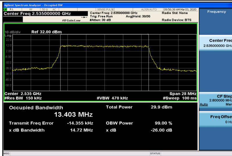
Band7-15MHz-QPSK-21100-75RB#0-13.403
