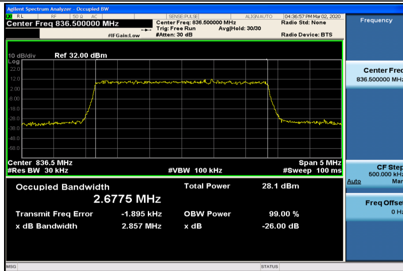
Band5-3MHz-16QAM-20525-15RB#0-2.6775
