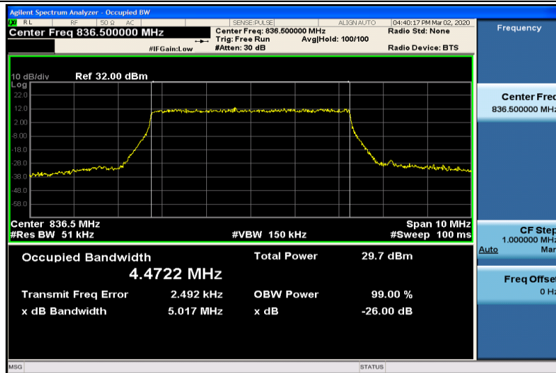
Band5-5MHz-QPSK-20525-25RB#0-4.4722
