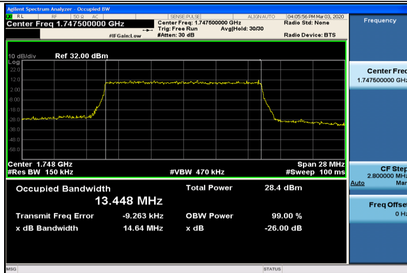
Band4-15MHz-16QAM-20325-75RB#0-13.448
