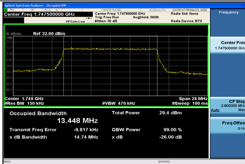
Band4-15MHz-QPSK-20325-75RB#0-13.448
