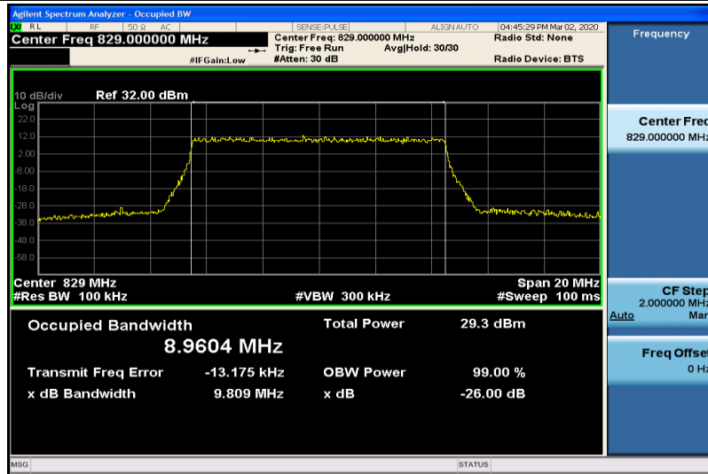
Band5-10MHz-16QAM-20450-50RB#0-8.9604
