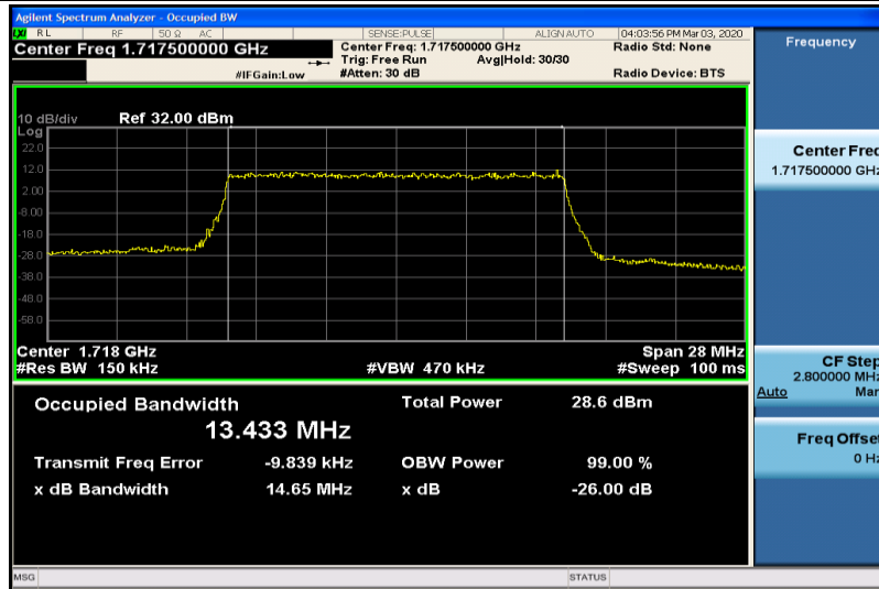
Band4-15MHz-16QAM-20025-75RB#0-13.433
