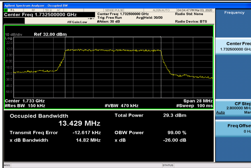
Band4-15MHz-QPSK-20175-75RB#0-13.429
