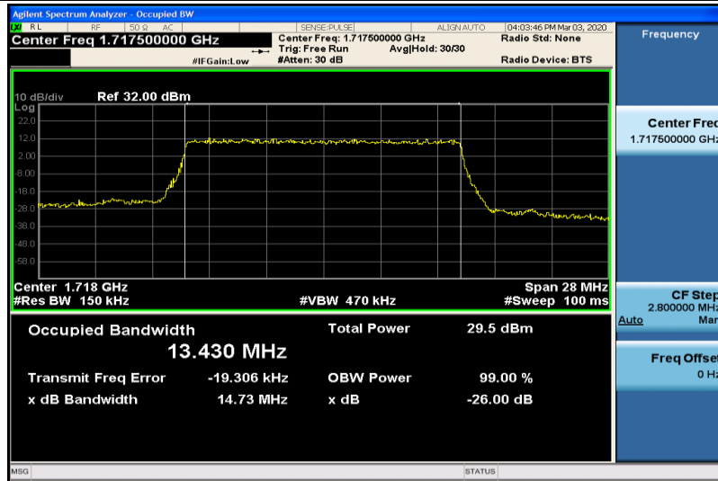
Band4-15MHz-QPSK-20025-75RB#0-13.430
