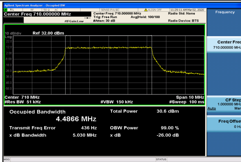
Band17-5MHz-QPSK-23790-25RB#0-4.4866
