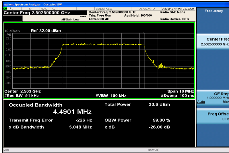
Band7-5MHz-QPSK-20775-25RB#0-4.4901
