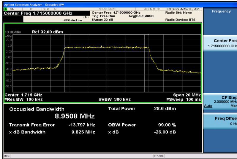
Band4-10MHz-16QAM-20000-50RB#0-8.9508
