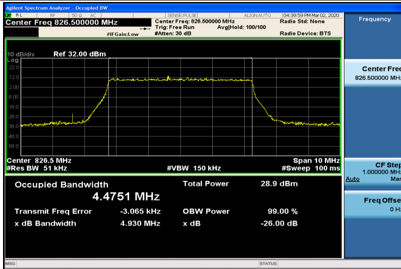
Band5-5MHz-16QAM-20425-25RB#0-4.4751
