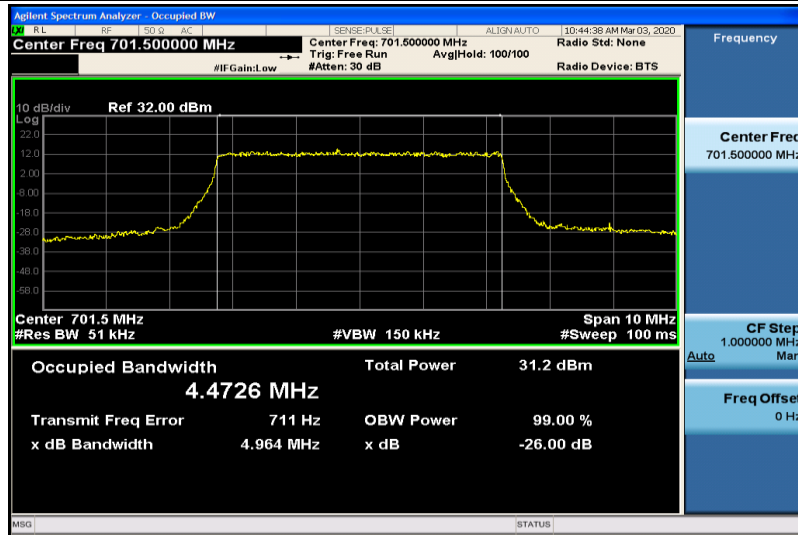
Band12-5MHz-QPSK-23035-25RB#0-4.4726
