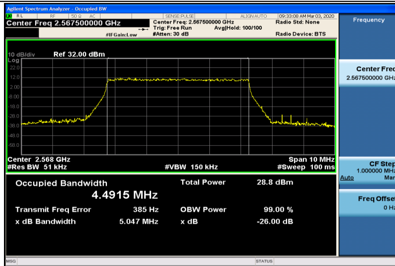
Band7-5MHz-16QAM-21425-25RB#0-4.4915
