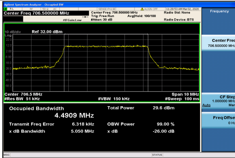
Band17-5MHz-16QAM-23755-25RB#0-4.4909
