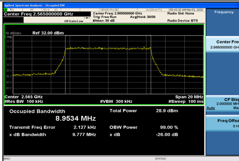
Band7-10MHz-16QAM-21400-50RB#0-8.9534
