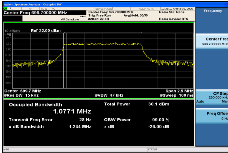
Band12-1.4MHz-QPSK-23017-6RB#0-1.0771
