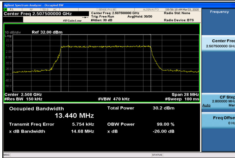
Band7-15MHz-QPSK-20825-75RB#0-13.440
