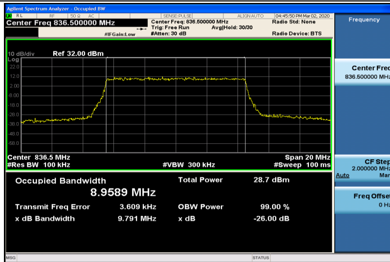
Band5-10MHz-16QAM-20525-50RB#0-8.9589
