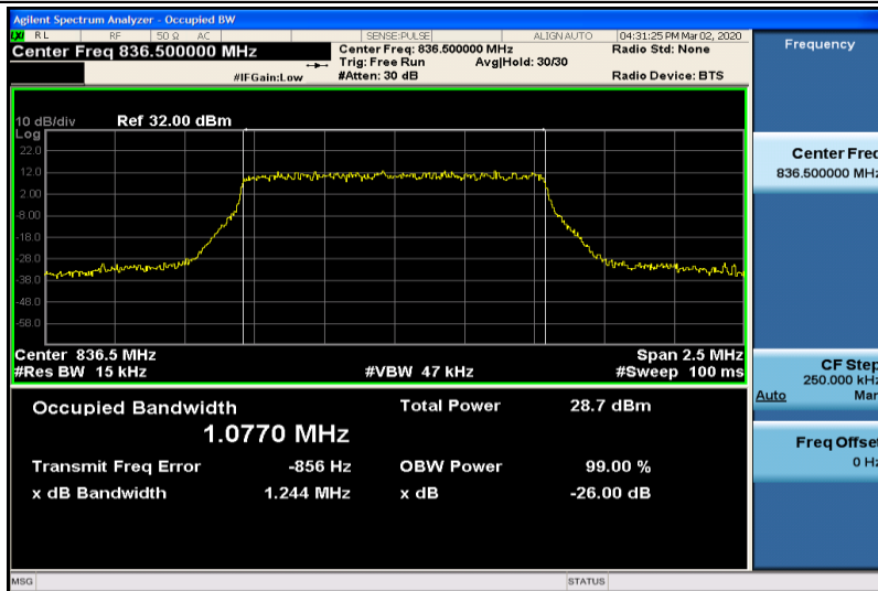
Band5-1.4MHz-QPSK-20525-6RB#0-1.0770
