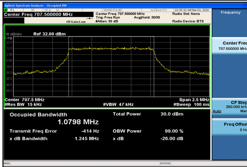
Band12-1.4MHz-QPSK-23095-6RB#0-1.0798
