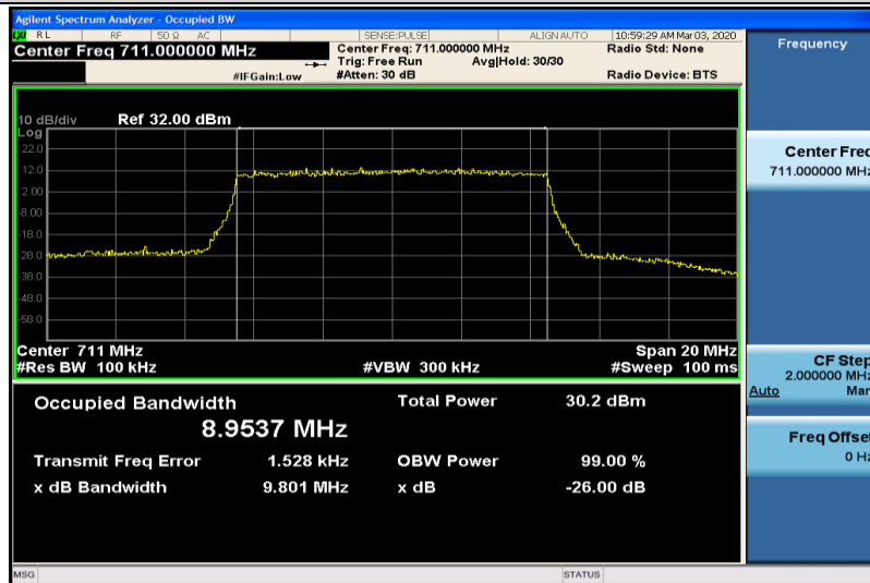
Band12-10MHz-16QAM-23130-50RB#0-8.9537
