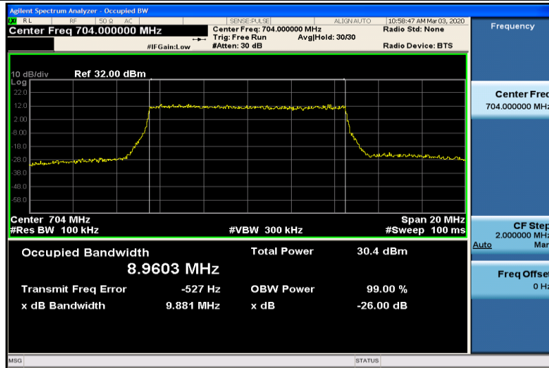
Band12-10MHz-16QAM-23060-50RB#0-8.9603
