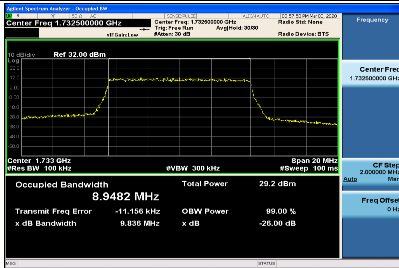
Band4-10MHz-QPSK-17325-50RB#0-8.9482
