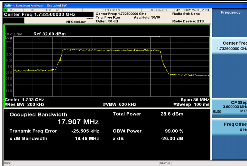
Band4-20MHz-16QAM-20175-100RB#0-17.907
