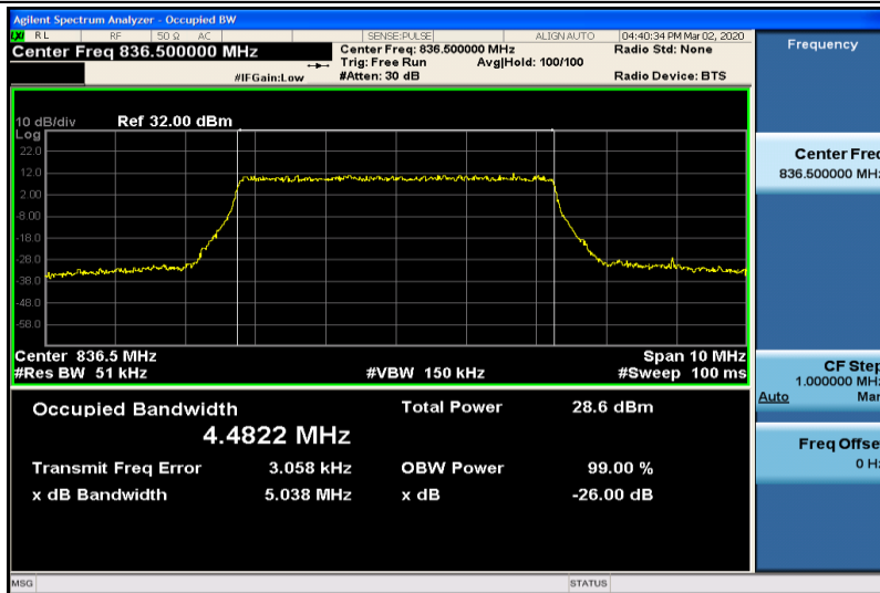
Band5-5MHz-16QAM-20525-25RB#0-4.4822
