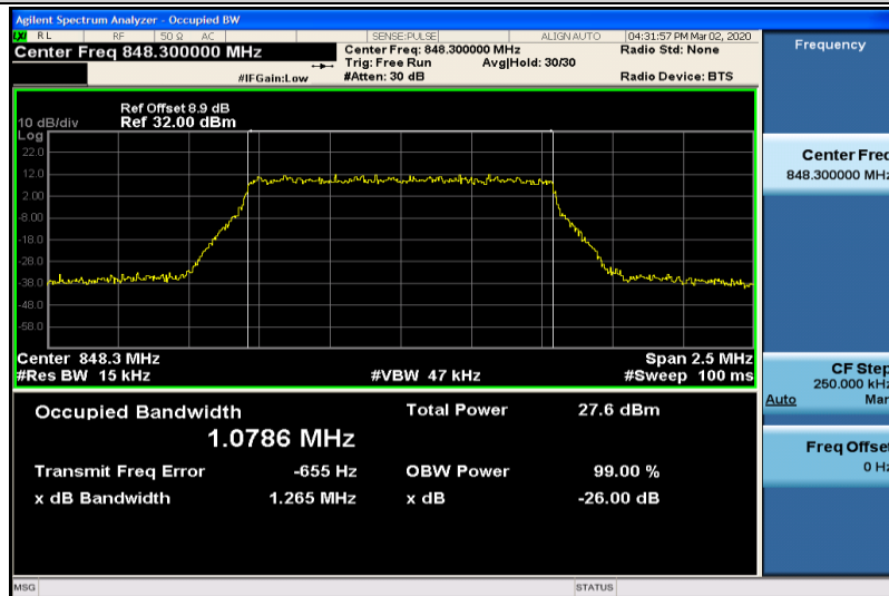
Band5-1.4MHz-16QAM-20643-6RB#0-1.0786
