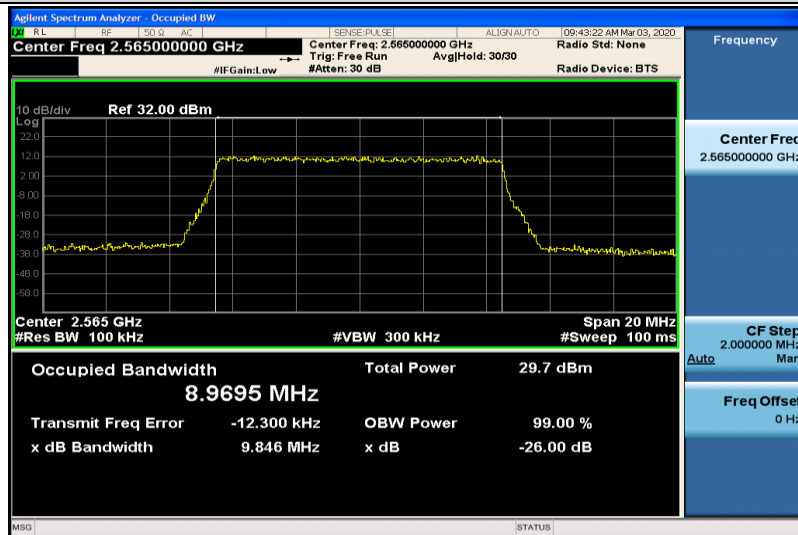
Band7-10MHz-QPSK-21400-50RB#0-8.9695
