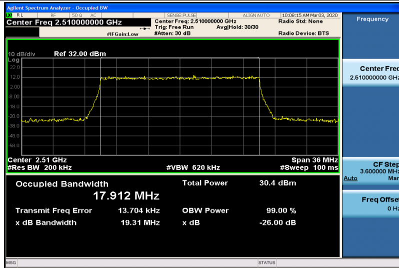
Band7-20MHz-QPSK-20850-100RB#0-17.912
