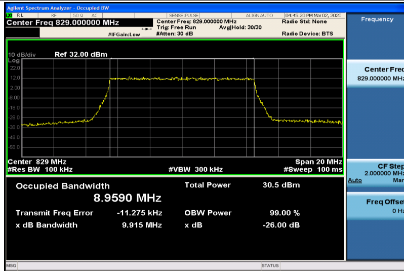
Band5-10MHz-QPSK-20450-50RB#0-8.9590
