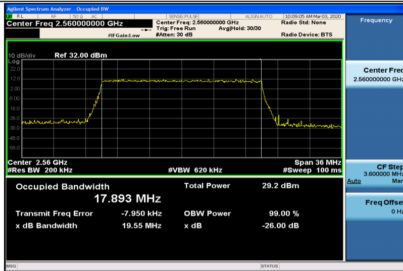
Band7-20MHz-16QAM-21350-100RB#0-17.893
