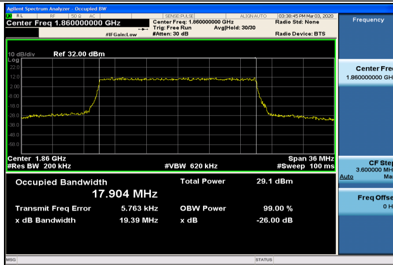
Band2-20MHz-16QAM-18600-100RB#0-17.904
