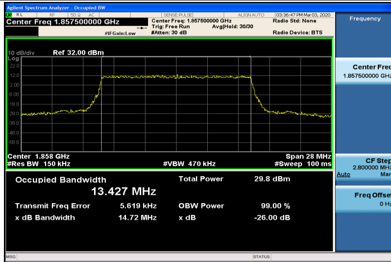
Band2-15MHz-QPSK-18675-75RB#0-13.427
