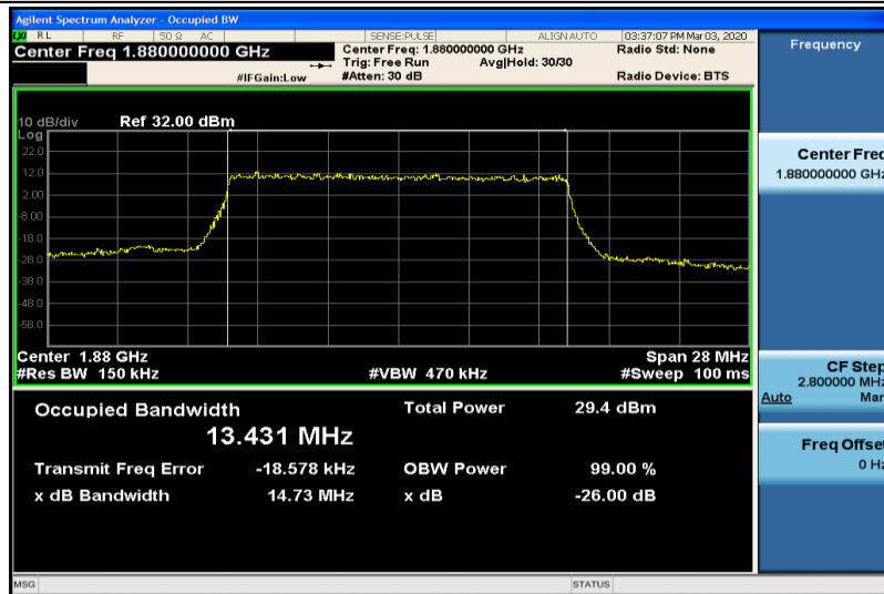
Band2-15MHz-QPSK-18900-75RB#0-13.431
