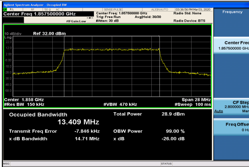
Band2-15MHz-16QAM-18675-75RB#0-13.409
