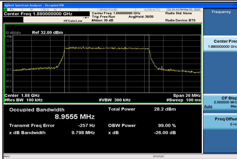
Band2-10MHz-16QAM-18900-50RB#0-8.9555
