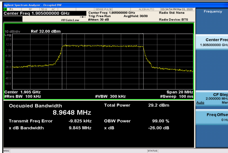
Band2-10MHz-QPSK-19150-50RB#0-8.9648
