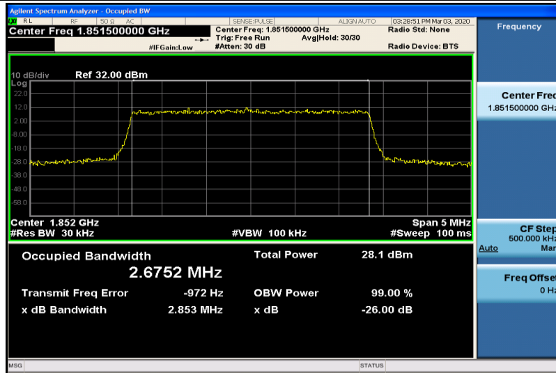
Band2-3MHz-16QAM-18515-15RB#0-2.6752
