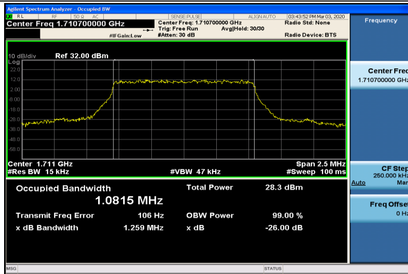
Band4-1.4MHz-QPSK-19957-6RB#0-1.0815
