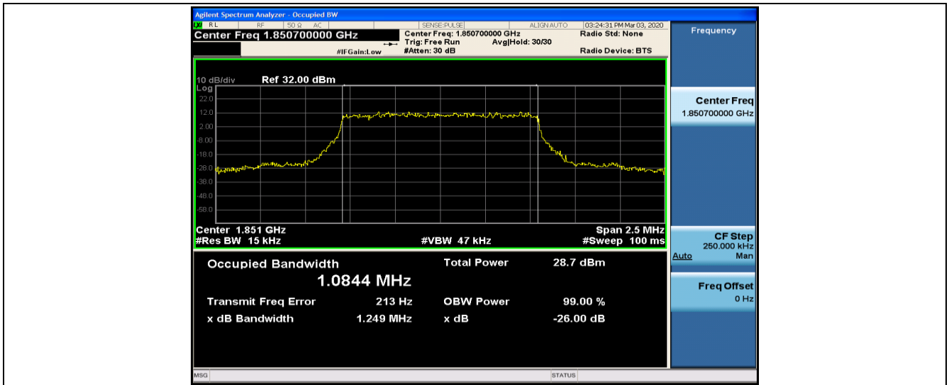
Band2-1.4MHz-QPSK-18607-6RB#0-1.0844
