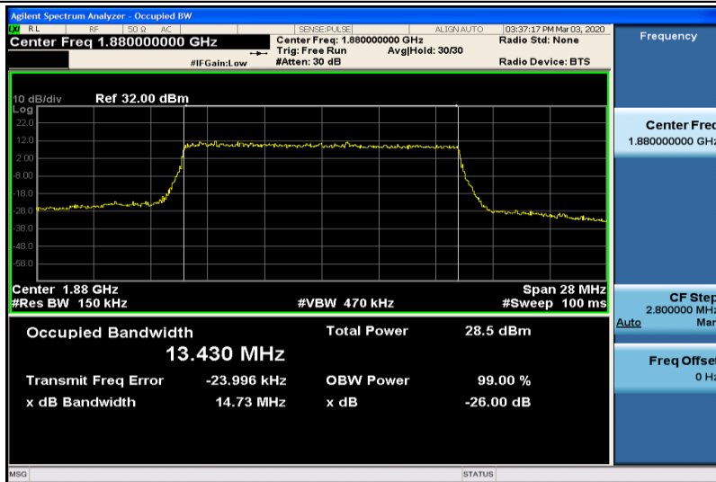
Band2-15MHz-16QAM-18900-75RB#0-13.430
