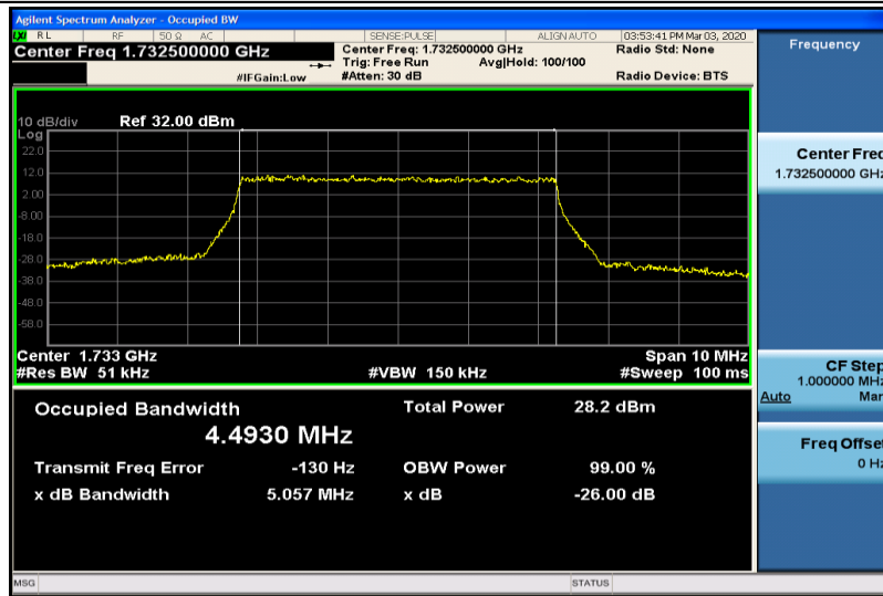
Band4-5MHz-16QAM-20175-25RB#0-4.4930
