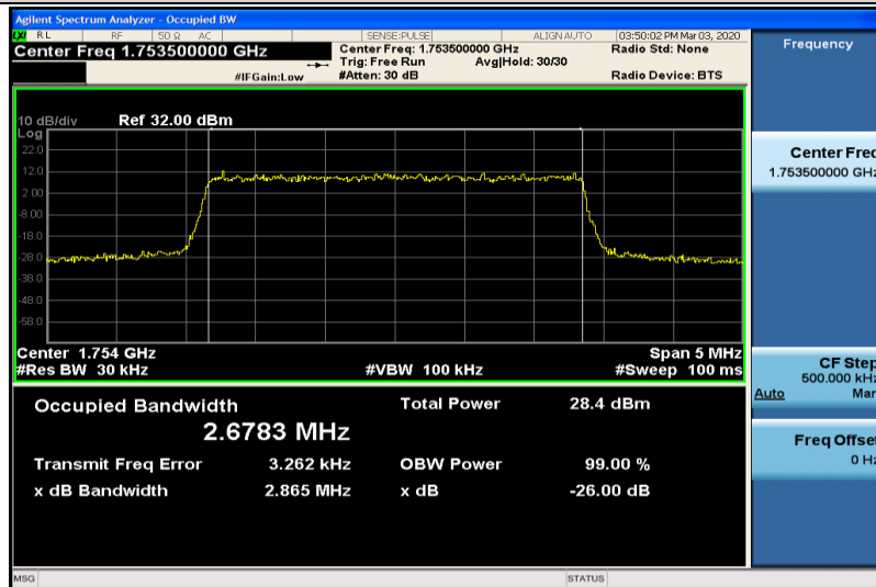
Band4-3MHz-QPSK-20385-15RB#0-2.6783
