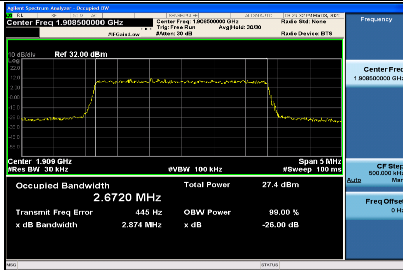
Band2-3MHz-16QAM-19185-15RB#0-2.6720
