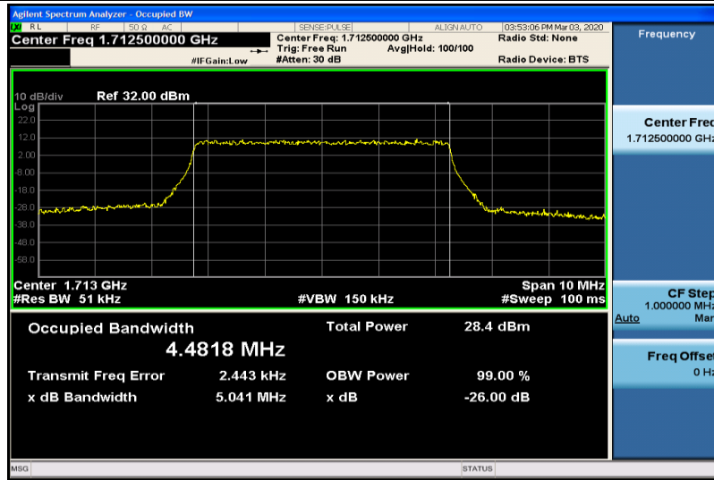
Band4-5MHz-16QAM-19975-25RB#0-4.4818
