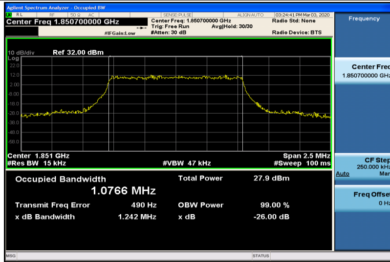
Band2-1.4MHz-16QAM-18607-6RB#0-1.0766
