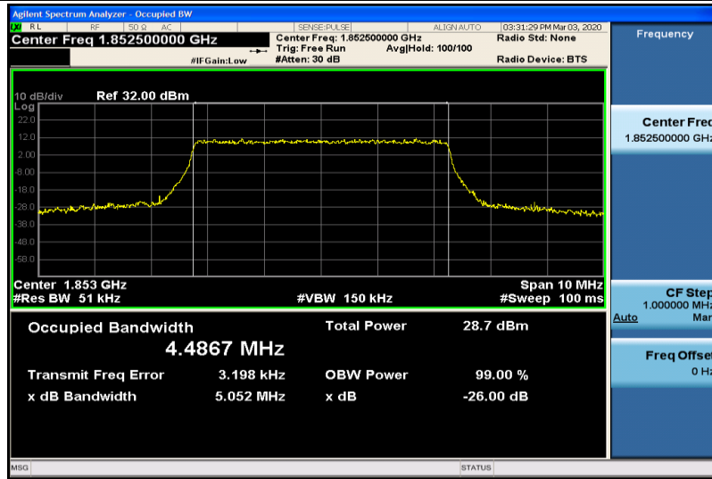
Band2-5MHz-16QAM-18625-25RB#0-4.4867
