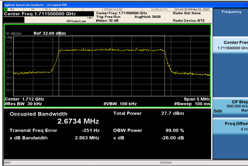
Band4-3MHz-16QAM-19965-15RB#0-2.6734
