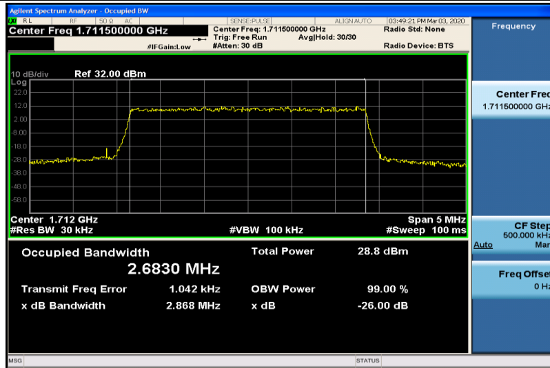
Band4-3MHz-QPSK-19965-15RB#0-2.6830
