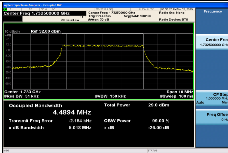
Band4-5MHz-QPSK-17325-25RB#0-4.4894
