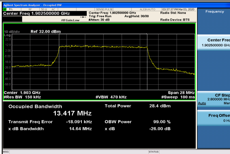
Band2-15MHz-16QAM-19125-75RB#0-13.417
