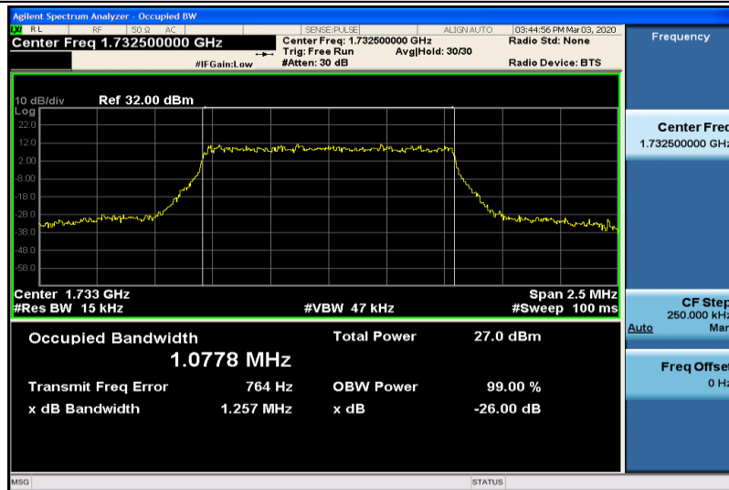
Band4-1.4MHz-16QAM-20175-6RB#0-1.0778
