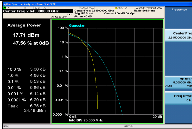
Band41-20MHz-16QAM-41140-1RB#0
