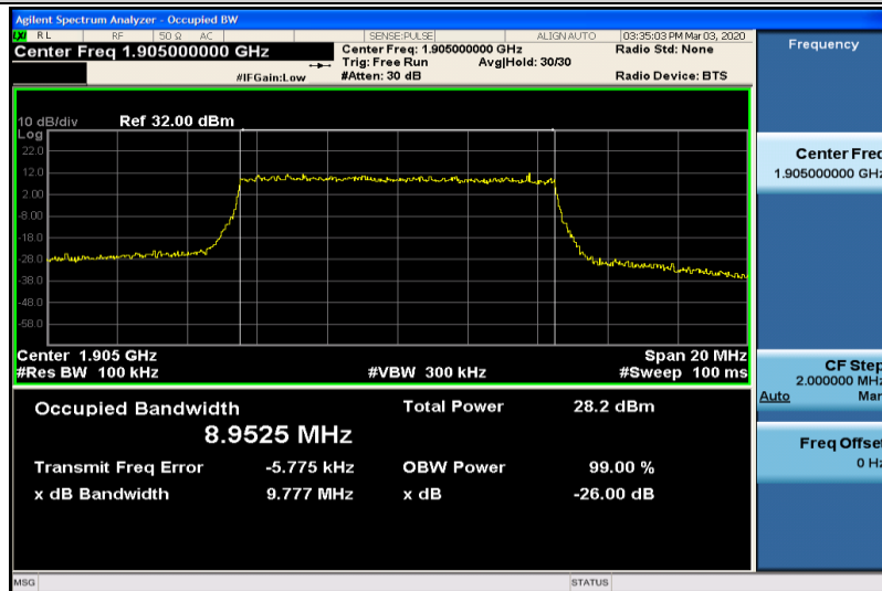
Band2-10MHz-16QAM-19150-50RB#0-8.9525
