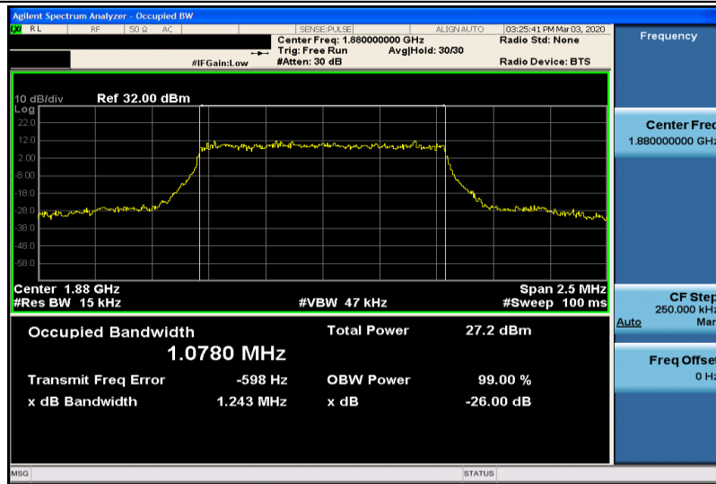
Band2-1.4MHz-16QAM-18900-6RB#0-1.0780
