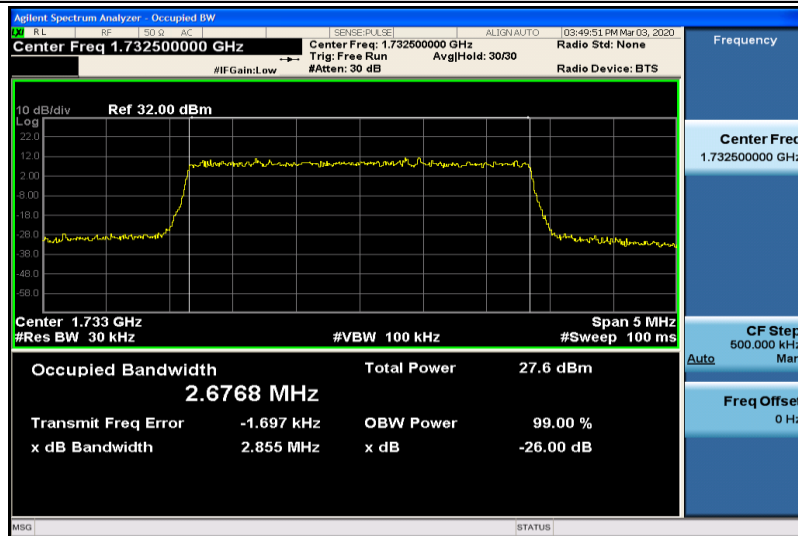
Band4-3MHz-16QAM-20175-15RB#0-2.6768
