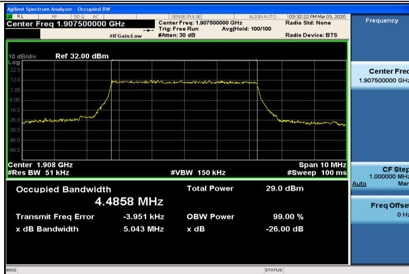
Band2-5MHz-QPSK-19175-25RB#0-4.4858
