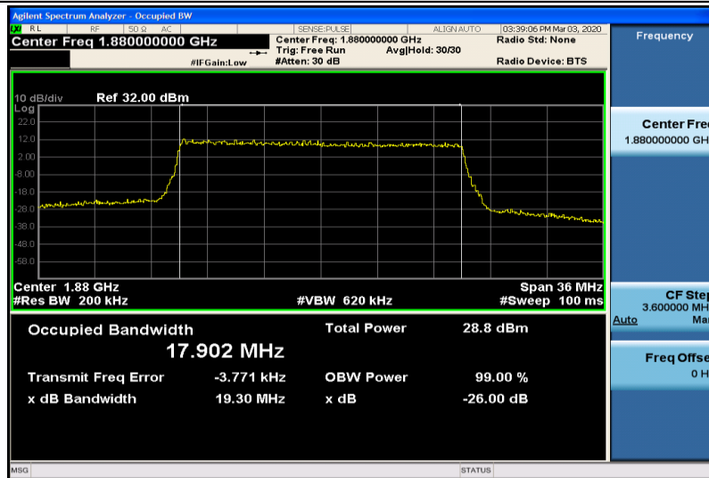
Band2-20MHz-16QAM-18900-100RB#0-17.902
