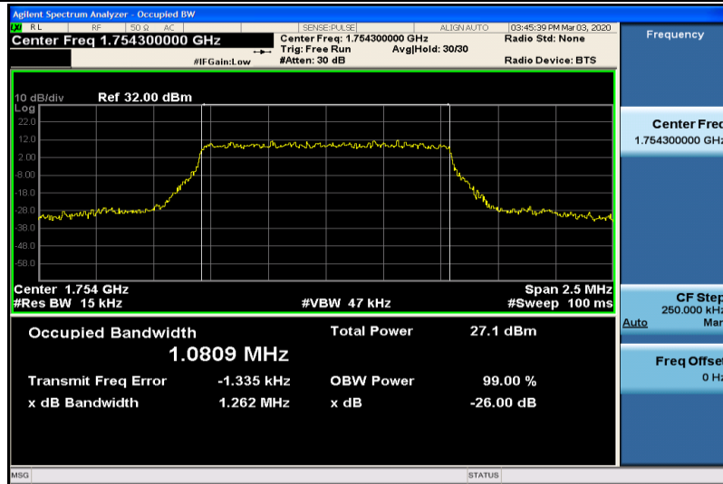
Band4-1.4MHz-16QAM-20393-6RB#0-1.0809
