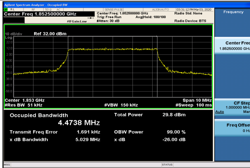
Band2-5MHz-QPSK-18625-25RB#0-4.4738
