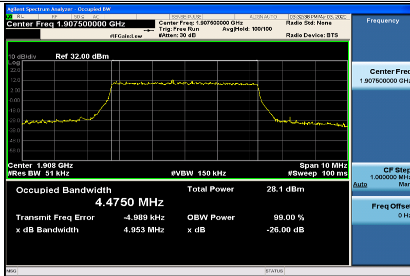
Band2-5MHz-16QAM-19175-25RB#0-4.4750
