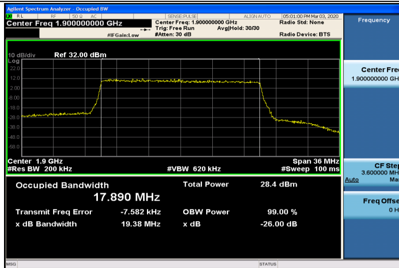
Band2-20MHz-16QAM-19100-100RB#0-17.890
