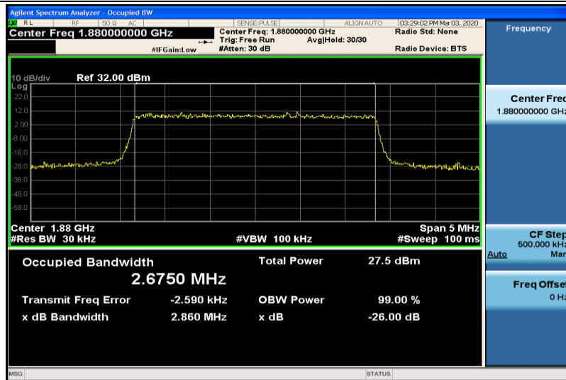
Band2-3MHz-QPSK-18900-15RB#0-2.6750
