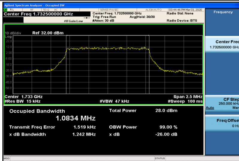
Band4-1.4MHz-QPSK-20175-6RB#0-1.0834
