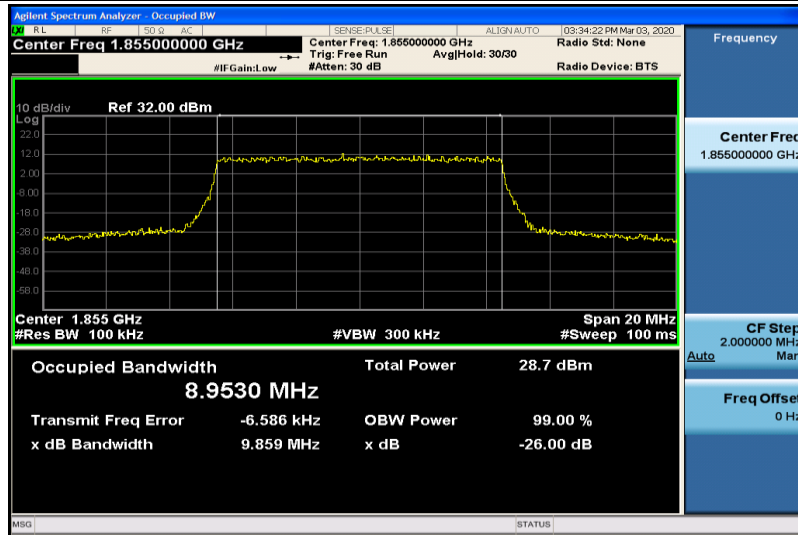
Band2-10MHz-16QAM-18650-50RB#0-8.9530
