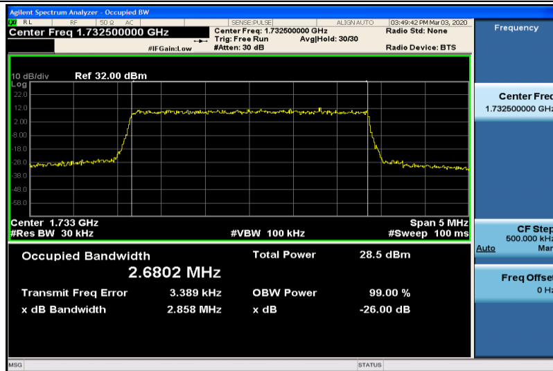
Band4-3MHz-QPSK-20175-15RB#0-2.6802
