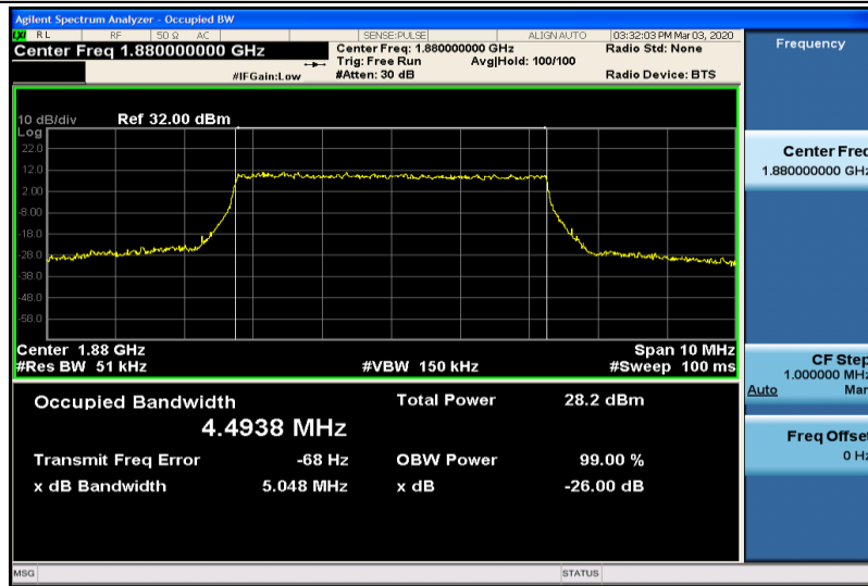
Band2-5MHz-16QAM-18900-25RB#0-4.4938
