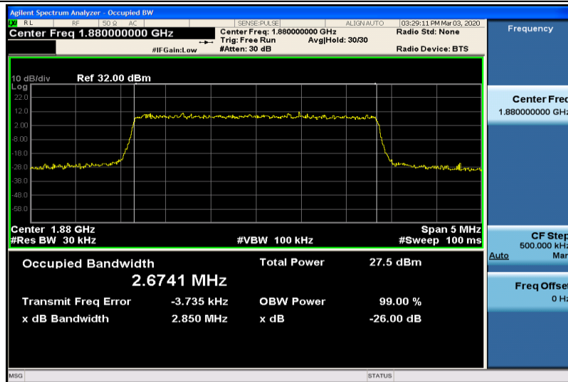
Band2-3MHz-16QAM-18900-15RB#0-2.6741
