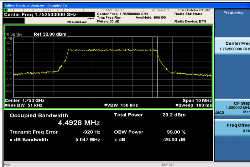
Band4-5MHz-QPSK-20175-25RB#0-4.4928
