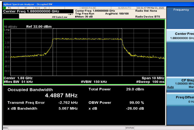
Band2-5MHz-QPSK-18900-25RB#0-4.4887
