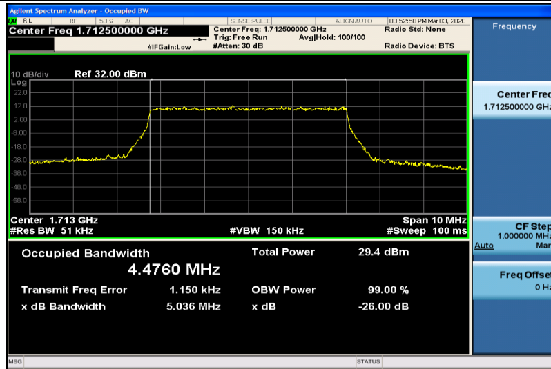
Band4-5MHz-QPSK-19975-25RB#0-4.4760
