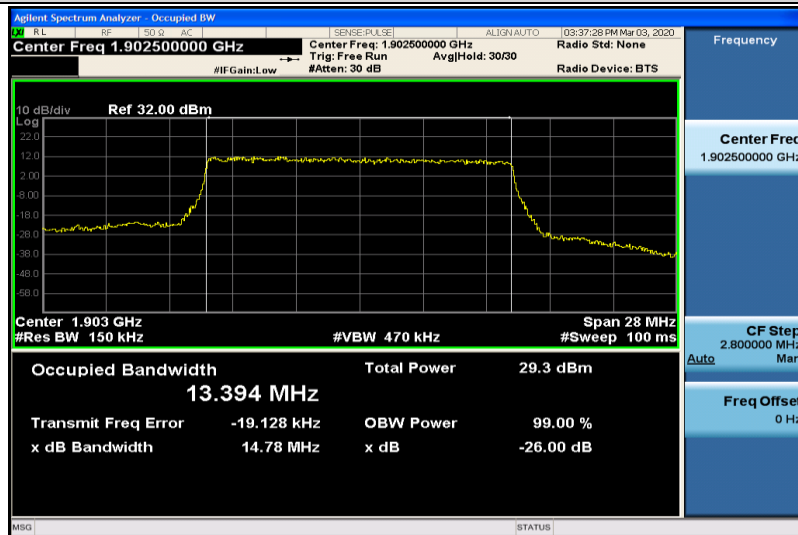
Band2-15MHz-QPSK-19125-75RB#0-13.394
