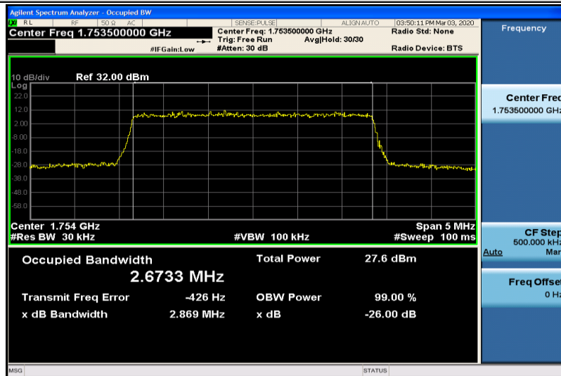
Band4-3MHz-16QAM-20385-15RB#0-2.6733
