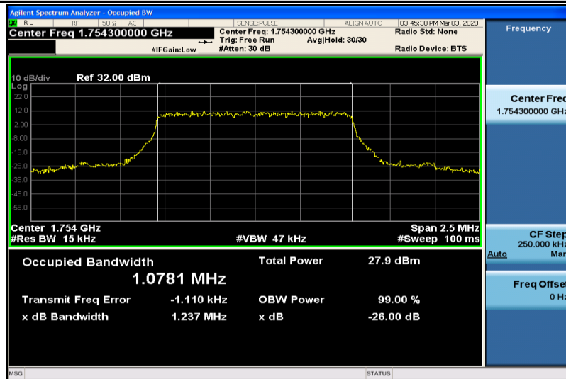
Band4-1.4MHz-QPSK-20393-6RB#0-1.0781
