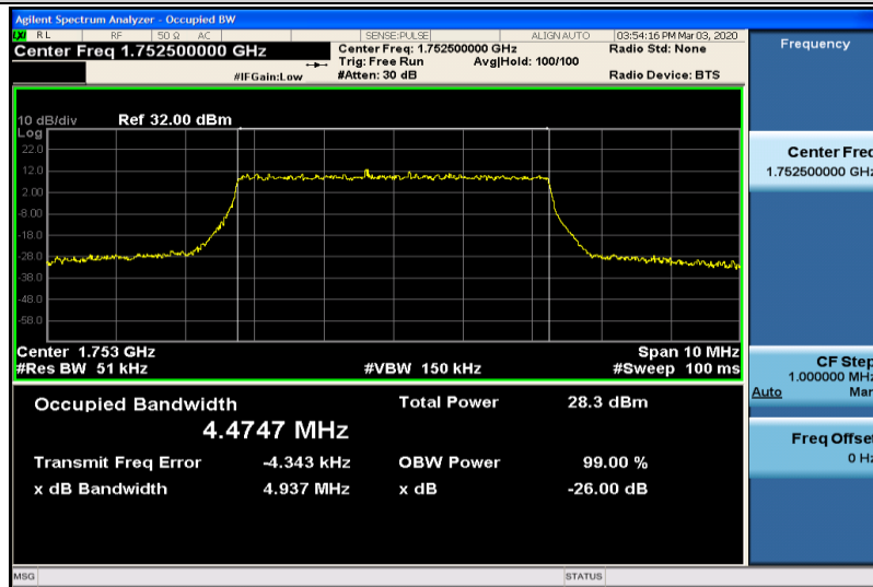
Band4-5MHz-16QAM-20375-25RB#0-4.4747
