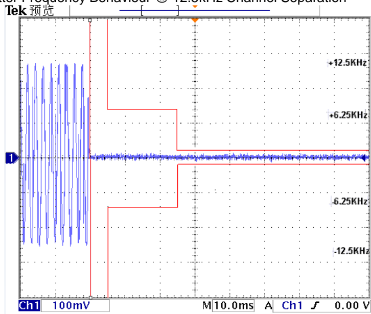
Transmitter Frequency Behaviour @ 12.5kHz Channel Separation-----On – Off
