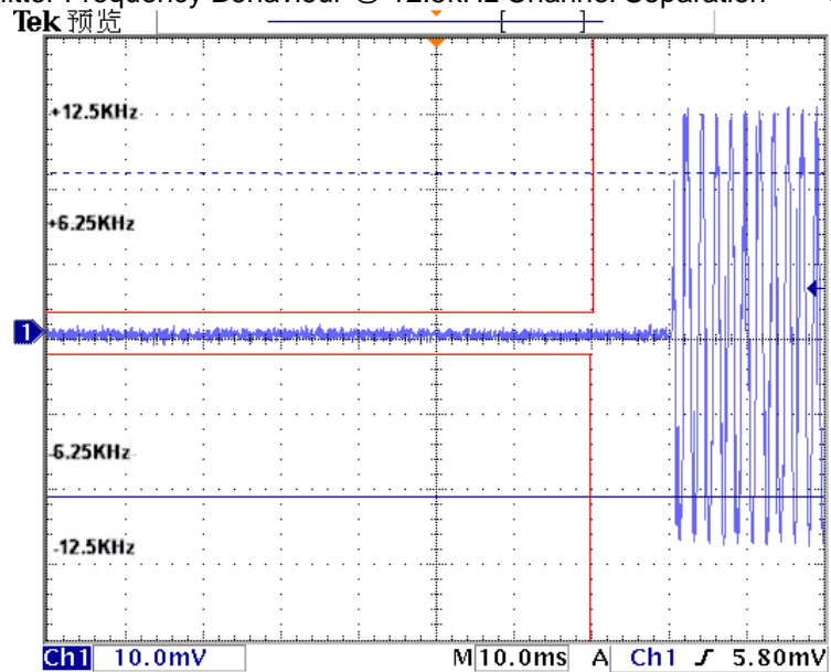
Transmitter Frequency Behaviour @ 12.5kHz Channel Separation-----On – Off
