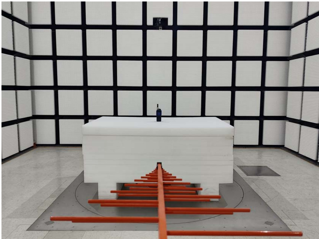
Radiated Emission Below 1GHz View- Model:DP815
