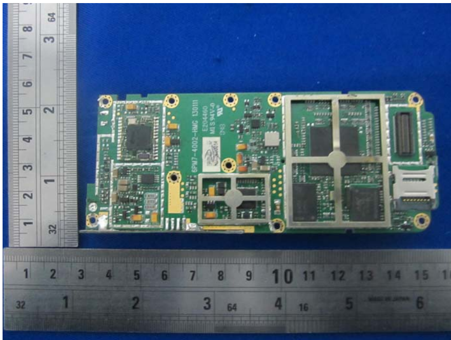
EUT –Main Board without Cover Top View
