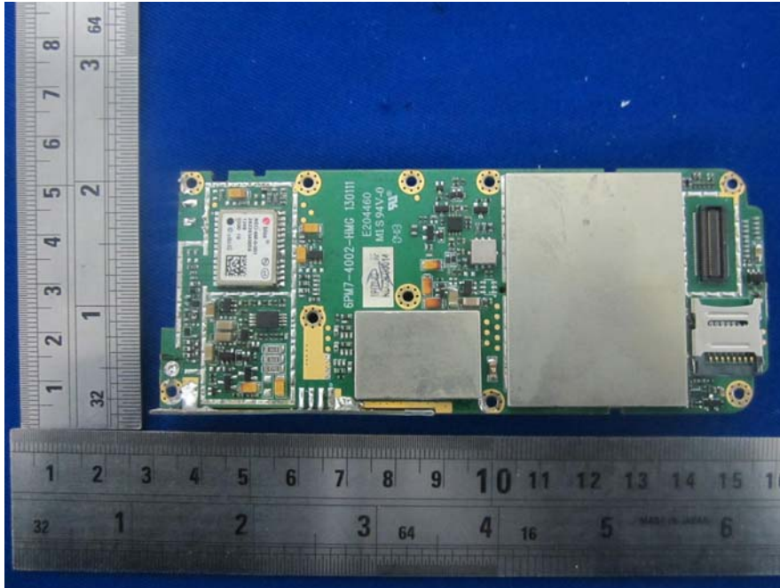
EUT –Main Board with Cover Top View
