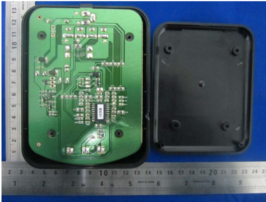
Charger –Cover Off View
