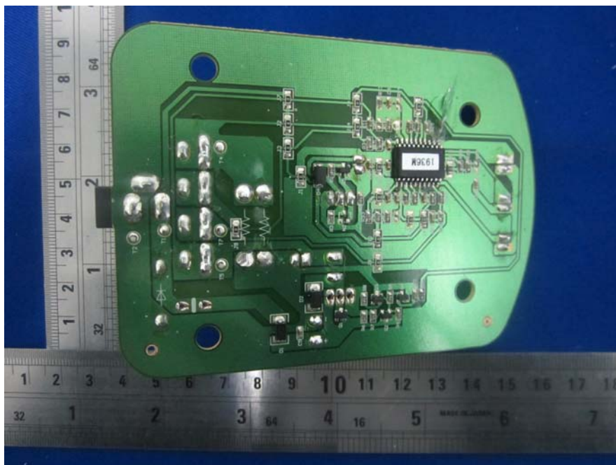
Charger –Main Board Bottom View
