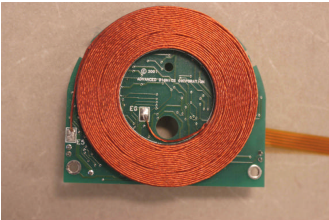
Back of Charger Circuit Board
