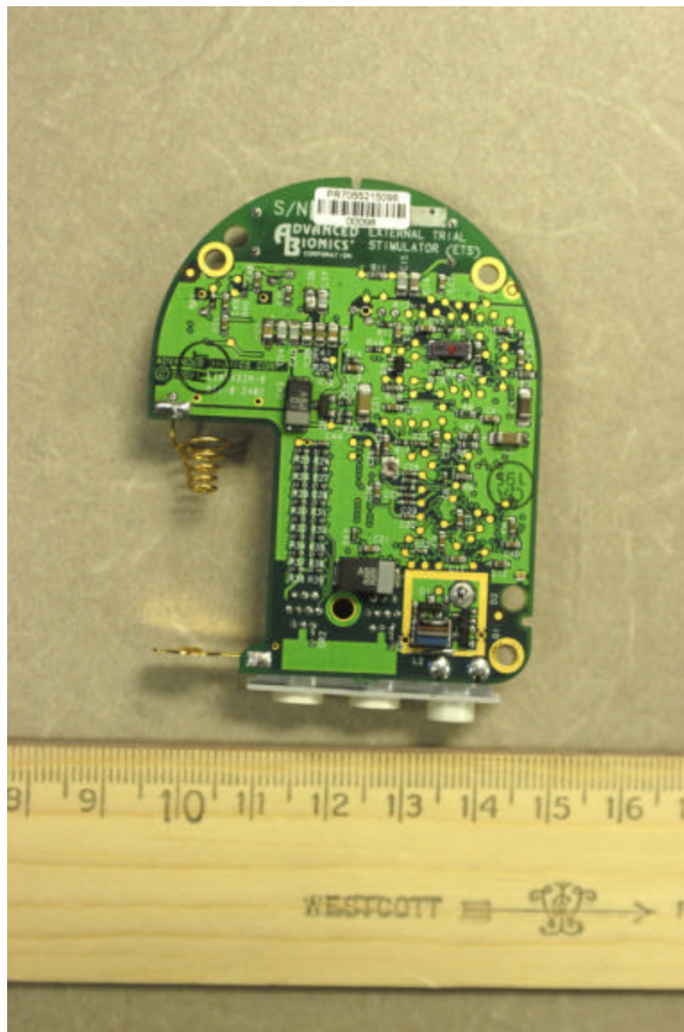
Back of External Trial Stimulator Circuit Board
