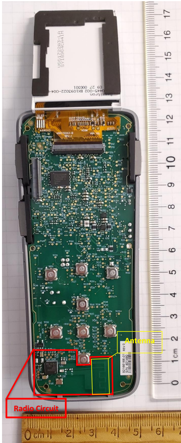
Figure 2: RC5 Internal Photo – Frontside (radio circuit outlined)
