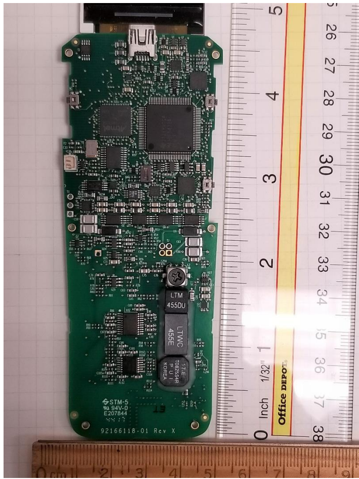
Figure 4: RC5 Internal Photo – PCBA Backside
