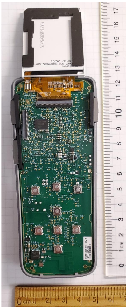
Figure 1: RC5 Internal Photo – Frontside
