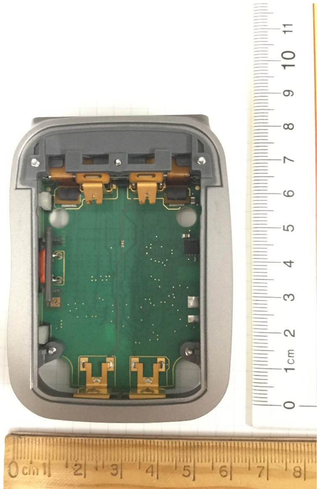
Figure 3: Wilson-I ETS Internal Photo – Backside
