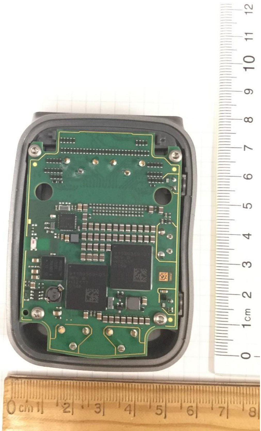
Figure 1: Wilson-I ETS Internal Photo – Frontside
