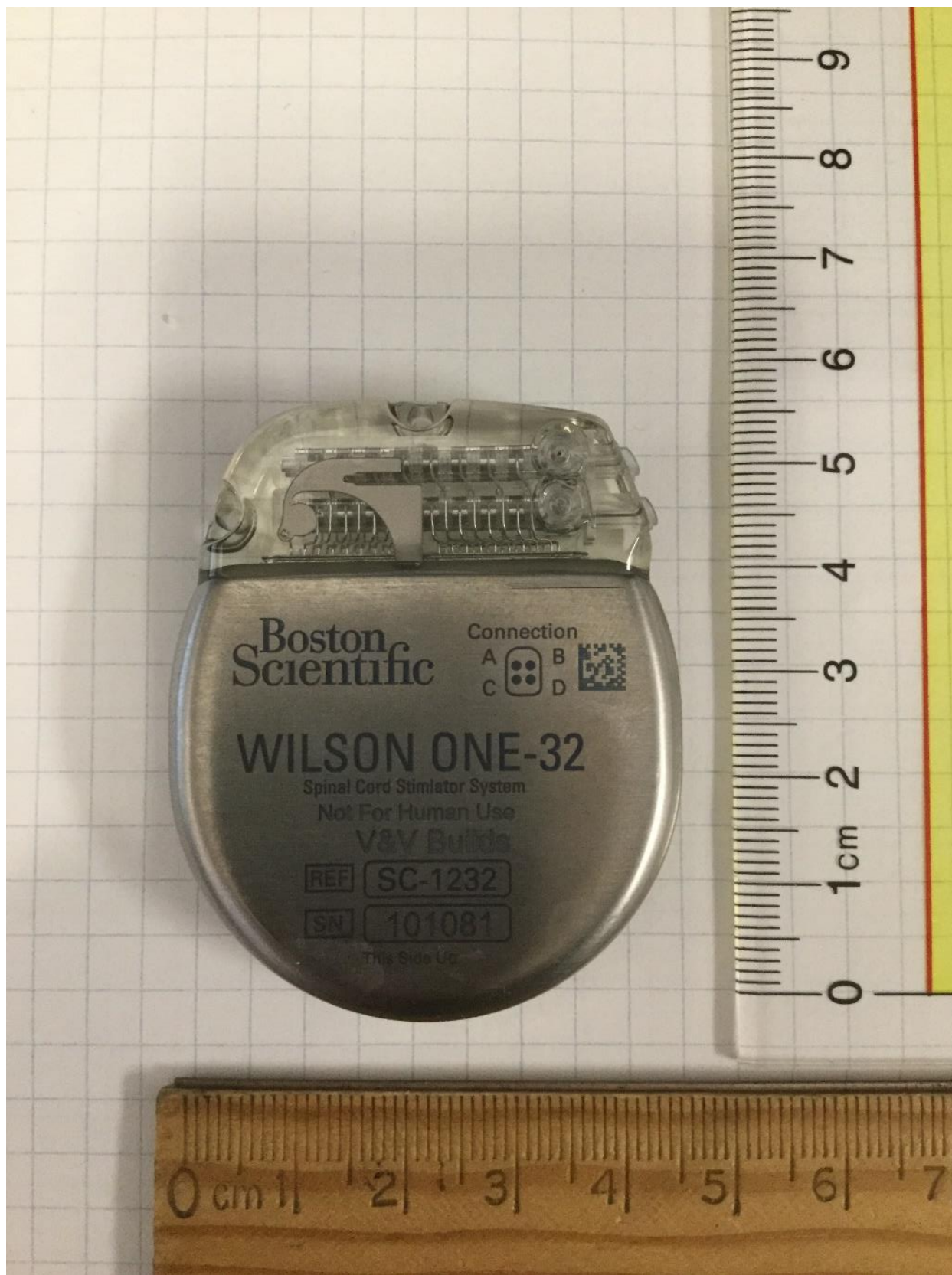
Figure 1: Wilson-I IPG External Photo – Frontside
