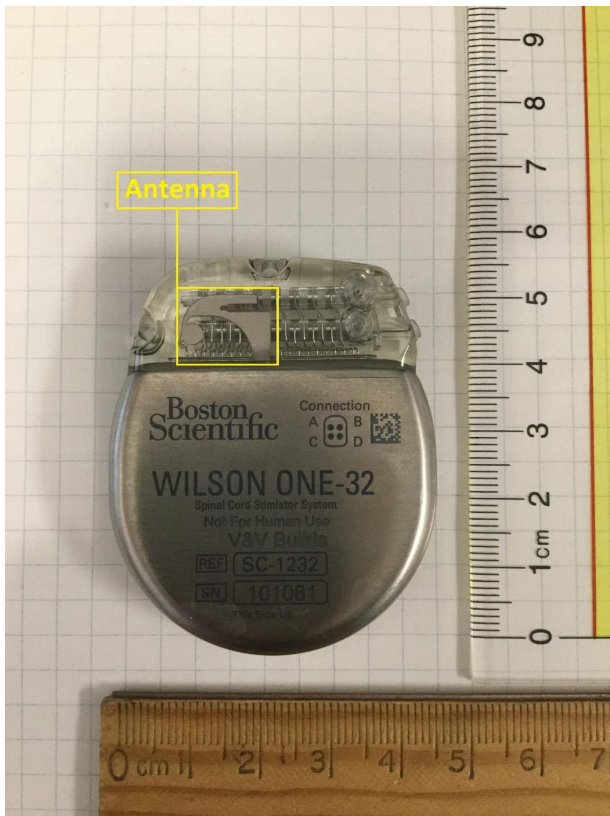
Figure 2: Wilson-I IPG External Photo – Frontside (antenna outlined)
