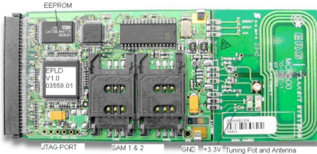
Figure 4: MCR500 PCB Top View
