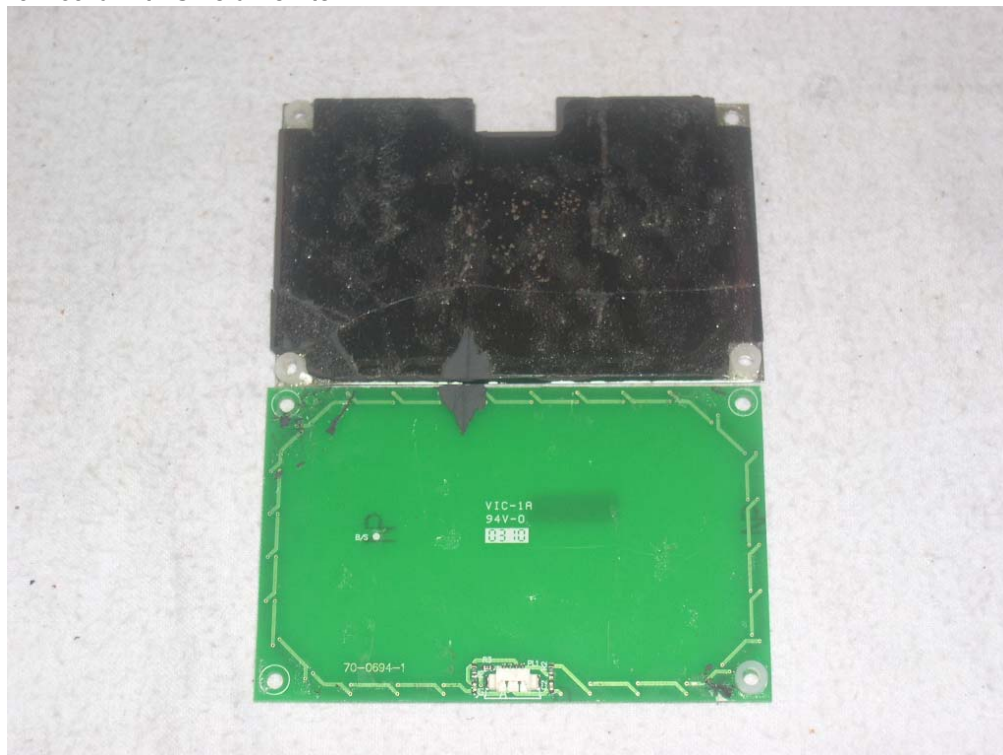
Antenna Board with Shield/Ferrite
