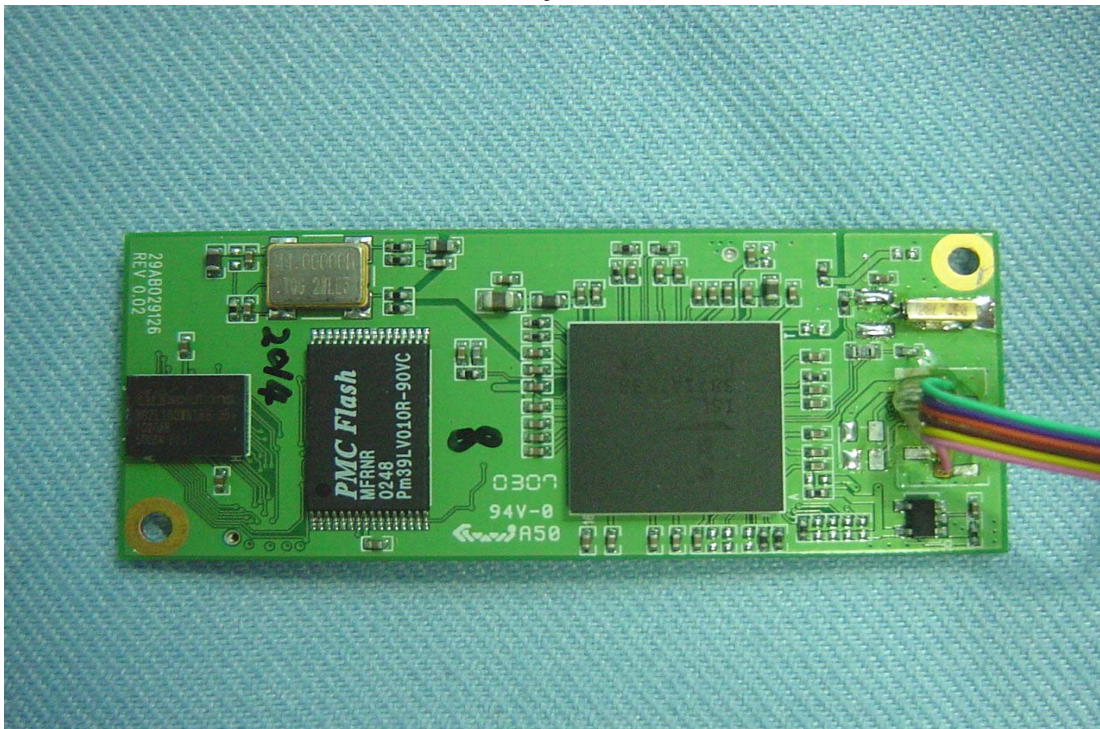
Back View of RF Module
