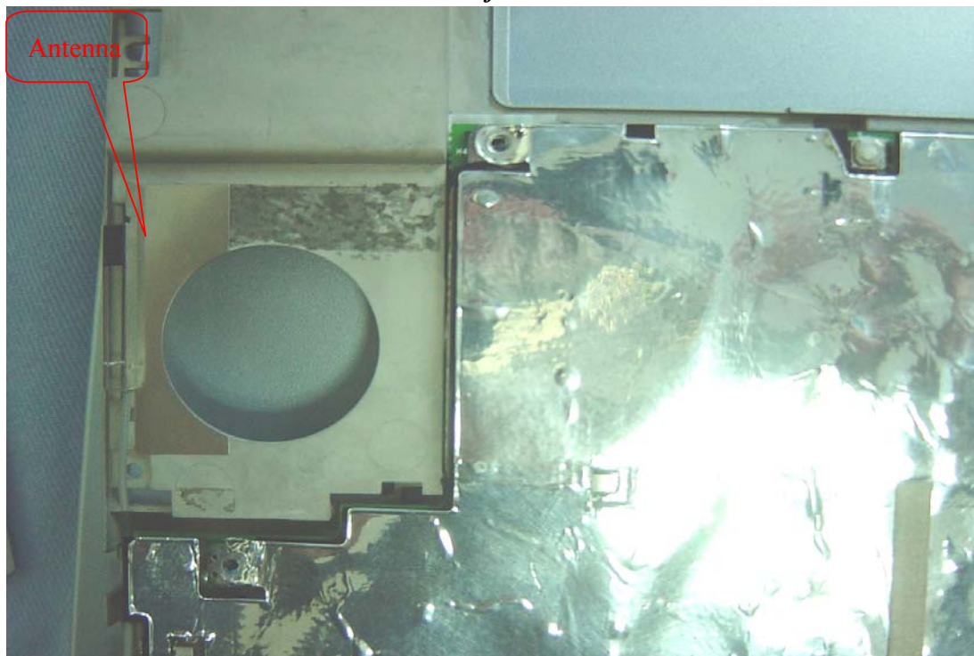
Internal of EUT --- 6
