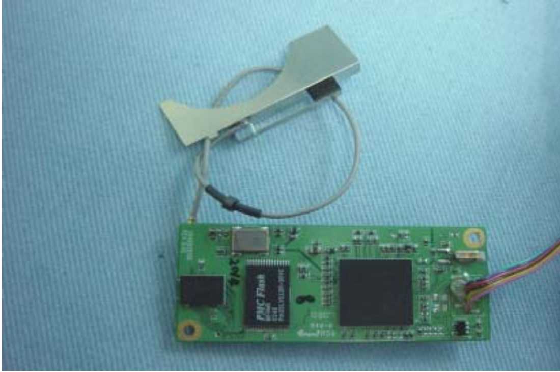
Front View of Antenna
